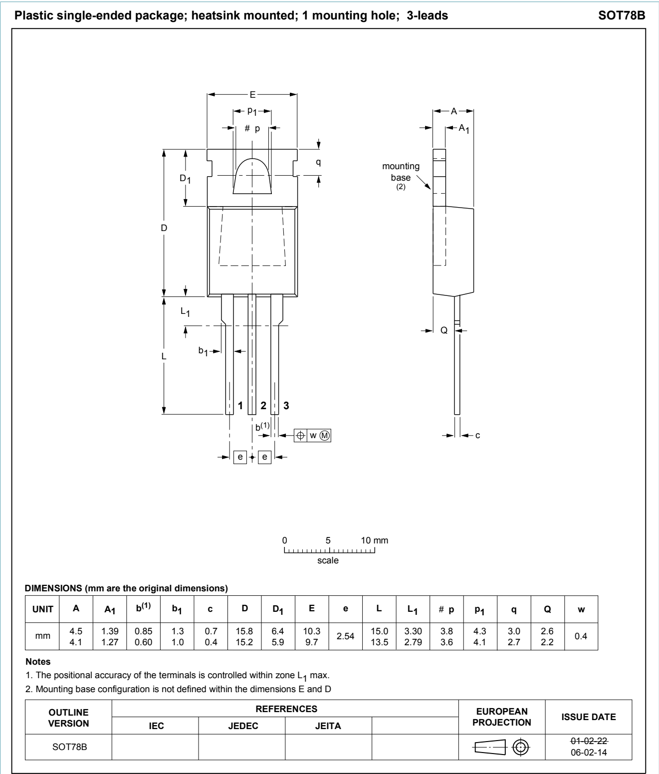
Fig. 1. Package outline TO-220AB (SOT78B)
