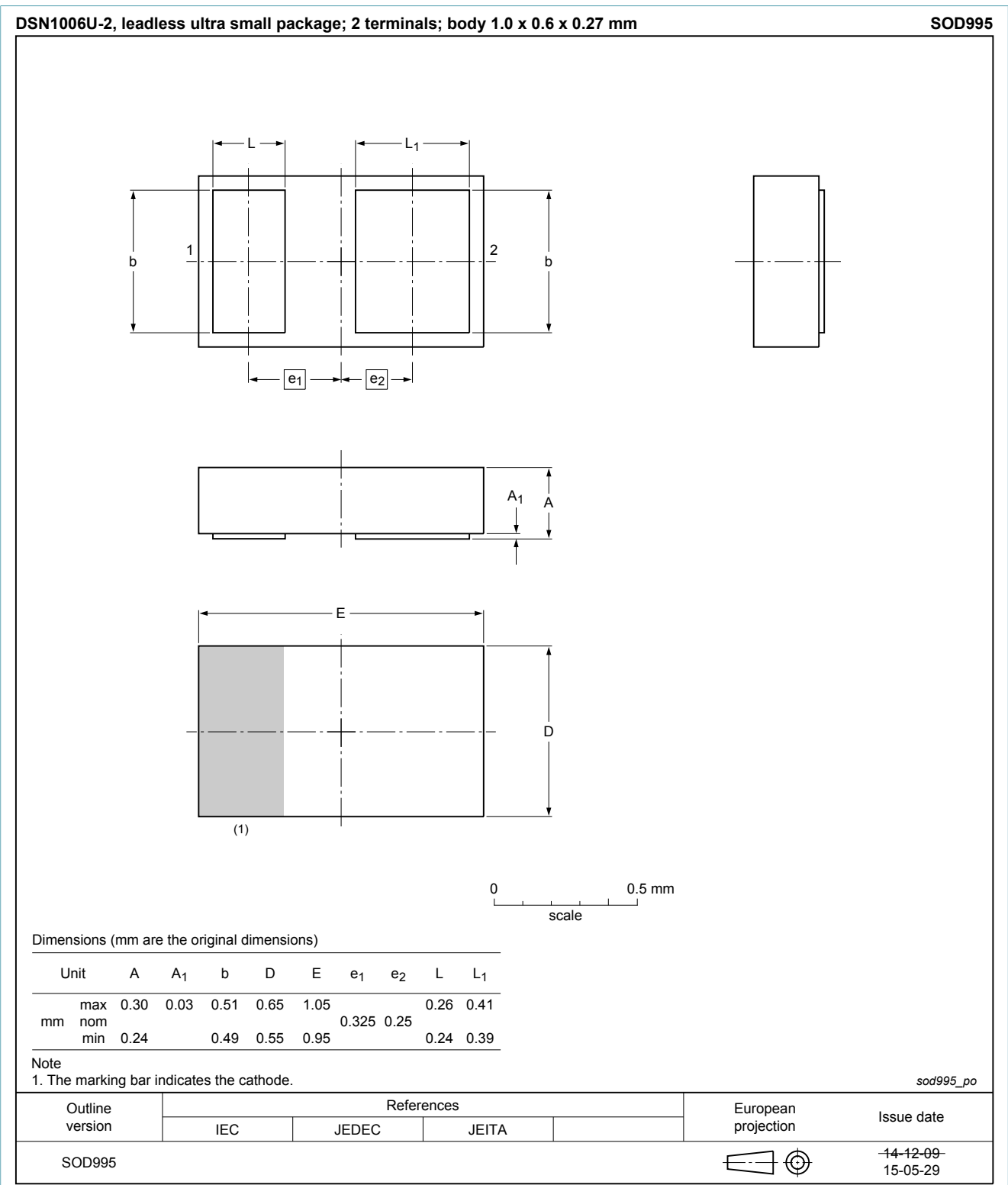
Fig. 1. Package outline DSN1006U-2 (SOD995)
