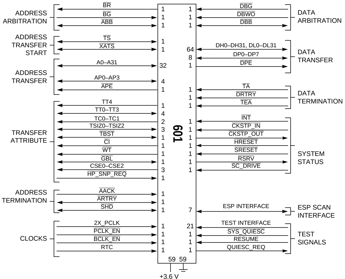
Figure 1-7. PowerPC 601 Microprocessor Signal Groups
