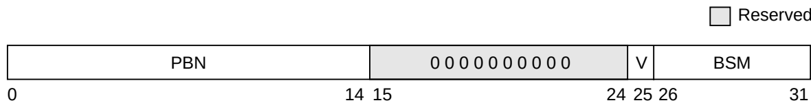
Figure 2-24. Lower BAT Register
