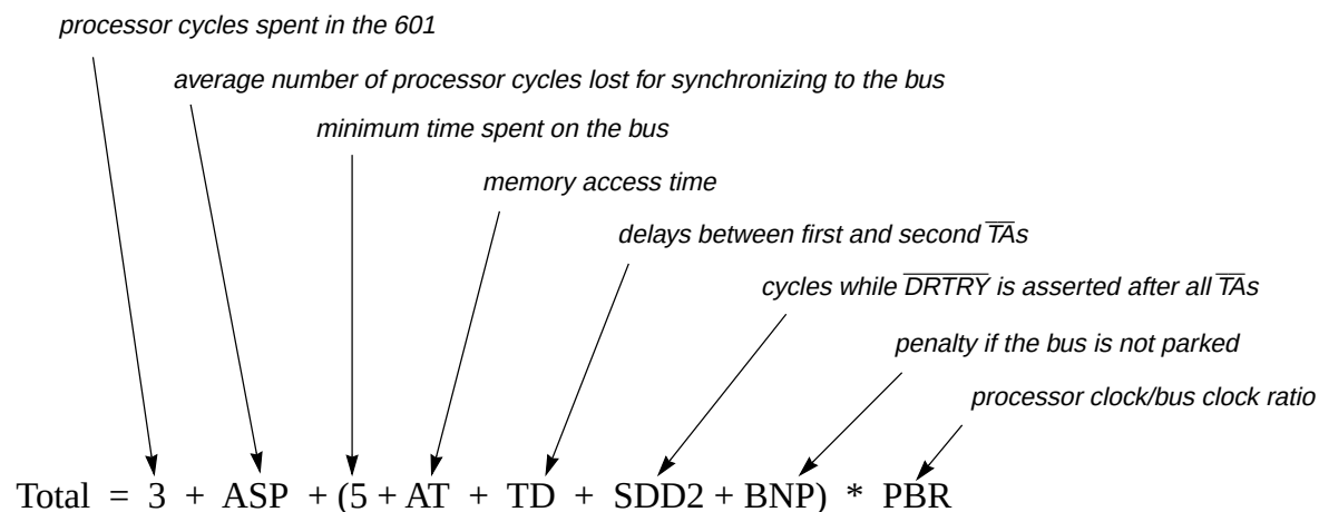
Figure 7-10. Formula for Calculating Total Time from Cache Miss to Data Available for Next Cache Hit (Processor Clock \neq Bus Clock)
