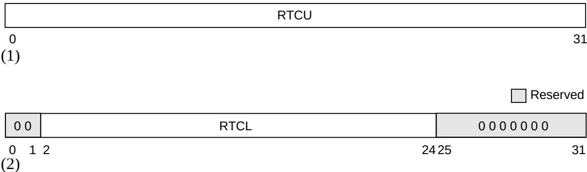
Figure 2-8. Real-Time Clock (RTC) Registers
