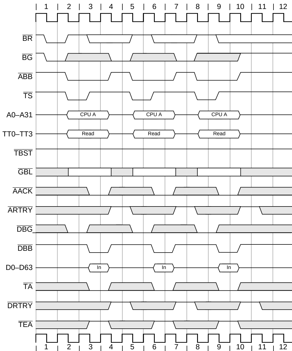
Figure 9-16. Fastest Single-Beat Reads
