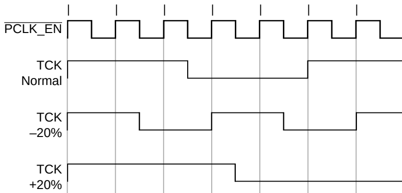
Figure 9-29. IEEE 1149.1 Interface TCK Requirements
