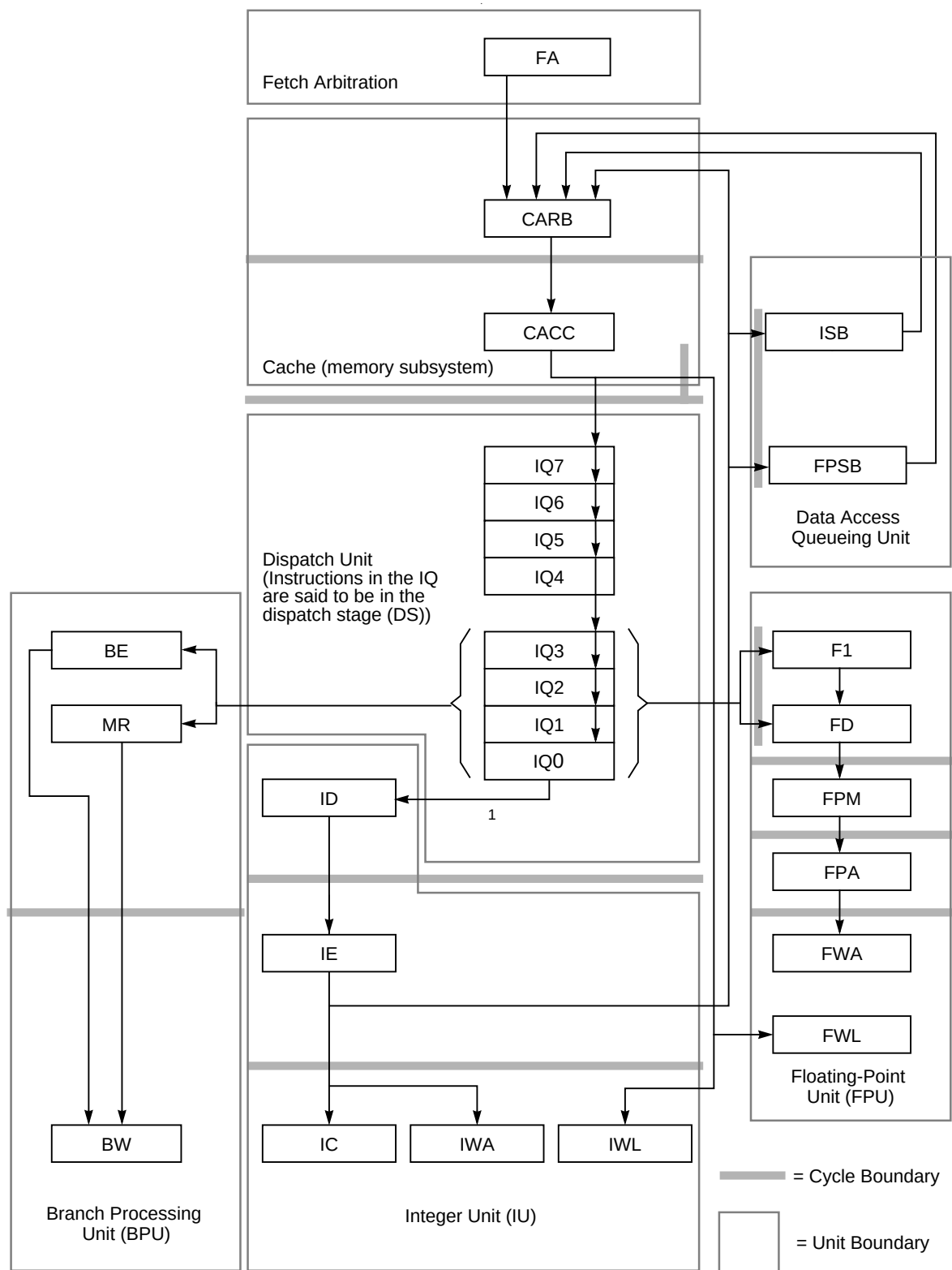
Figure 1-5. Pipeline Diagram of the Processor Core
