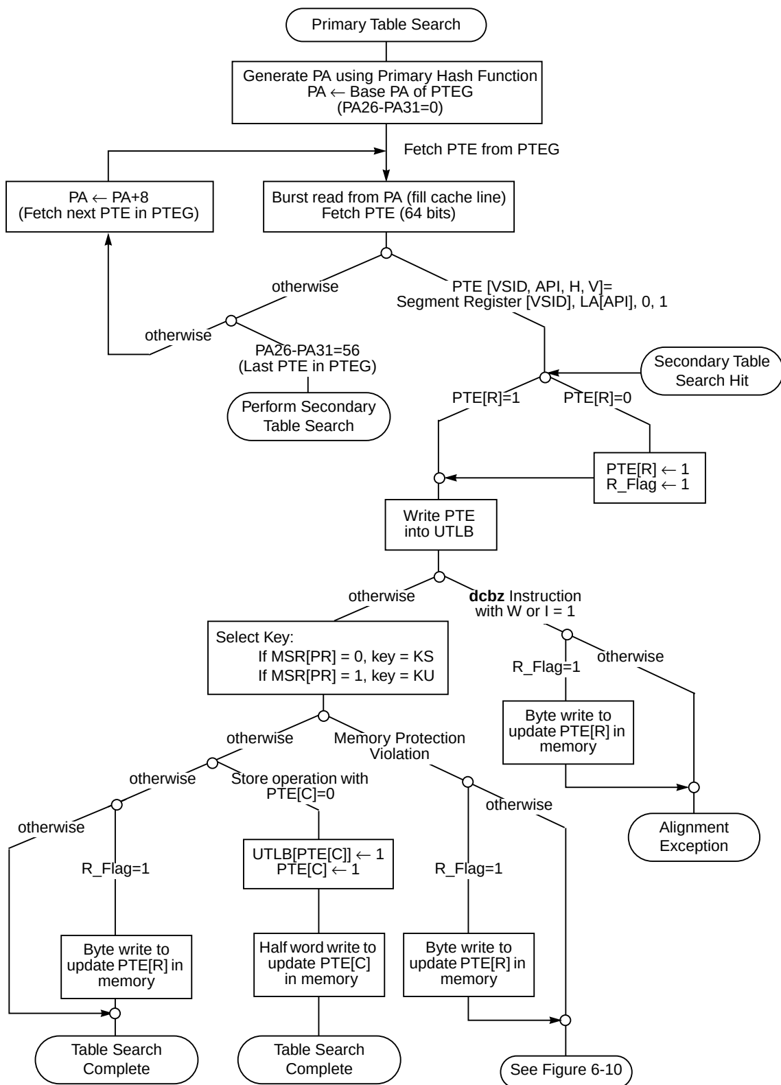
Figure 6-23. Primary Table Search Flow
