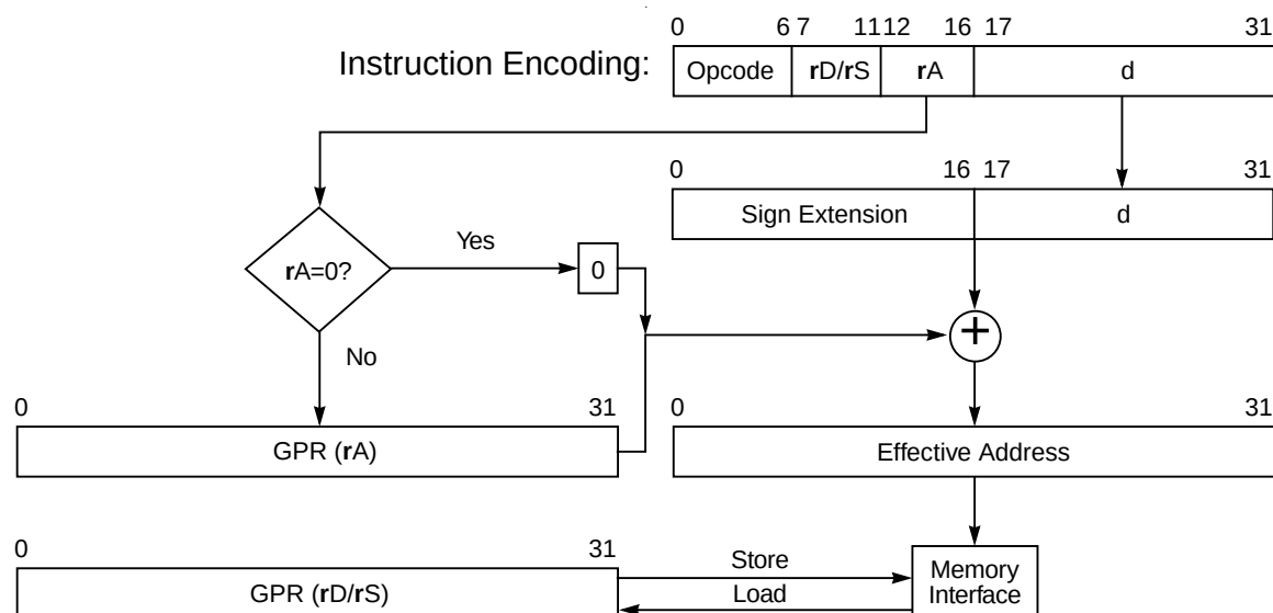
Figure 3-1. Register Indirect with Immediate Index Addressing
