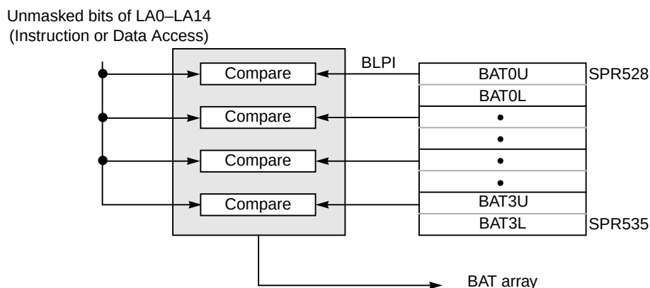
Figure 6-5. BAT Array Organization
