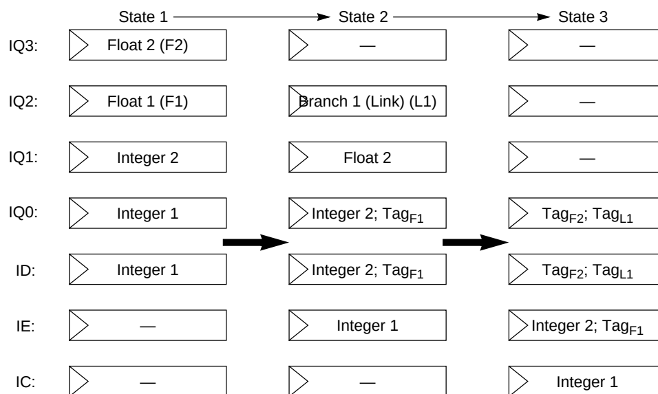
Figure 7-12. Instruction Tagging in the IU Pipeline
