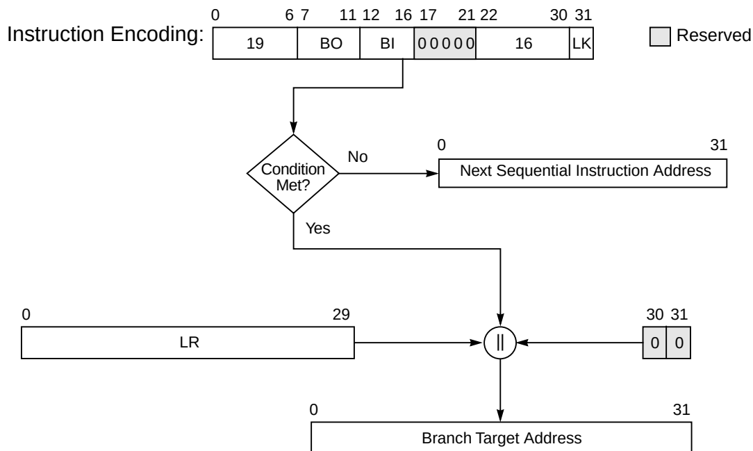
Figure 3-10. Branch Conditional to Link Register Addressing
