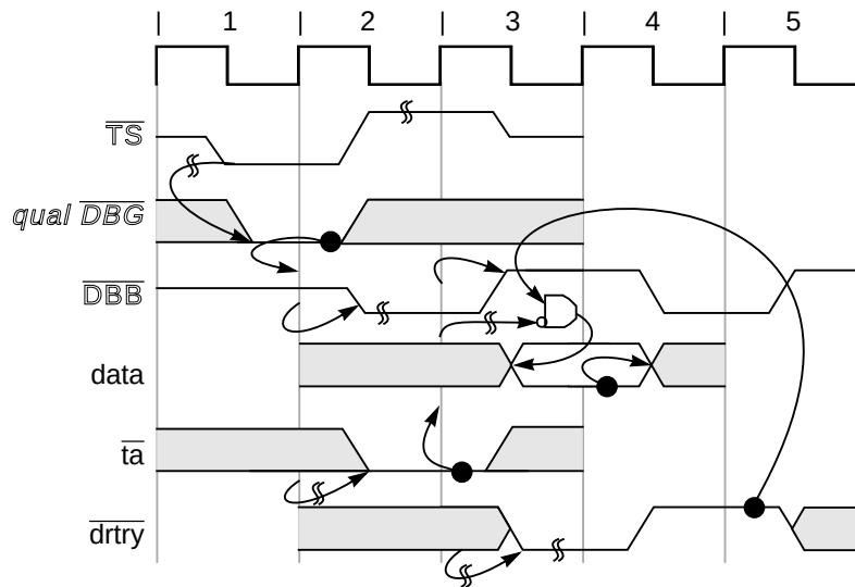
Figure 9-13. Termination with \overline{\text{DRTRY}}
