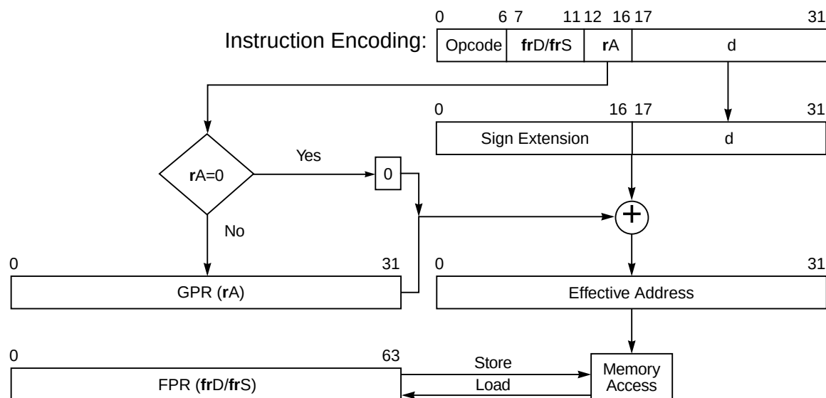
Figure 3-4. Register Indirect with Immediate Index Addressing
