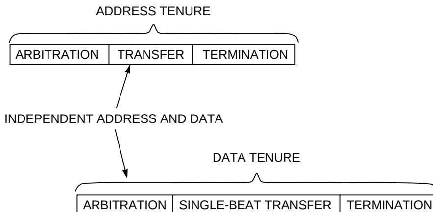
Figure 9-3. Overlapping Tenures on the PowerPC 601 Microprocessor Bus for a Single-Beat Transfer
