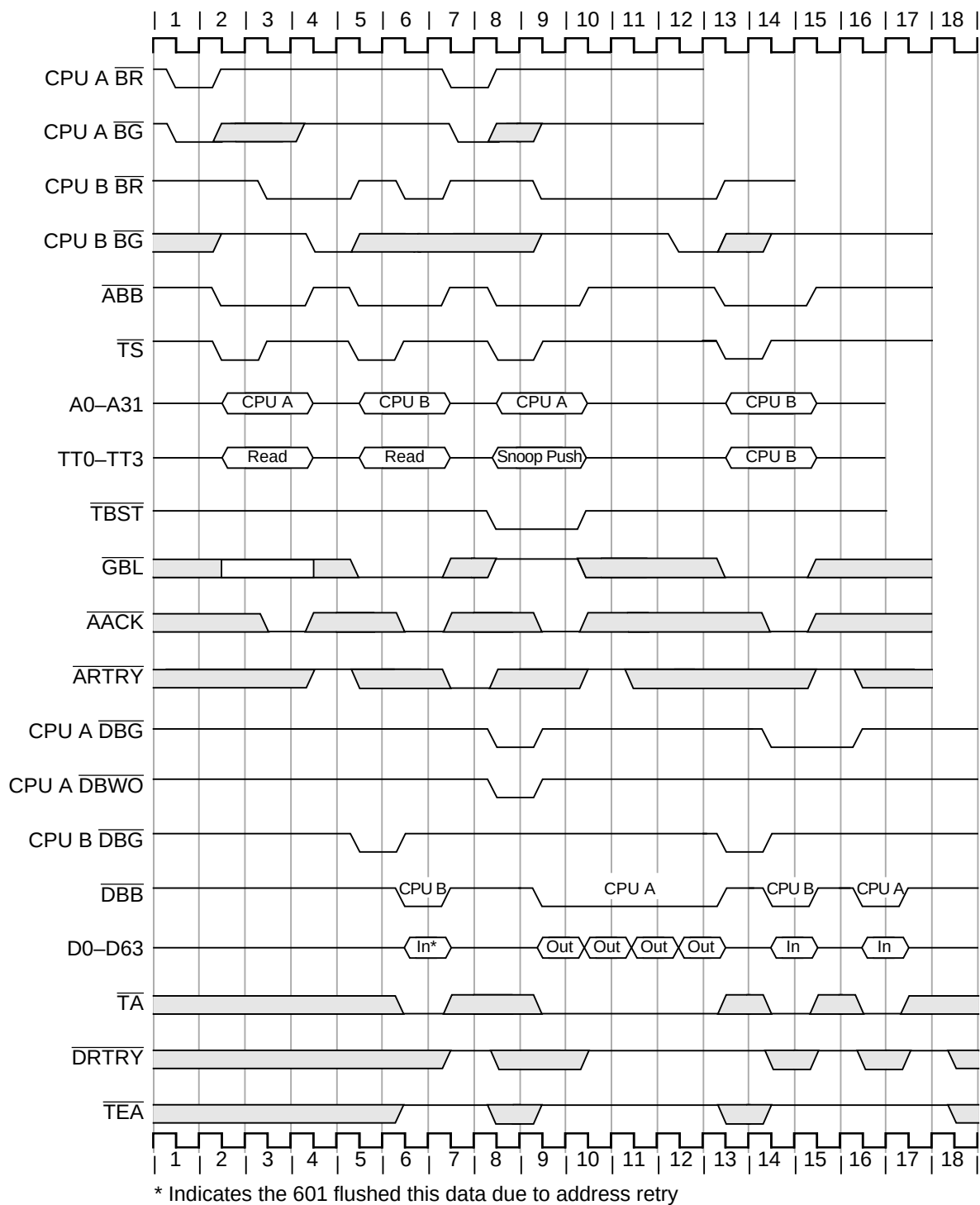
Figure 9-31. Data Bus Write-Only Transaction
