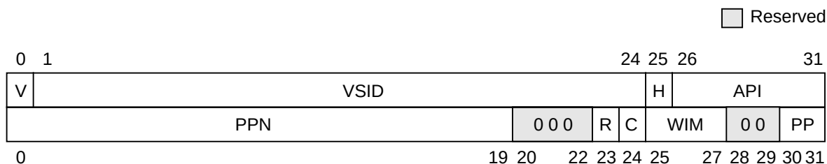
Figure 6-14. Page Table Entry Format
