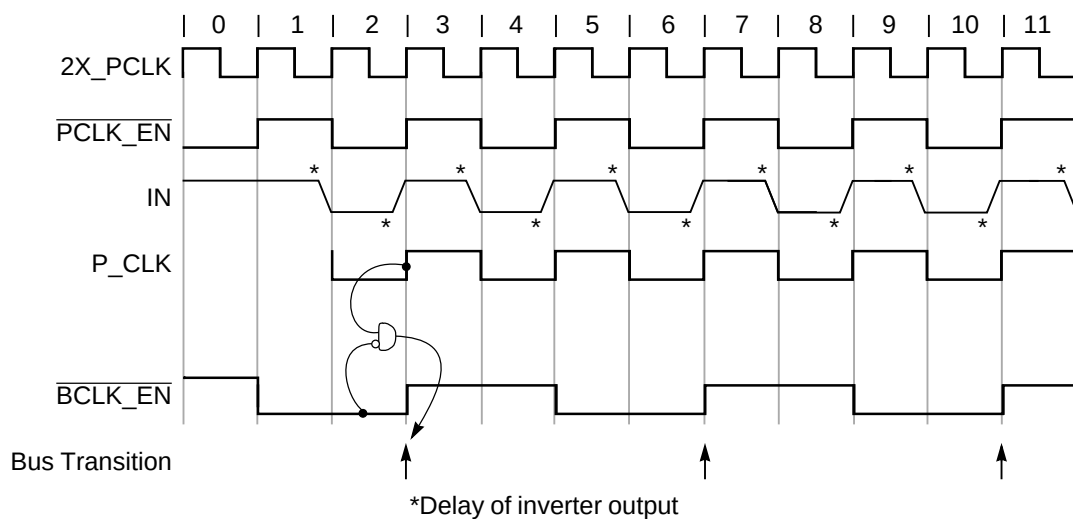
Figure 8-6. Generation of Bus Transitions—Logical Bus Clock = 1/2 P_CLK
