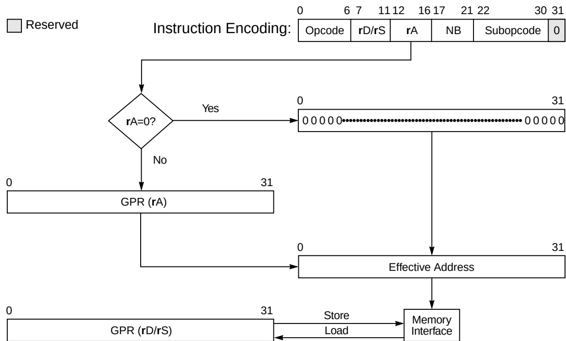
Figure 3-3. Register Indirect Addressing
