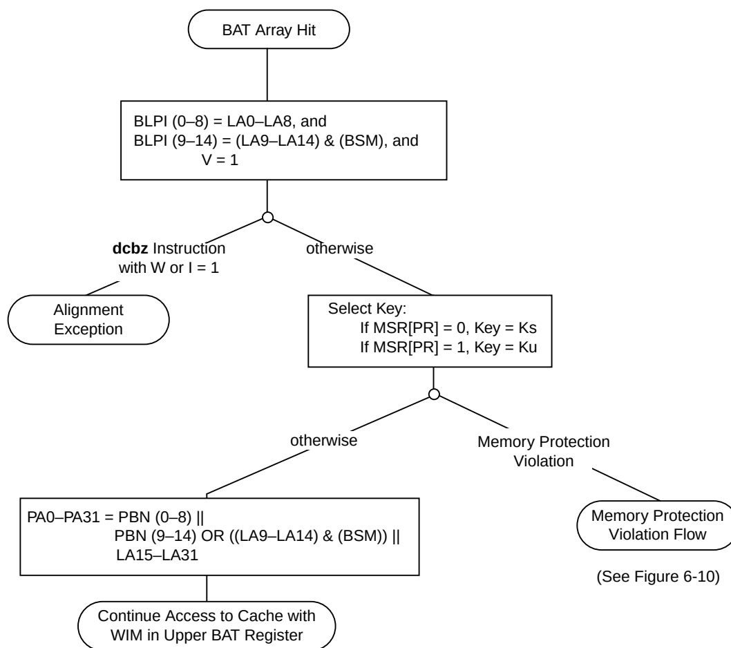
Figure 6-9. Block Address Translation Flow
