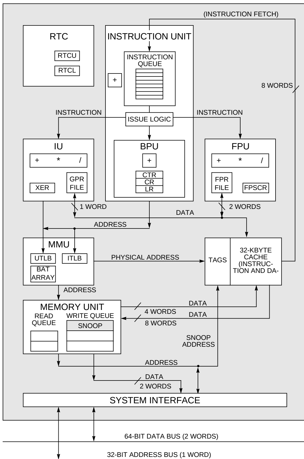
Figure 1-1. PowerPC 601 Microprocessor Block Diagram
