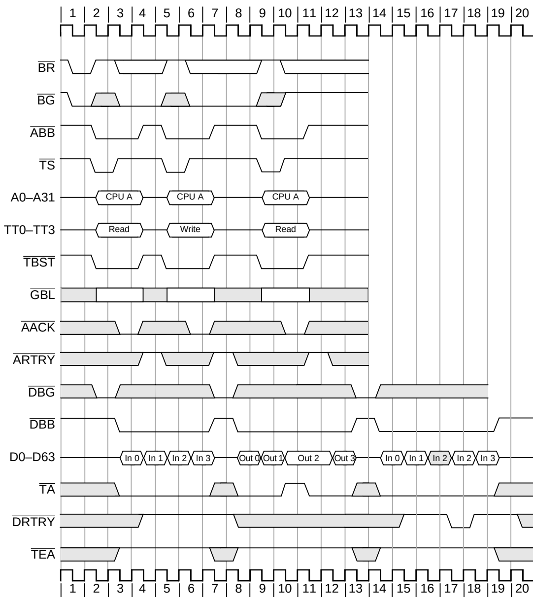
Figure 9-21. Burst Transfers with Data Delay Controls
