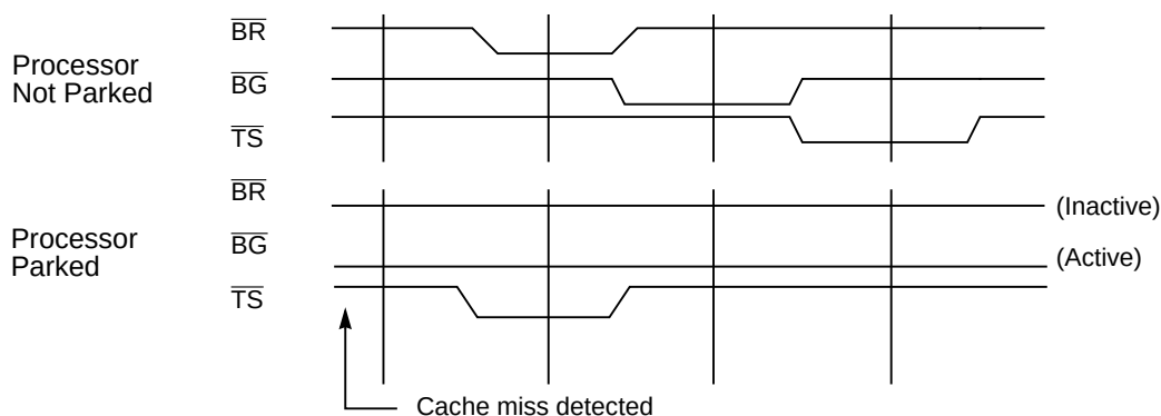
Figure 7-3. Bus Timing for Parked and Nonparked Bus Masters
