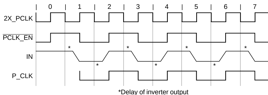
Figure 8-4. Generation of Internal Clock (P_CLK)
