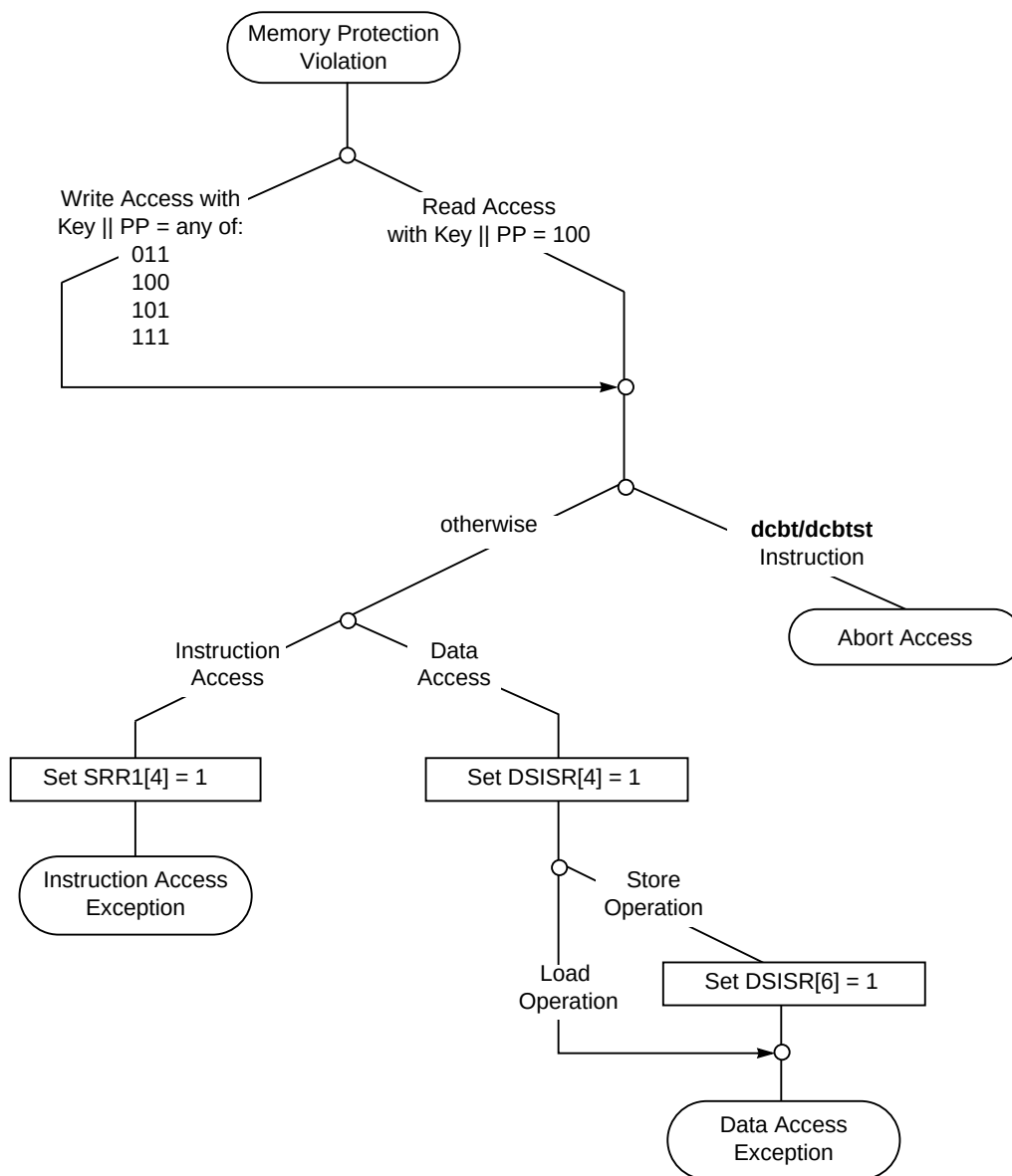
Figure 6-10. Memory Protection Violation Flow
