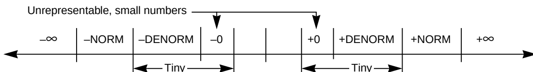
Figure 2-43. Approximation to Real Numbers
