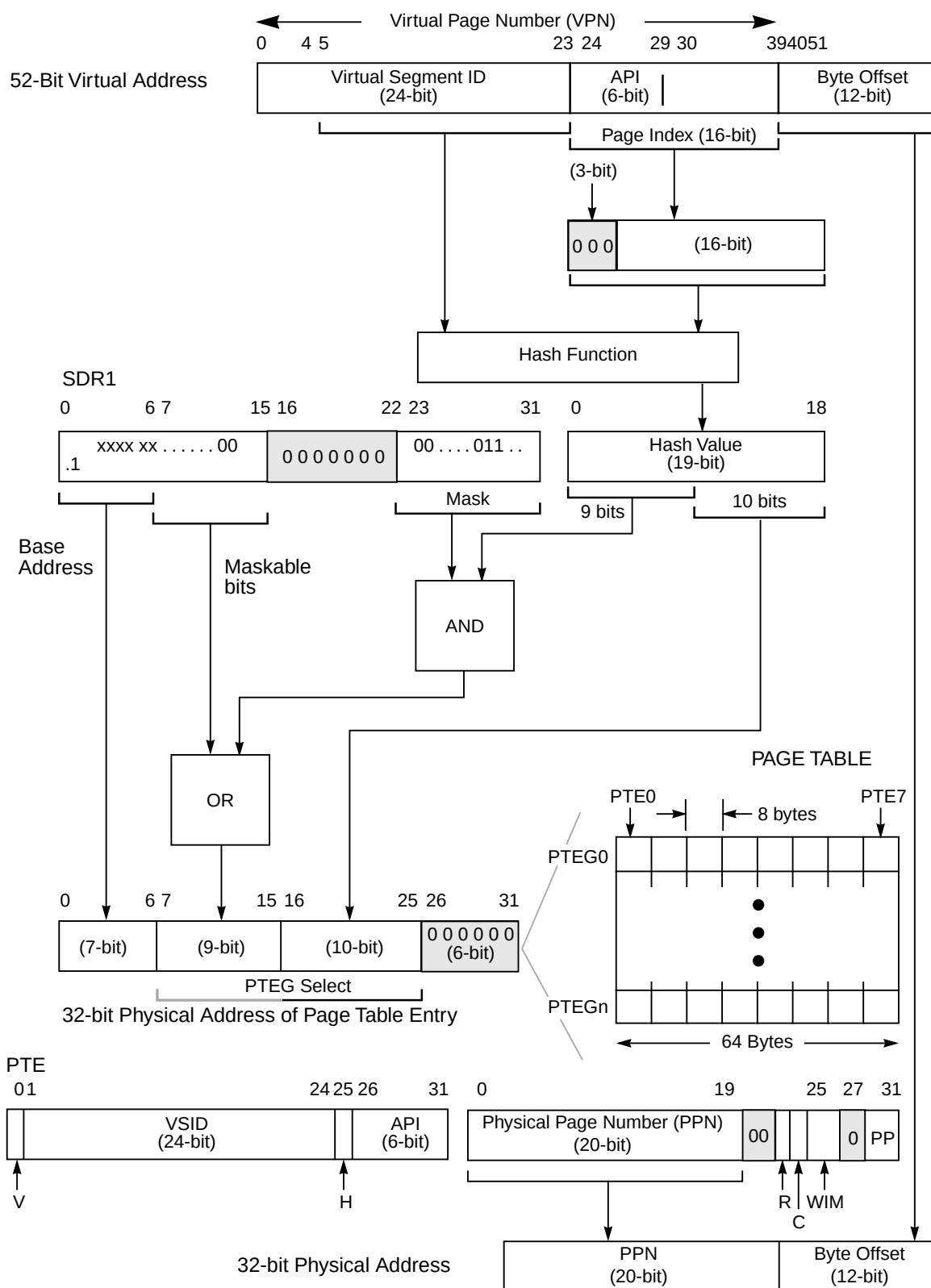
Figure 6-19. Generation of Addresses for Page Tables
