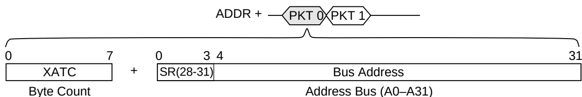
Figure 9-25. I/O Controller Interface Operation—Packet 1
