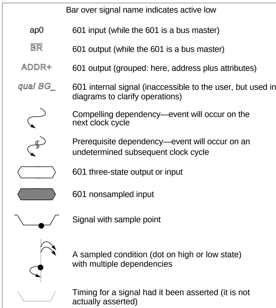
Figure 9-2. Timing Diagram Legend
