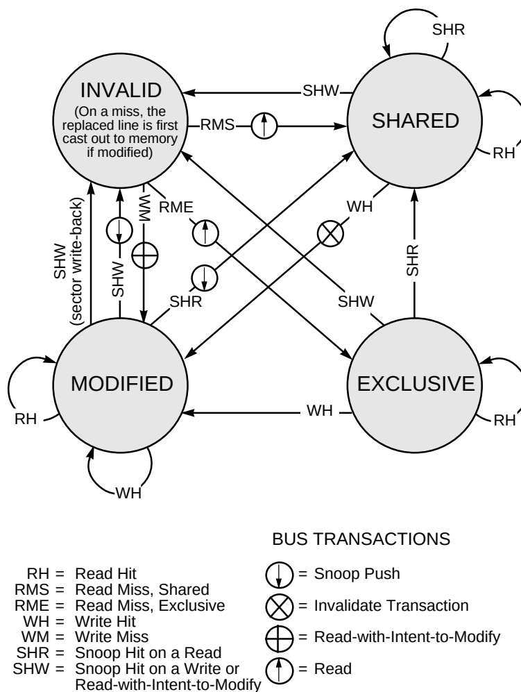
Figure 4-4. MESI Cache Coherency Protocol—State Diagram (WIM = 001)
