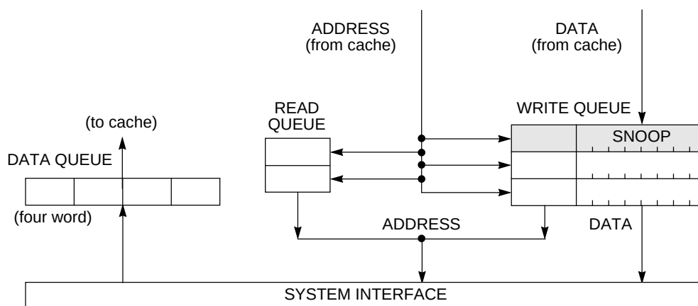
Figure 4-5. Memory Unit
