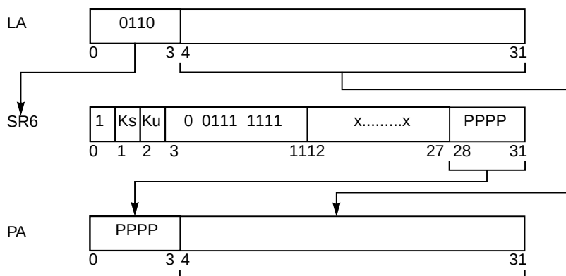
Figure 6-26. Memory-Forced I/O Controller Interface Access Example
