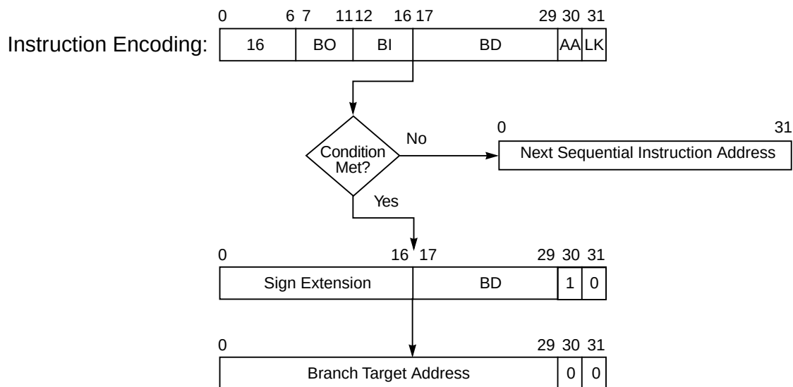
Figure 3-9. Branch Conditional to Absolute Addressing
