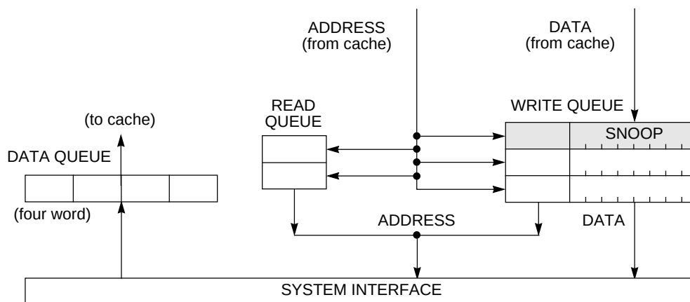
Figure 1-2. Memory Unit
