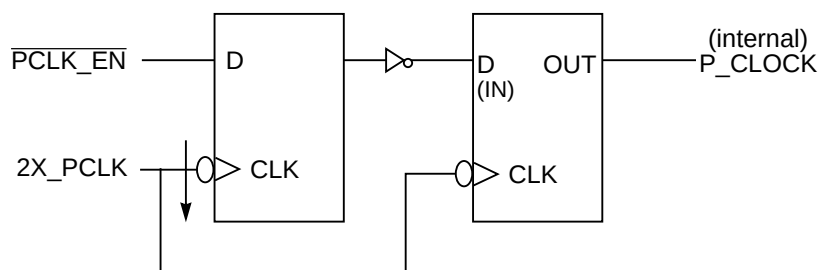
Figure 8-3. Internal P_CLOCK Generation
