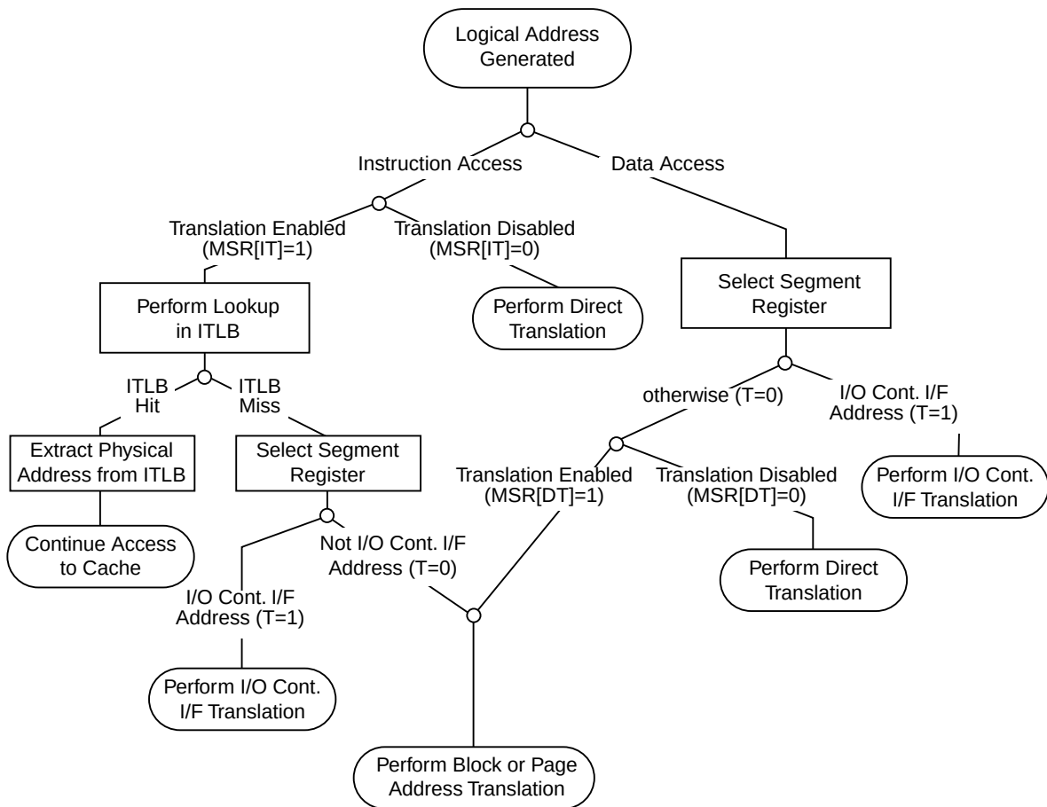
Figure 6-4. Address Translation Type Selection
