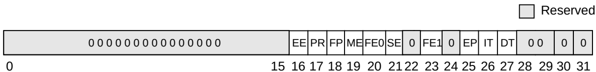
Figure 5-4. Machine State Register (MSR)
