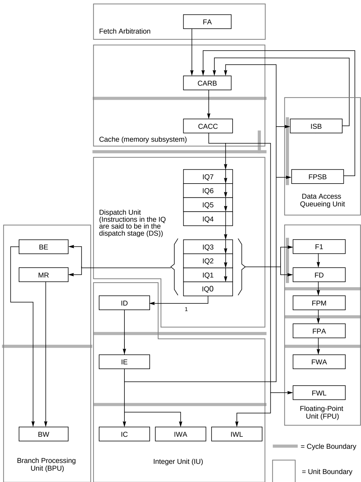
Figure 7-1. Instruction Flow Diagram Showing the Processor Core
