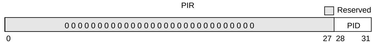
Figure 2-29. Processor Identification Register (PIR)
