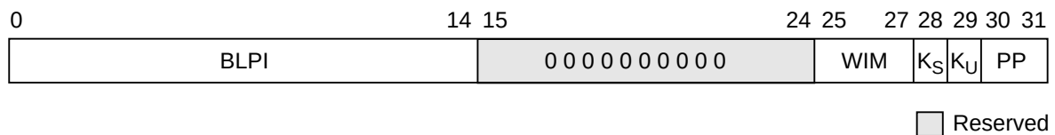
Figure 6-6. Format of Upper BAT Registers
