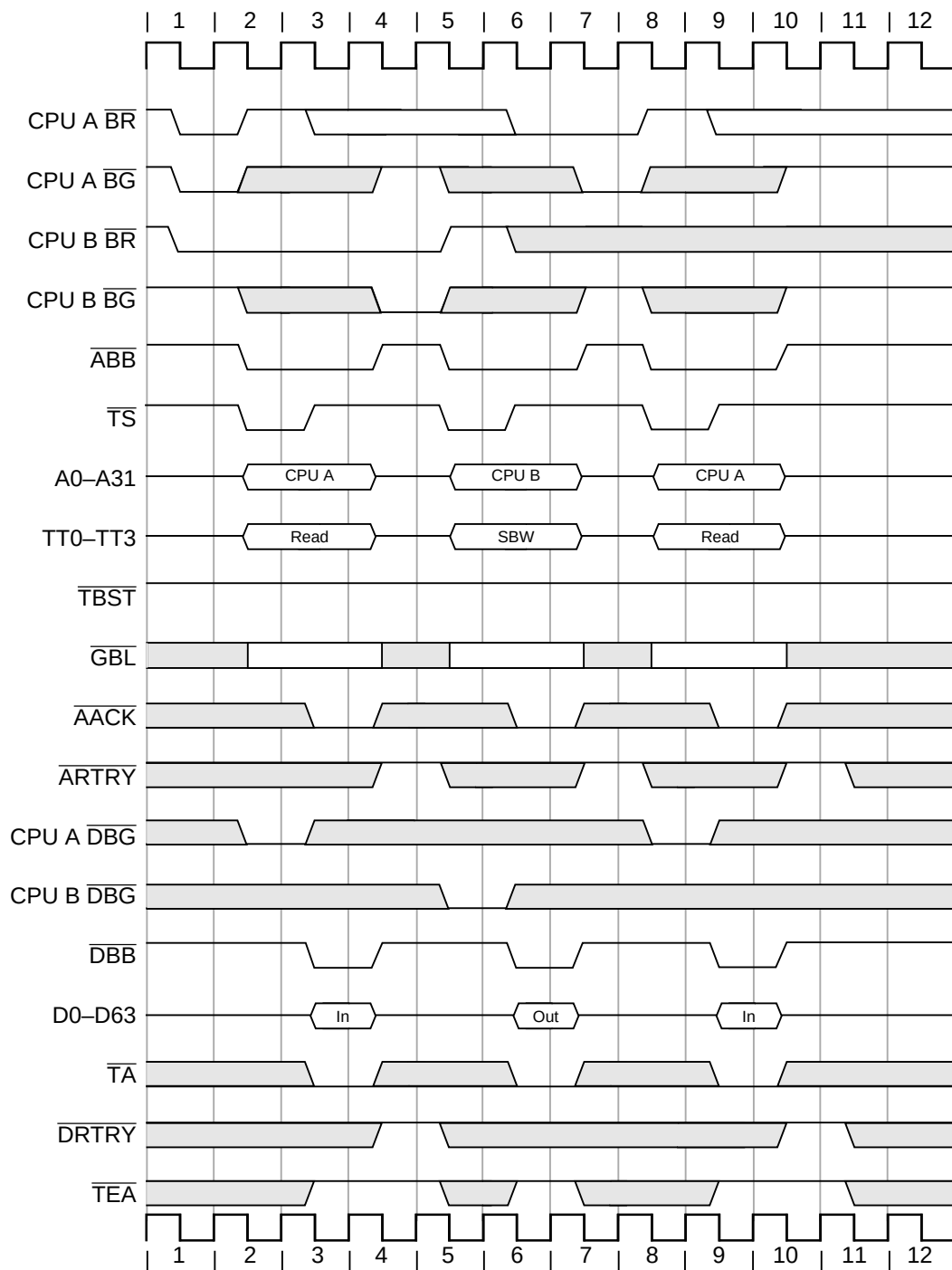
Figure 9-20. Back-to-Back Single-Beat Transfers
