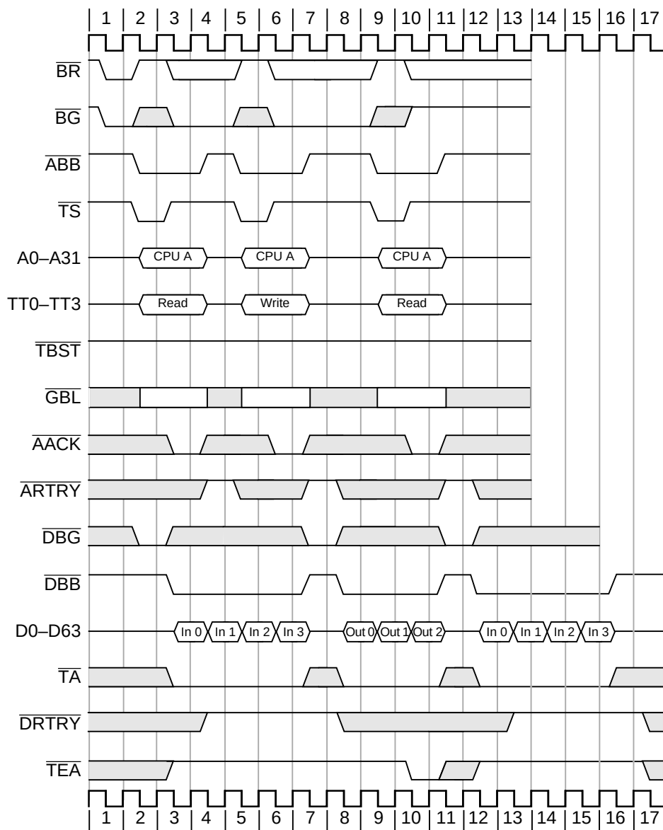
Figure 9-22. Use of Transfer Error Acknowledge ( \overline{\text{TEA}} )
