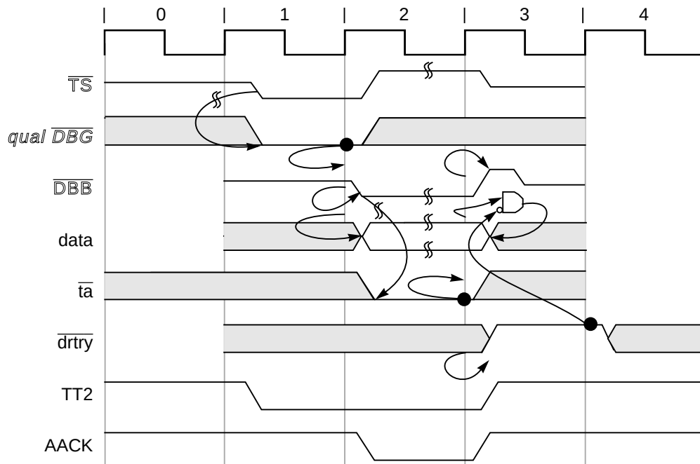
Figure 9-10. Normal Single-Beat Read Termination
