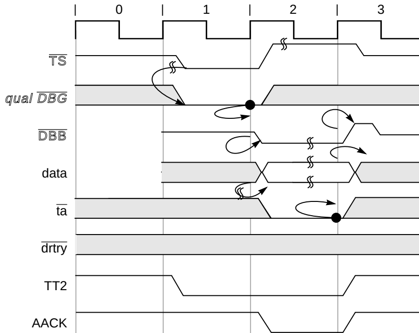
Figure 9-11. Normal Single-Beat Write Termination
