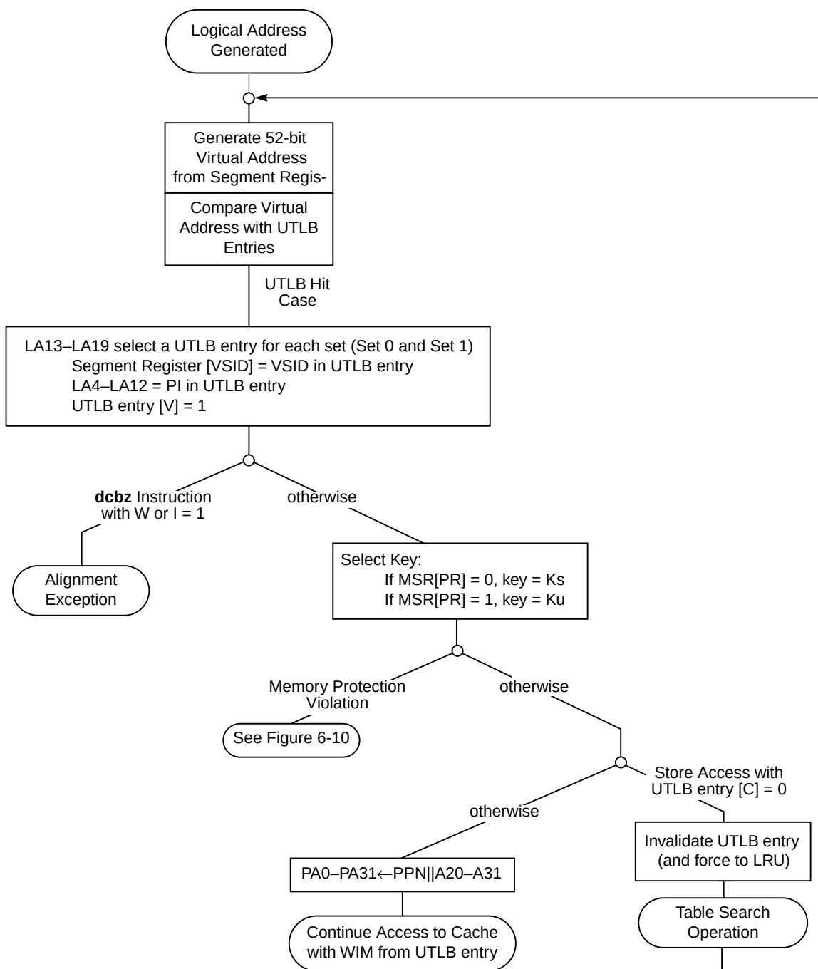
Figure 6-15. Page Address Translation Flow—UTLB Hit
