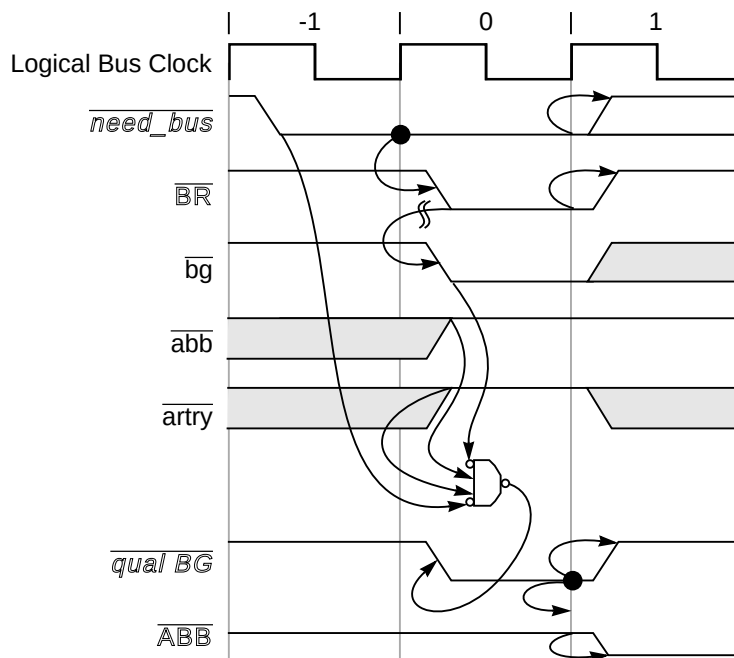
Figure 9-4. Address Bus Arbitration
