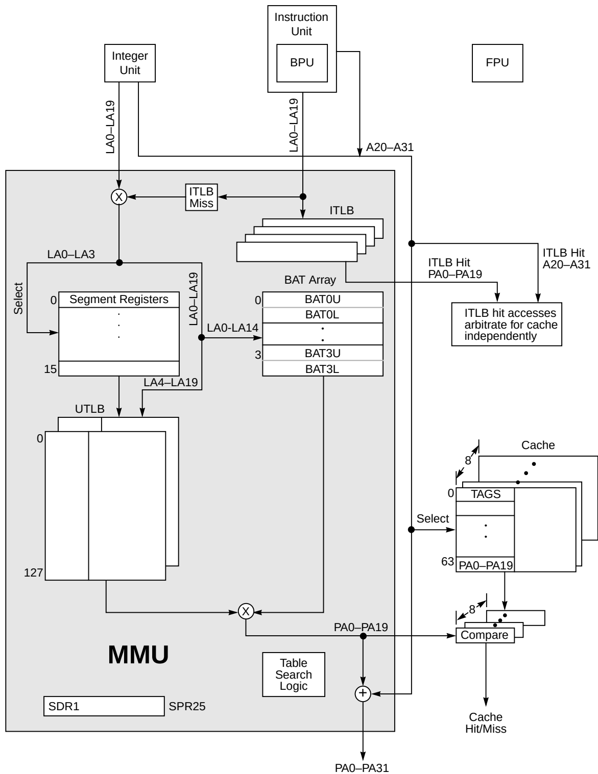
Figure 6-1. MMU Block Diagram
