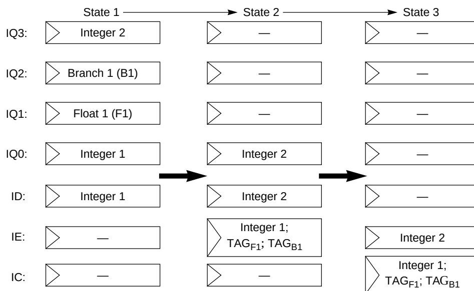
Figure 7-11. Collapsing of Instruction Stream after Out-of-Order Dispatch
