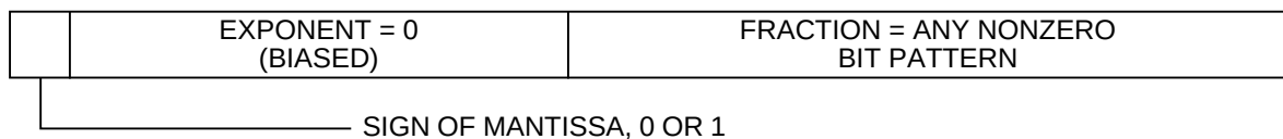
Figure 2-46. Format for Denormalized Numbers
