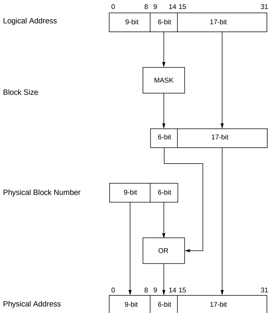
Figure 6-8. Block Physical Address Generation
