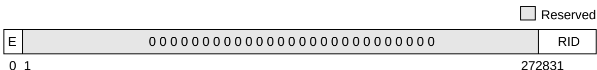
Figure 2-21. External Access Register (EAR)
