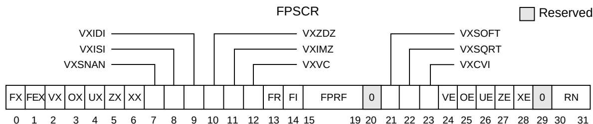
Figure 2-4. Floating-Point Status and Control Register (FPSCR)
