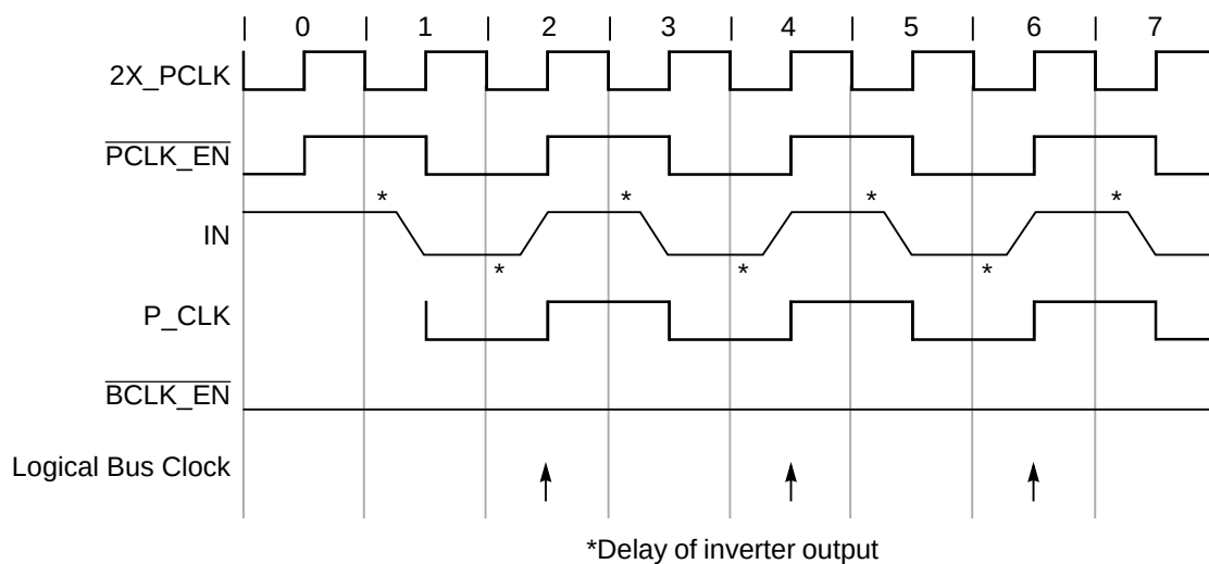
Figure 8-5. Generation of Bus Transitions—Logical Bus Clock = P_CLK
