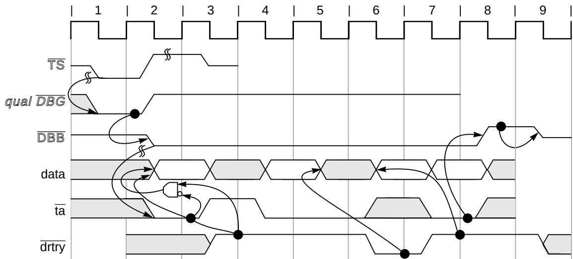
Figure 9-14. Read Burst with \overline{TA} Wait States and \overline{DRTRY}
