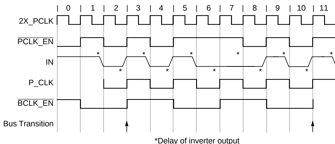
Figure 8-8. Generation of Bus Transitions—Cycle Stretching
