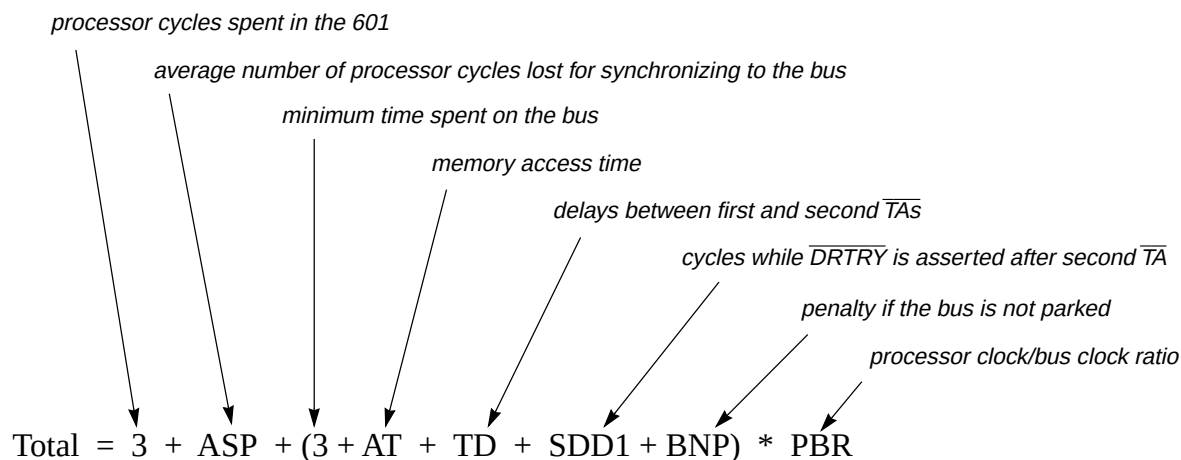
Figure 7-9. Formula for Calculating Total Time from Cache Miss to Dependent Operation Execution (Processor Clock/Bus Clock \neq 1:1)
