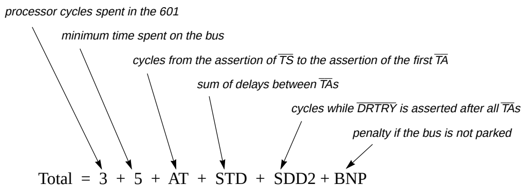
Figure 7-7. Formula for Calculating Total Time from Cache Miss to Data Available for the Next Cache Hit
