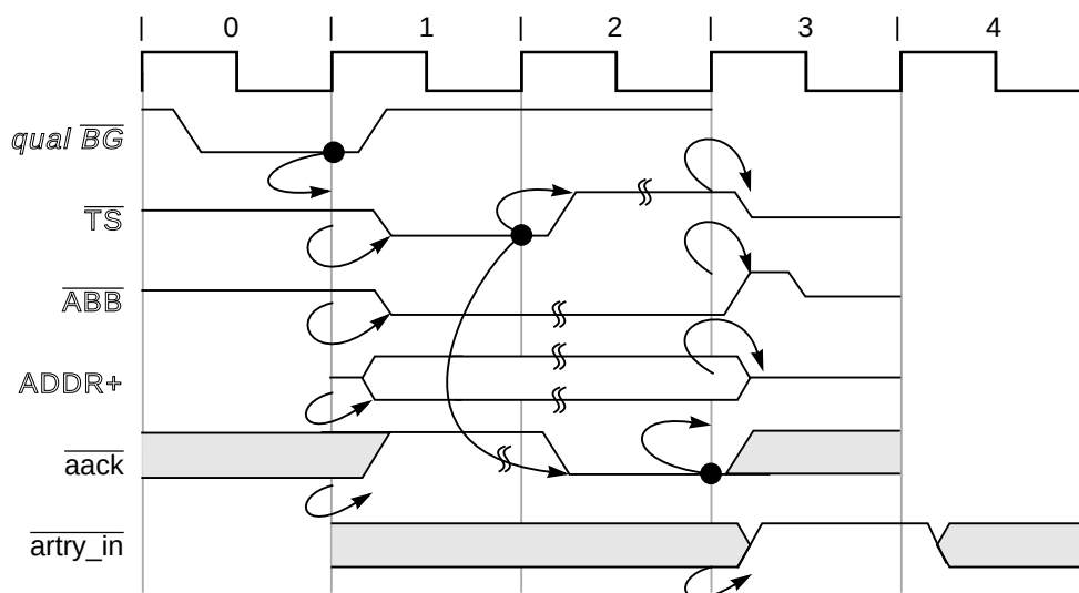
Figure 9-6. Address Bus Transfer
