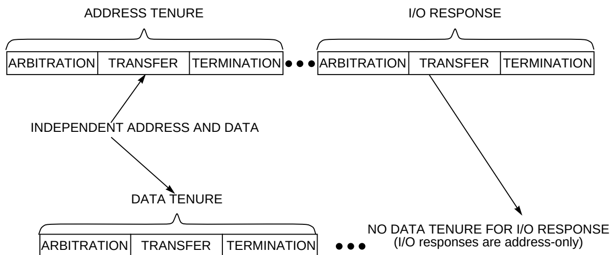
Figure 9-23. I/O Controller Interface Tenures
