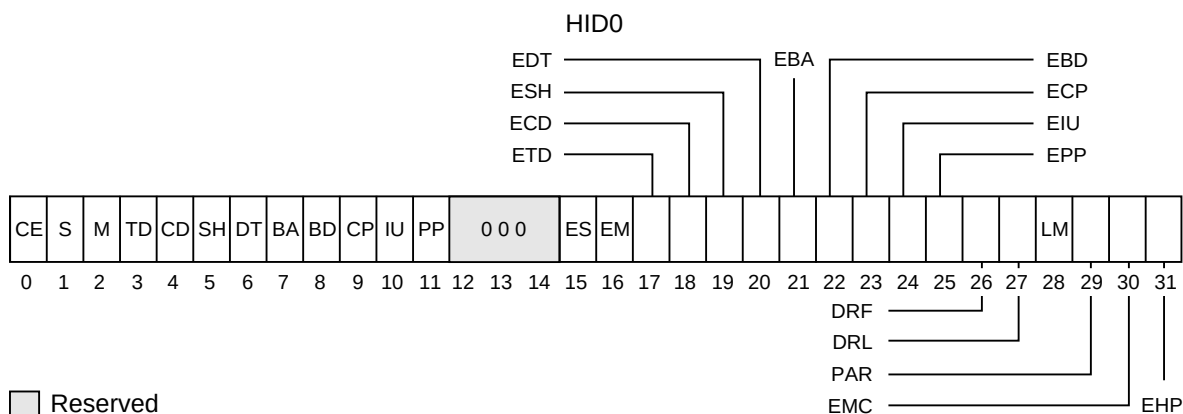
Figure 2-25. Checkstop Sources and Enables Register (HID0)
