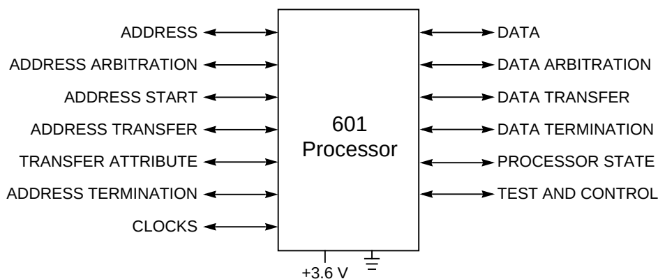
Figure 1-6. System Interface
