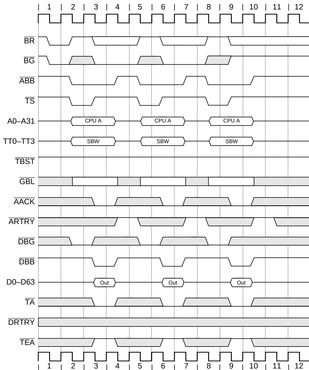
Figure 9-17. Fastest Single-Beat Writes
