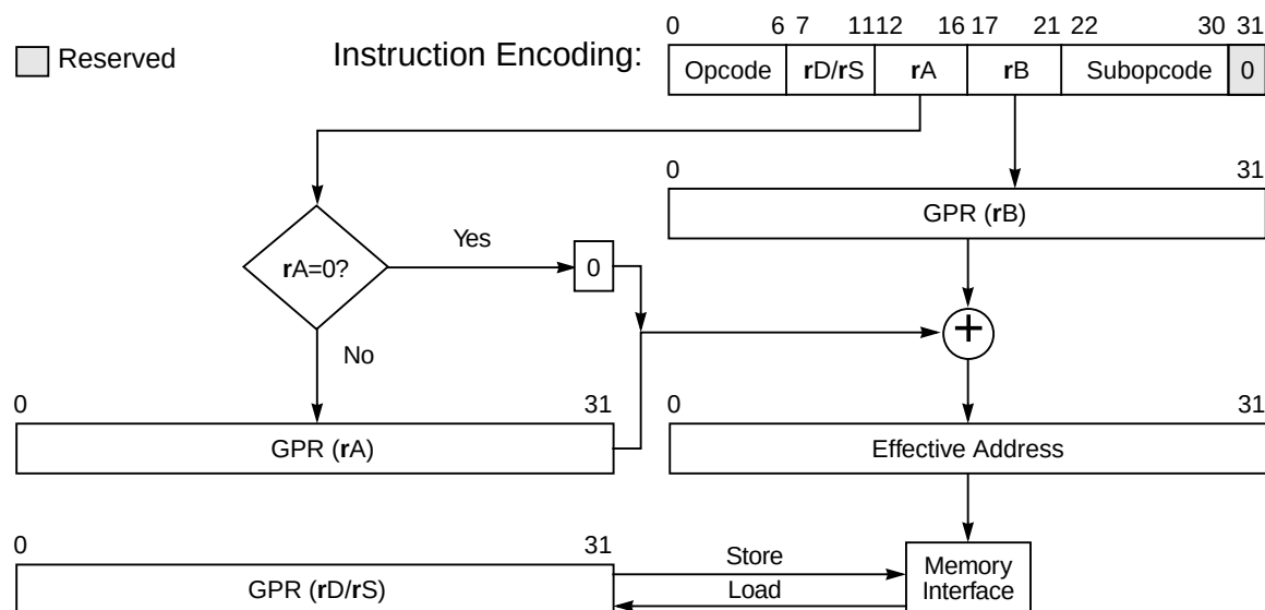
Figure 3-2. Register Indirect with Index Addressing
