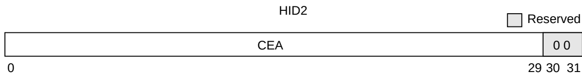
Figure 2-27. Instruction Address Breakpoint Register (IABR)— HID2
