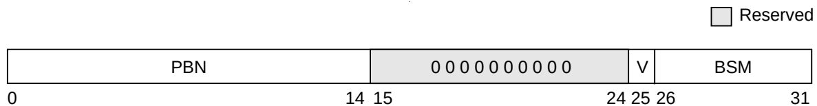
Figure 6-7. Format of Lower BAT Registers
