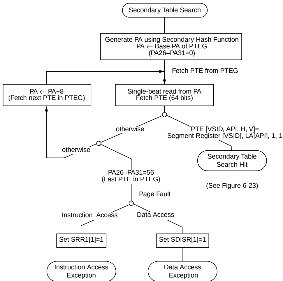
Figure 6-24. Secondary Table Search Flow
