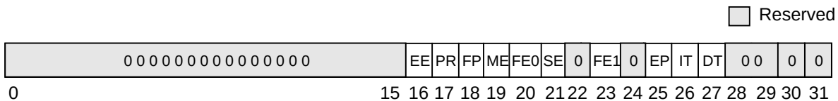
Figure 2-11. Machine State Register (MSR)
