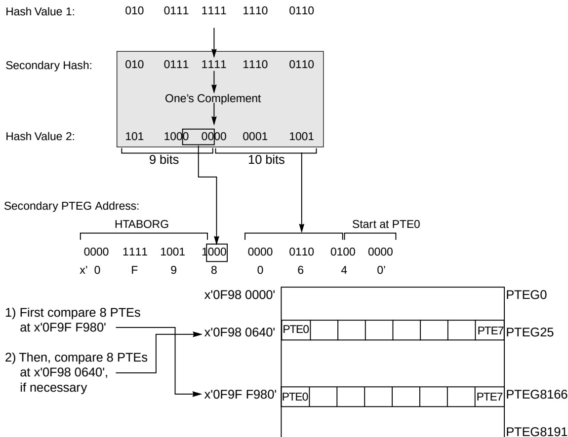
Figure 6-22. Example Secondary PTEG Address Generation
