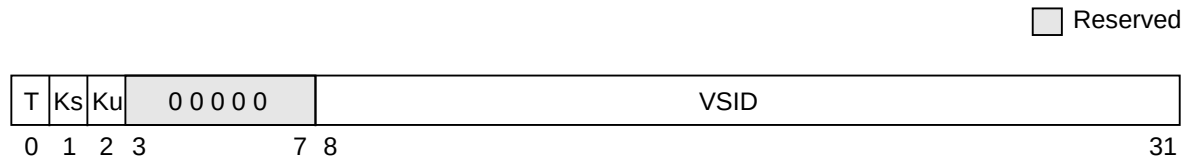
Figure 6-13. Segment Register Format for Page Address Translation
