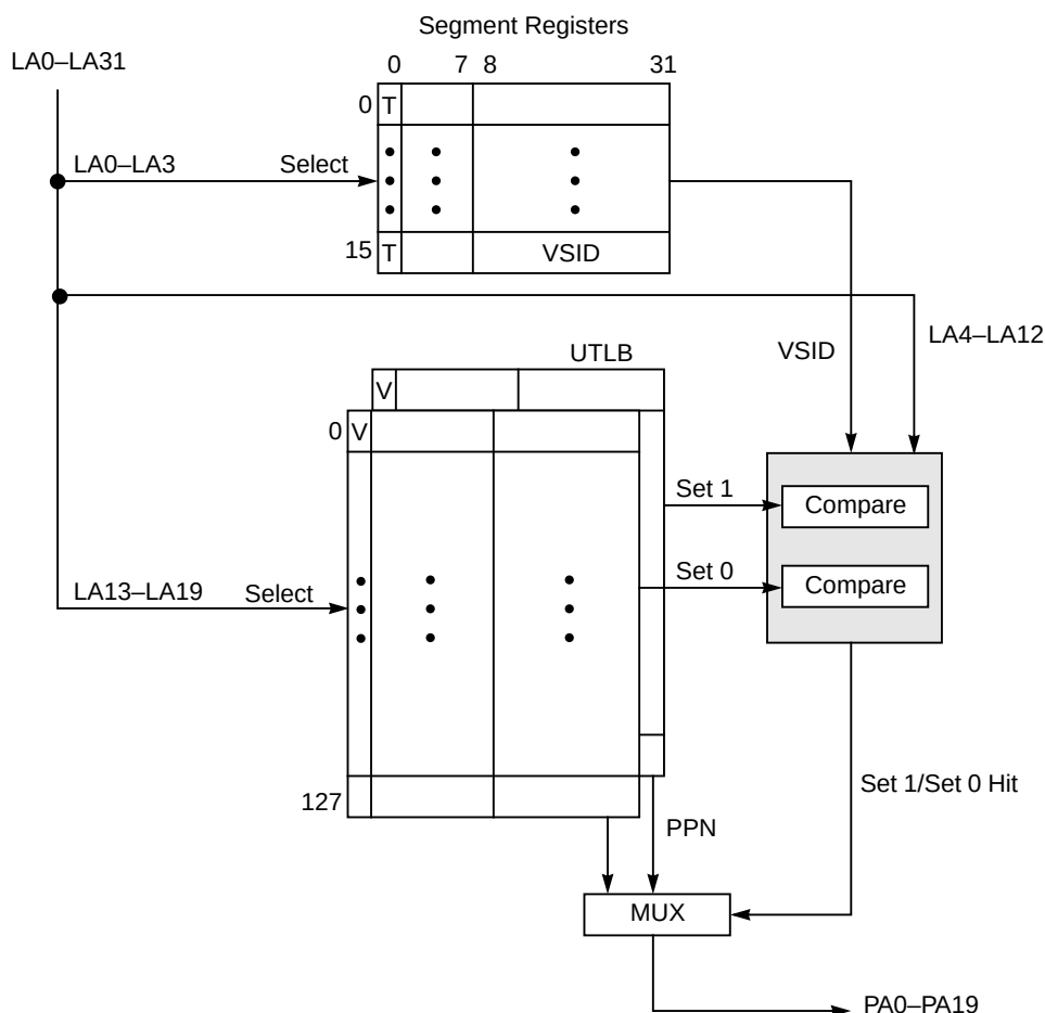
Figure 6-11. Segment Register and UTLB Organization
