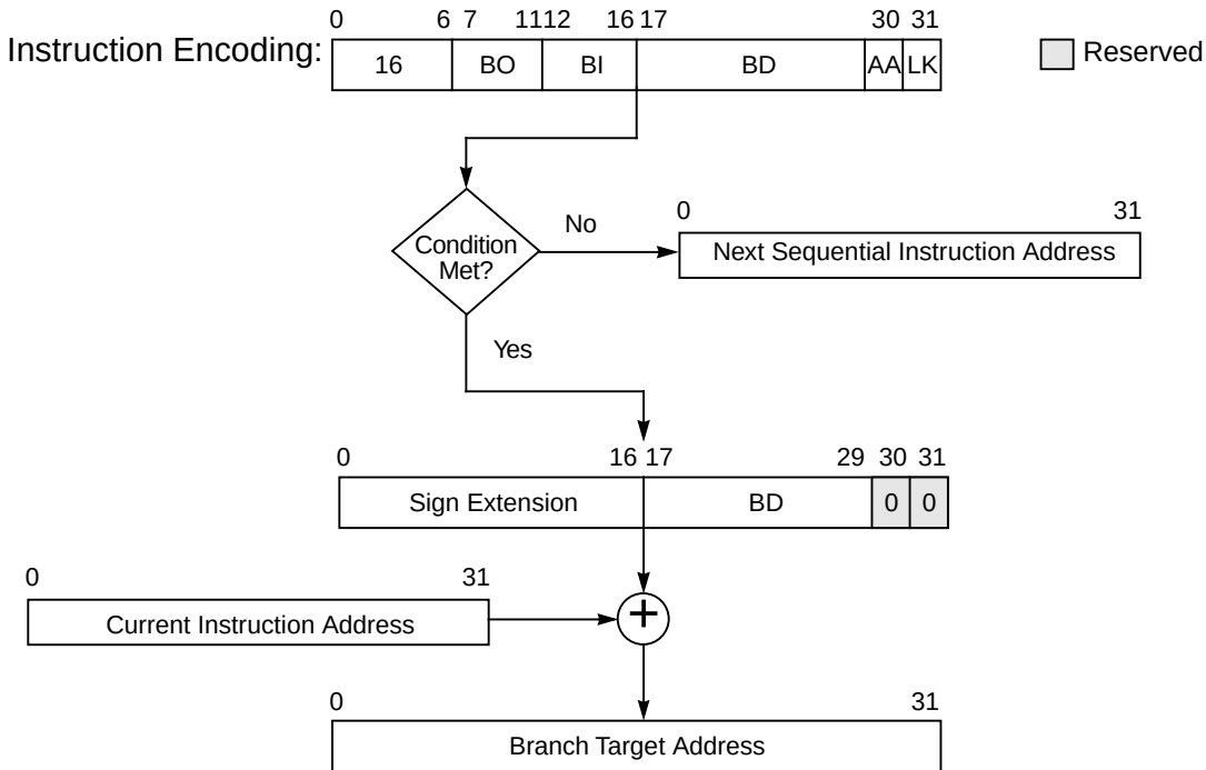
Figure 3-7. Branch Conditional Relative Addressing
