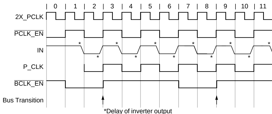
Figure 8-7. Generation of Bus Transitions—Logical Bus Clock=1/3 P_CLK
