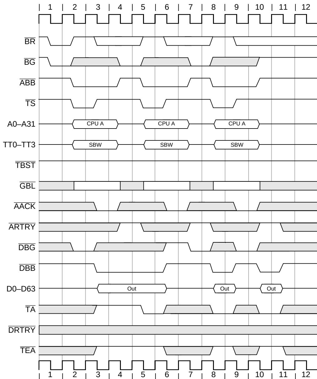
Figure 9-19. Single-Beat Writes Showing Data Delay Controls
