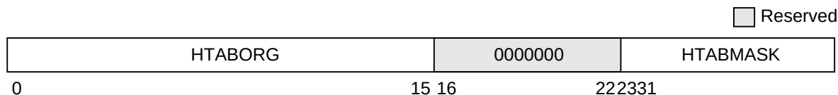
Figure 2-17. Table Search Description Register 1 (SDR1)
