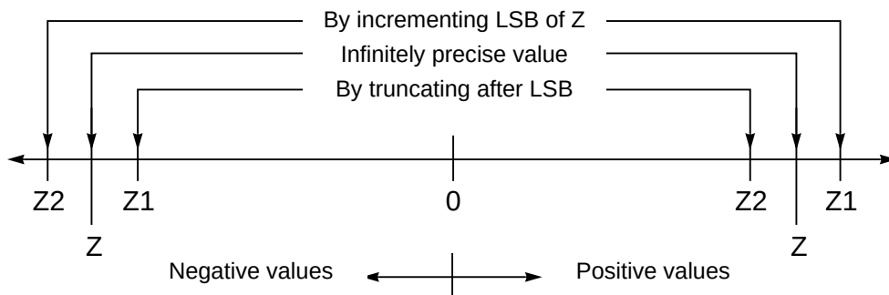
Figure 2-52. Relation of Z1 and Z2
