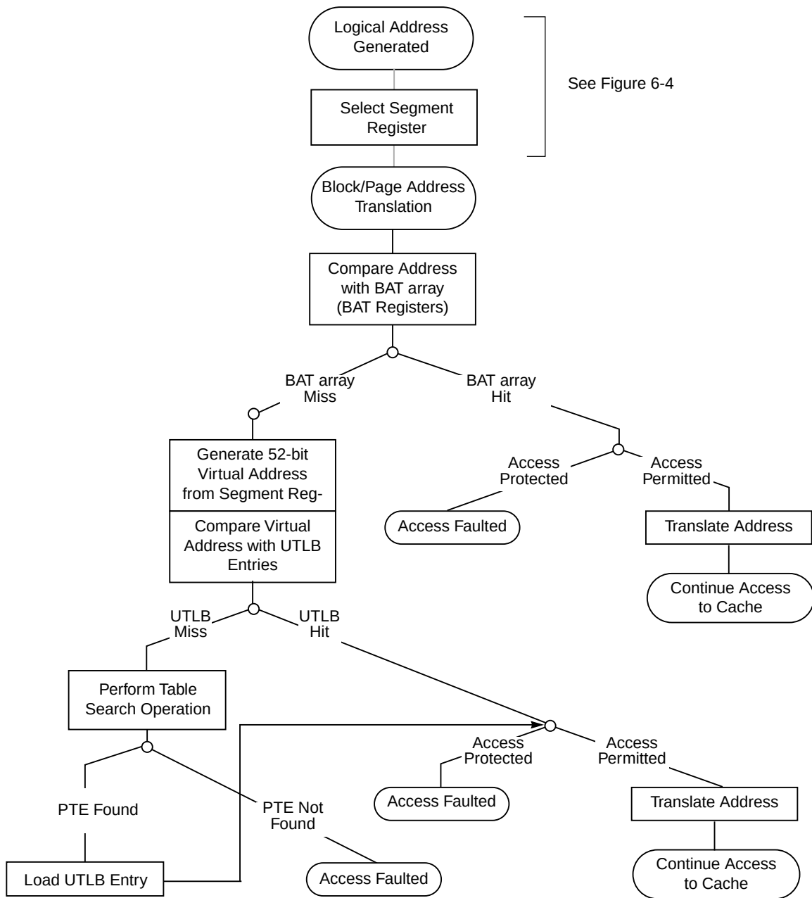
Figure 6-3. MMU Block and Page Address Translation Flow
