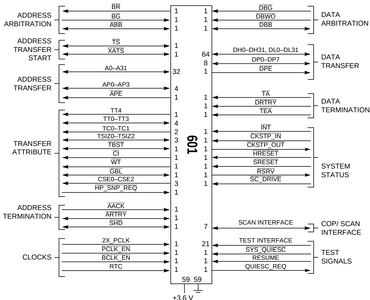
Figure 8-1. PowerPC 601 Microprocessor Signal Groups
