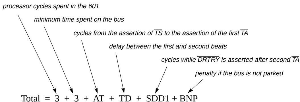
Figure 7-6. Formula for Calculating Total Time from Cache Miss to Execution of Dependent Operation
