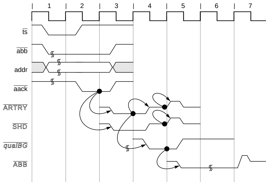
Figure 9-8. Snooped Address Cycle with \overline{\text{ARTRY}}
