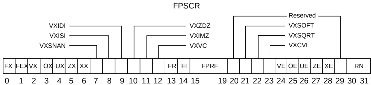
Figure 5-5. Floating-Point Status and Control Register (FPSCR)
