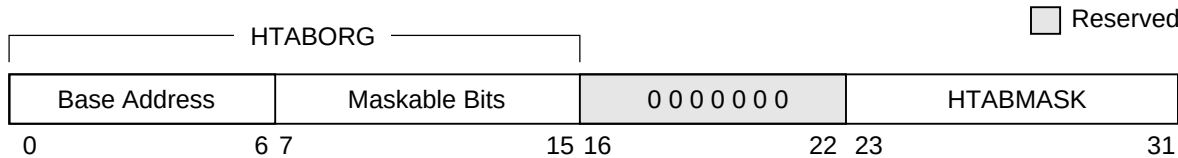
Figure 6-17. SDR1 Register Format
