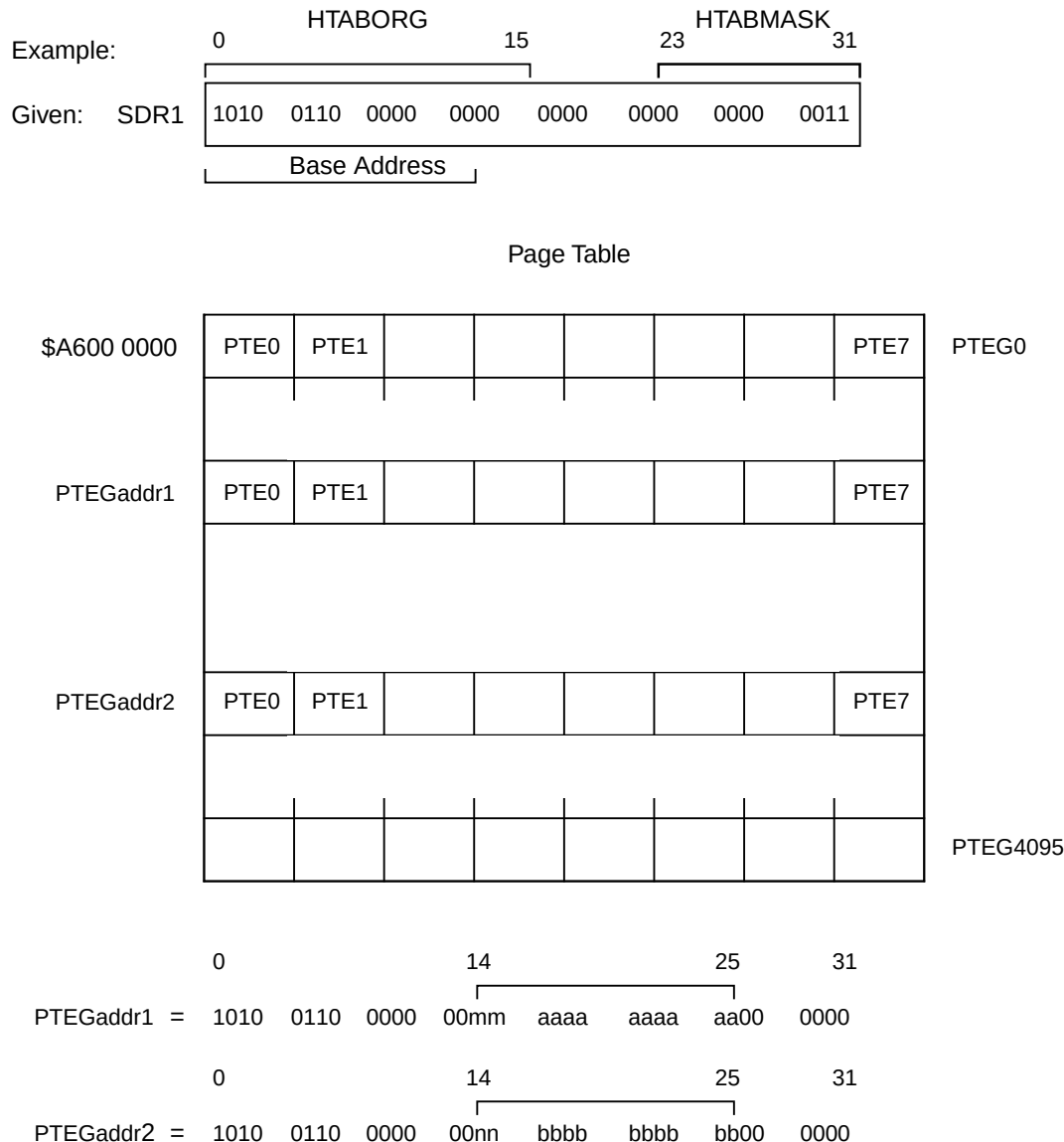
Figure 6-20. Example Page Table Structure
