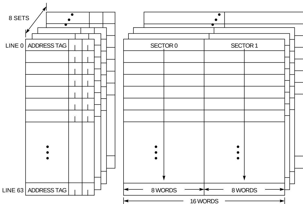
Figure 1-4. Cache Unit Organization
