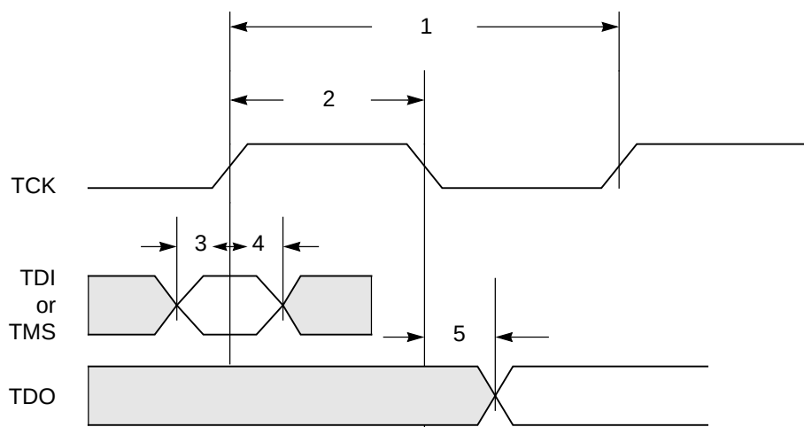
Figure 9-30. IEEE 1149.1 Signal Clocking Requirements
