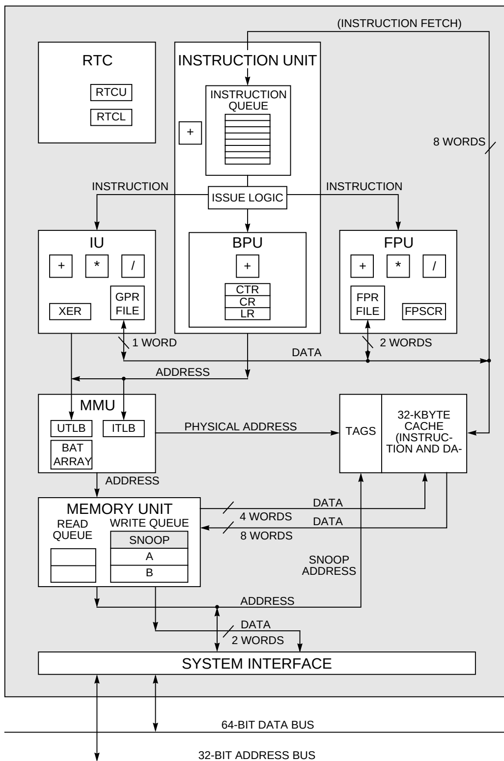
Figure 9-1. PowerPC 601 Microprocessor Block Diagram
