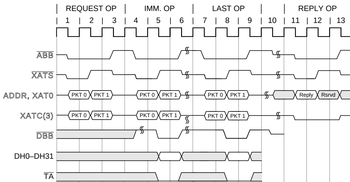
Figure 9-27. I/O Controller Interface Load Access Example
