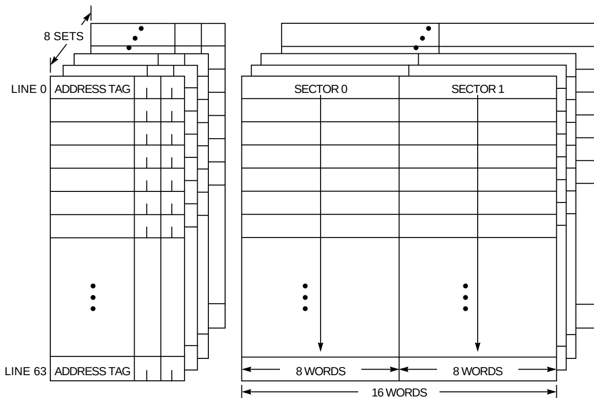
Figure 4-1. Cache Organization
