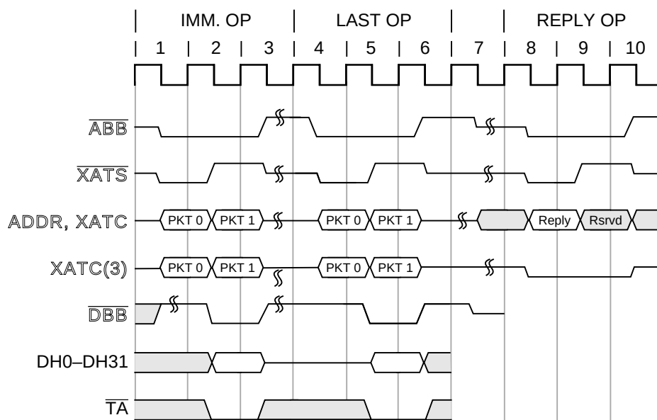
Figure 9-28. I/O Controller Interface Store Access Example
