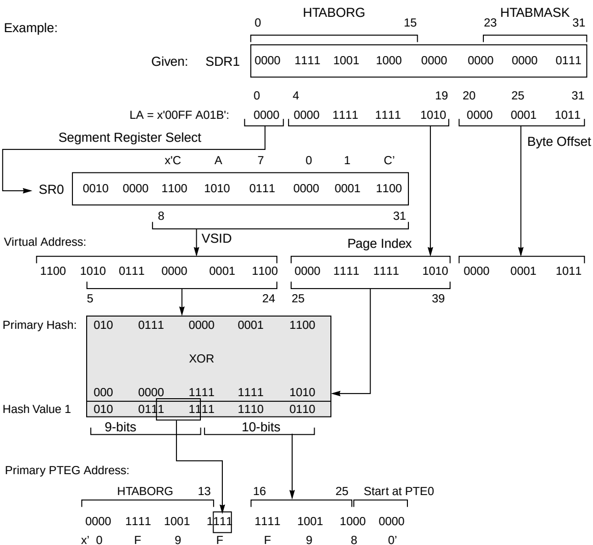
Figure 6-21. Example Primary PTEG Address Generation
