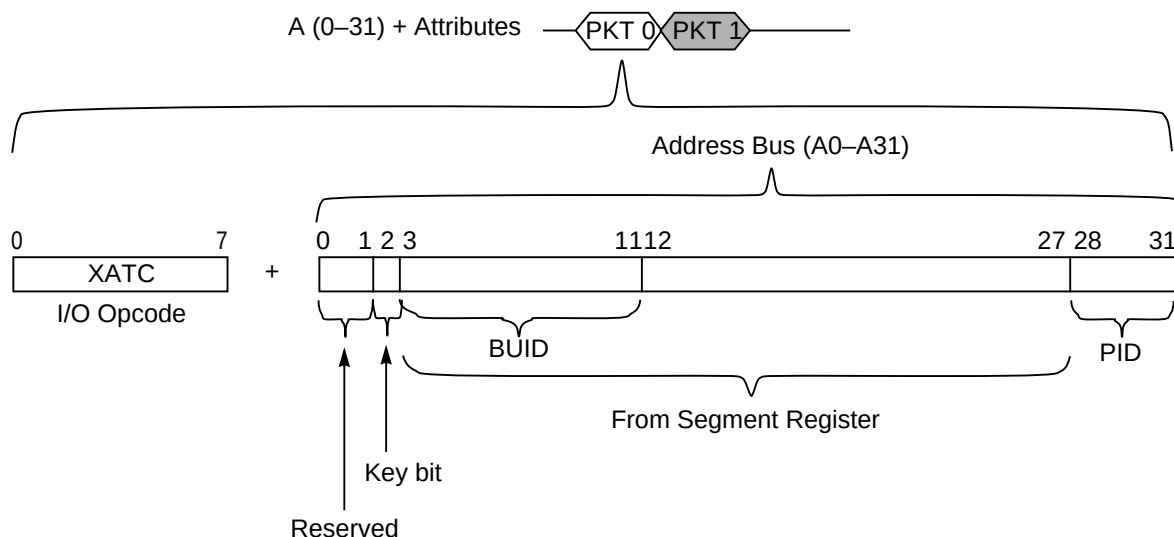
Figure 9-24. I/O Controller Interface Operation—Packet 0
