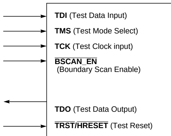
Figure 8-2. IEEE 1149.1-Compatible Boundary Scan Interface
