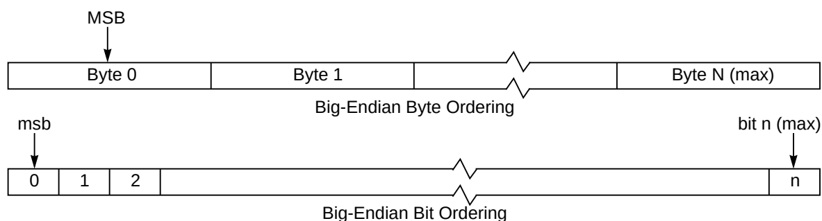
Figure 2-31. Big-Endian Byte and Bit Ordering
