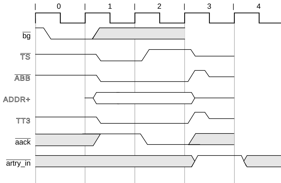
Figure 9-7. Address-Only Bus Transaction
