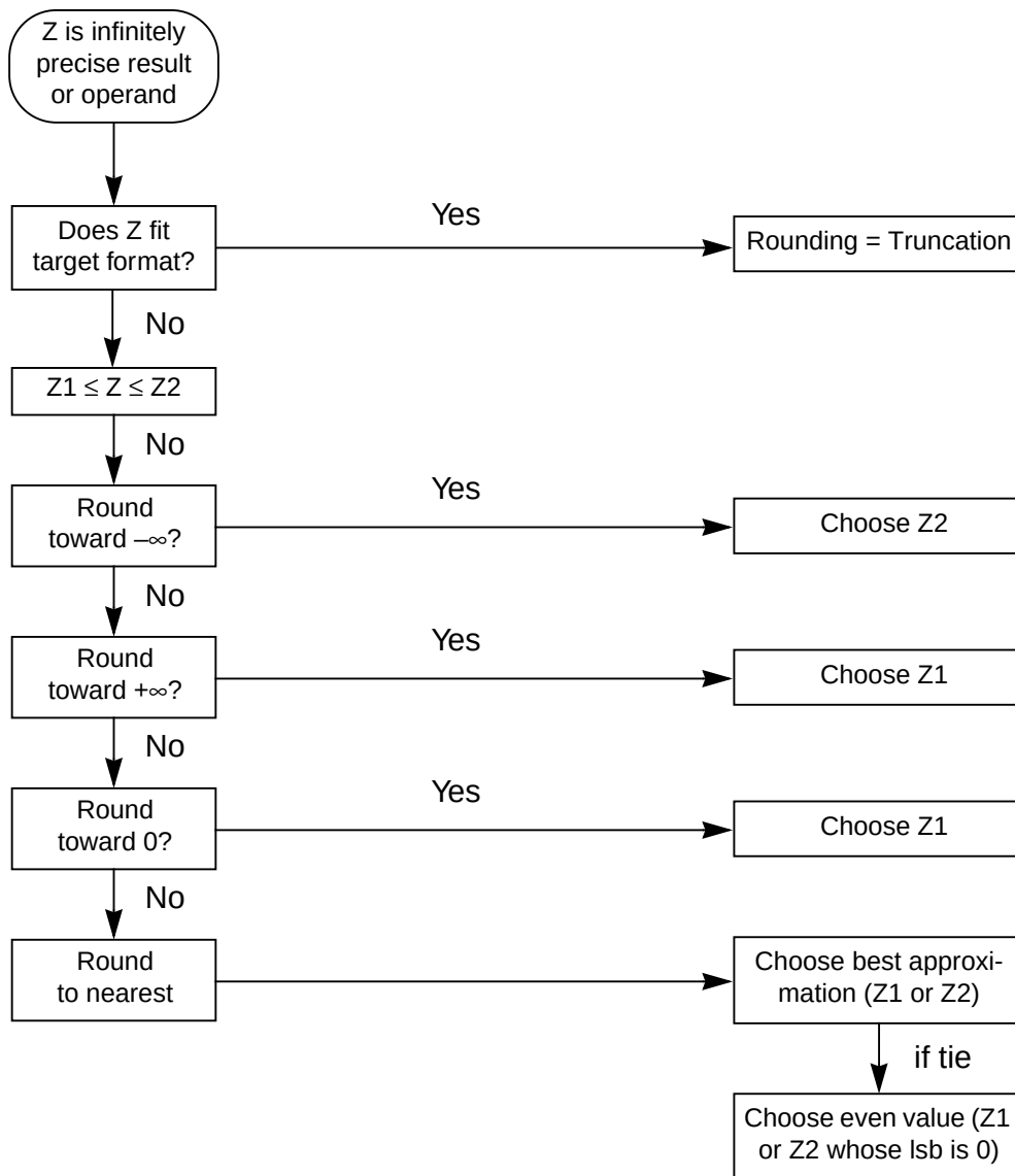
Figure 2-53. Selection of Z1 and Z2
