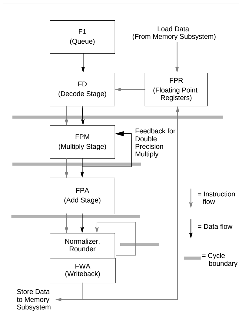
Figure 7-14. Floating-Point Data and Instruction Flow
