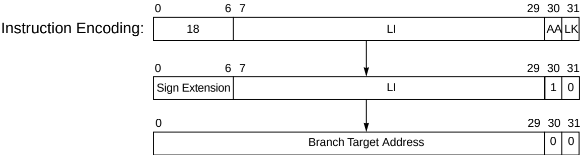
Figure 3-8. Branch to Absolute Addressing
