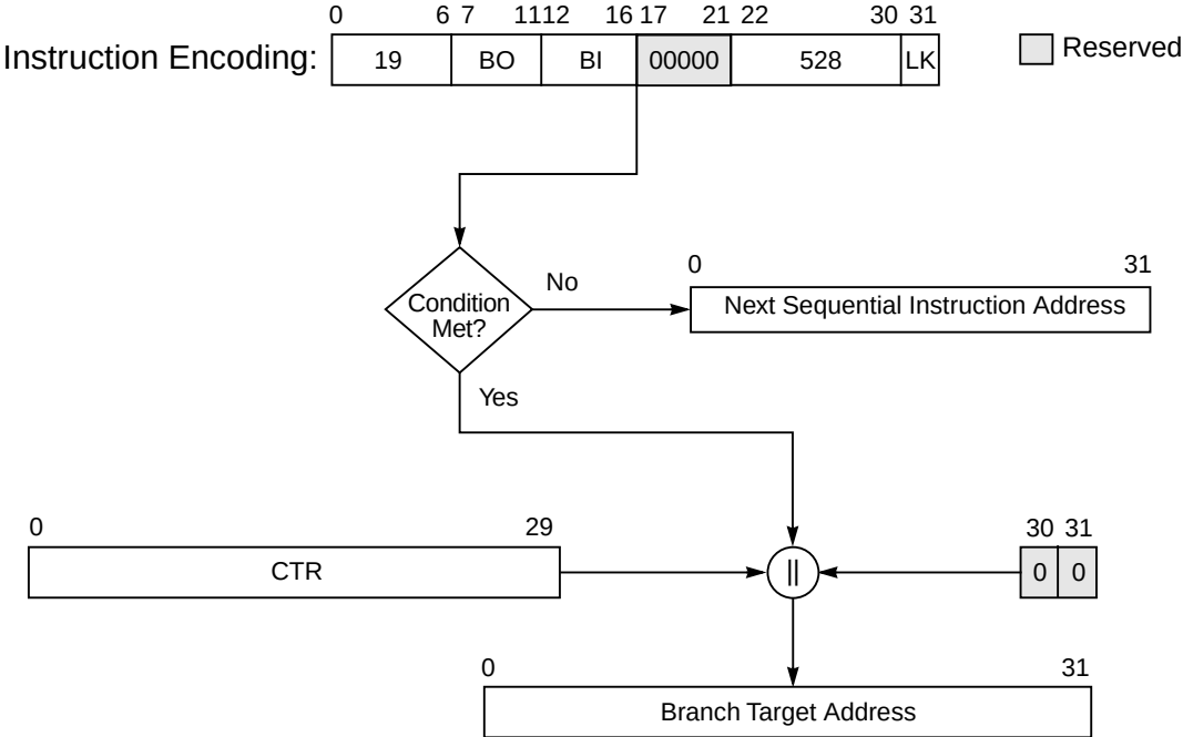
Figure 3-11. Branch Conditional to Count Register Addressing
