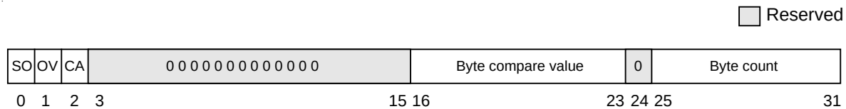
Figure 2-7. Integer Exception Register (XER)
