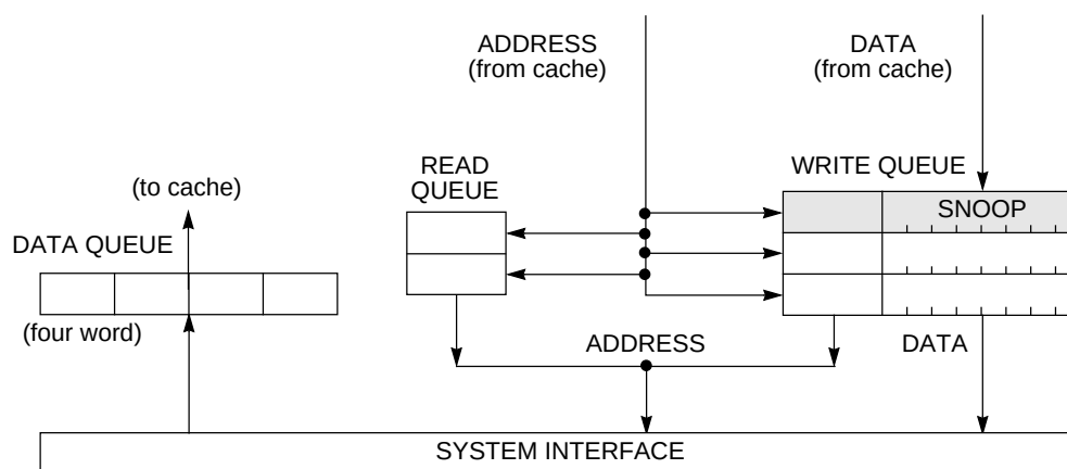
Figure 7-2. Bus Interface Unit
