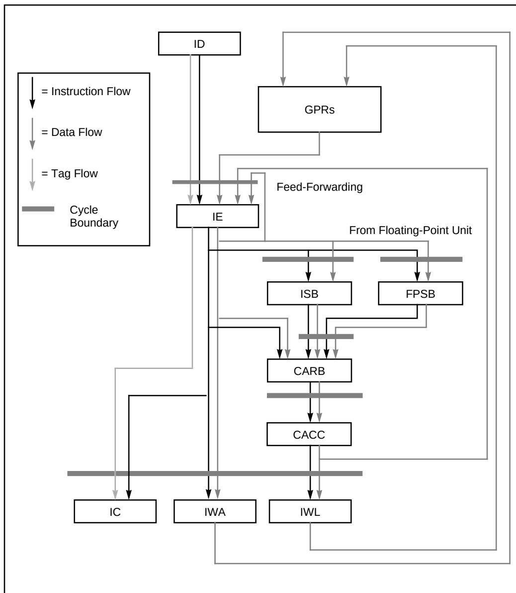
Figure 7-13. IU Pipeline Showing Data, Instruction, and Tag Flow
