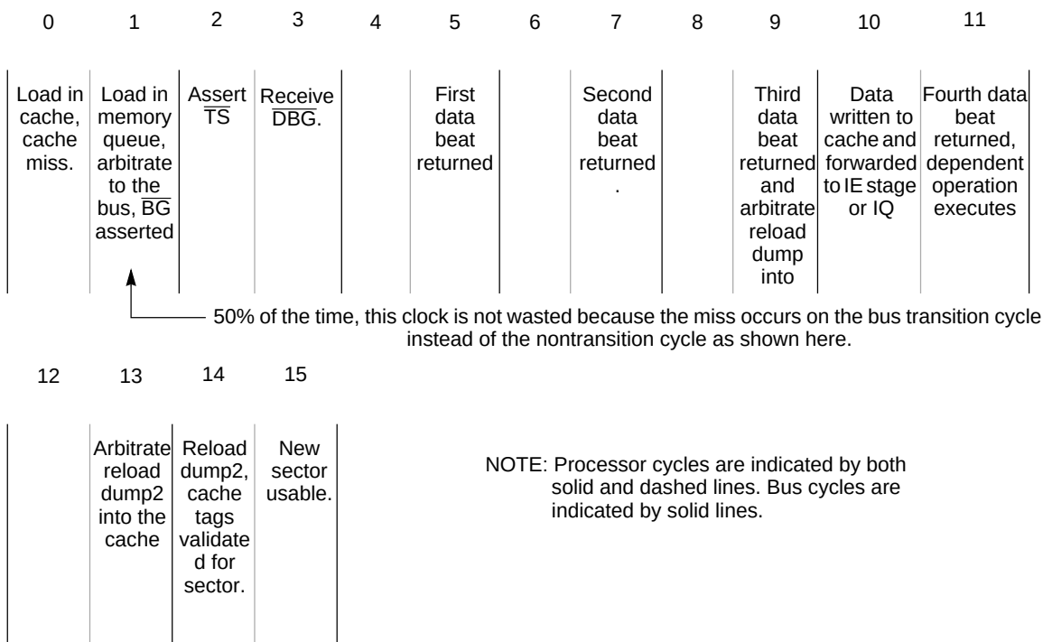
Figure 7-8. Cache Miss Timing when the Processor Clock Frequency is Twice the Bus Clock Frequency (Best-Case)
