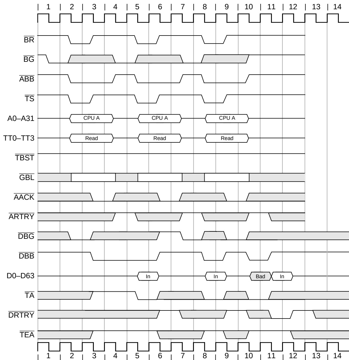
Figure 9-18. Single-Beat Reads Showing Data-Delay Controls
