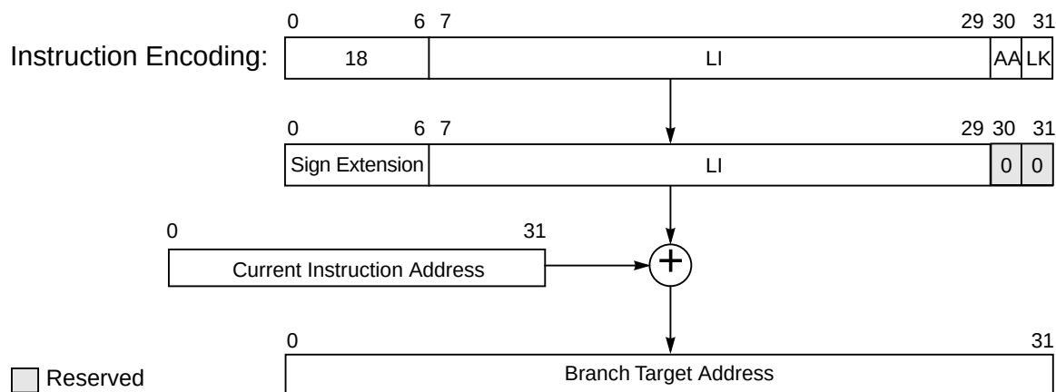
Figure 3-6. Branch Relative Addressing
