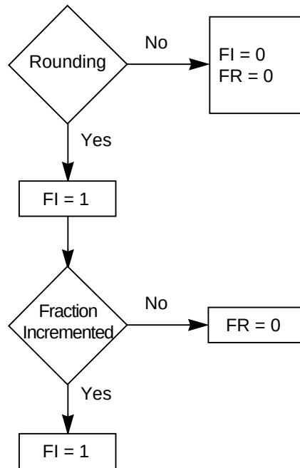
Figure 2-51. Rounding Flow Diagram
