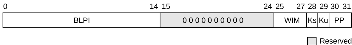
Figure 2-23. Upper BAT Register
