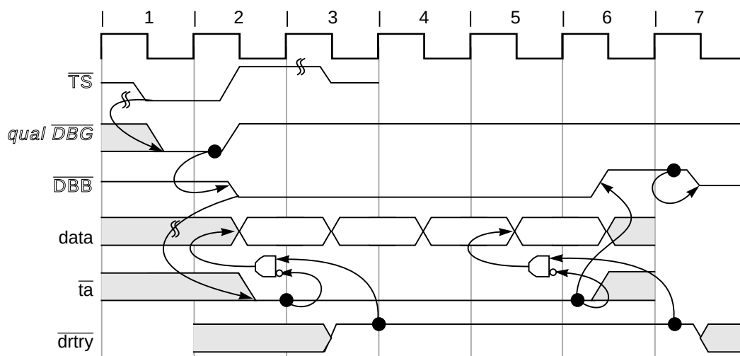
Figure 9-12. Normal Burst Transaction
