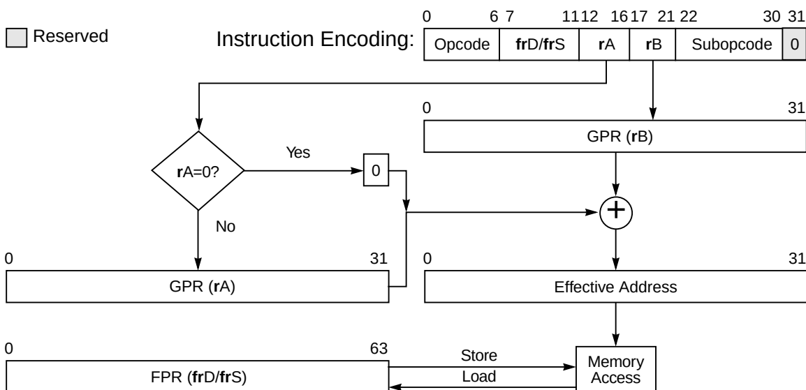
Figure 3-5. Register Indirect with Index Addressing
