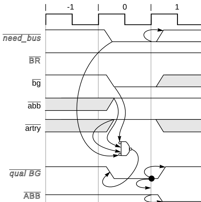
Figure 9-5. Address Bus Arbitration Showing Bus Parking
