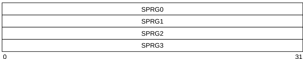
Figure 2-20. General SPRs (SPRG0–SPRG3)
