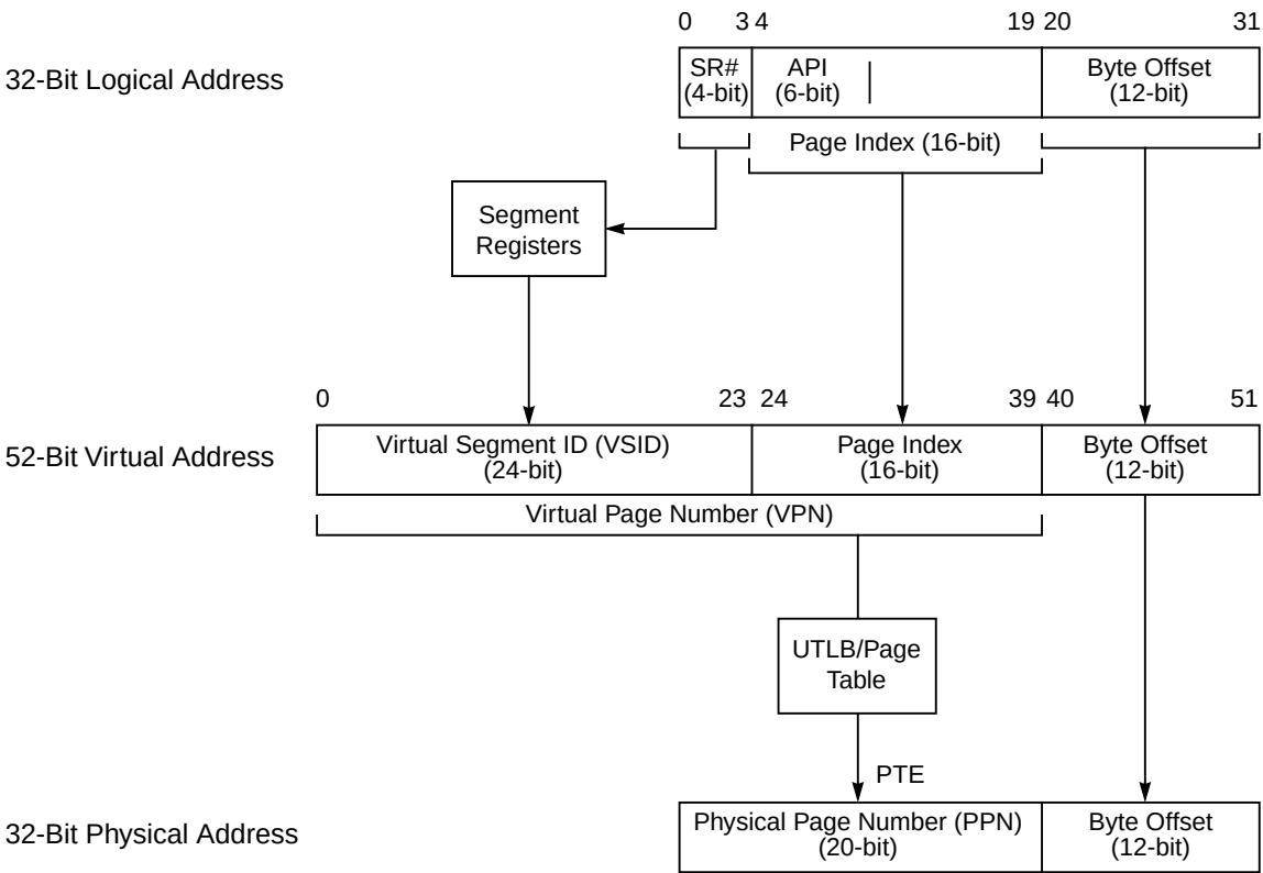
Figure 6-12. Page Address Translation Overview
