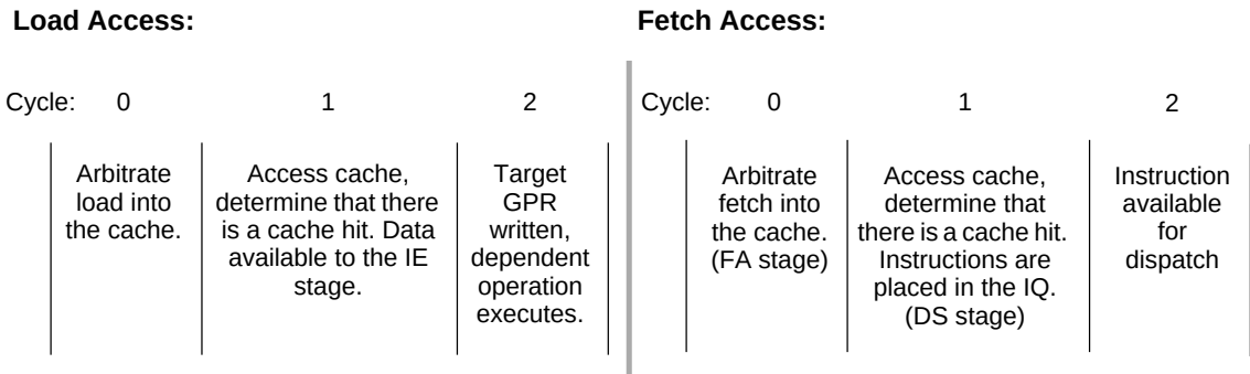
Figure 7-4. Cache Hit Timing for a Load Access and a Fetch Access
