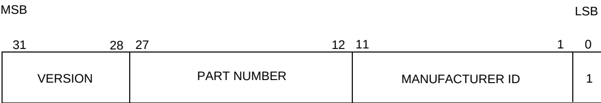
Figure 9-6 IDREGISTER Configuration
