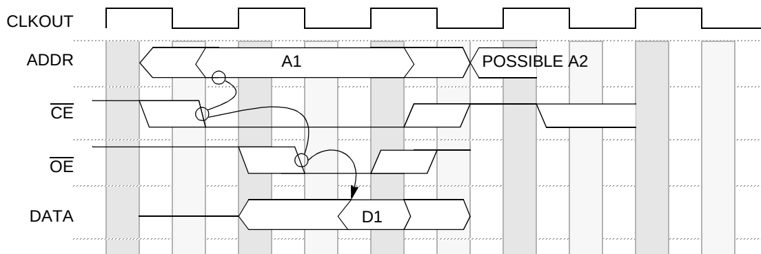
Figure 5-17 Asynchronous Read (Zero Wait States)
