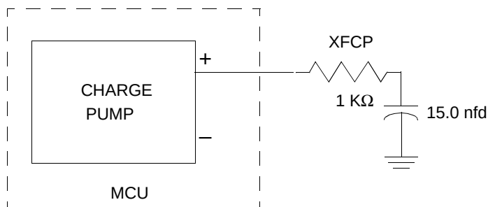
Figure 5-29 Charge Pump with Loop Filter Schematic
