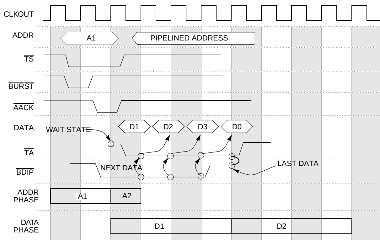
Figure 5-9 External Burst Read Cycle
