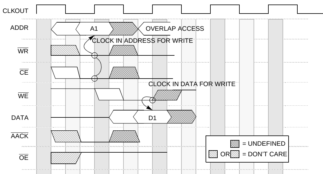
Figure 5-20 Synchronous Write (Zero Wait States)
