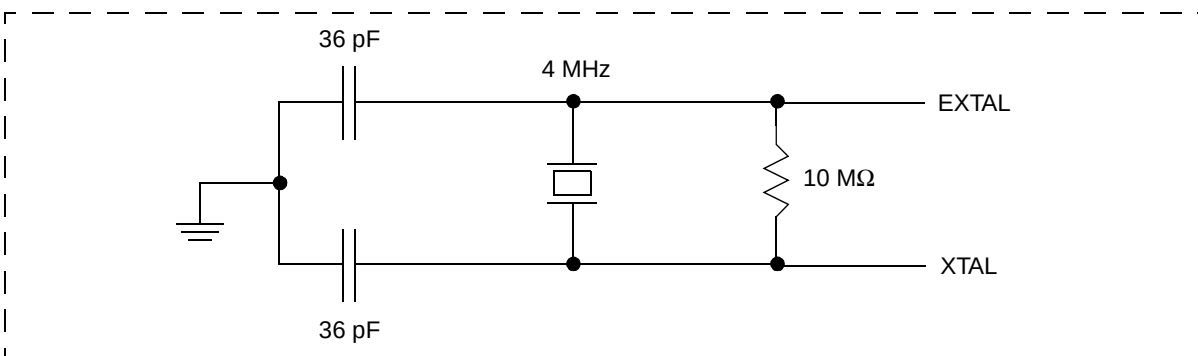
Figure 5-28 Crystal Oscillator
