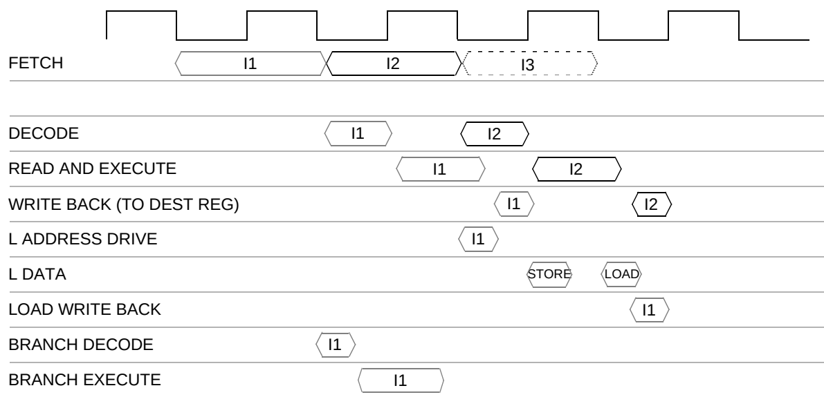
Figure 3-4 Basic Instruction Pipeline
