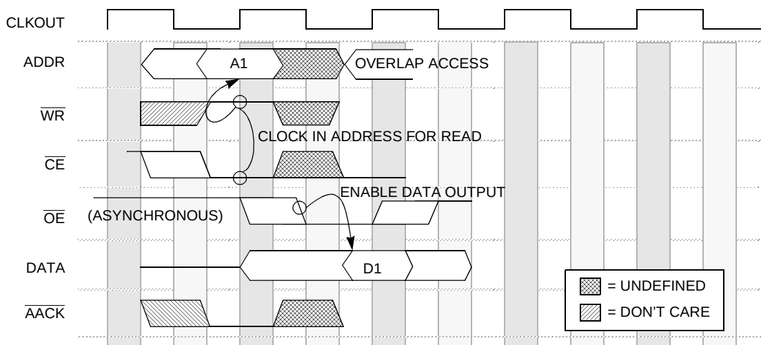
Figure 5-19 Synchronous Read with Asynchronous \overline{\text{OE}} (Zero Wait States)
