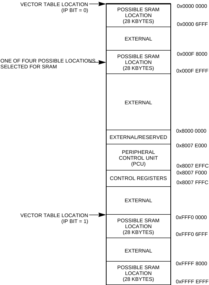
Figure 7-1 Placement of Internal SRAM in Memory Map
