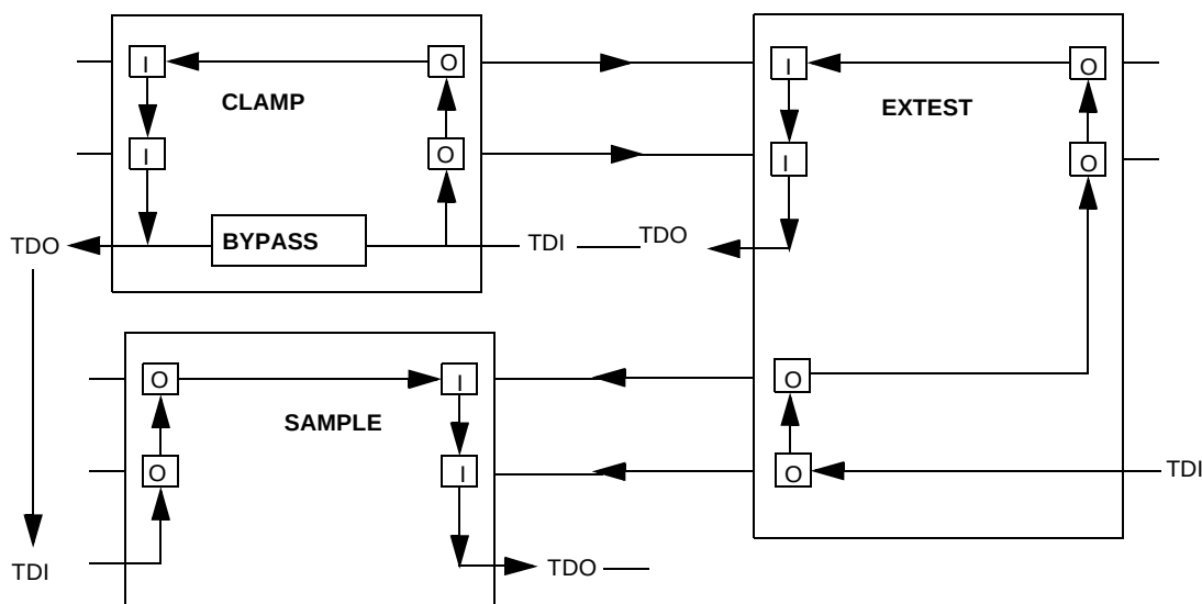
Figure 9-5 Typical Clamp Example
