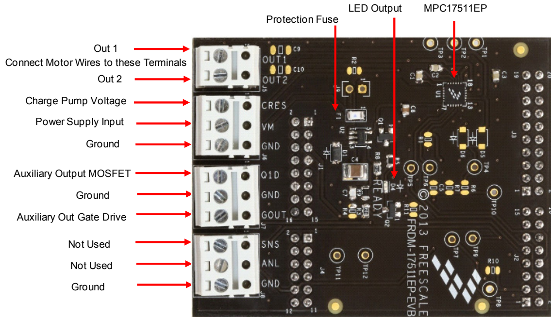
Figure 2. Board Description
