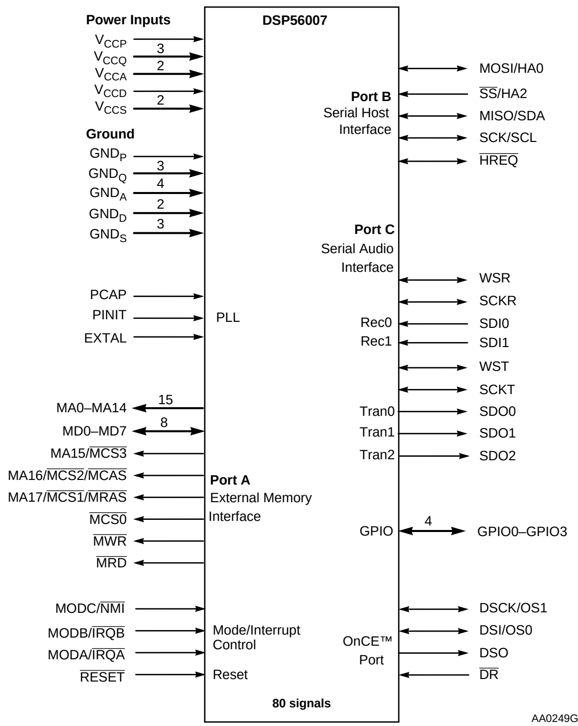
Figure 2-1 DSP56007 Signals
