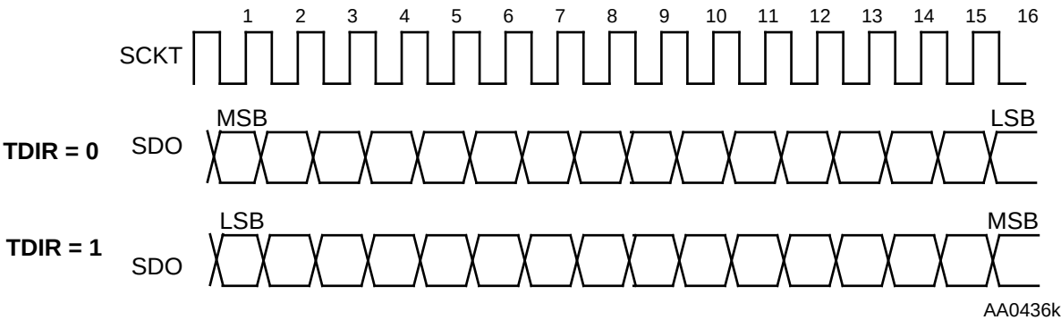
Figure 6-10 Transmitter Data Shift Direction (TDIR) Programming
