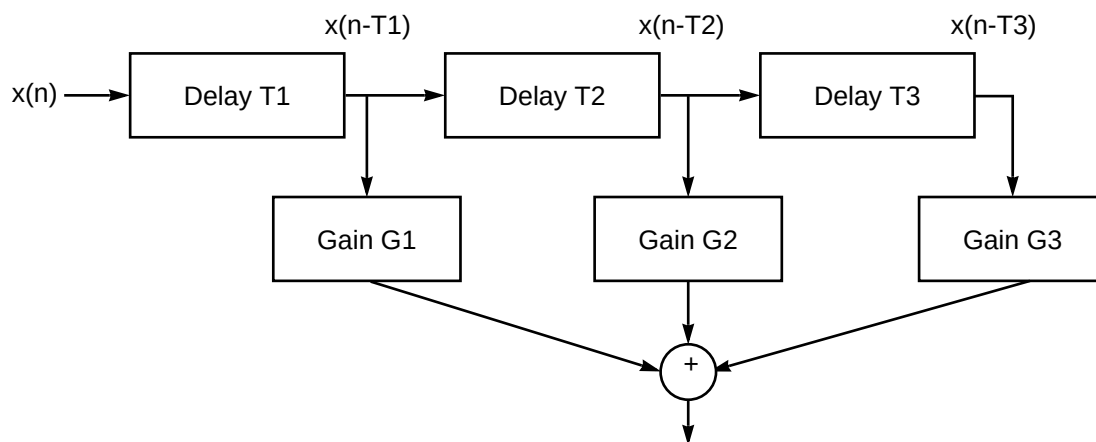
Figure C-4 3 Tap FIR Filter
