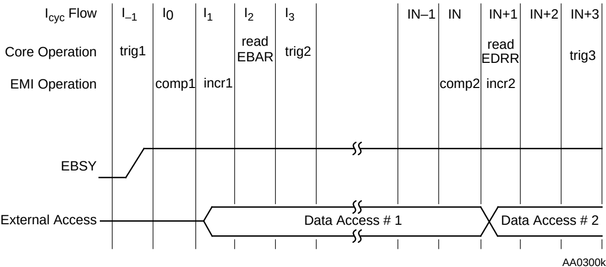
Figure 4-8 EMI Pipeline
