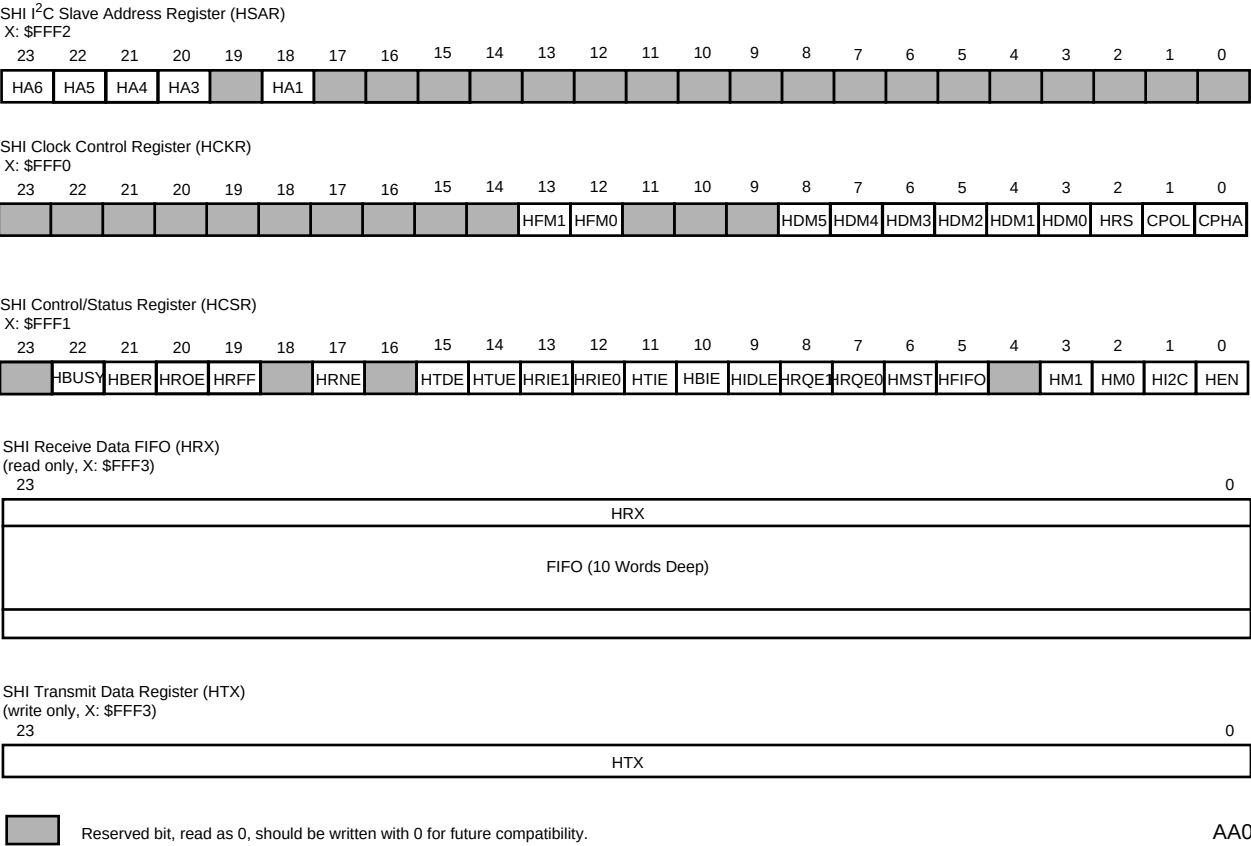
Figure 5-4 SHI Programming Model—DSP Side
