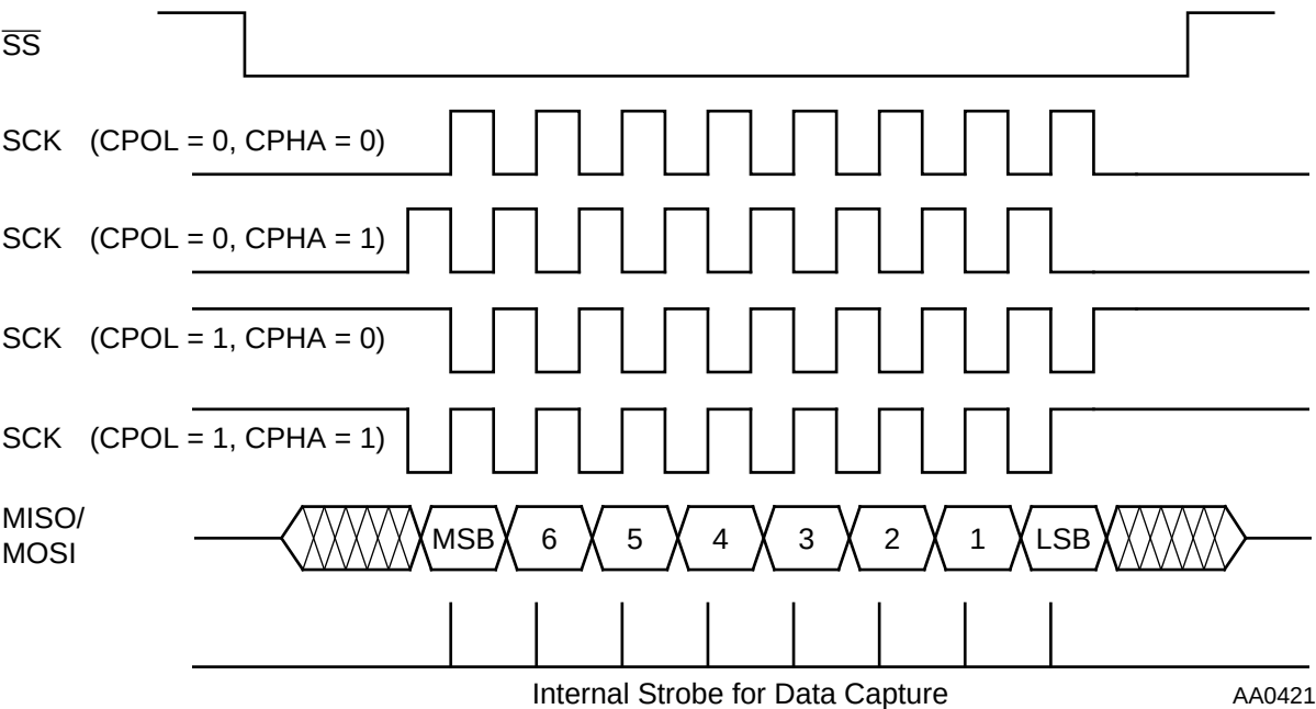
Figure 5-6 SPI Data-To-Clock Timing Diagram
