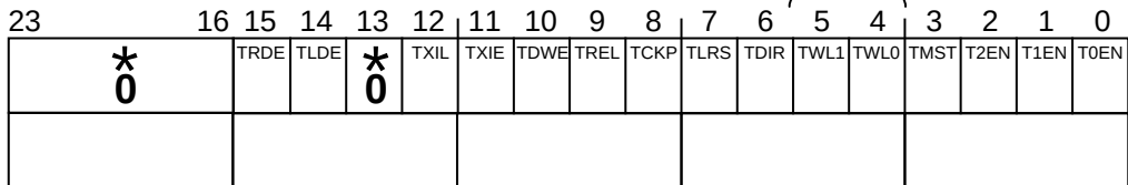
Figure B-14 SAI Transmitter Control/Status Register (TCS)
