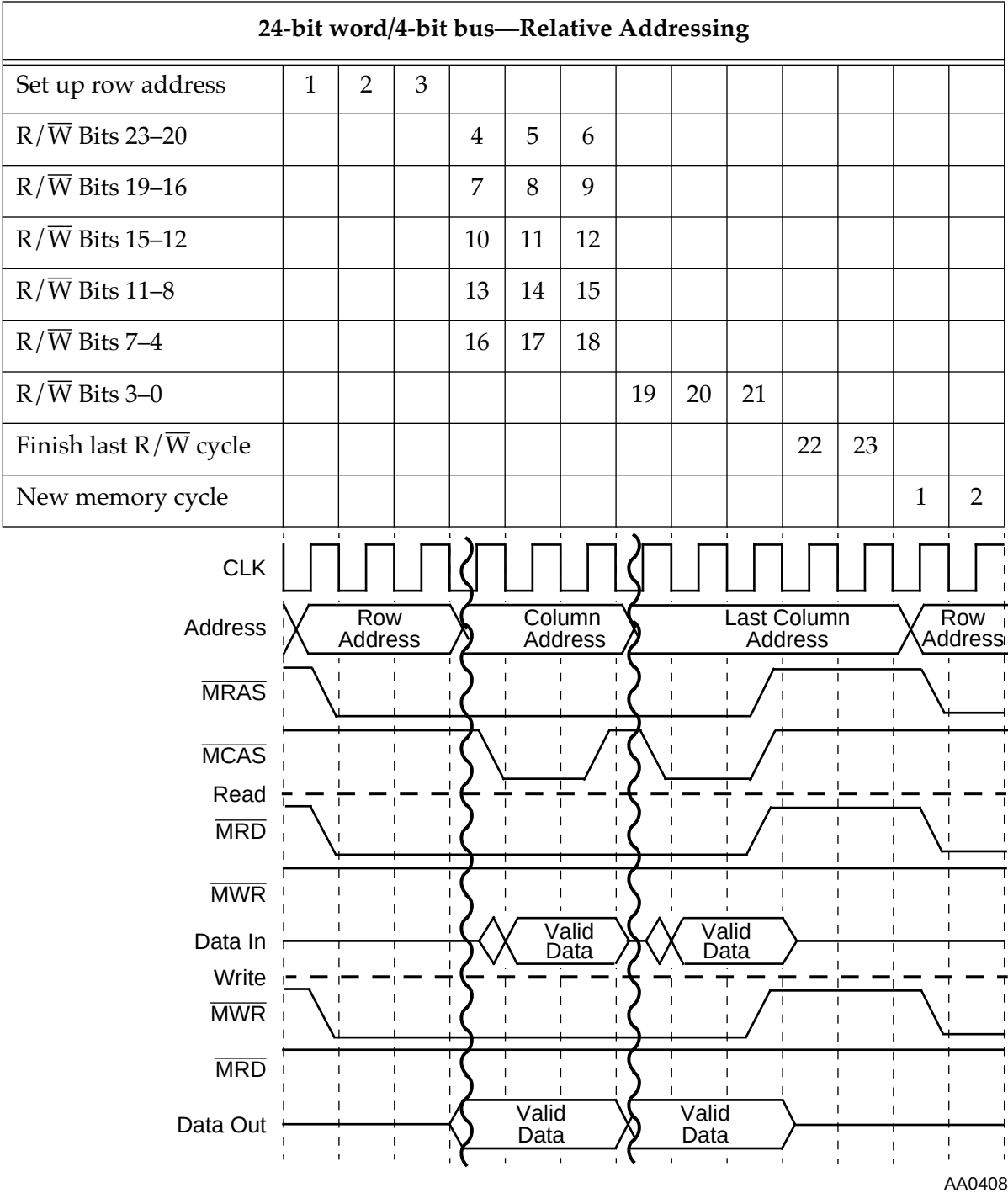
Figure 4-18 Fast Read or Write DRAM Access Timing—6
