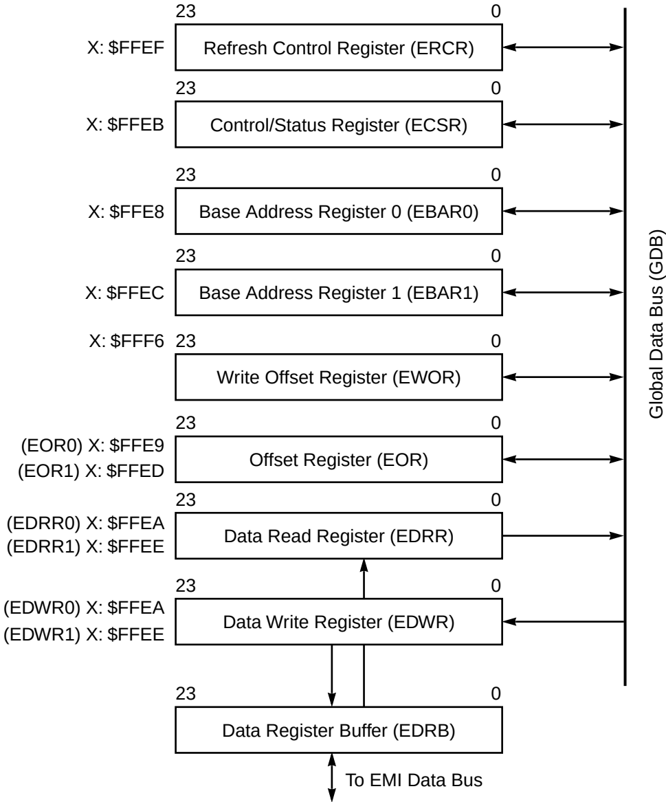
Figure 4-1 EMI Registers
