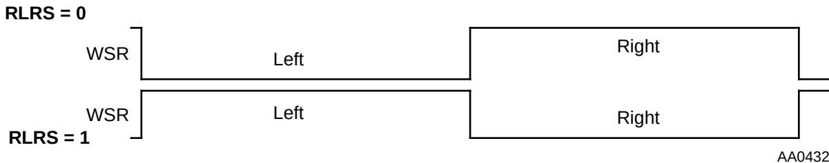
Figure 6-6 Receiver Left/Right Selection (RLRS) Programming
