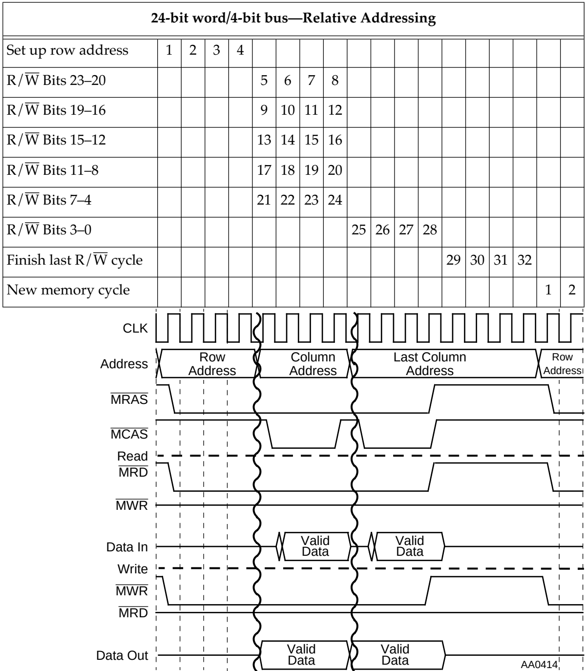
Figure 4-24 Slow Read or Write DRAM Access Timing—6
