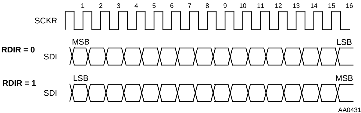
Figure 6-5 Receiver Data Shift Direction (RDIR) Programming
