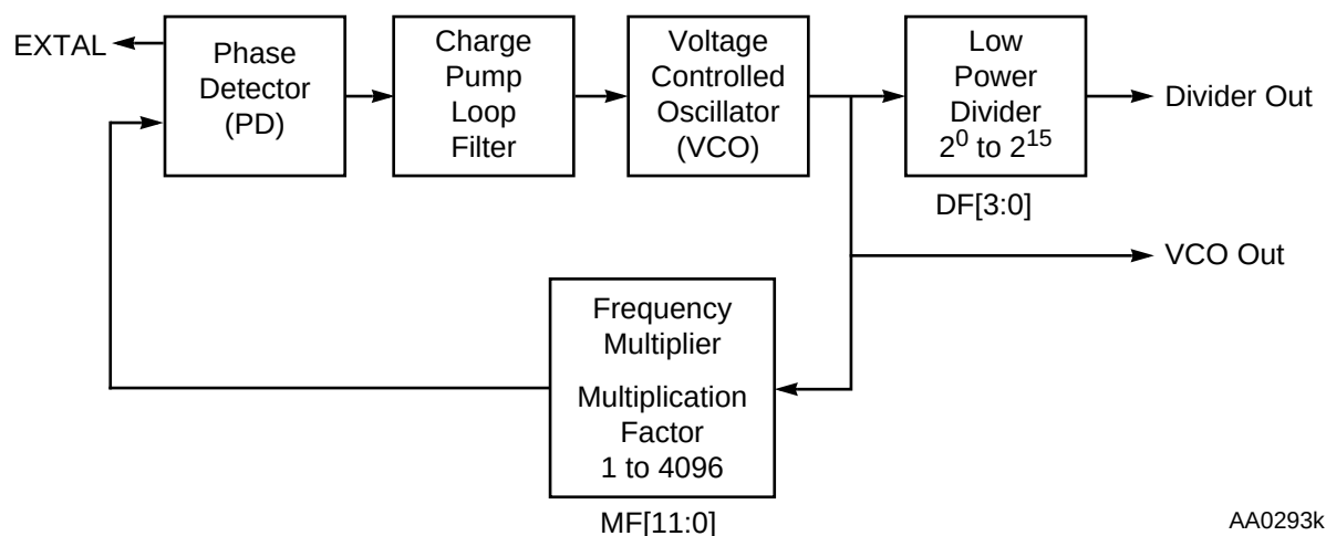
Figure 3-5 PLL Configuration
