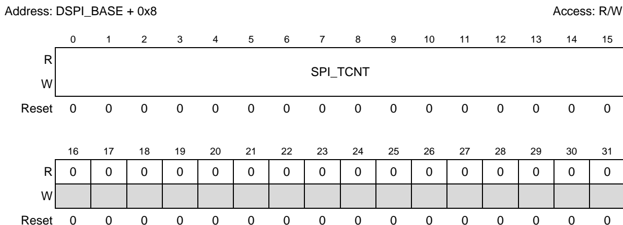
Figure 25-4. DSPI Transfer Count Register (DSPI_TCR)
