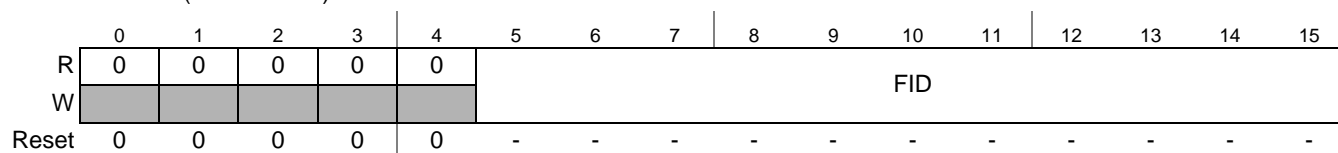
Figure 22-101. Message Buffer Frame ID Registers (MBFIDRn)
