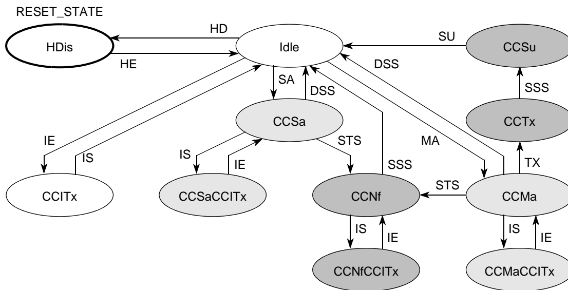
Figure 22-133. Double Transmit Message Buffer State Diagram (Transmit Side)
