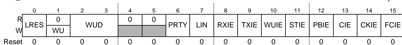
Figure 26-8. LIN Control Register 1 (eSCI_LCR1)
