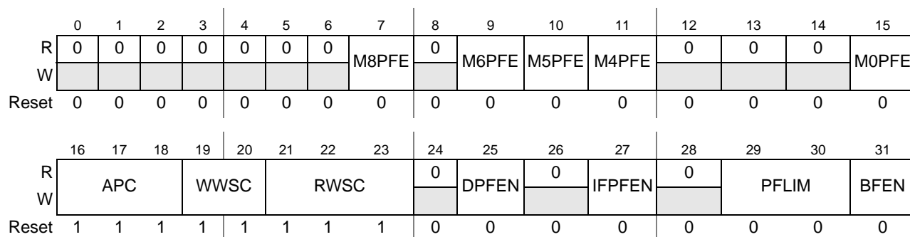
Figure 12-10. Flash Bus Interface Configuration Register (FLASH_BIUCR)
