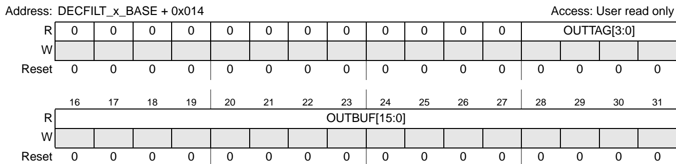
Figure 28-7. Decimation Filter Interface Output Buffer Register (DECFLT_x_OB)
