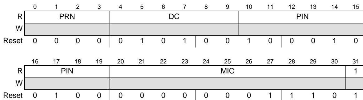
Figure 31-12. NDEDI Device ID Register (DID)
