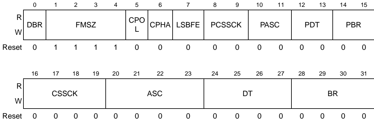
Figure 25-5. DSPI Clock and Transfer Attributes Register 0–7 (DSPI_CTAR0–DSPI_CTAR7)
