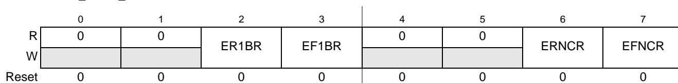
Figure 17-2. ECC Configuration (ECSM_ECR) Register
