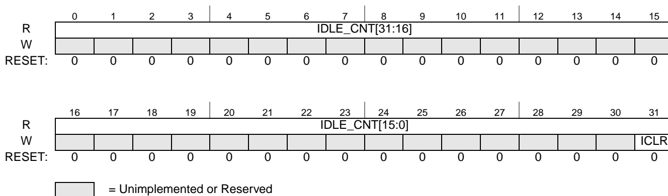
Figure 29-13. ETPUIDLER Register
