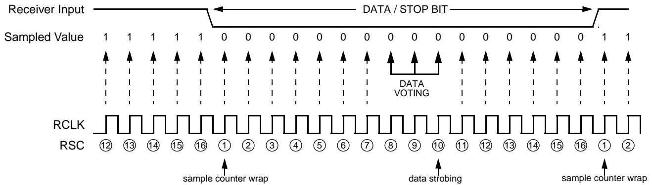
Figure 26-33. Data and Stop Bit Sampling and Strobing
