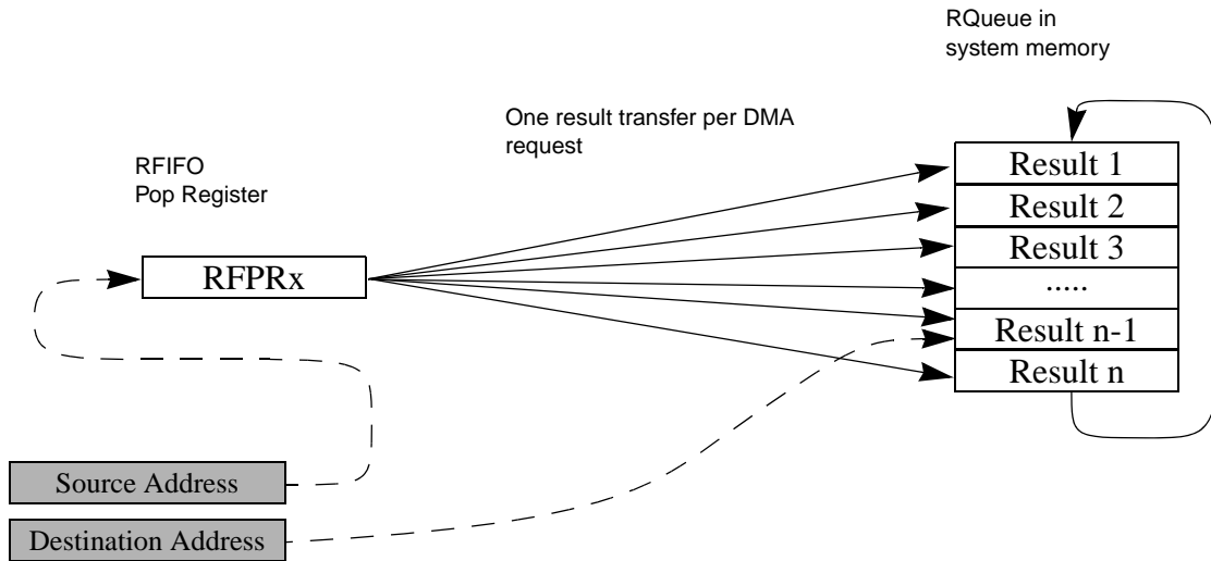
Figure 27-75. RQueue/RFIFO Interface
