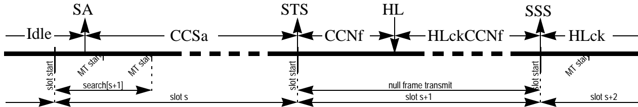
Figure 22-126. Null Frame Transmission from Idle state with locking
