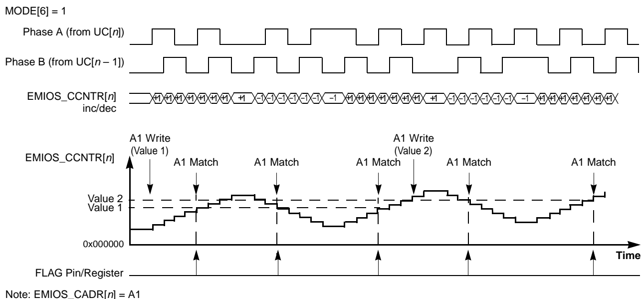
Figure 23-30. QDEC Example with Phase_A & Phase_B Encoder
