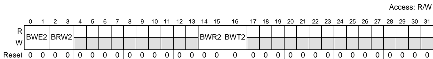
Figure 31-50. Break / Watchpoint Control Register 2 (BWC2)
