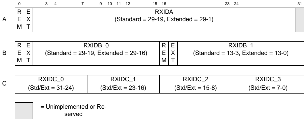
Figure 24-4. ID Table 0 - 7
