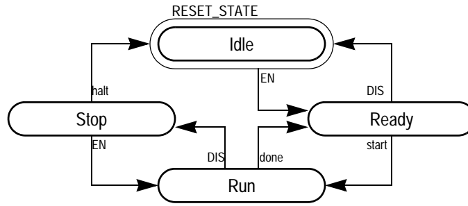
Figure 26-25. Transmitter State Diagram
