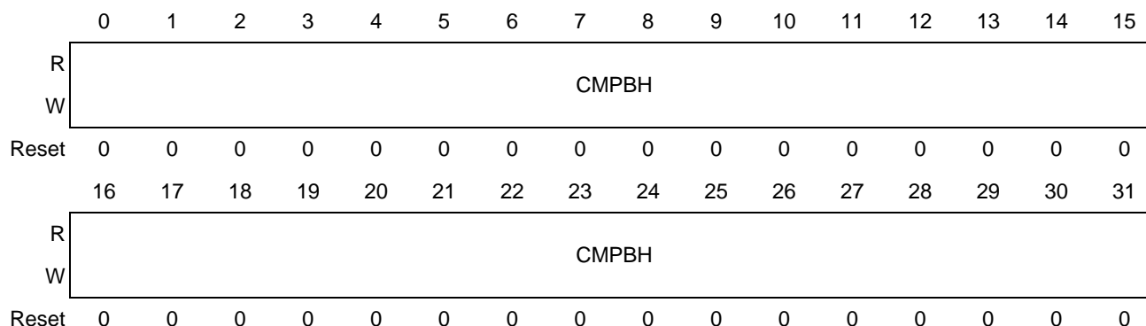
Figure 7-23. Compare B Register High (SIU_CBRH)
