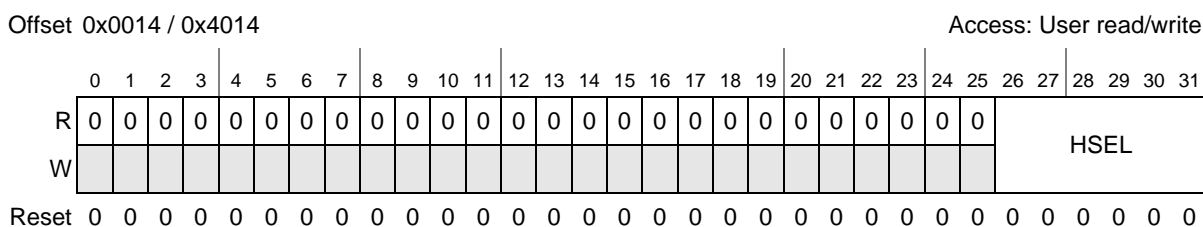
Figure 12-8. FLASH_x_HSR Register
