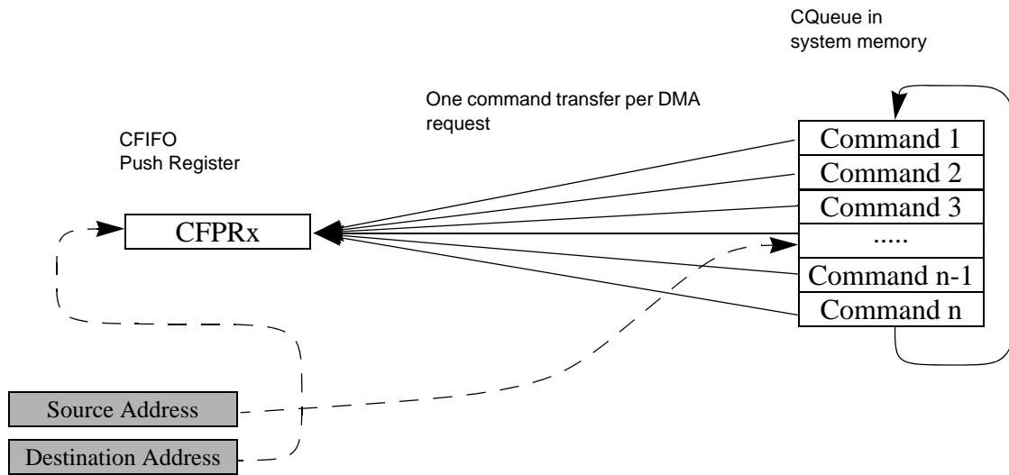
Figure 27-74. CQueue/CFIFO Interface
