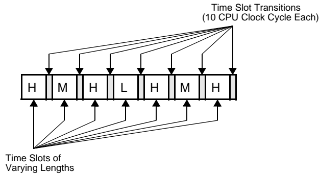
Figure 29-36. Time-Slot Sequence
