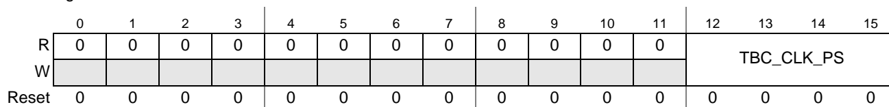
Figure 27-34. ADC Time Stamp Control Register (ADC_TSCR)
