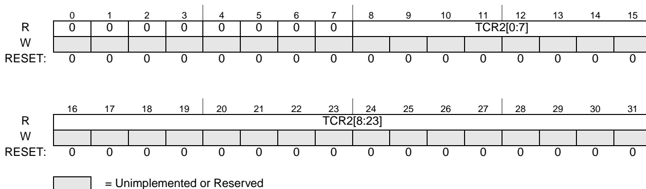
Figure 29-10. ETPUTB2R Register
