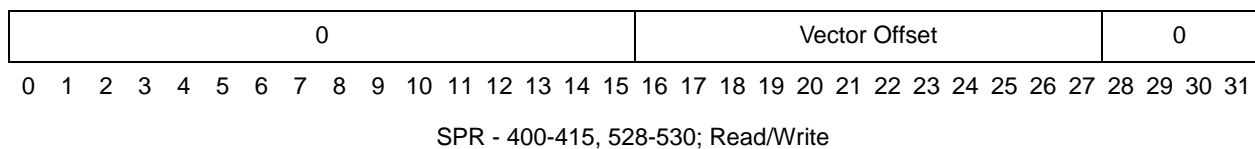
Figure 13-16. PXR40 Interrupt Vector Offset Register (IVOR)
