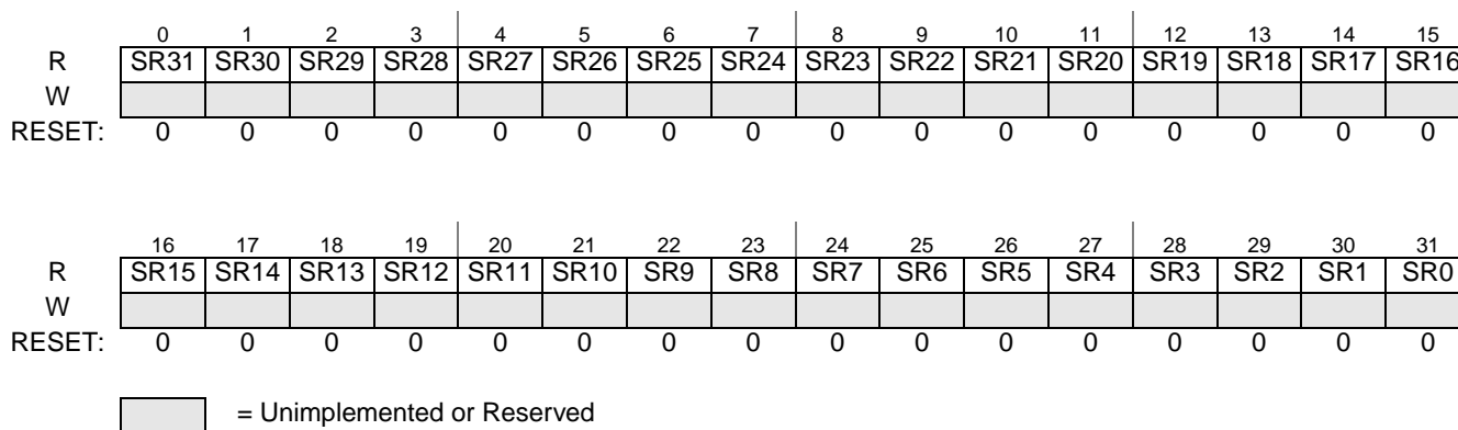
Figure 29-21. ETPUCPSSR Register
