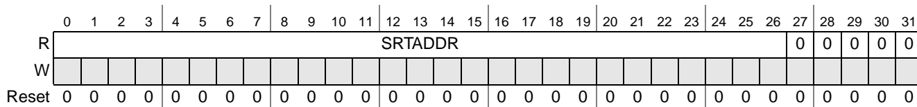
Figure 16-5. MPU Region Descriptor, Word 0 Register (MPU_RGD n .Word0)
