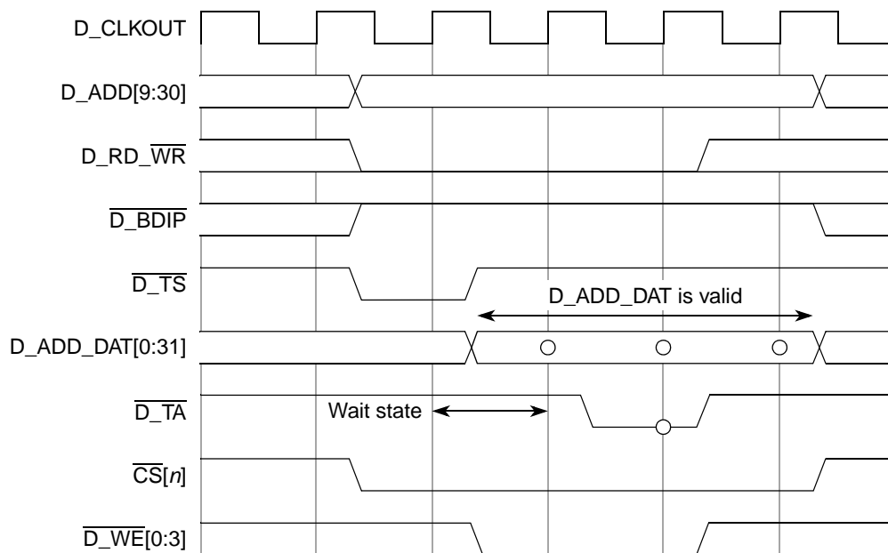
Figure 30-15. Single Beat 32-bit Write Cycle, \overline{CS} Access, One Wait State
