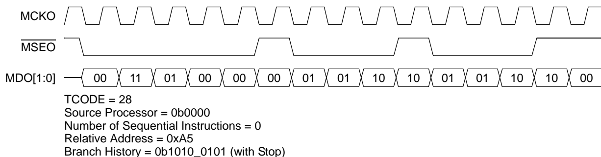
Figure 31-27. Program Trace (MDO = 2)—Indirect Branch Message (History)
