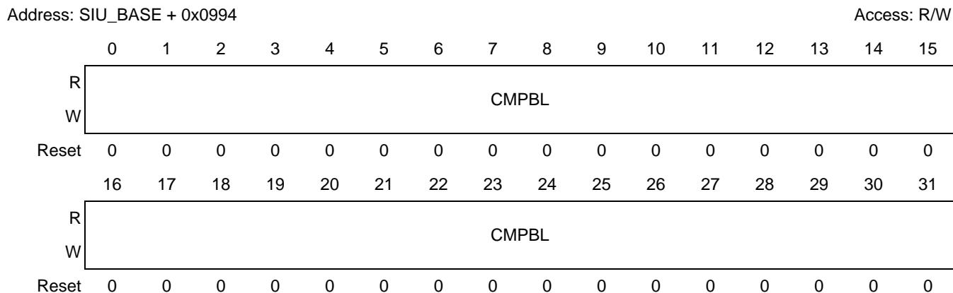
Figure 7-24. Compare B Register Low (SIU_CBRL)
