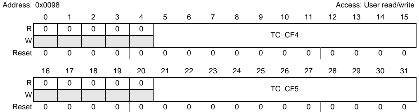
Figure 27-14. EQADC CFIFO Transfer Counter Register 2 (EQADC_CFTCR2)
