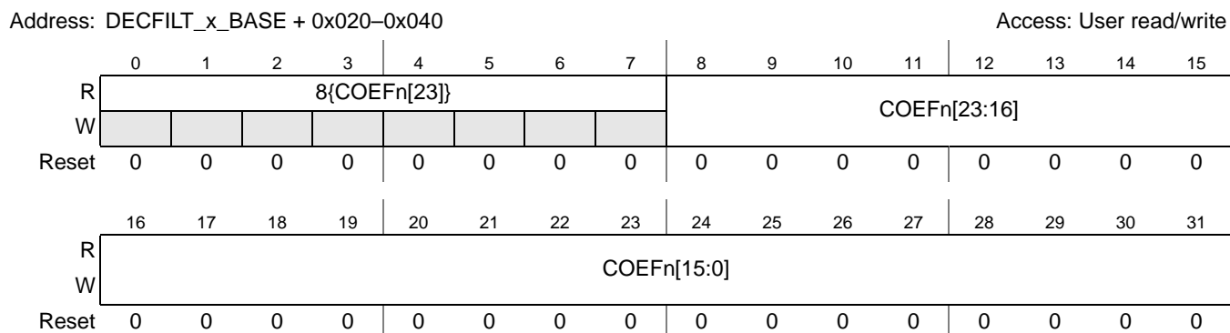
Figure 28-8. Decimation Filter Coefficient n Register (DECFLT_x_COEFn)
