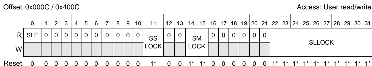
Figure 12-6. FLASH_x_SLMLR Register
