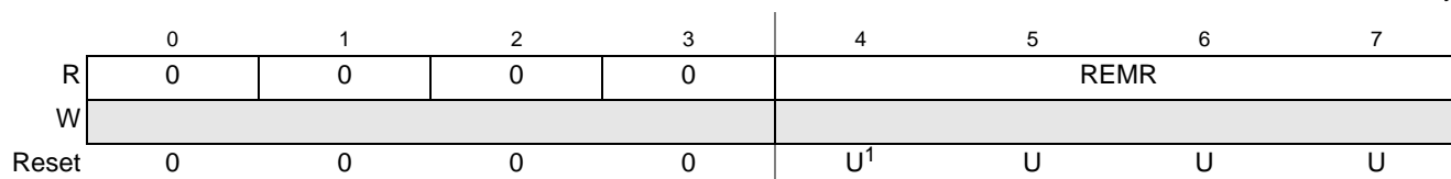
Figure 17-12. RAM ECC Master Number (ECSM_REMR) Register
