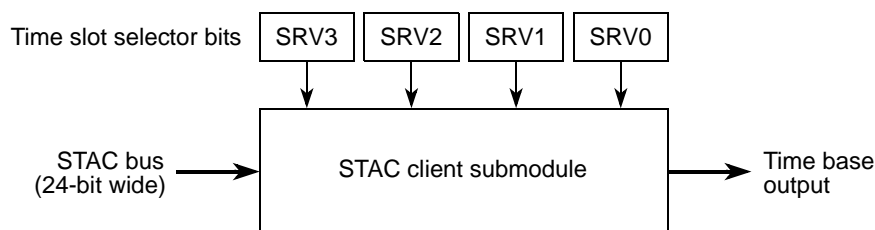
Figure 23-59. STAC Client Submodule Block Diagram
