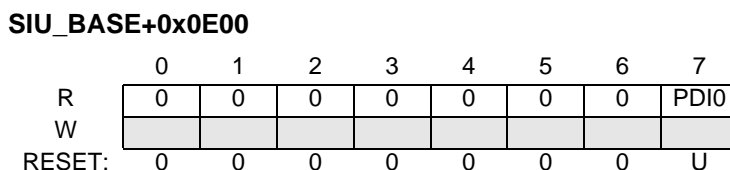
Figure 7-46. GPIO Pin Data In Register 0 (SIU_GPDIO)
