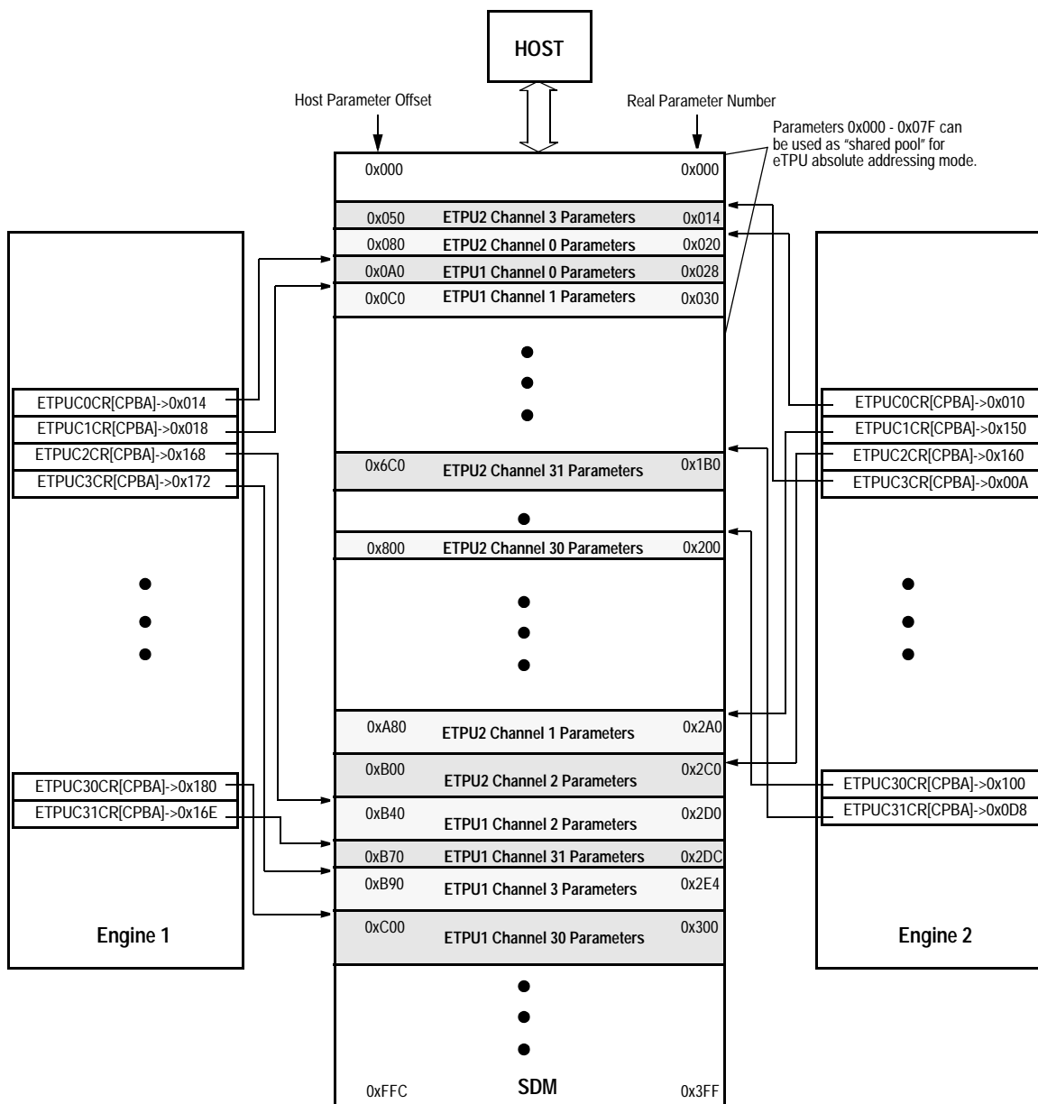
Figure 29-26. SDM Organization Example (4 Kbytes)
