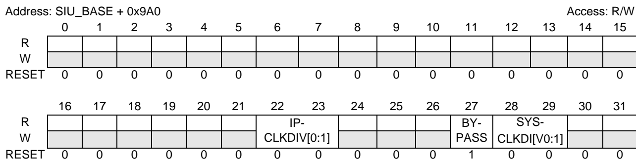
Figure 7-25. System Clock Register (SIU_SYSDIV)
