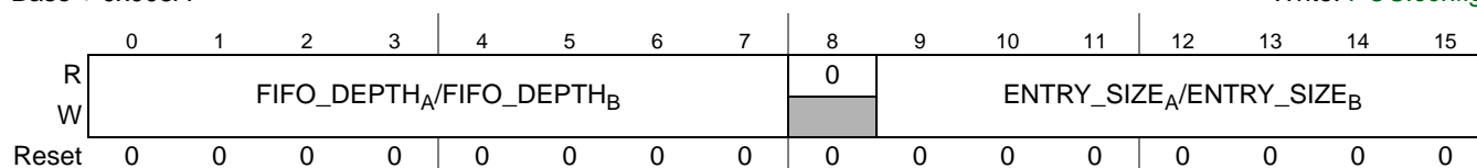
Figure 22-56. Receive FIFO Depth and Size Register (RFDSR)
