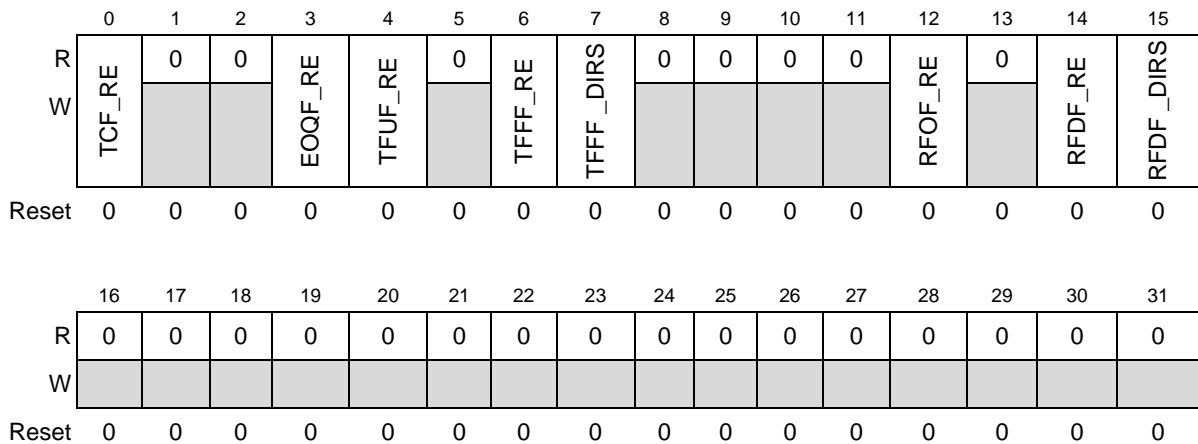
Figure 25-7. DSPI DMA/Interrupt Request Select and Enable Register (DSPI_RSER)
