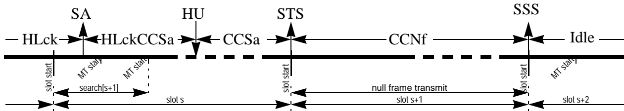
Figure 22-125. Null Frame Transmission from HLck state with unlock
