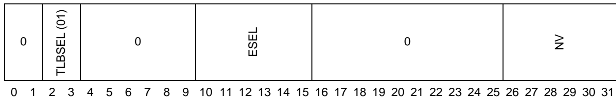
Figure 13-7. MMU Assist Register 0 (MAS0)
