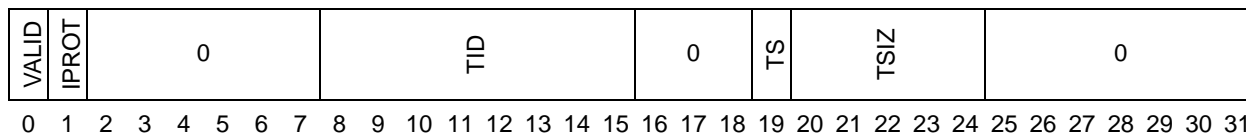
Figure 13-8. MMU Assist Register 1 (MAS1)
