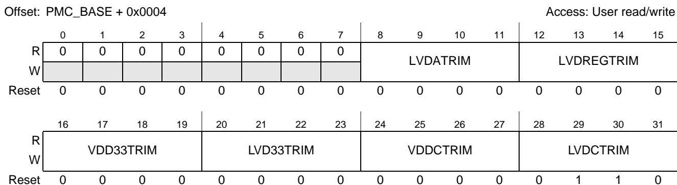
Figure 5-3. Trimming Register (PMC_TRIMR)
