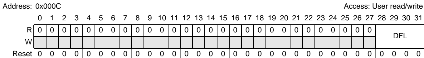
Figure 27-4. EQADC External Trigger Digital Filter Register (EQADC_ETDFR)
