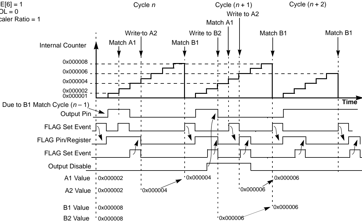
Figure 23-43. OPWFMB Mode with Active Output Disable
