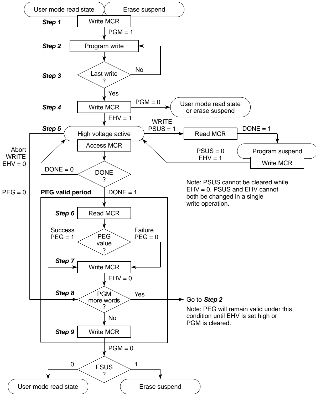
Figure 12-17. Program Sequence
