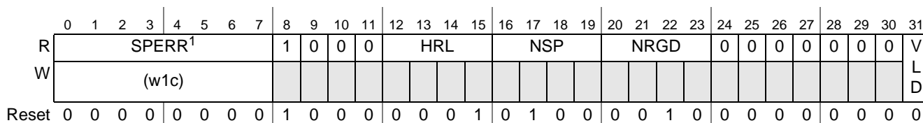
Figure 16-2. MPU Control/Error Status Register (MPU_CESR)
