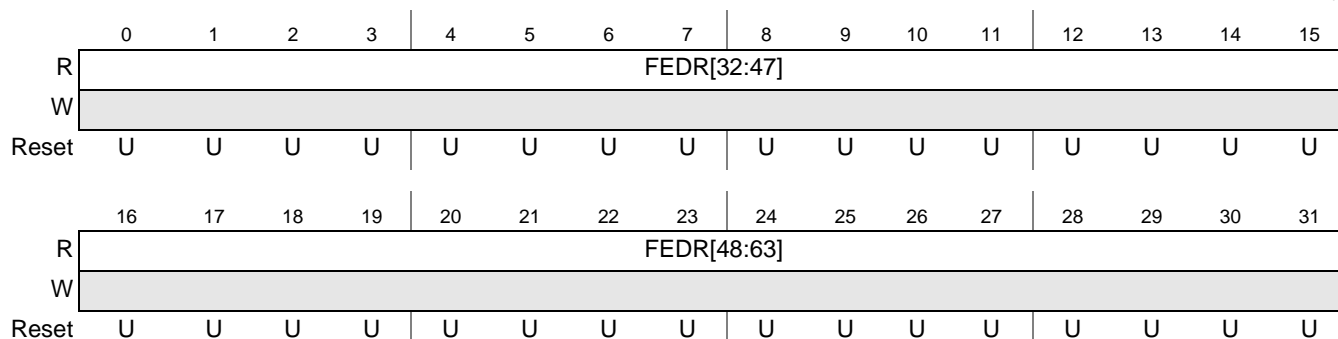
Figure 17-9. Flash ECC Data Low (ECSM_FEDRL) Register
