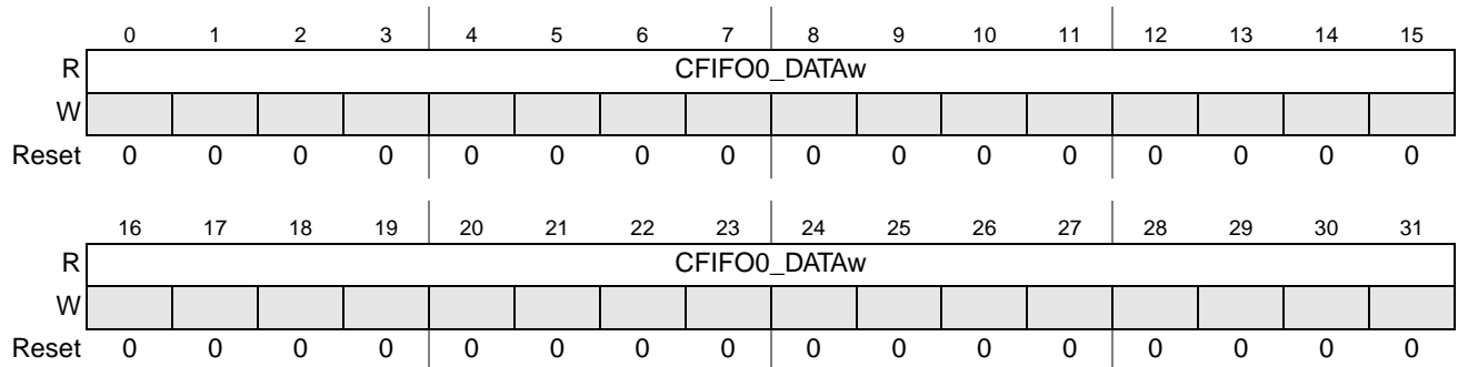
Figure 27-19. EQADC CFIFO0 Registers (EQADC_CF0Rw) (w=0, ..., 3)
