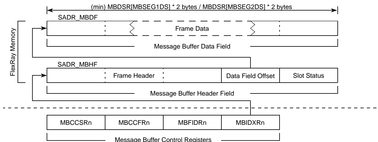
Figure 22-104. Individual Message Buffer Structure
