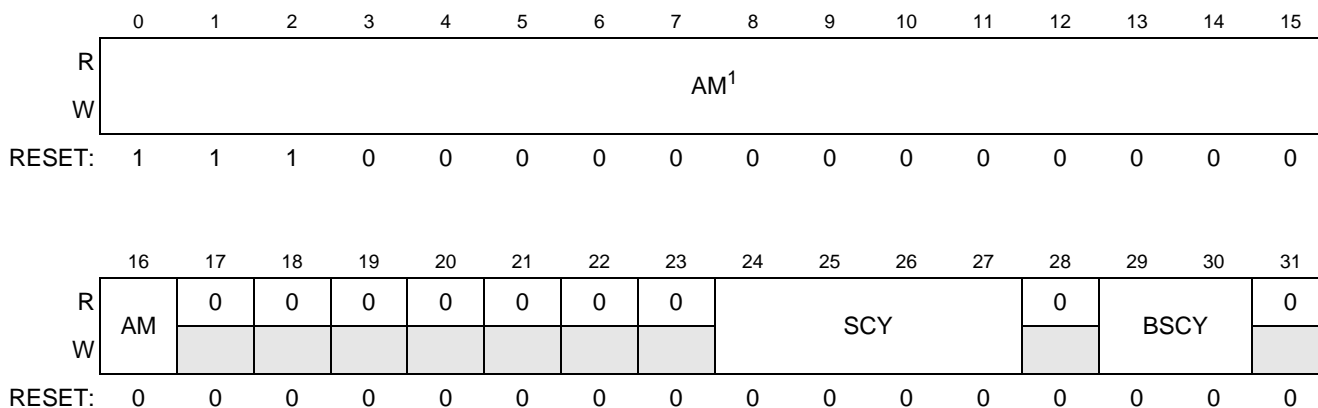
Figure 30-6. EBI Option Registers (EBI_CAL_OR0-3)
