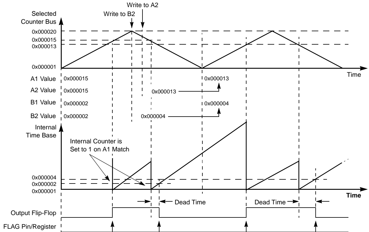
Figure 23-49. OPWMCB with Trailing Dead Time Insertion
