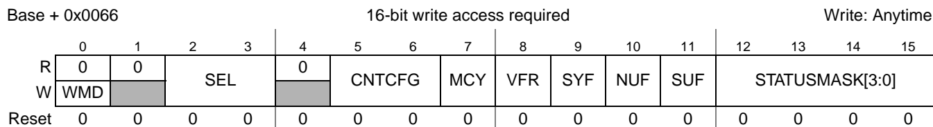
Figure 22-45. Slot Status Counter Condition Register (SSCCR)
