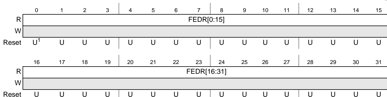
Figure 17-8. Flash ECC Data High (ECSM_FEDRH) Register
