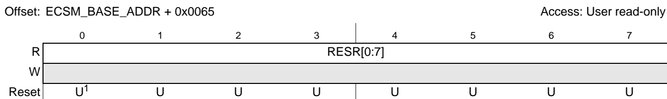
Figure 17-11. RAM ECC Syndrome (ECSM_RESR) Register
