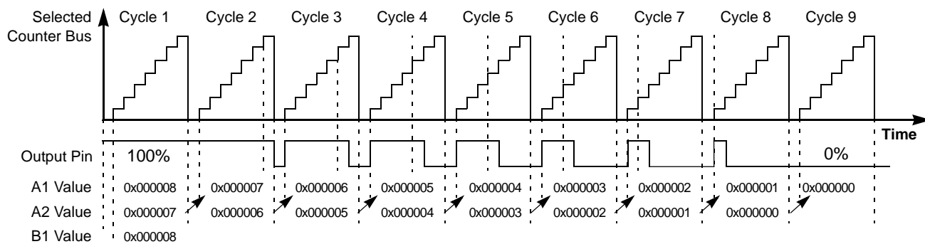
Figure 23-56. OPWMB Mode from 100% to 0% Duty Cycle
