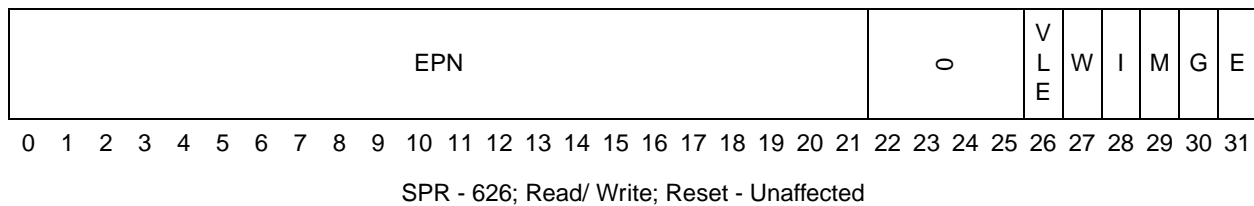
Figure 13-9. MMU Assist Register 2 (MAS2)
