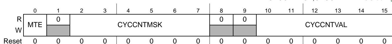
Figure 22-48. MTS A Configuration Register (MTSACFR)
