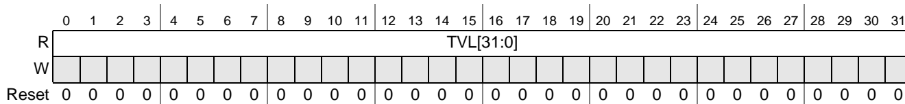
Figure 20-4. Current Timer Value Register (PIT_RTI_CVAL, PIT_CH n _CVAL)
