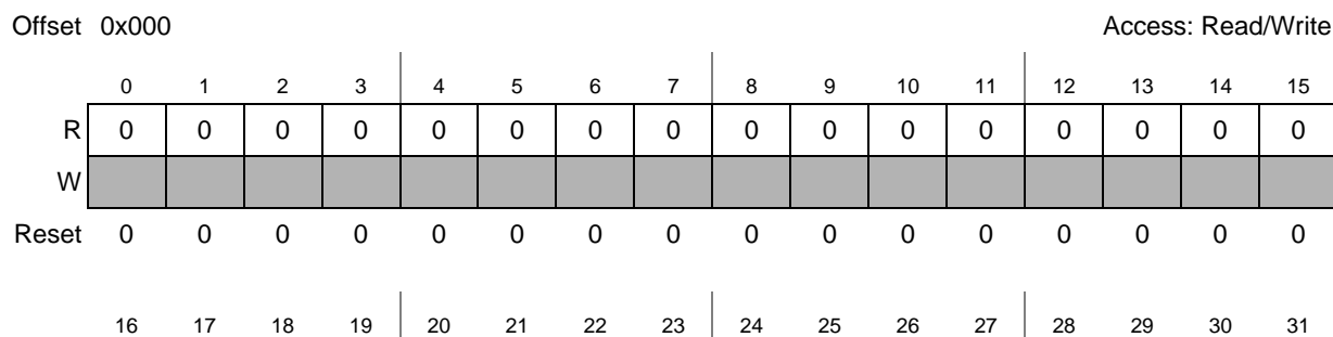
Figure 20-2. PIT Module Control Register (PIT_MCR)
