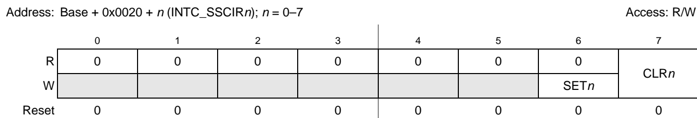
Figure 10-12. INTC Software Set/Clear Interrupt Register (INTC_SSCIR n )
