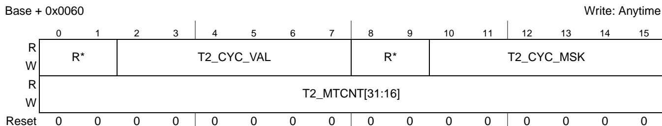
Figure 22-42. Timer 2 Configuration Register 0 (TI2CR0)
