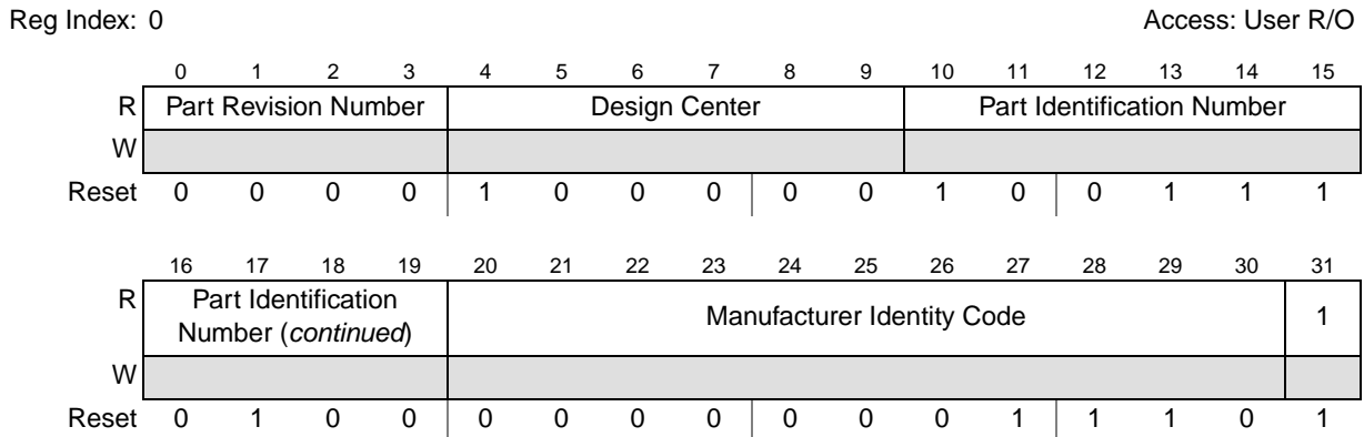
Figure 31-3. Nexus Device ID Register (DID)
