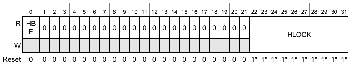
Figure 12-5. FLASH_x_HLR Register
