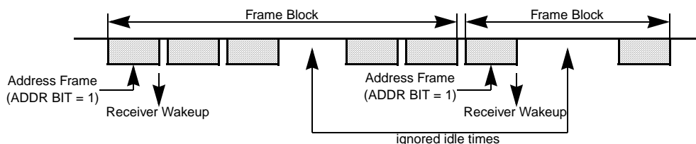
Figure 26-37. Address-Mark Wakeup Format
