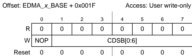
Figure 21-16. eDMA Clear DONE Status Bit Register (EDMA_x_CDSBR)
