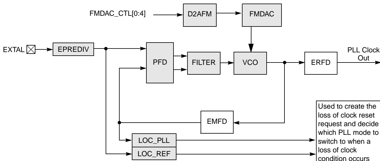
Figure 6-2. FMPLL Block Diagram
