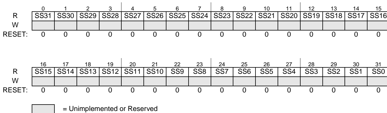
Figure 29-22. ETPUCSSR Register
