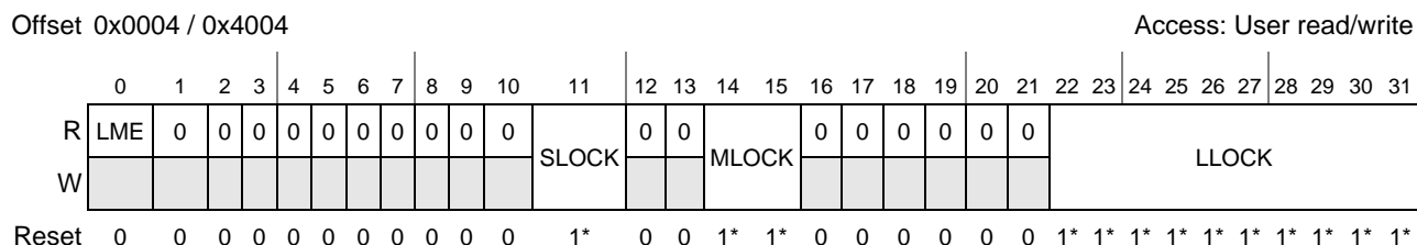
Figure 12-4. FLASH_x_LMLR Register
