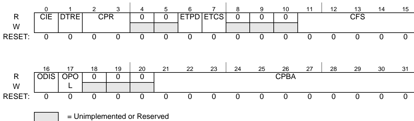
Figure 29-23. ETPUCxCR Register
