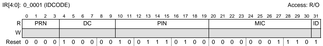
Figure 32-3. Device Identification Register
