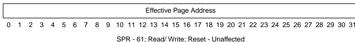
Figure 13-5. DEAR
