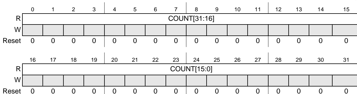
Figure 28-12. Decimation Filter Final Integration Count Value Register (DECFILT_x_FINTCNT)
