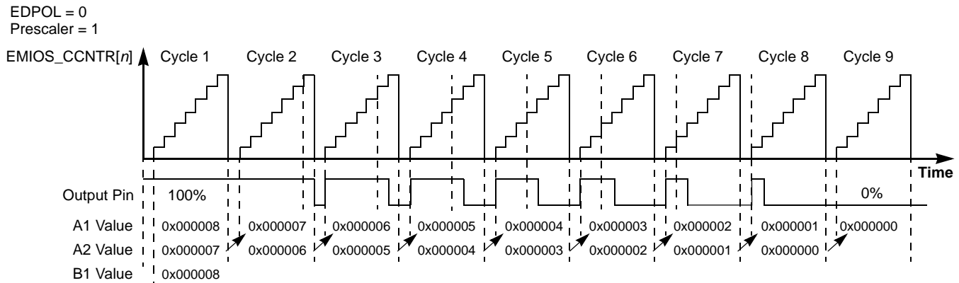
Figure 23-44. OPWFB Mode from 100% to 0% Duty Cycle
