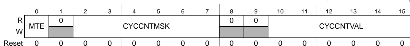
Figure 22-49. MTS B Configuration Register (MTSBCFR)
