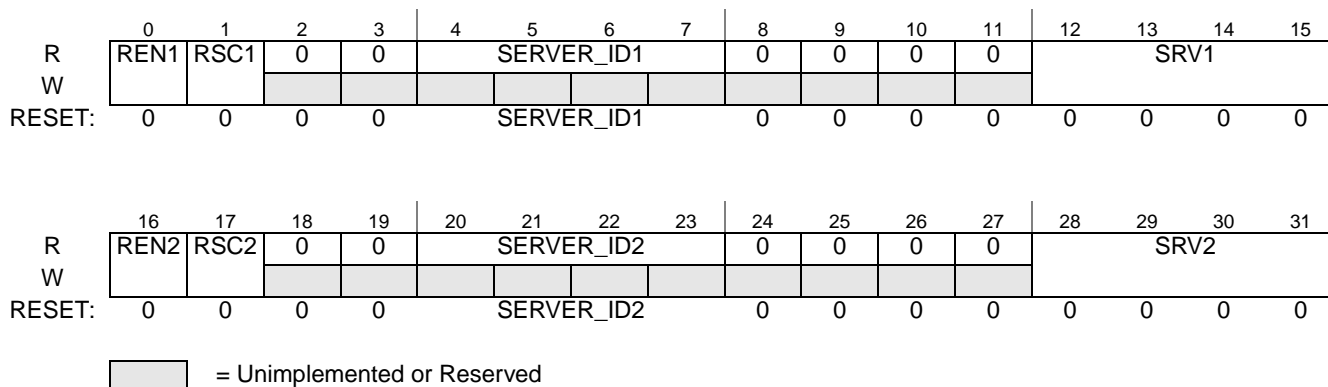
Figure 29-11. ETPUREDCCR Register
