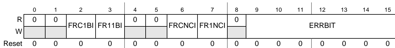
Figure 17-4. ECC Error Generation (ECSM_EEGR) Register
