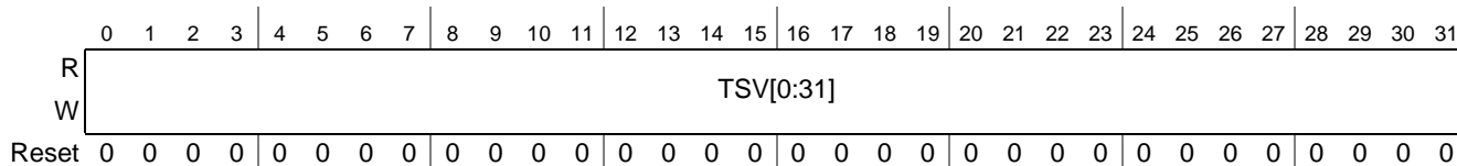
Figure 20-3. Timer Load Value Register (PIT_RTI_LDVAL, PIT_CH n _LDVAL)
