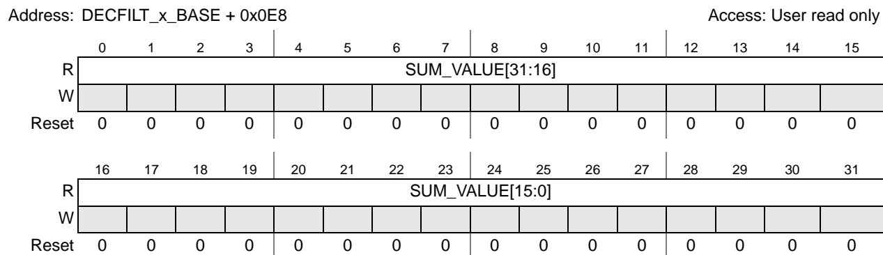
Figure 28-13. Decimation Filter Current Integration Value Register (DECFLT_x_CINTVAL)
