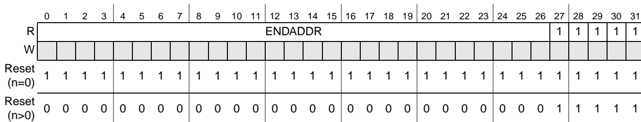
Figure 16-6. MPU Region Descriptor, Word 1 Register (MPU_RGD n .Word1)
