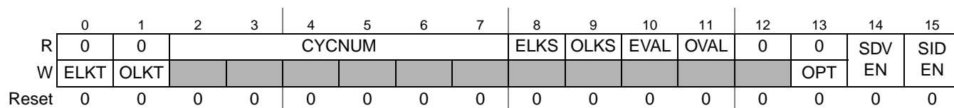
Figure 22-33. Sync Frame Table Configuration, Control, Status Register (SFTCCSR)
