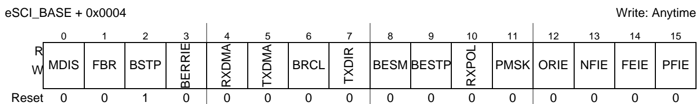
Figure 26-4. Control Register 2 (eSCI_CR2)
