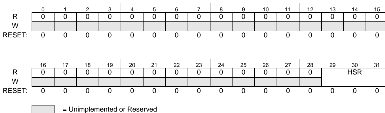
Figure 29-25. ETPUCxHSRR Register
