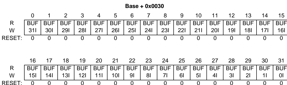
Figure 24-14. Interrupt Flags 1 Register (FLEXCAN_x_IFLAG1)
