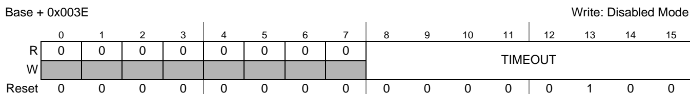
Figure 22-30. System Memory Access Time-Out Register (SYMATOR)
