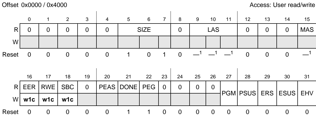
Figure 12-3. Module Configuration Register (FLASH_x_MCR)
