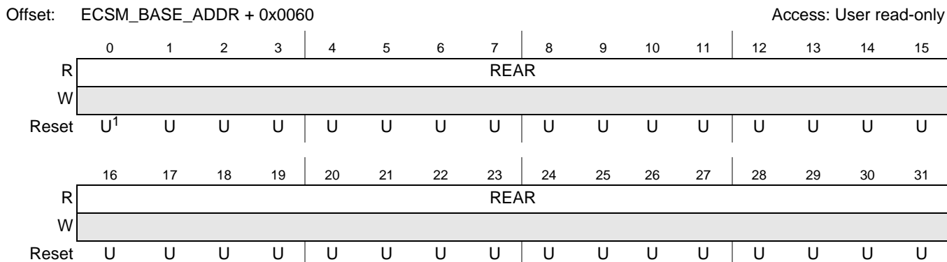
Figure 17-10. RAM ECC Address (ECSM_REAR) Register
