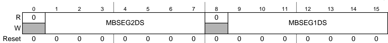
Figure 22-7. Message Buffer Data Size Register (MBDSR)
