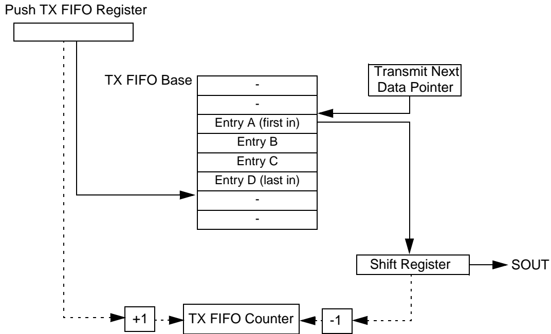
Figure 25-42. TX FIFO Pointers and Counter
