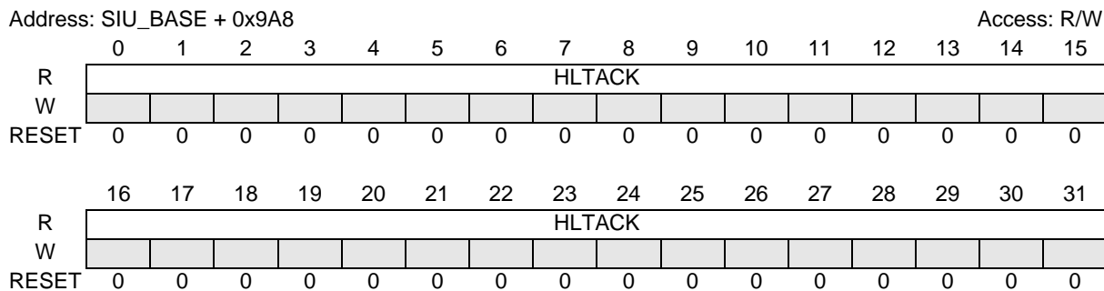
Figure 7-27. Halt Acknowledge Register (SIU_HLTACK)
