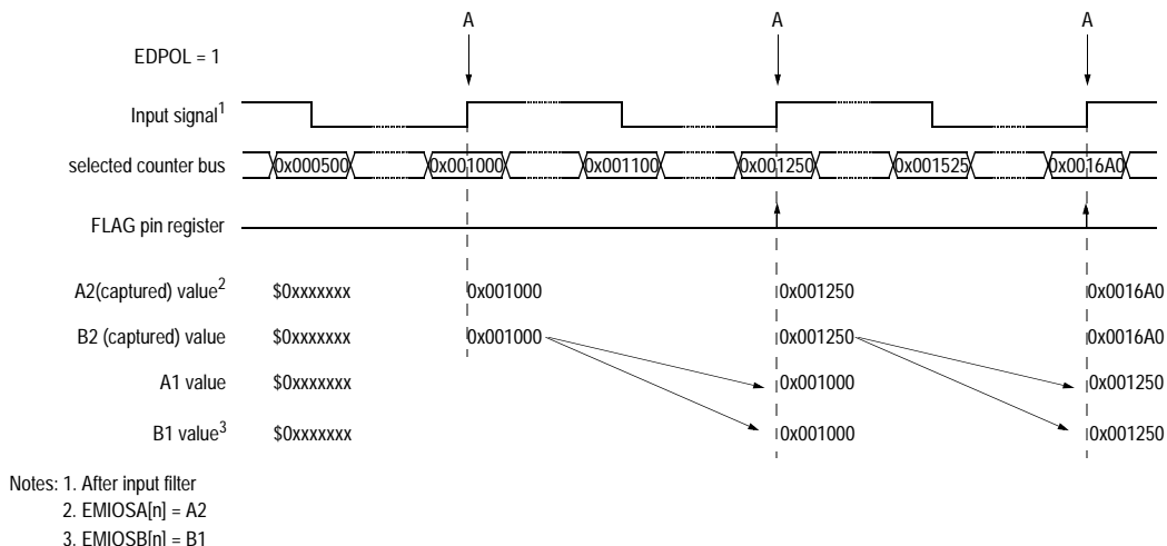
Figure 23-20. IPM Example
