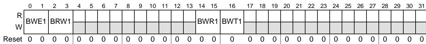
Figure 31-49. Break / Watchpoint Control Register 1 (BWC1)
