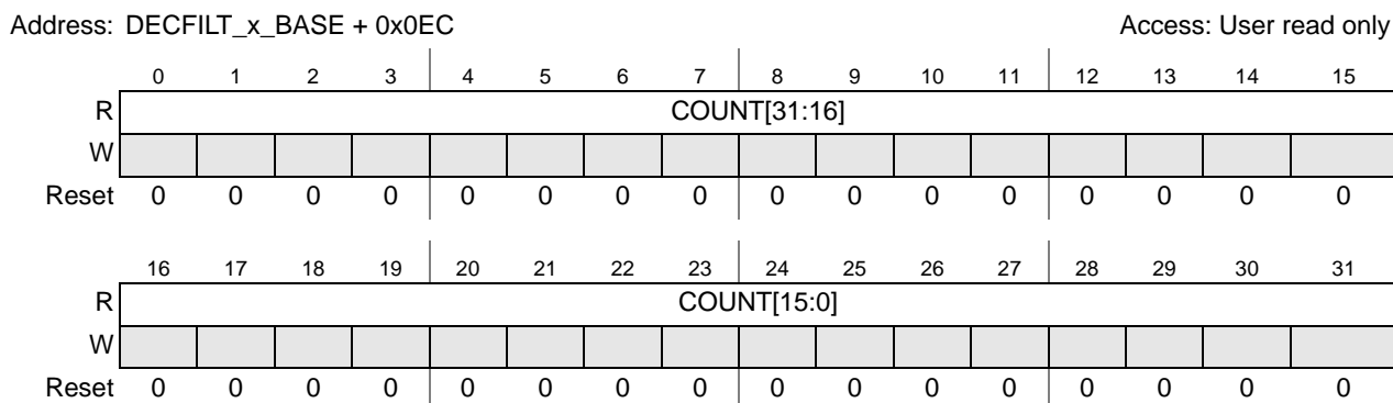
Figure 28-14. Decimation Filter Current Integration Count Value Register (DECFLT_x_CINTCNT)
