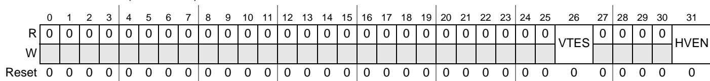
Figure 10-7. INTC Module Configuration Register (INTC_MCR)
