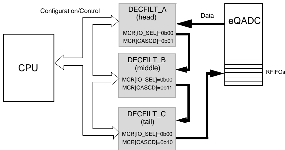
Figure 28-18. Cascaded Filters
