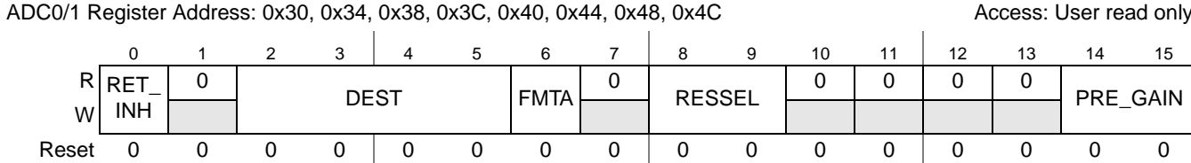
Figure 28-21. Alternate Configuration 1-8 Control Registers (ADC_ACR1-8)
