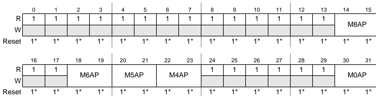
Figure 12-11. Flash Bus Interface Access Protection Register (FLASH_BIUAPR)
