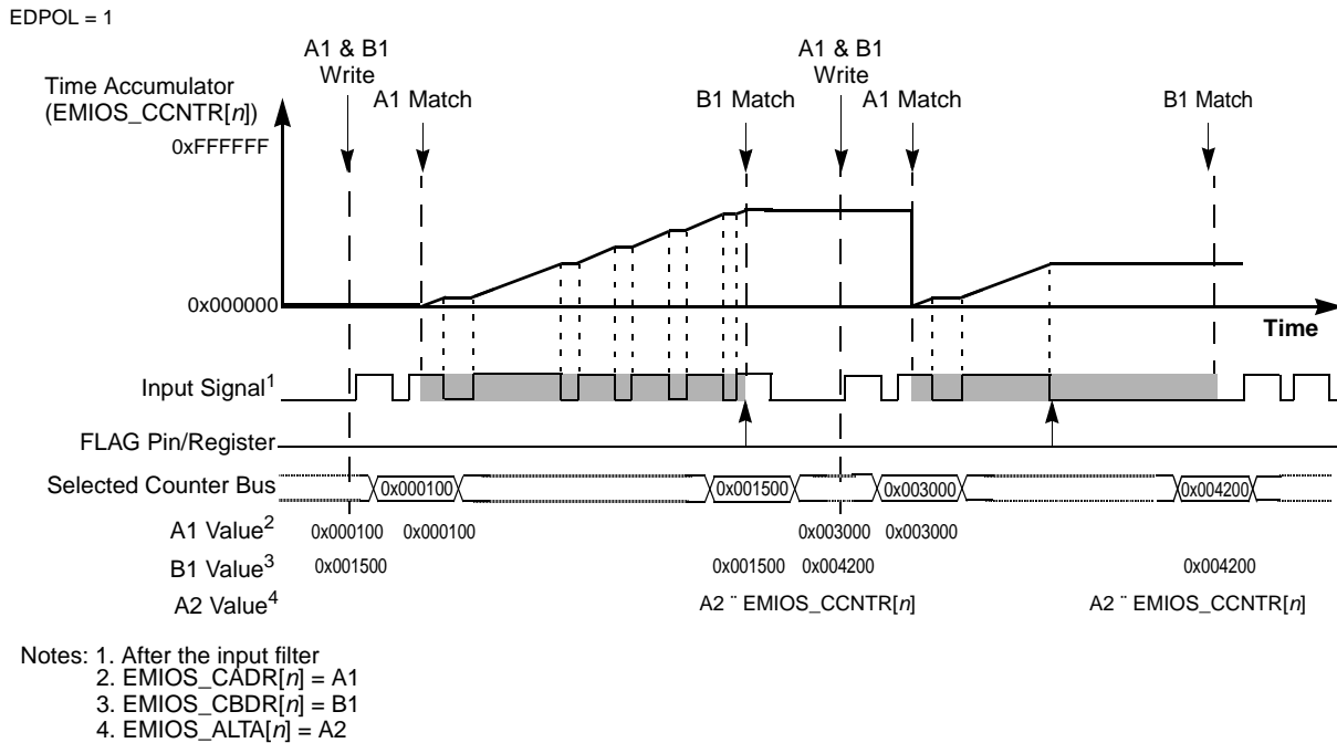
Figure 23-31. WTPA Example
