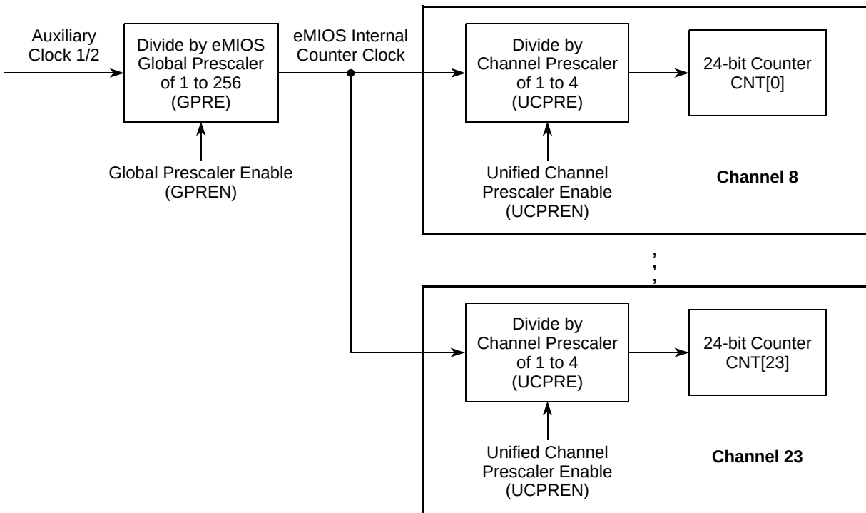
Figure 18-14. eMIOS prescalers
