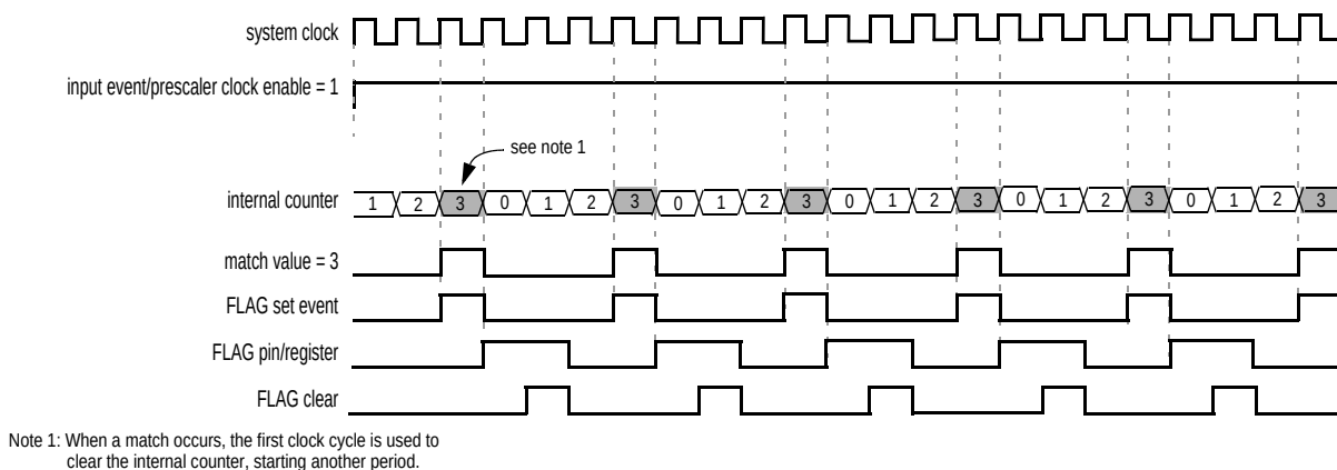
Figure 18-38. Time base period when running in the fastest prescaler ratio
