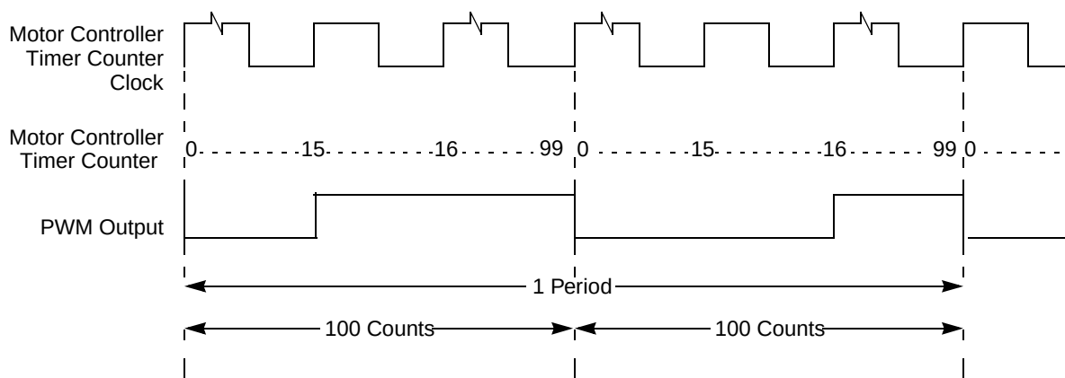
Figure 41-28. PWM Output: MCCTL0[DITH] = 1 , MCCx[MCAM] = 0x1 , MCDCx[DUTY] = 31 , MCPER[PER] = 200 , MCCTL1[RECIRC] = 0
