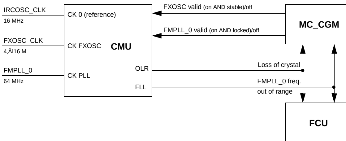
Figure 8-33. CMU component interaction
