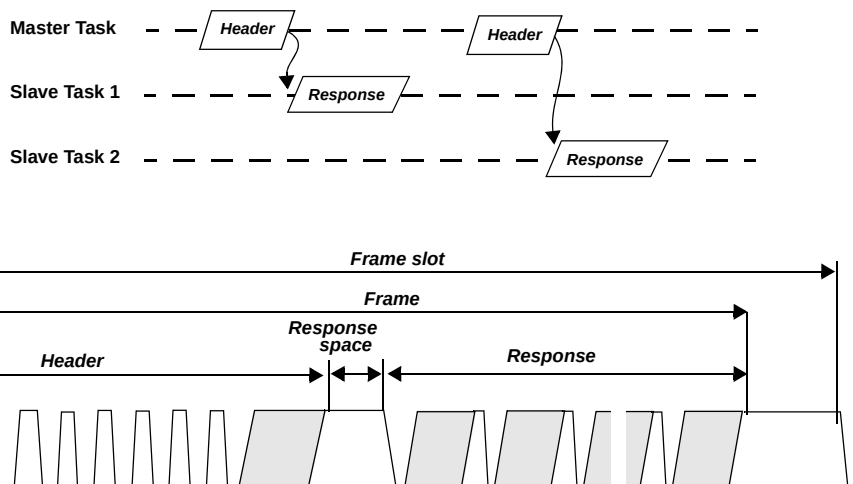
Figure 27-3. LIN frame structure
