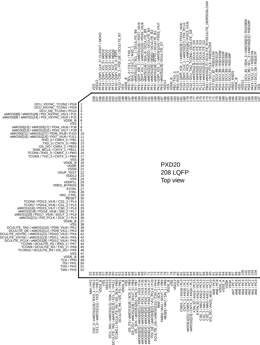
Figure 3-2. 208-pin LQFP pinout
