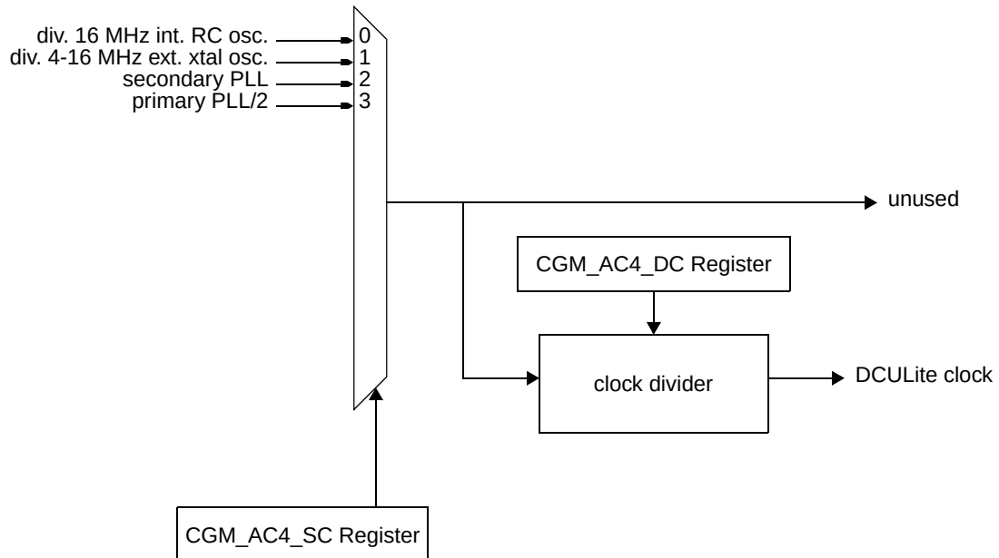
Figure 8-24. MC_CGM Auxiliary Clock 4 Generation Overview
