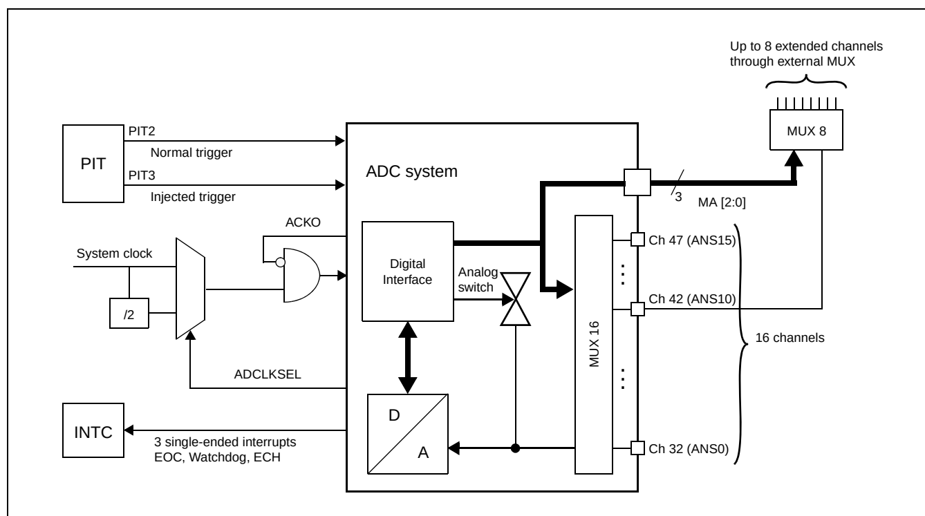
Figure 5-1. ADC implementation
