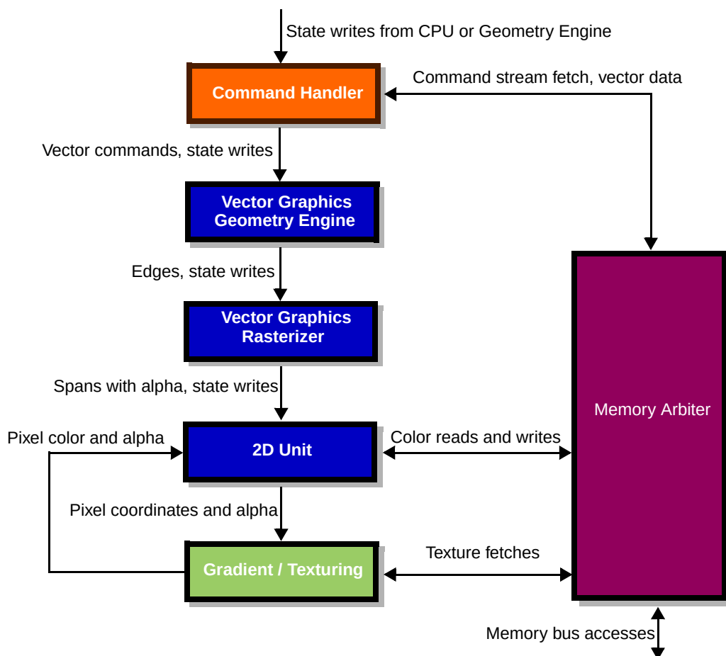
Figure 31-13. 2D+VG Architecture
