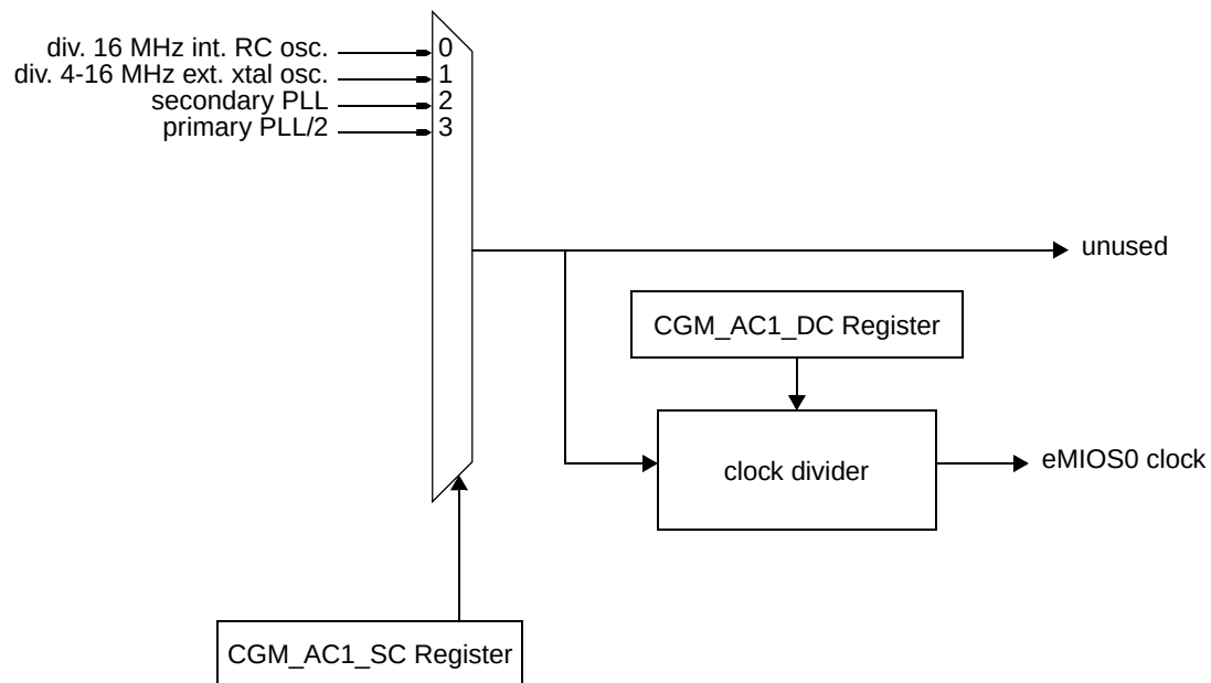
Figure 8-21. MC_CGM Auxiliary Clock 1 Generation Overview
