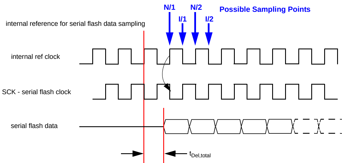
Figure 35-20. Serial Flash Sampling Clock Timing
