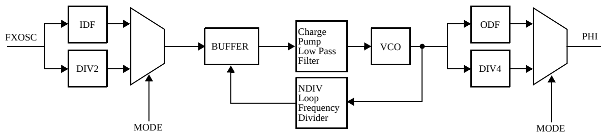
Figure 8-30. FMPLL block diagram
