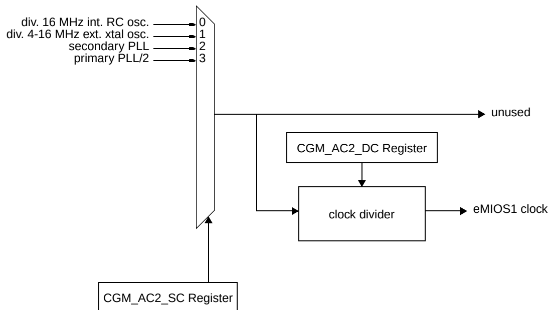
Figure 8-22. MC_CGM Auxiliary Clock 2 Generation Overview
