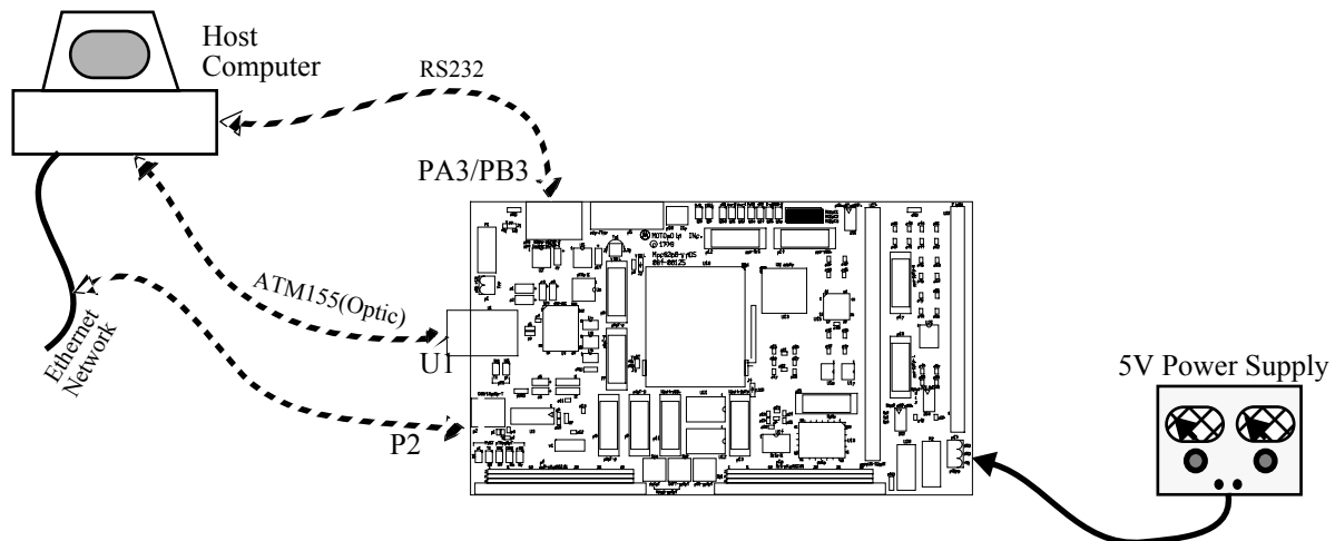
Figure 2-8. Stand Alone Configuration
