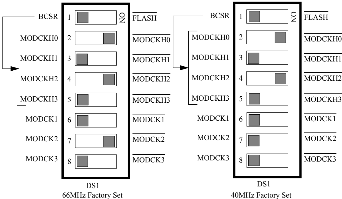
Figure 2-4. DS1 Description
