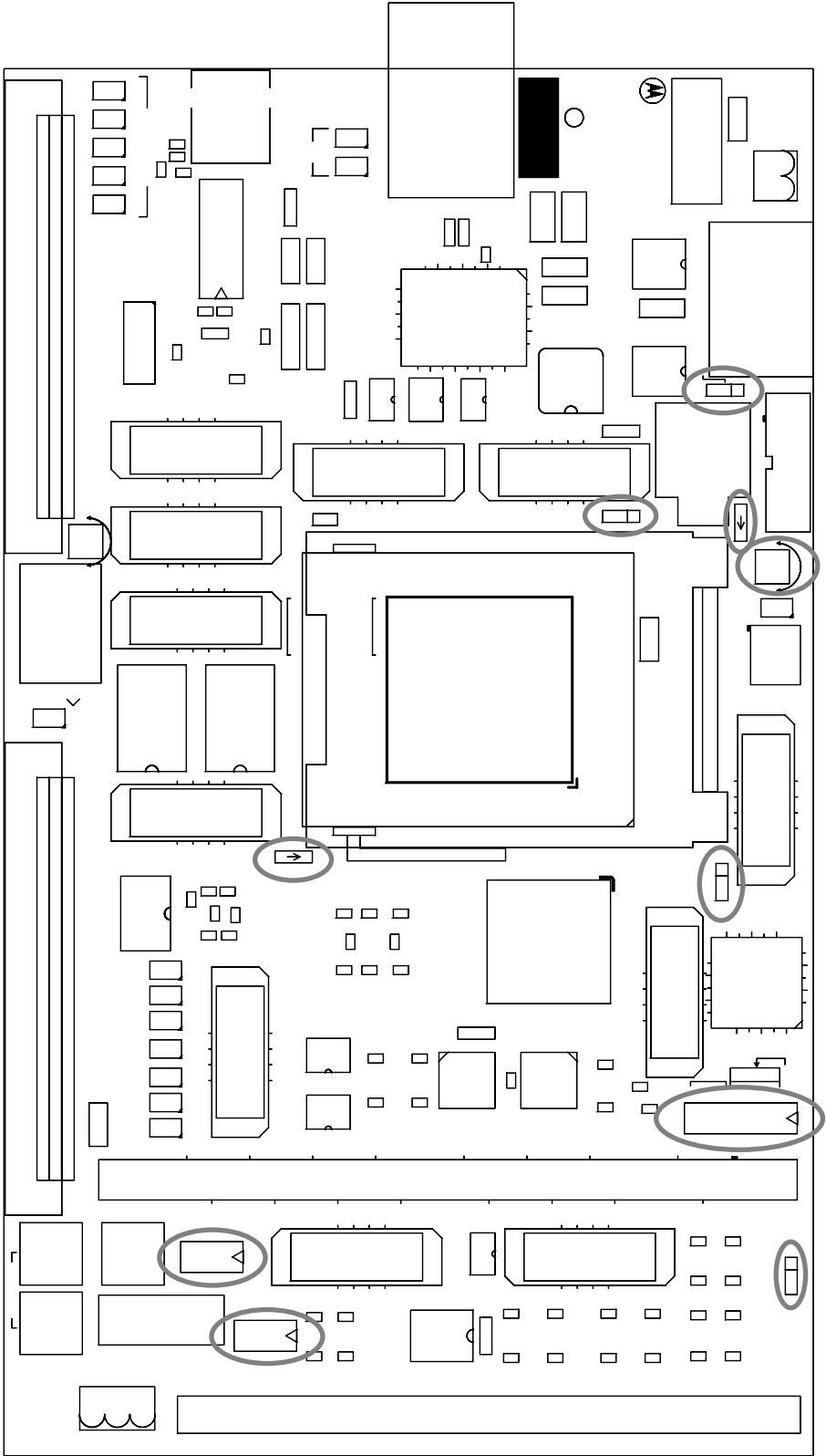
Figure 2-1. MPC8260ADS Top Side Part Location Diagram
