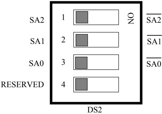
Figure 2-6. DS2 Description
