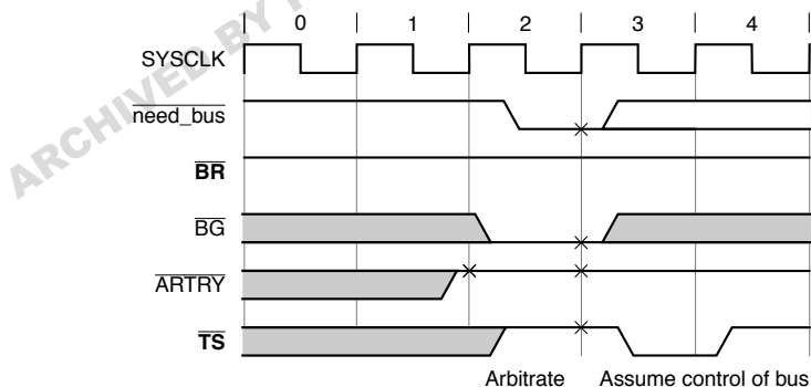
Figure 9-20. Bus Arbitration—Parked Case
