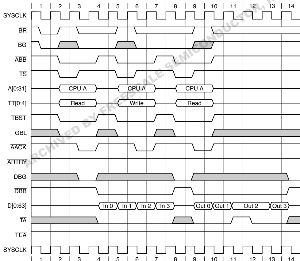
Figure 9-17. Burst Transfers with Data Delay Controls
