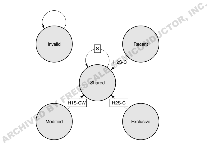
Figure 3-19. Read Transaction—MPX Bus Mode, L1\_INTVEN = 0b111
