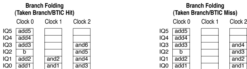
Figure 6-11. Branch Folding
