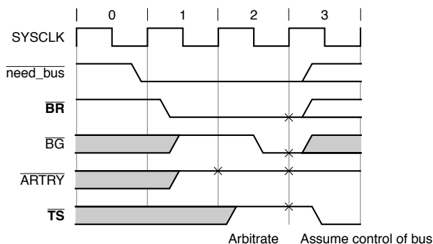
Figure 9-19. MPX Bus Address Bus Arbitration—Non-Parked Case
