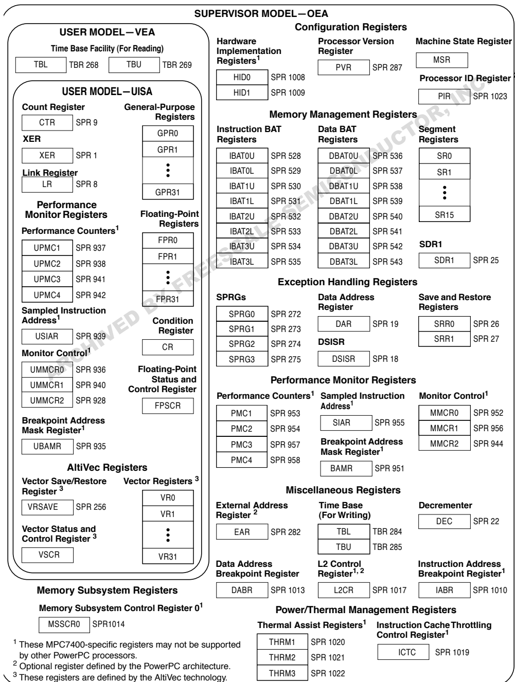
Figure 2-1. Programming Model—MPC7400 Microprocessor Registers
