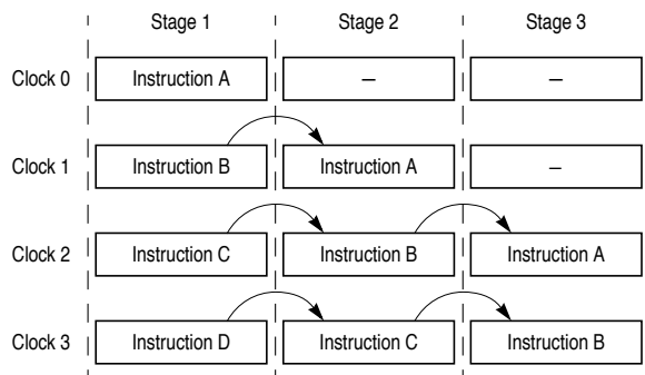
Figure 6-1. Pipelined Execution Unit
