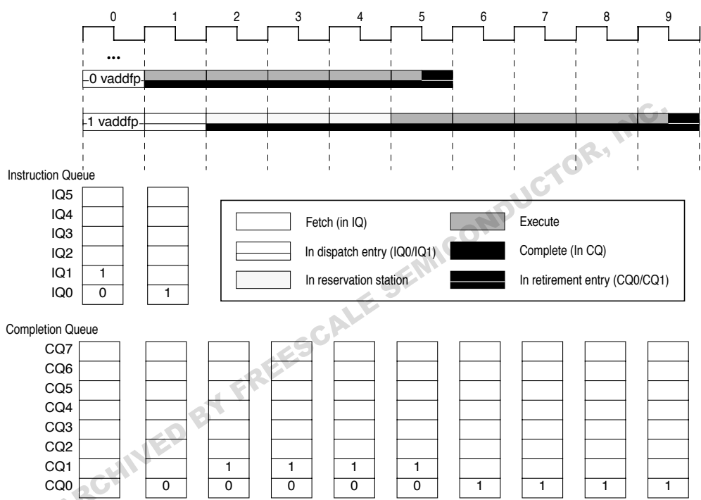
Figure 6-16. Data Forwarding in Java Mode
