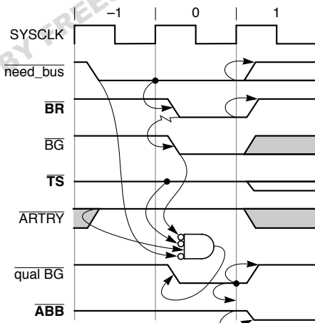
Figure 9-4. Address Bus Arbitration
