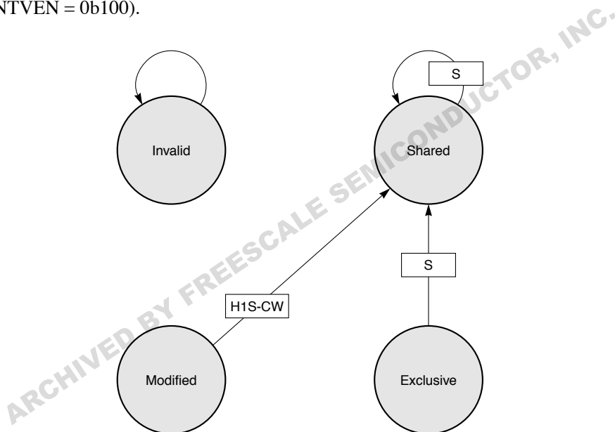
Figure 3-8. Read Transaction—MPX Bus Mode, L1_INTVEN = 0b100
