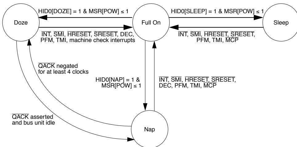
Figure 10-1. Power Management State Diagram
