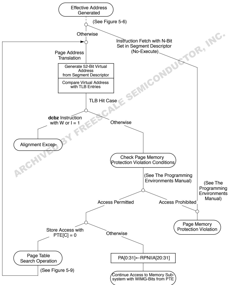
Figure 5-10. Page Address Translation Flow—TLB Hit
