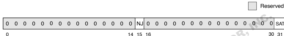
Figure 7-2. Vector Status and Control Register (VSCR)
