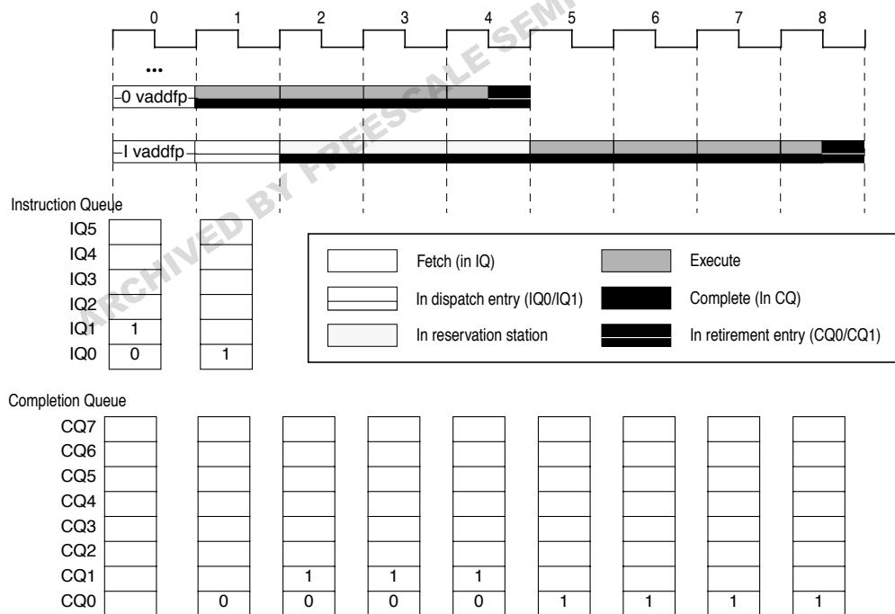
Figure 6-15. Data Dependencies in Non-Java Mode
