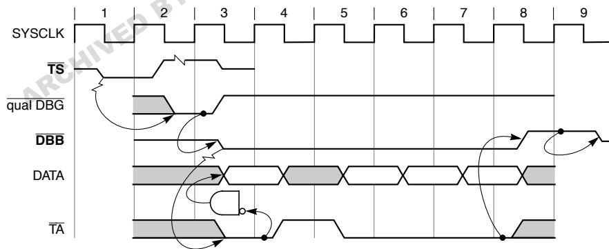
Figure 9-12. Read Burst with \overline{TA} Wait States
