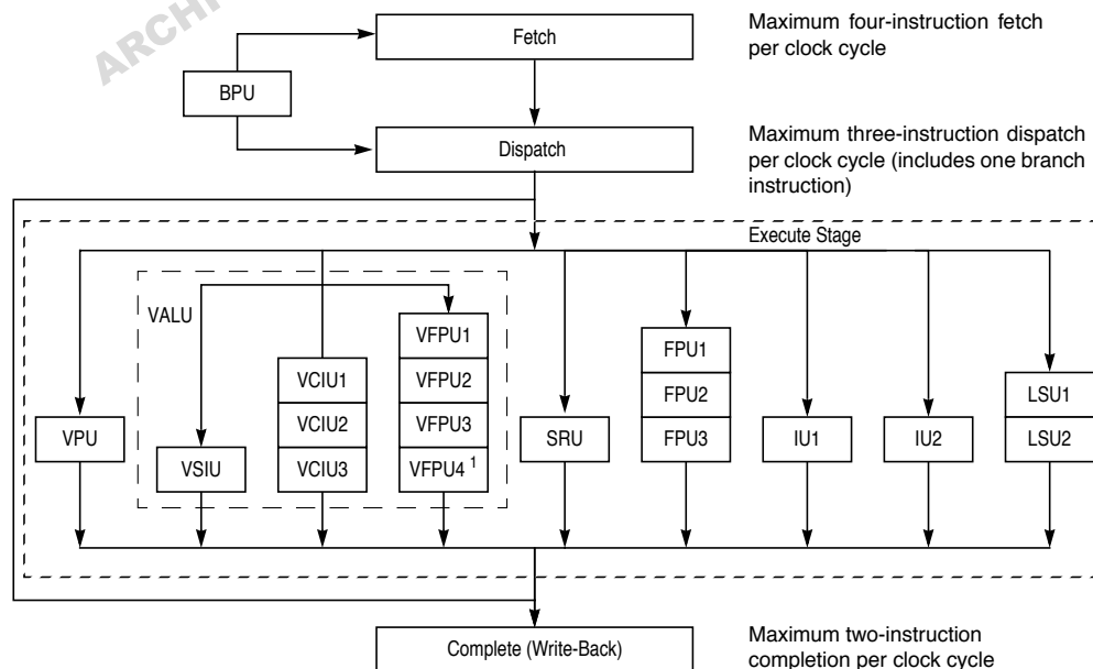
Figure 6-2. Superscalar/Pipeline Diagram
