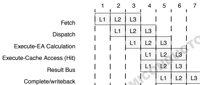
Figure 6-7. Data L1 Load Hit (No Stalls)
