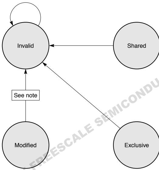
Figure 3-18. Kill Transaction—MPX Bus Mode, L1_INTVEN = 0b110
