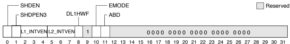
Figure 2-14. Memory Subsystem Control Register (MSSCR0)
