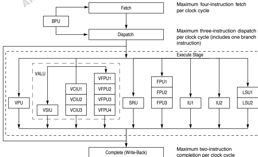
Figure 1-6. Pipeline Diagram
