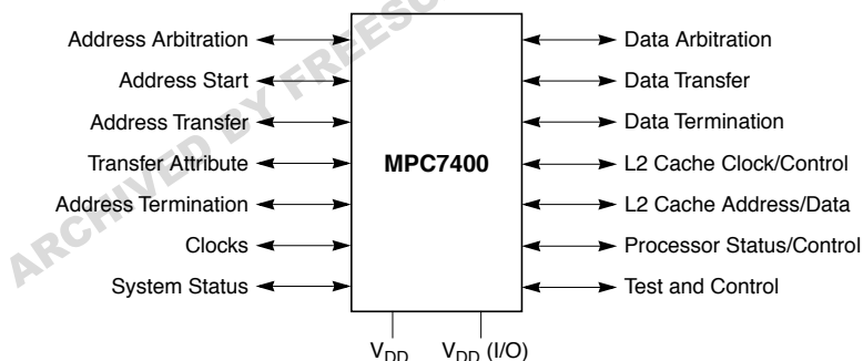
Figure 1-3. System Interface
