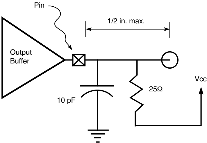
Figure 5. T val (max) Falling Edge
