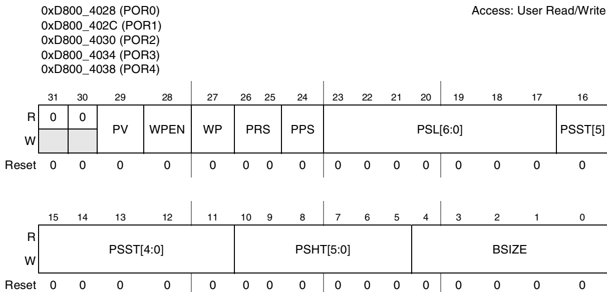
Figure 20-7. PCMCIA Option Registers 0–4 (POR0–POR4)
