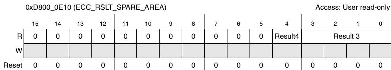
Figure 19-13. ECC_Rslt_Spare_Area Register
