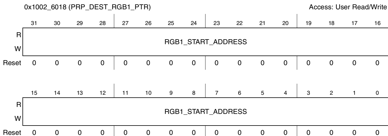
Figure 41-34. PrP Destination RGB1 Start Address Register
