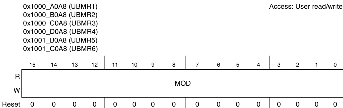
Figure 28-16. UART BRM Modulator Register Summary (UBMR)
