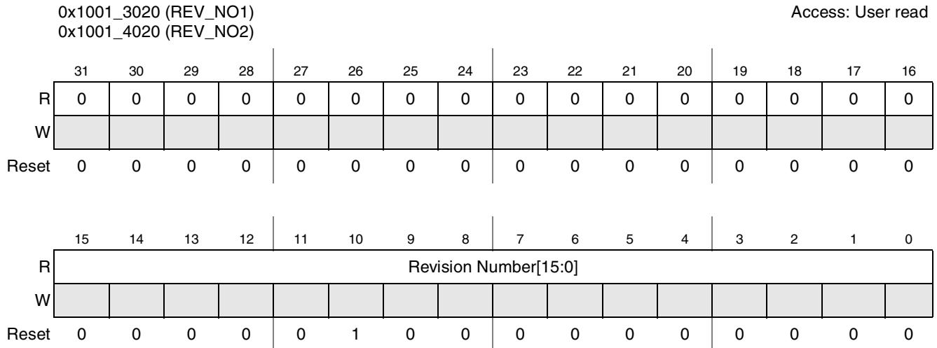
Figure 27-12. SDHC Revision Number Register
