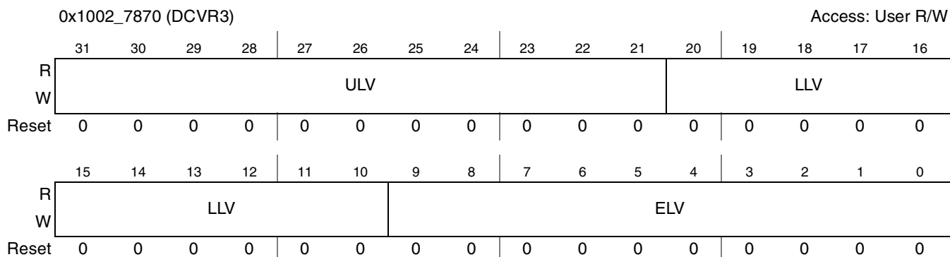
Figure 4-25. DPTC Comparator Value Register 3 (DCVR3)
