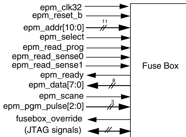
Figure 14-31. Fuse Box Interface
