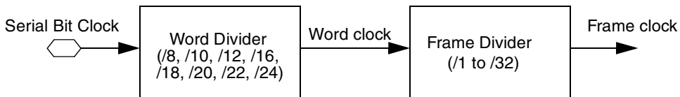
Figure 42-44. SSI Clocking
