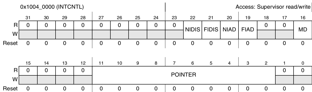
Figure 10-3. Interrupt Control Register Format
