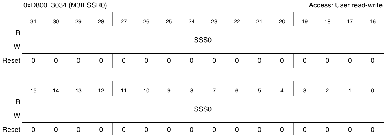
Figure 16-7. M3IF Snooping Status Register 0 (M3IFSSR0)
