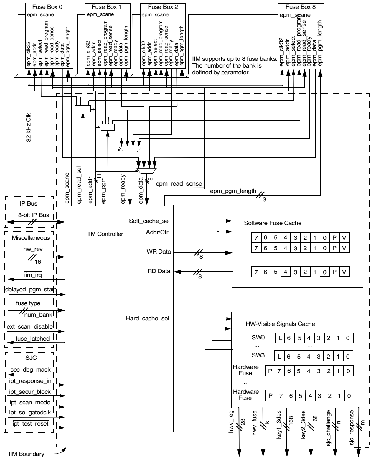
Figure 14-1. IIM Microarchitecture
