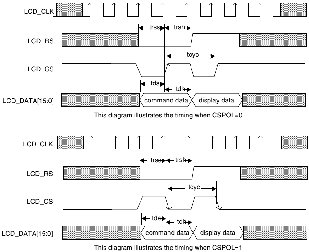
Figure 44-24. SLCDC Parallel Transfers to LCD Device
