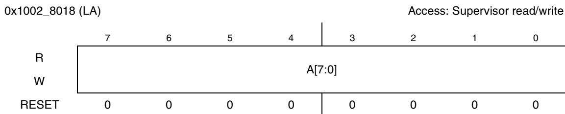
Figure 14-9. Lower Address Register
