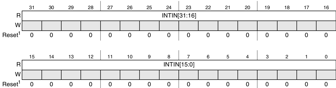
Figure 10-22. Interrupt Source Register High Format
