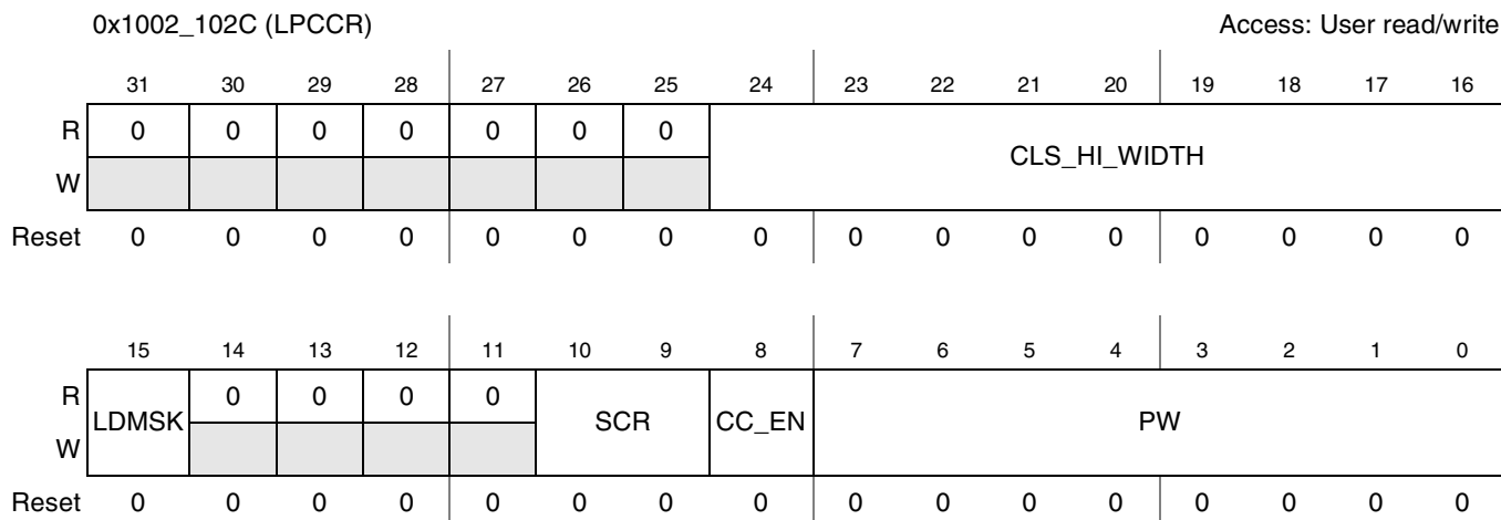
Figure 43-35. LCDC PWM Contrast Control Register (LPCCR)
