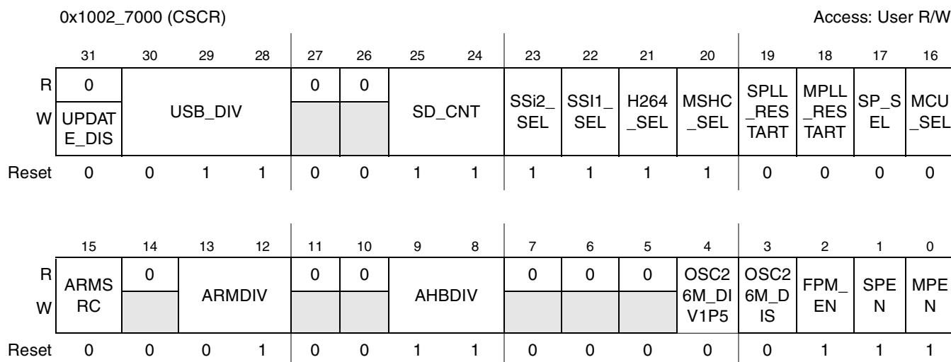
Figure 3-4. Clock Source Control Register (CSCR)
