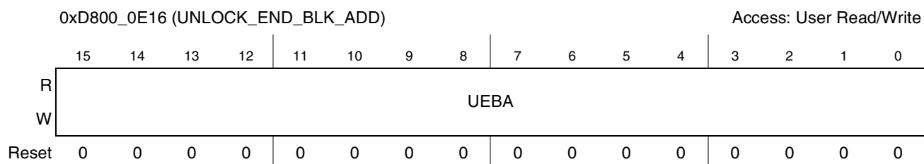
Figure 19-16. UNLOCK_END_BLK_ADD Register
