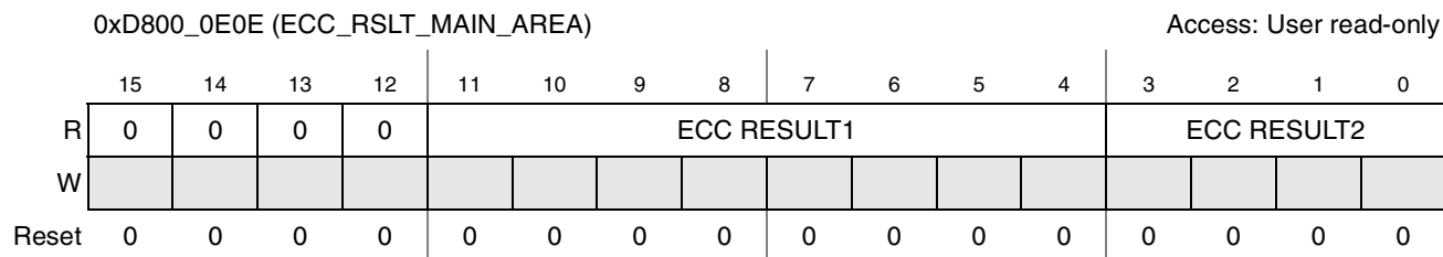
Figure 19-11. ECC_RSLT_MAIN_AREA Register
