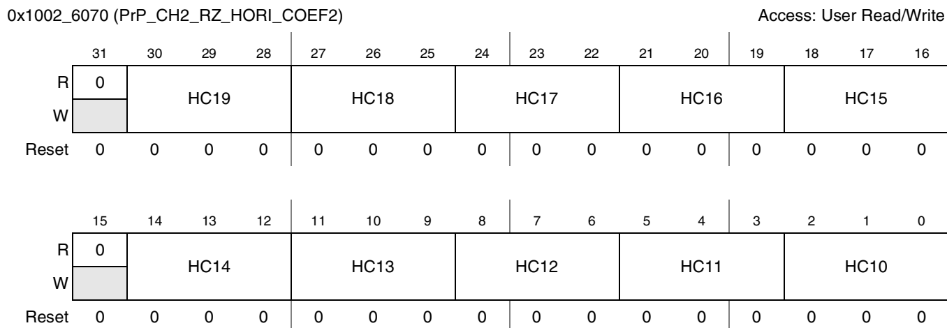
Figure 41-56. PrP Channel-2 Horizontal Resize Coefficient 2
