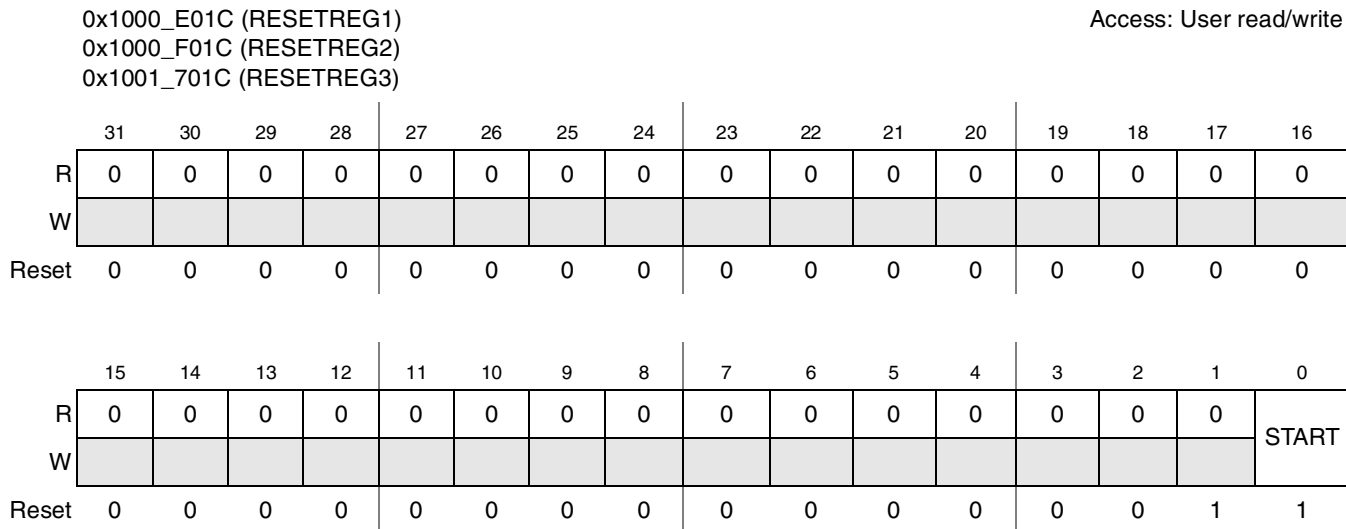
Figure 23-22. Reset Register Diagram
