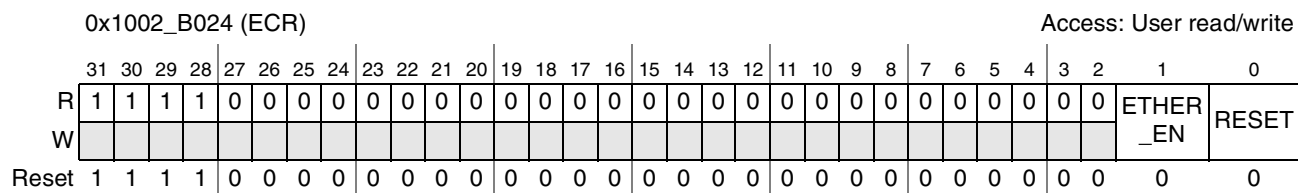
Figure 29-8. ECR Register
