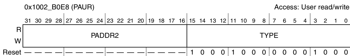
Figure 29-15. PAUR Register
