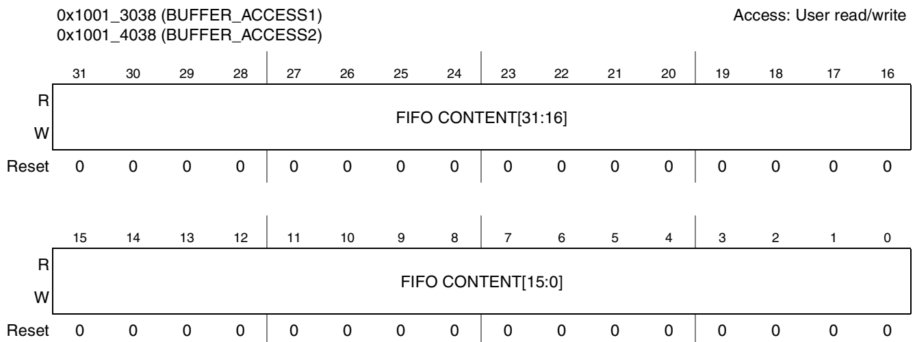
Figure 27-17. SDHC Buffer Access Register
