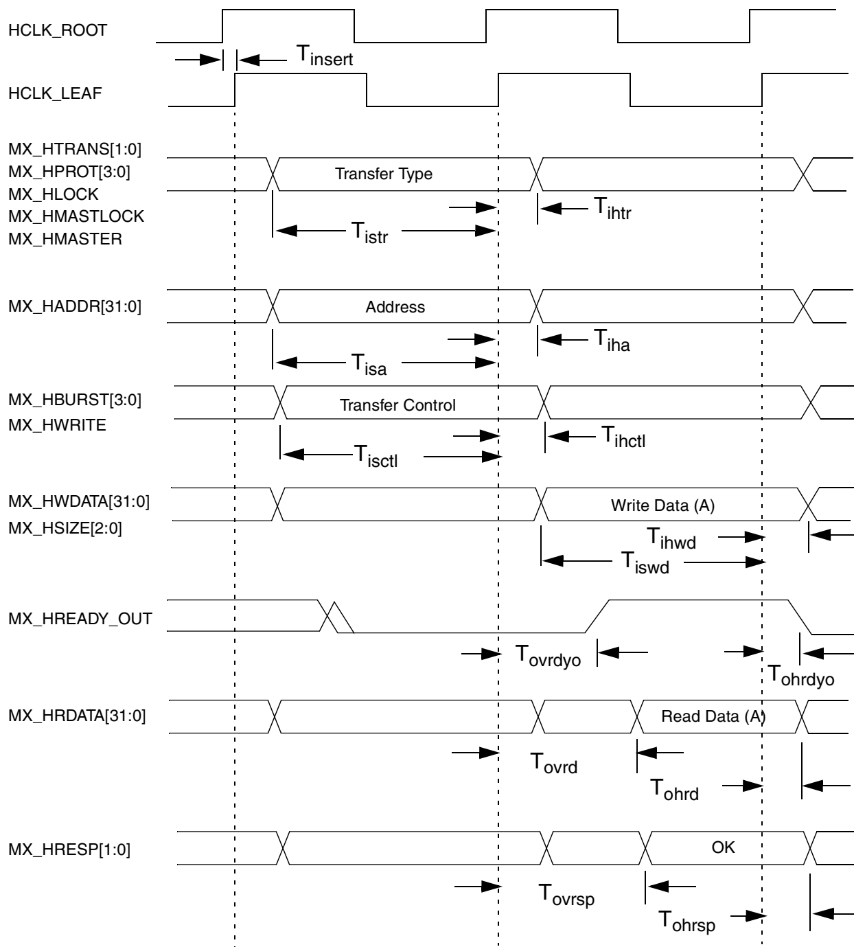
Figure 9-11. Alternate Bus Master Timing Parameters
