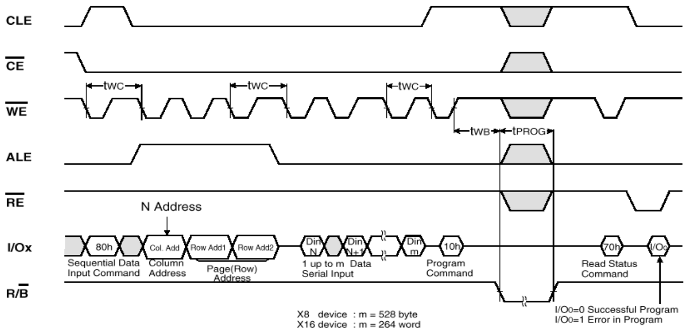
Figure 19-22. Program Operation
