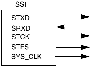
SSI Internal Continuous Clock (RXDIR=0, TXDIR=1, RFDIR=X, TFDIR=1, SYN=1, SYS_CLK_EN = 1) SSI I2S Master Mode (I2S_Mode=01, SYS_CLK_EN)
