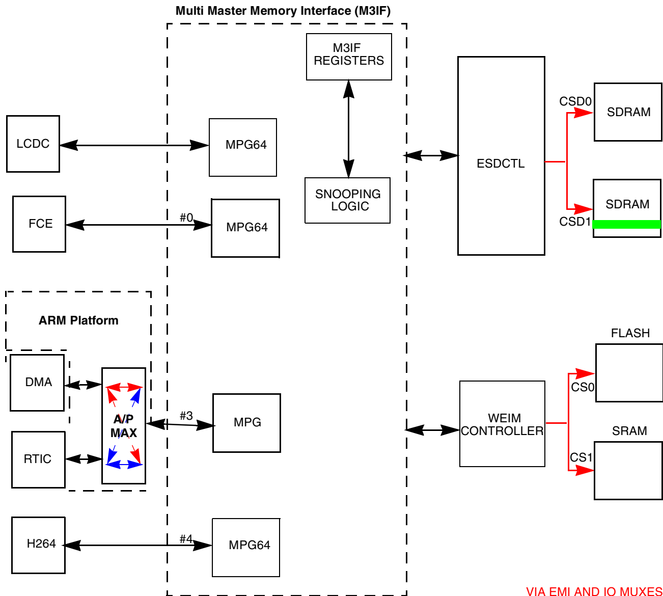
Figure 16-28. M3IF System Example
