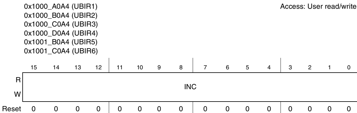
Figure 28-15. UART BRM Incremental Register Summary (UBIR)
