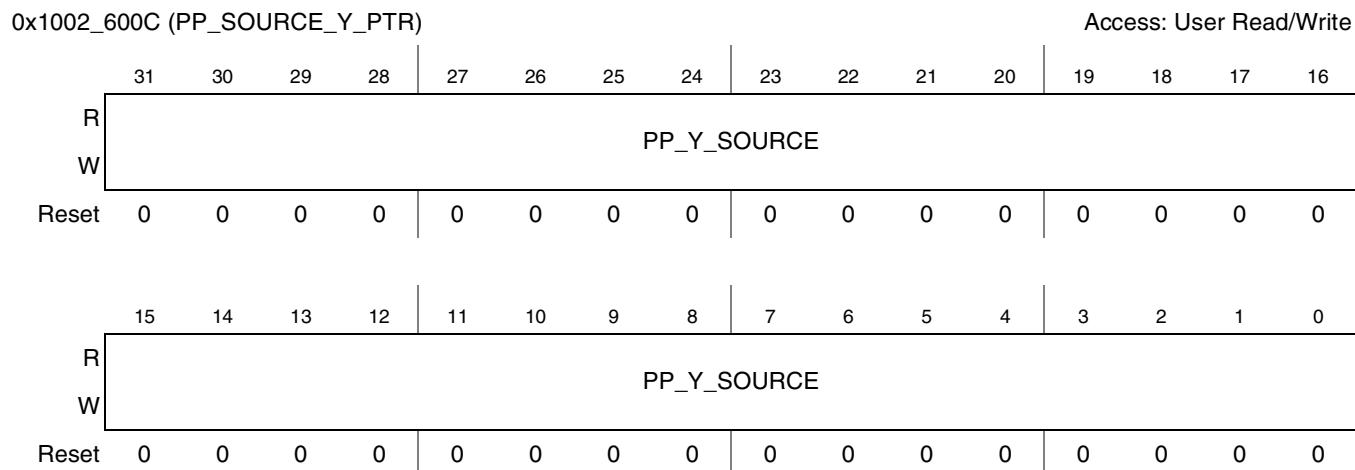
Figure 41-10. PP Source Y Address Register
