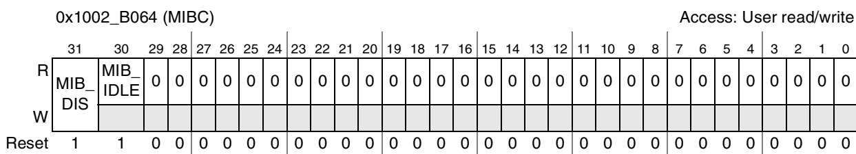
Figure 29-11. MIBC Register
