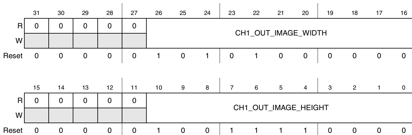
Figure 41-43. PrP Destination Channel-1 Output Image Size Register
