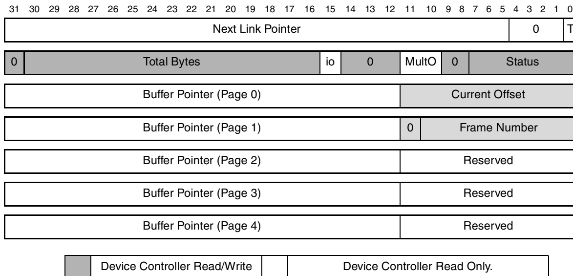
Figure 30-75. Endpoint Transfer Descriptor (dTD)
