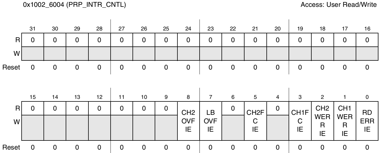
Figure 41-29. PRP Interrupt Control Register
