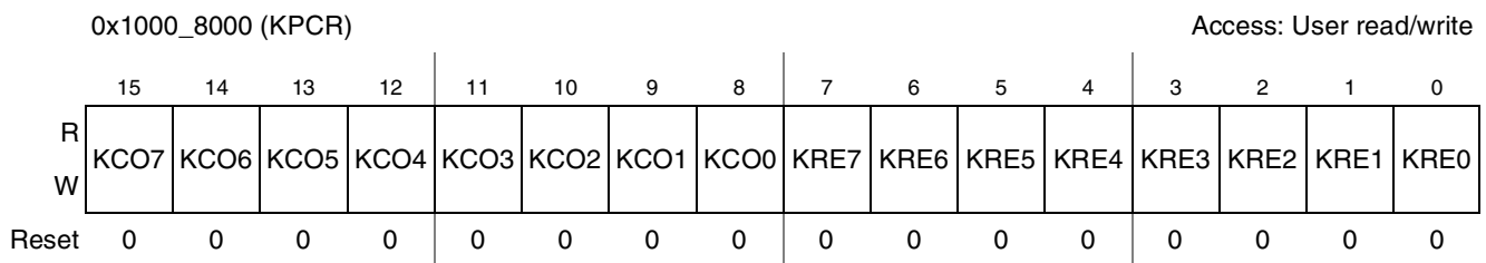
Figure 25-3. KPCR Register
