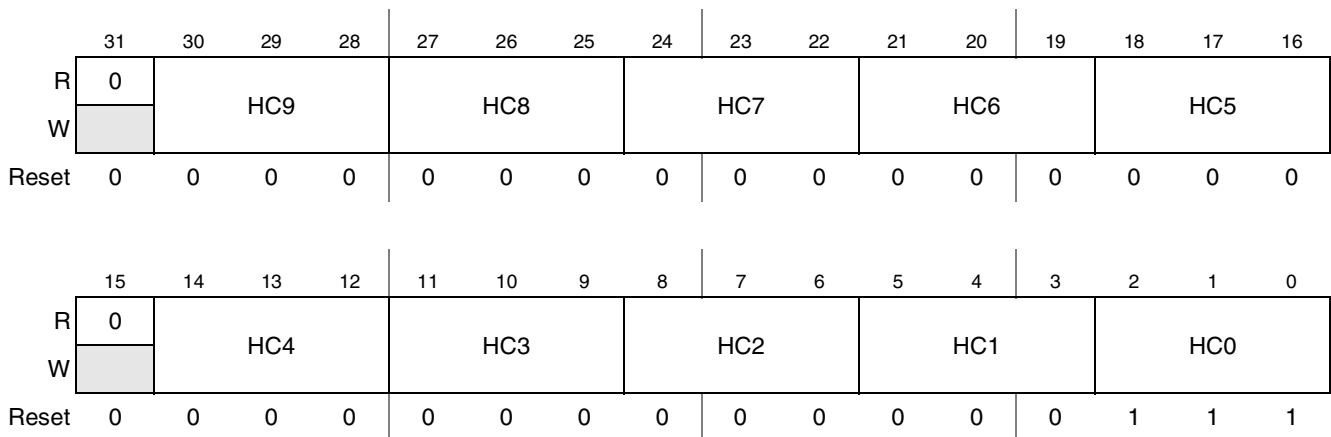
Figure 41-55. PrP Channel-2 Horizontal Resize Coefficient 1
