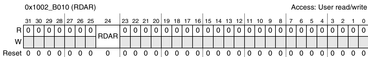
Figure 29-6. RDAR Register
