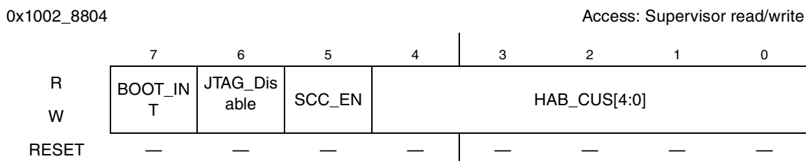
Figure 14-19. Word1 in Fusebank0r
