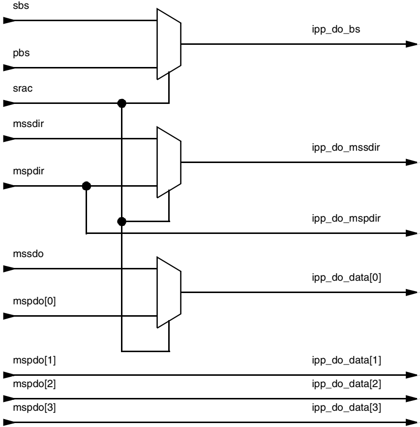
Figure 26-3. Gasket Memory Interface Logic
