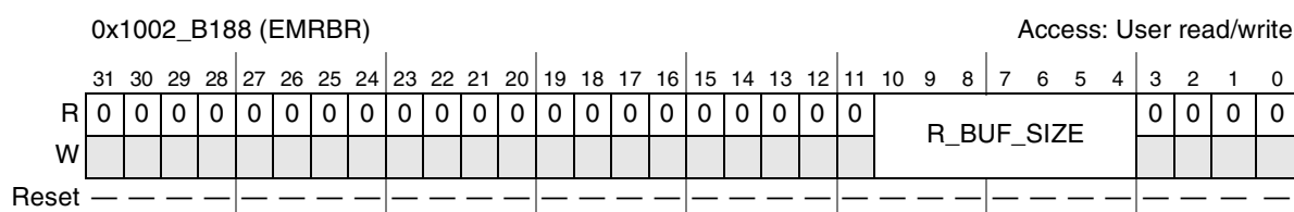
Figure 29-26. EMRBR Register
