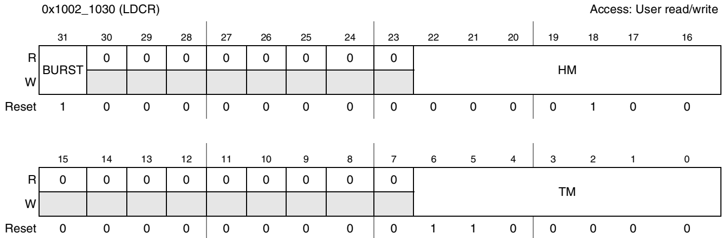
Figure 43-36. LCDC DMA Control Register (LDCR)
