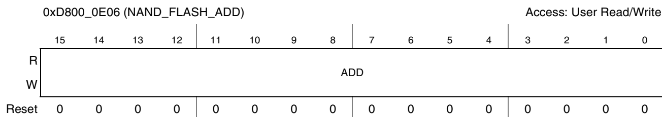
Figure 19-6. NAND Flash Address Register
