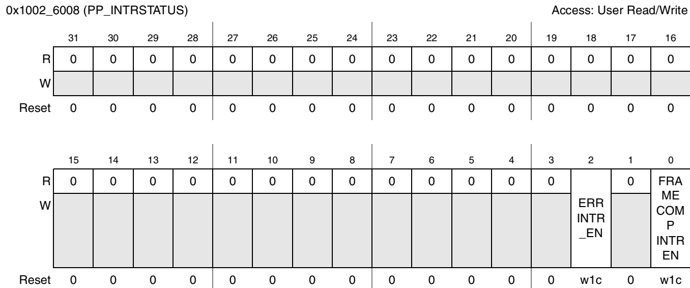
Figure 41-9. PP Interrupt Status Register
