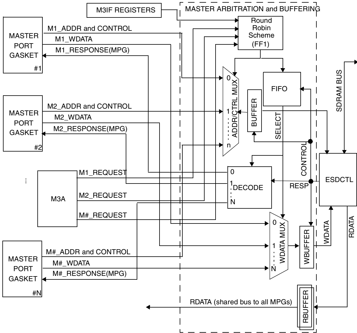
Figure 16-25. MAB Overview Block Diagram
