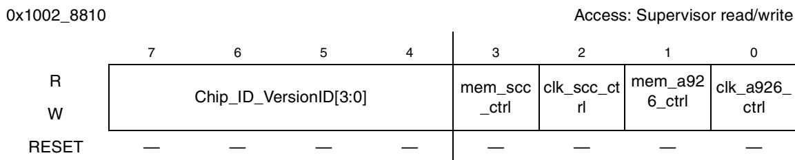
Figure 14-22. Words 3 of Fusebank0
