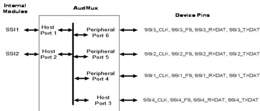
Figure 38-17. AUDMUX Pin Connections
