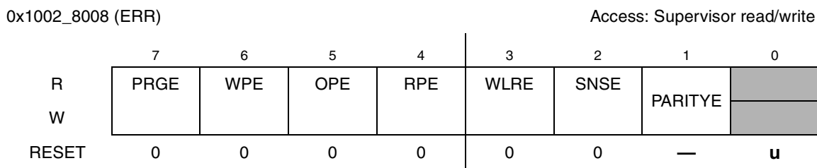
Figure 14-5. Module Errors Register
