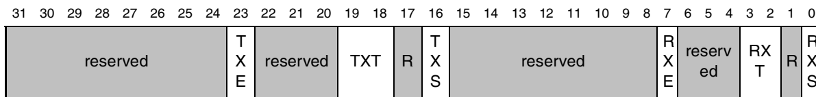
Figure 30-40. ENDPTCTRL0—Endpoint Control 0
