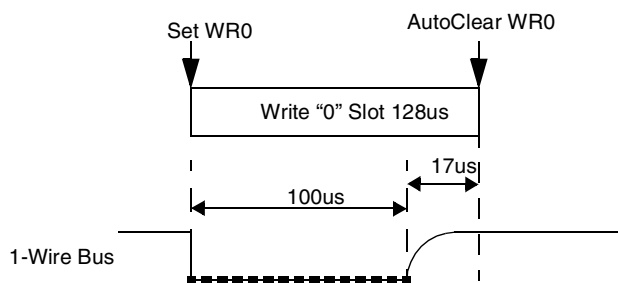
Figure 21-4. Write 0 Timing
