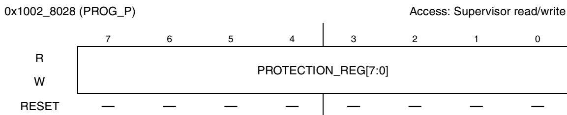
Figure 14-13. Program Protection Register
