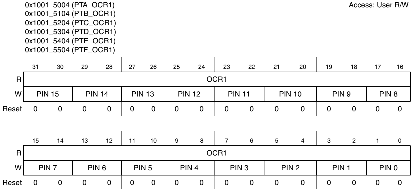
Figure 6-5. Output Configuration Register 1 (OCR1)
