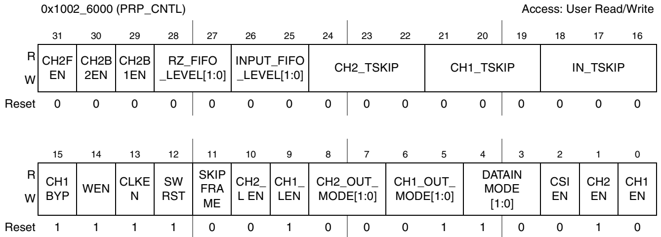
Figure 41-28. PRP Control Register
