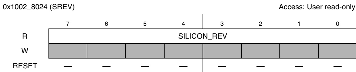
Figure 14-12. Silicon Revision Register
