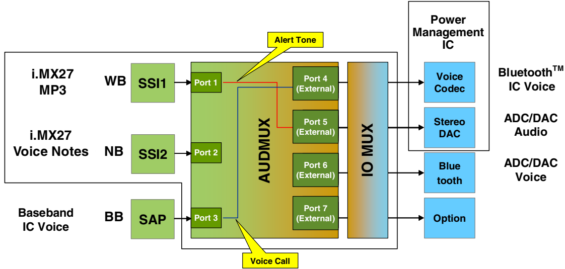
Figure 1-7. Typical AUDMUX Application
