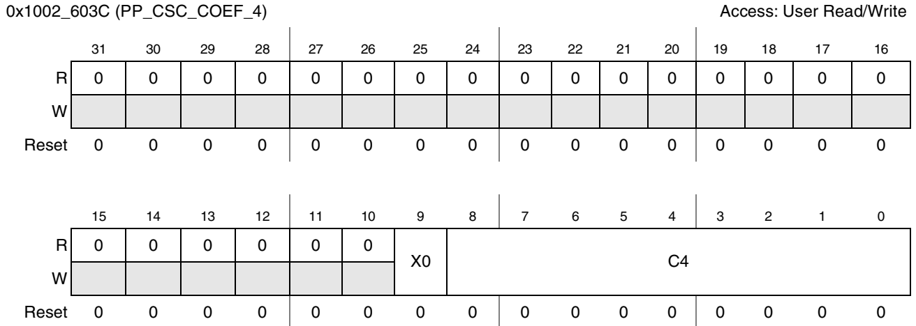
Figure 41-22. PP CSC Coefficient_4 Register
