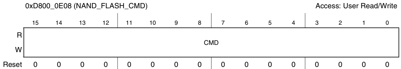
Figure 19-7. NAND_Flash_CMD Register
