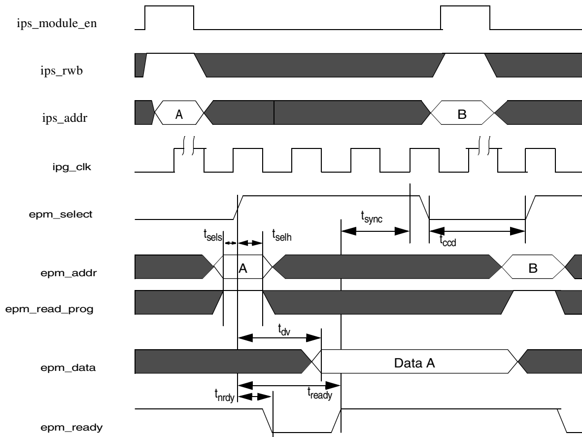
Figure 14-32. Fuse Box Read Cycle Timing
