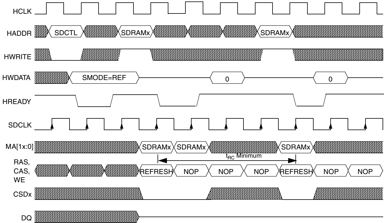
Figure 18-77. Software Initiated Auto-Refresh Timing Diagram
