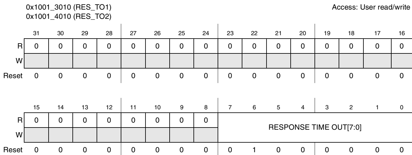
Figure 27-8. MMC/SD Response Time Out Register
