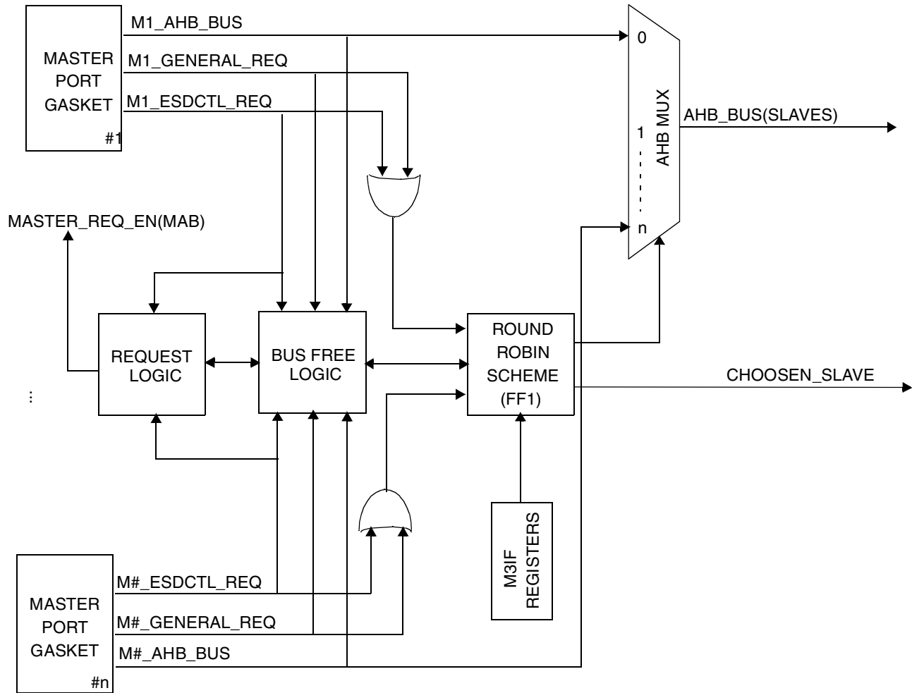
Figure 16-21. M3A Block Diagram
