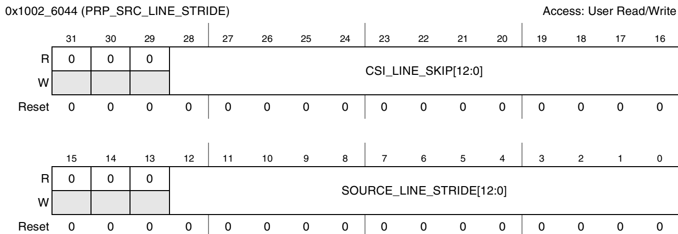
Figure 41-45. PrP Source Line Stride Register
