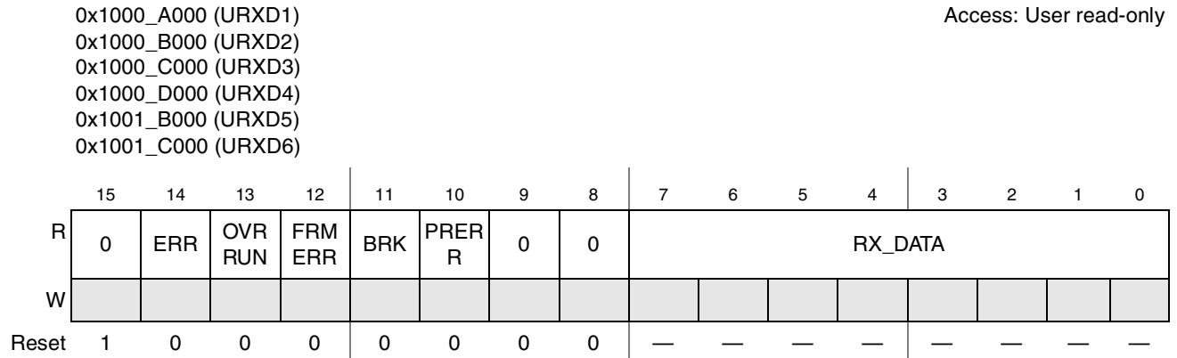
Figure 28-4. UART Receiver Register (URXD)
