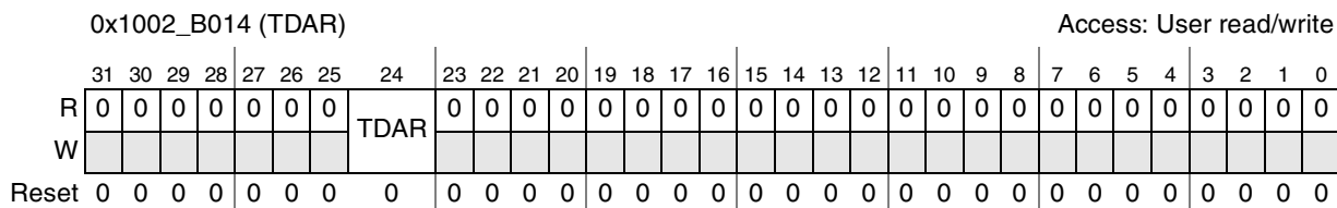
Figure 29-7. TDAR Register
