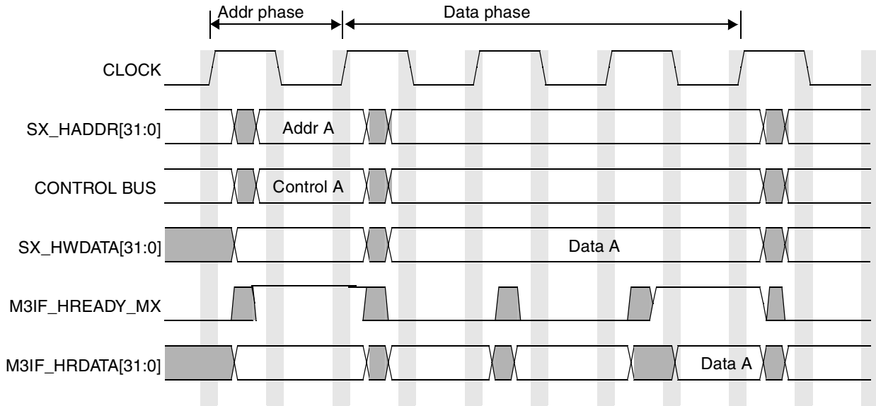
Figure 16-12. MPG with Wait States
