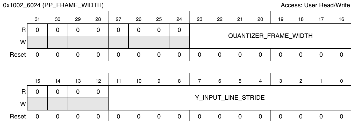
Figure 41-16. PP Source Frame Width Register
