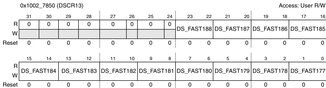
Figure 4-18. Drive Strength Control Register 13 (DSCR13)
