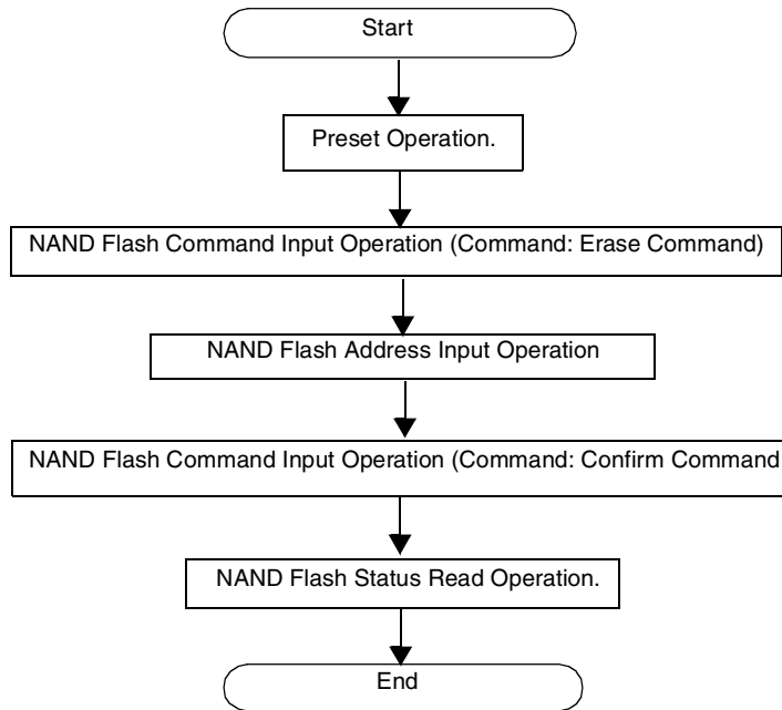
Figure 19-36. Flowchart of Erase NAND Flash Operation
