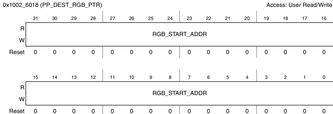
Figure 41-13. PP Destination RGB Frame Start Address Register
