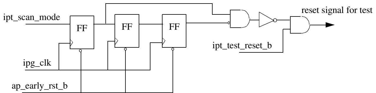
Figure 14-36. Scan Out Protection Circuit
