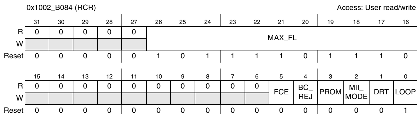
Figure 29-12. RCR Register
