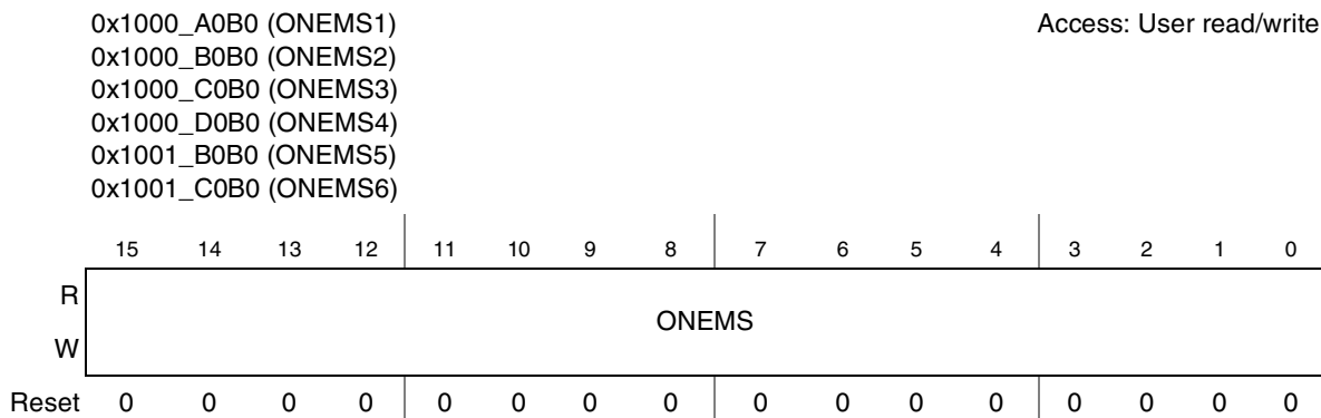
Figure 28-18. UART One Millisecond Register Summary (ONEMS)
