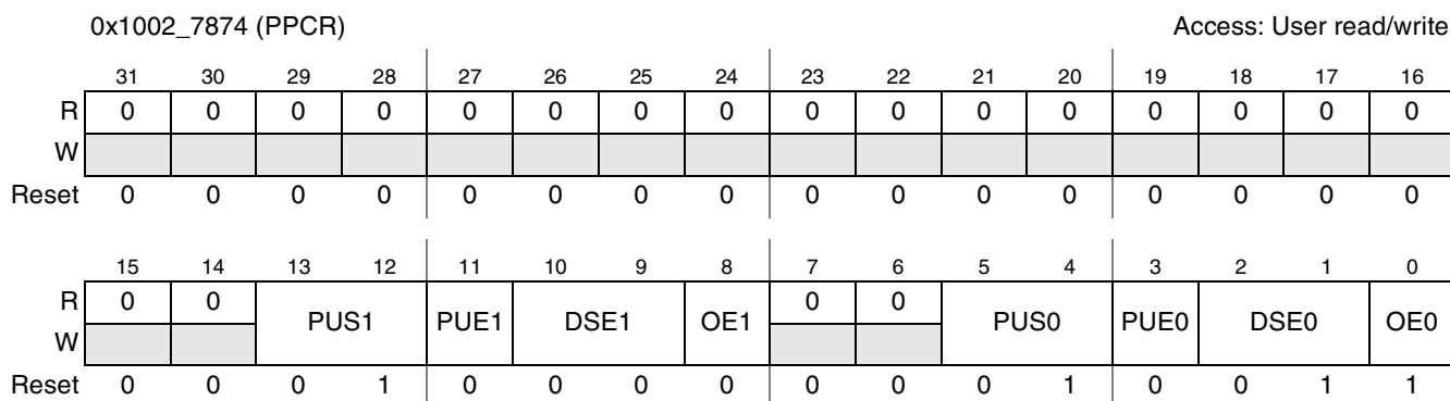
Figure 4-26. PMIC Pad Control Register (PPCR)
