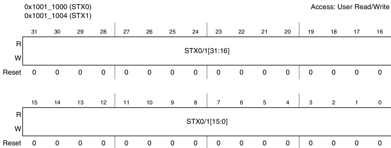
Figure 42-15. SSI Transmit Data Registers
