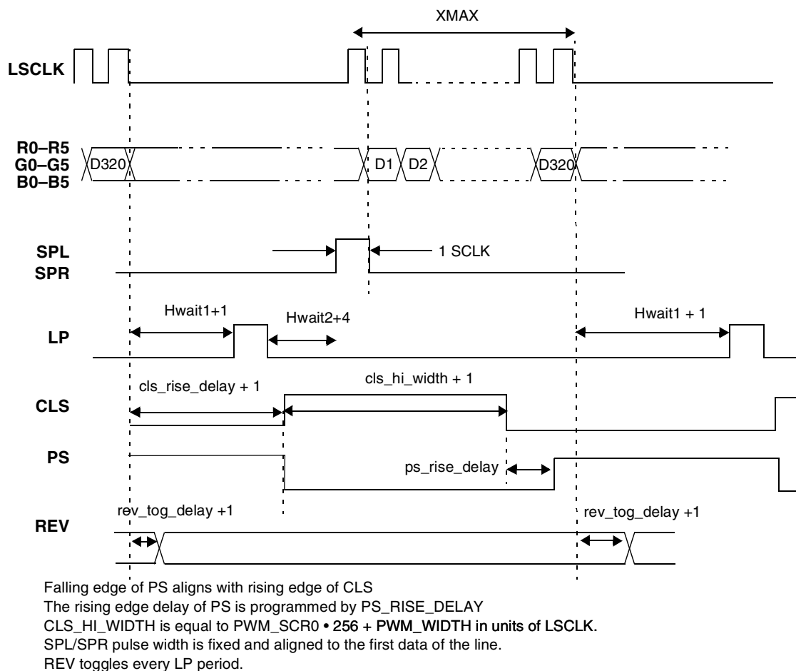
Figure 43-34. Horizontal Timing in Device_Number
