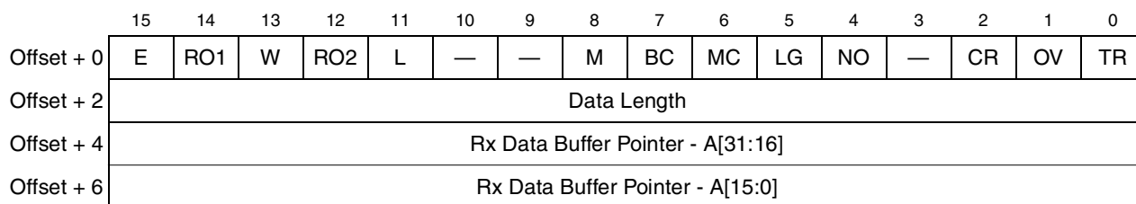
Figure 29-27. Receive Buffer Descriptor (RxBD)
