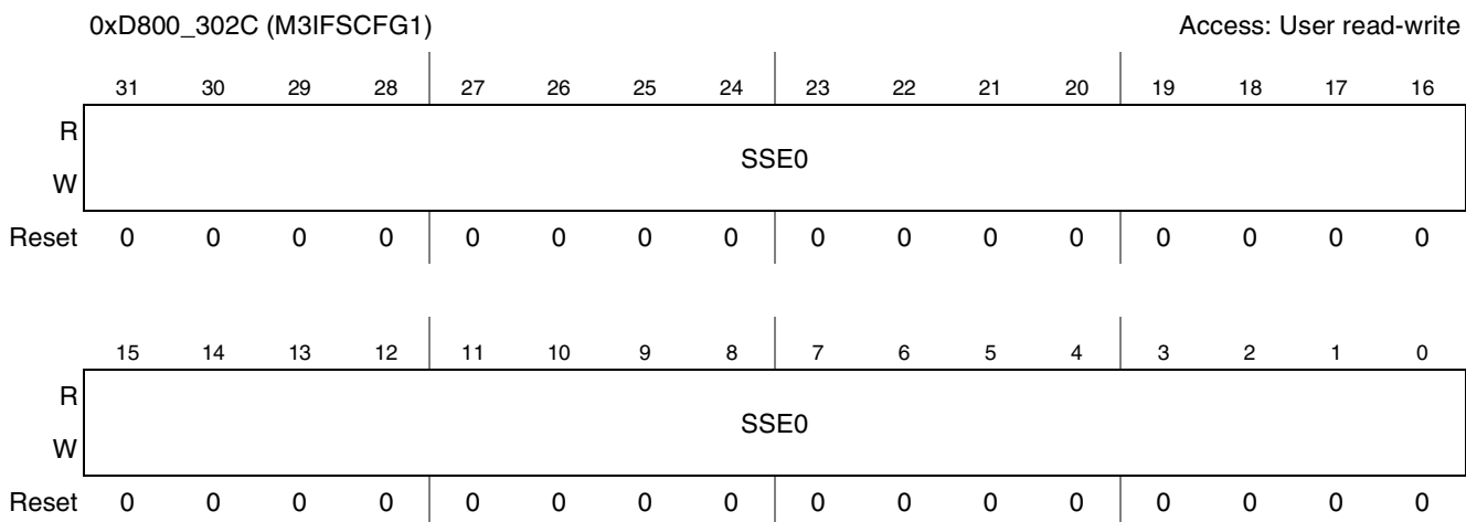
Figure 16-5. M3IF Snooping Configuration Register 1 (M3IFSCFG1)
