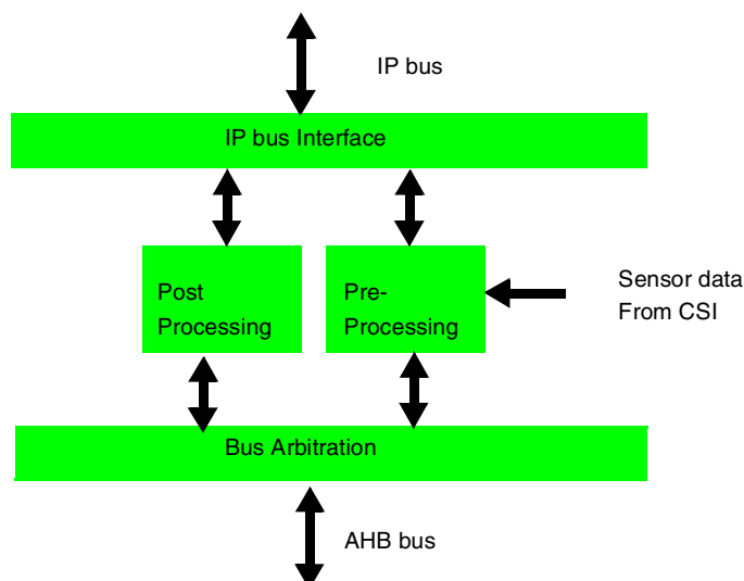
Figure 1-4. eMMA_It Architecture
