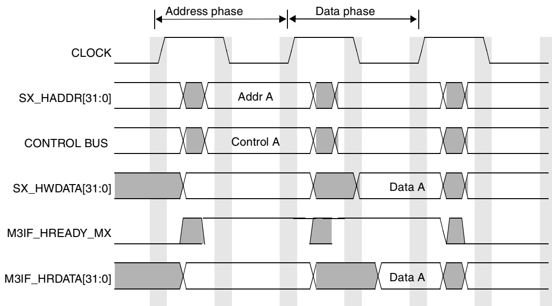
Figure 16-11. MPG Simple Transfer
