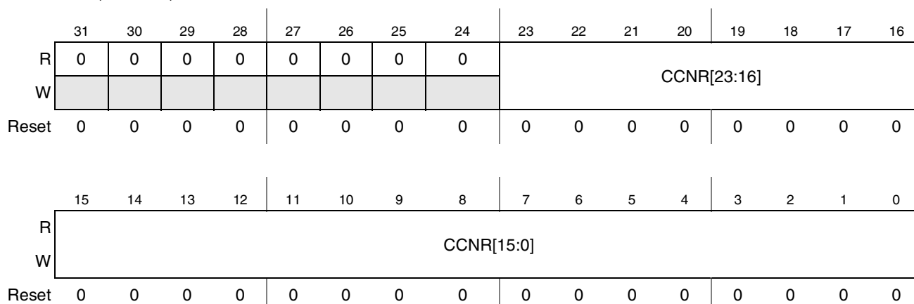
Figure 37-26. Channel Counter Register (CCNR0–CCNR15)
