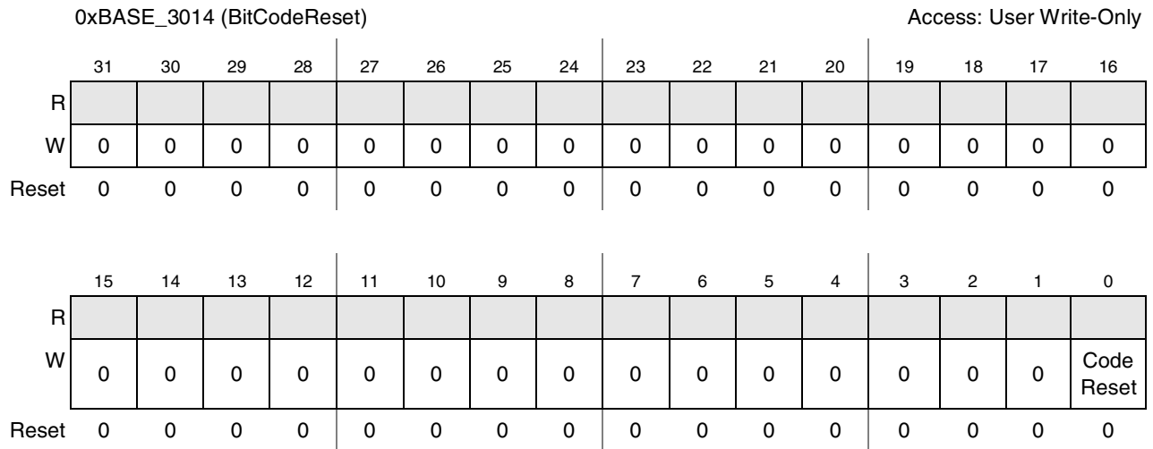
Figure 40-8. Video Codec BIT Code Reset Register
