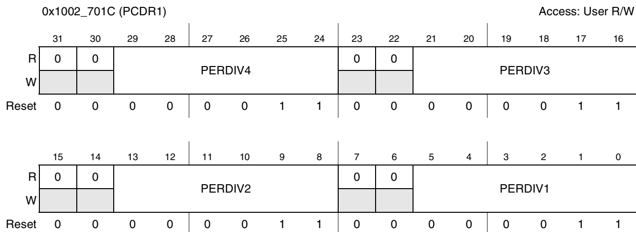
Figure 3-11. Peripheral Clock Divider Register 1(PCDR1)
