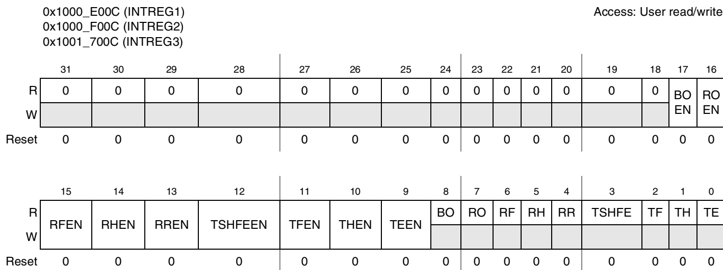
Figure 23-18. Interrupt Control Register Diagram
