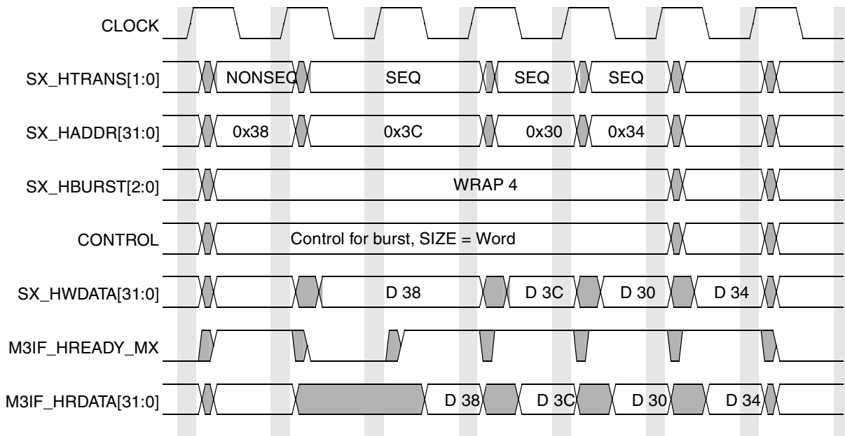
Figure 16-15. MPG Four Beat Wrapping Burst
