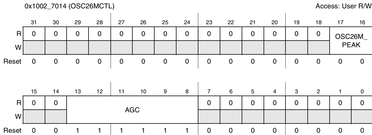
Figure 3-9. Oscillator 26M Control Register (OSC26MCTL)
