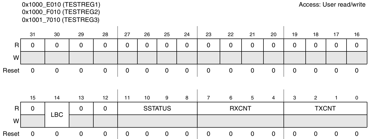
Figure 23-19. Test Control Register Diagram
