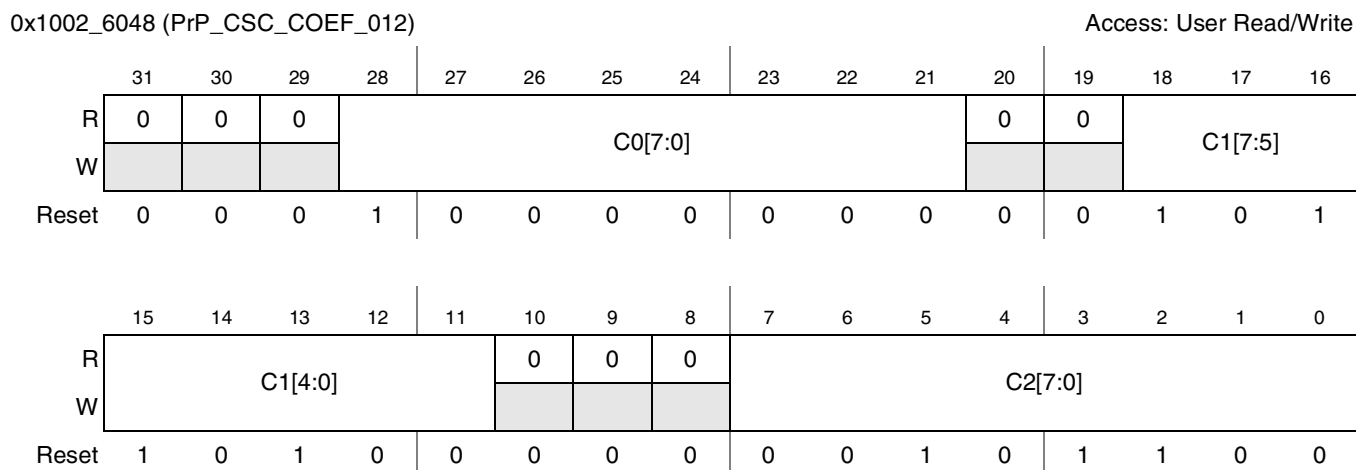
Figure 41-46. PrP CSC Coefficient 012
