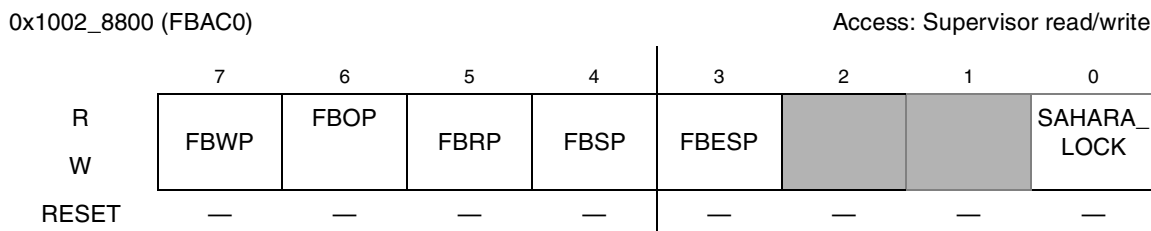
Figure 14-18. Fuse Bank 0 Access Protection Register
