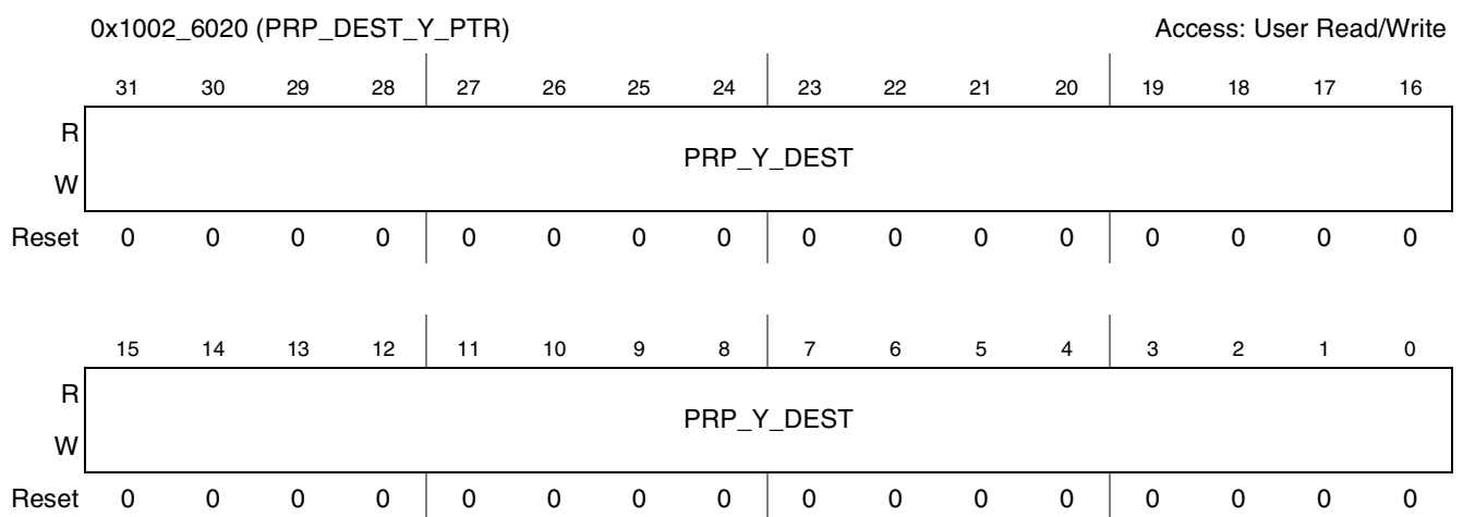
Figure 41-36. PrP Destination Y Address Register
