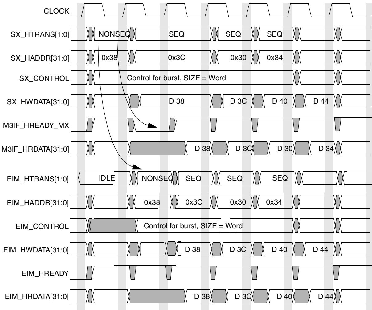
Figure 16-22. M3A Simple Transfer Timing Diagram
