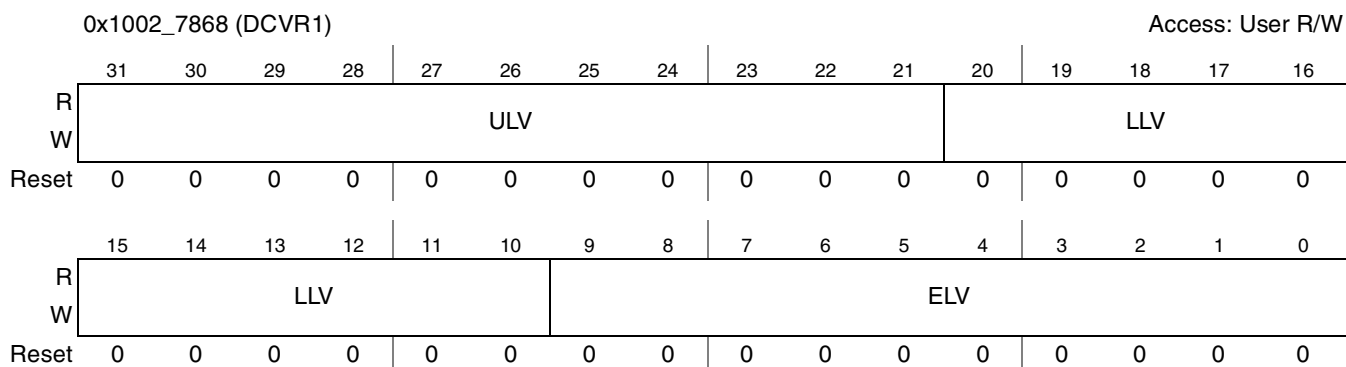
Figure 4-23. DPTC Comparator Value Register 1 (DCVR1)
