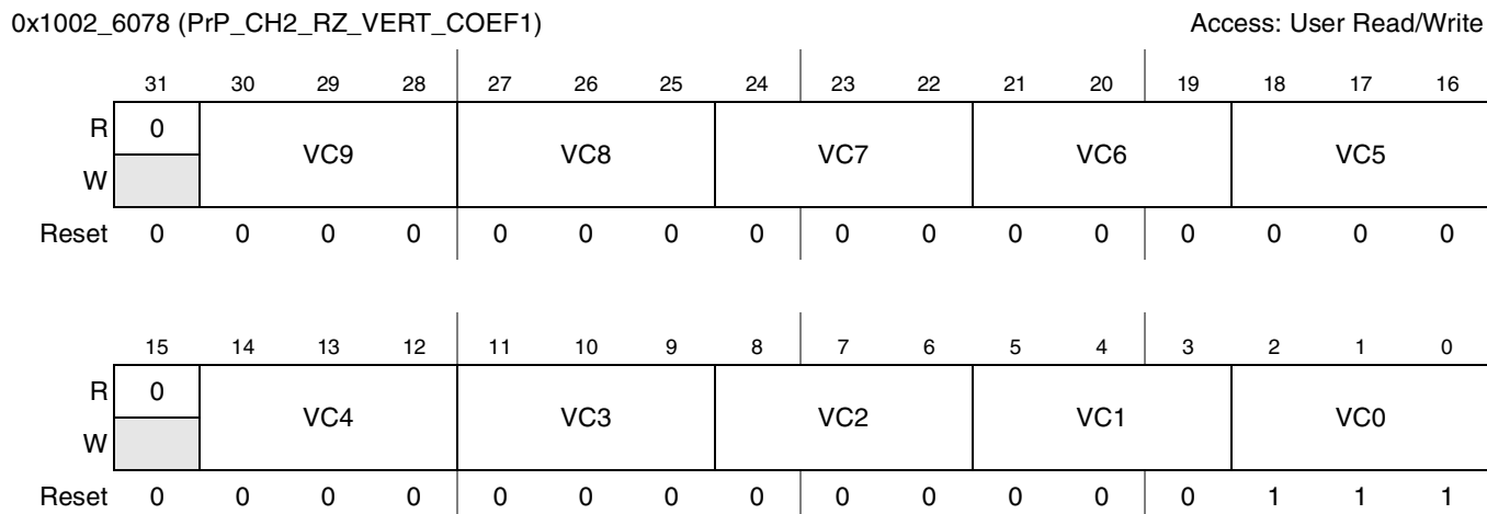
Figure 41-58. PrP Channel2 Vertical Resize Coefficient 1
