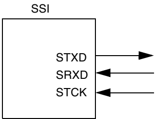
SSI External Gated Clock (RXDIR=1, TXDIR=0, SYN=1)
