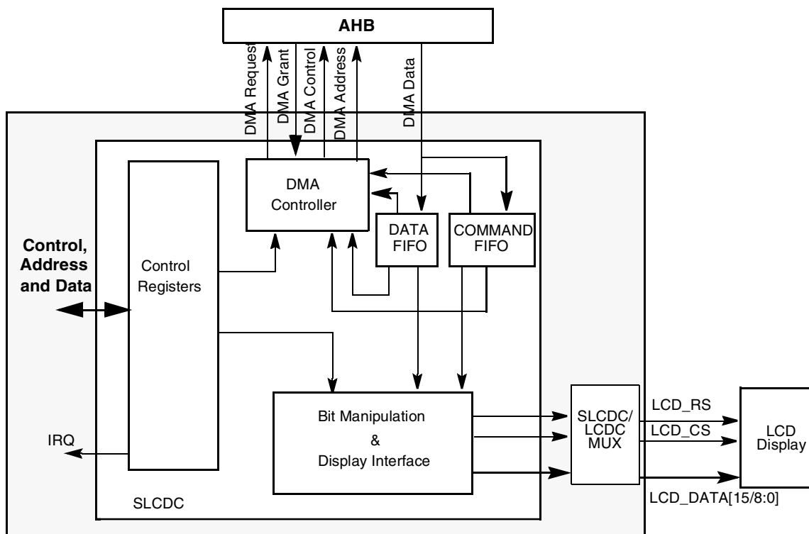
Figure 44-1. SLCDC System Diagram
