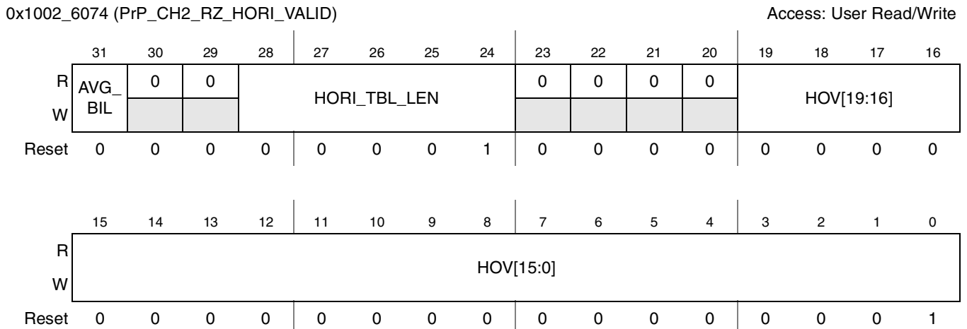
Figure 41-57. PrP Channel-2 Resize Horizontal Valid
