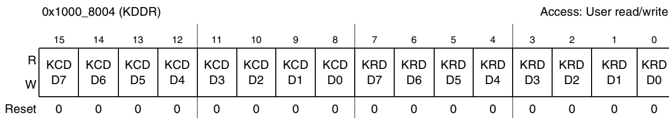
Figure 25-5. KDDR Register
