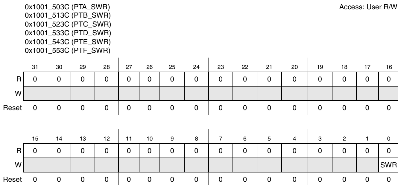
Figure 6-25. Software Reset Register (SWR)
