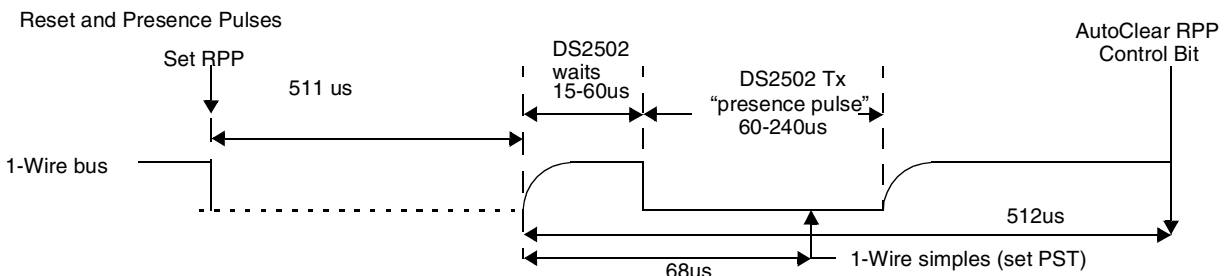
Figure 21-3. 1-Wire Initialization
