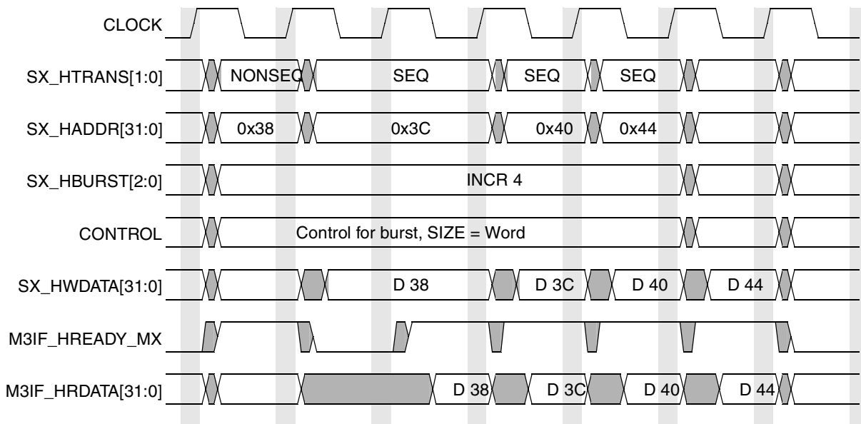
Figure 16-16. MPG Four Beat Incrementing Burst
