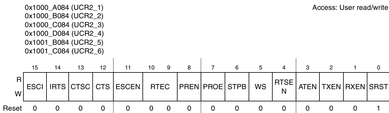
Figure 28-7. UART Control Register 2 (UCR2) Summary
