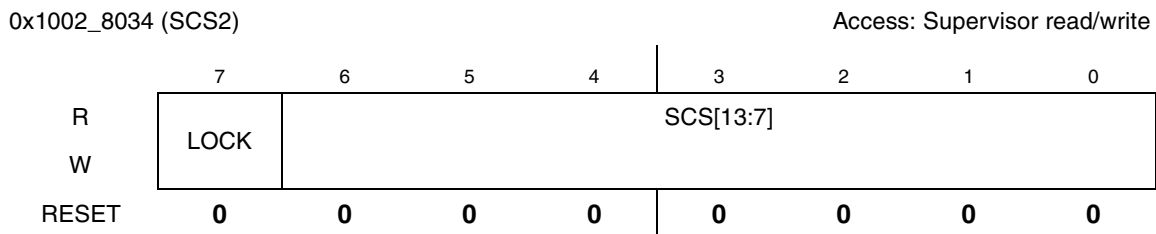
Figure 14-16. Software Controllable Signals Register 2
