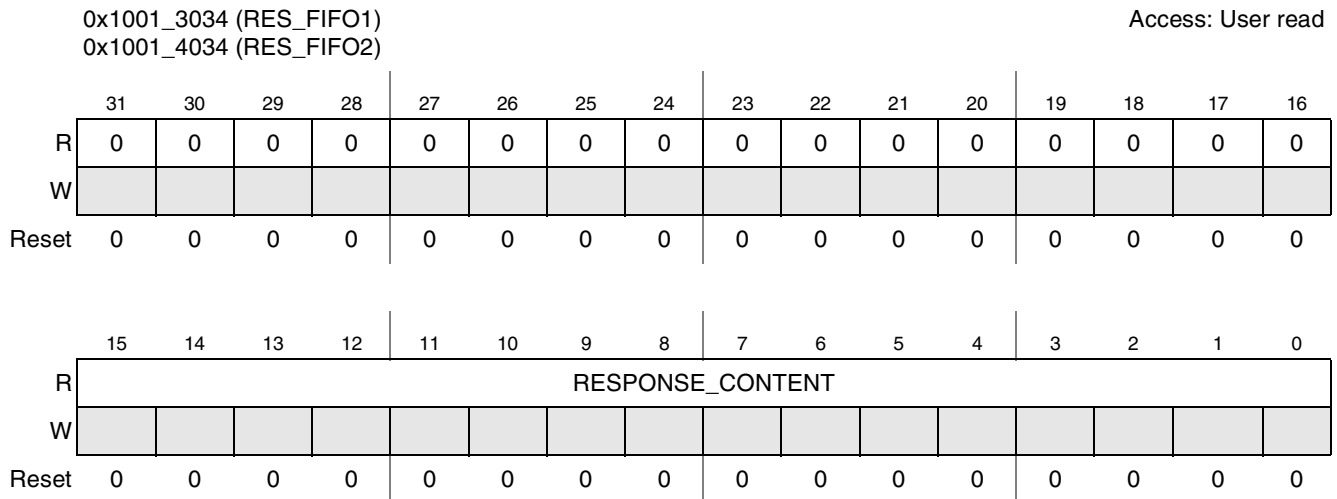
Figure 27-16. SDHC Response FIFO Register
