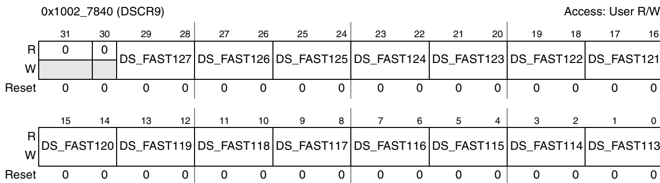
Figure 4-14. Drive Strength Control Register 9 (DSCR9)
