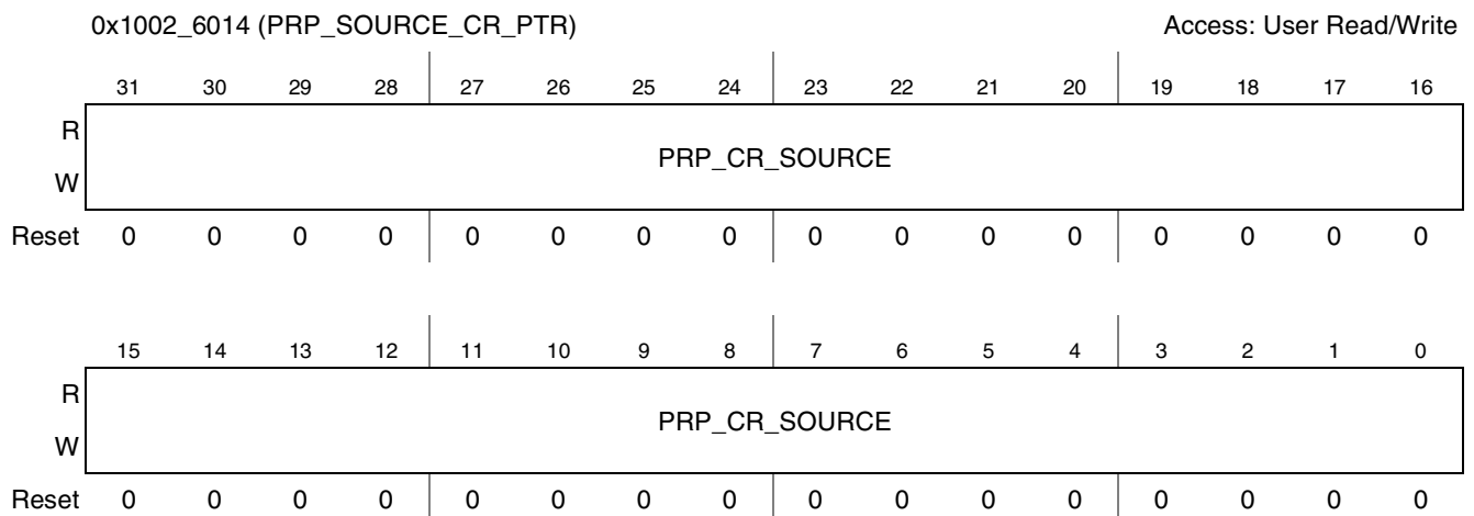
Figure 41-33. PrP Source Cr Address Register
