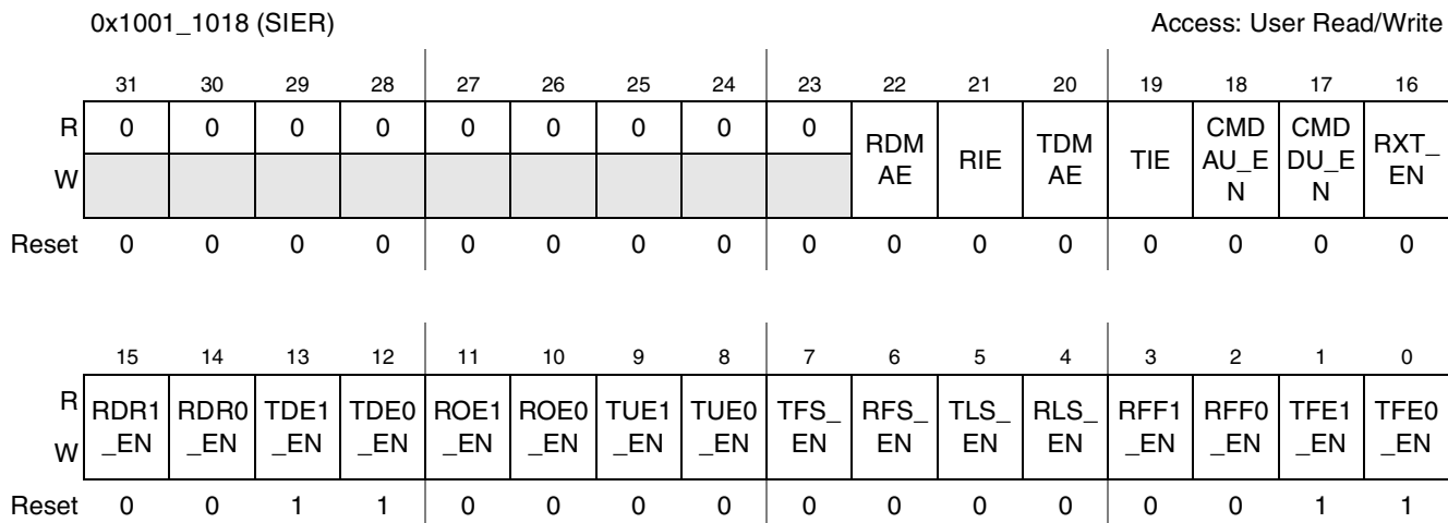
Figure 42-28. SSI Interrupt Enable Register
