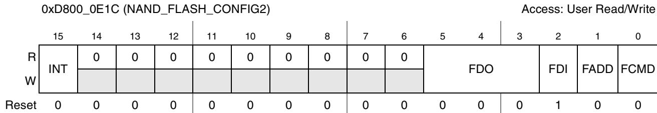
Figure 19-19. NAND_FLASH_CONFIG2 Register
