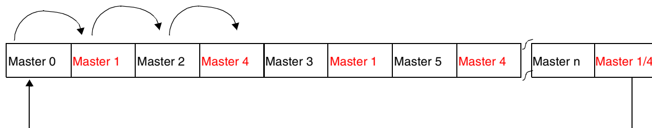
Figure 16-24. M3A—Round Robin Token Chain—Masters 1 and 4 has 50% Priority
