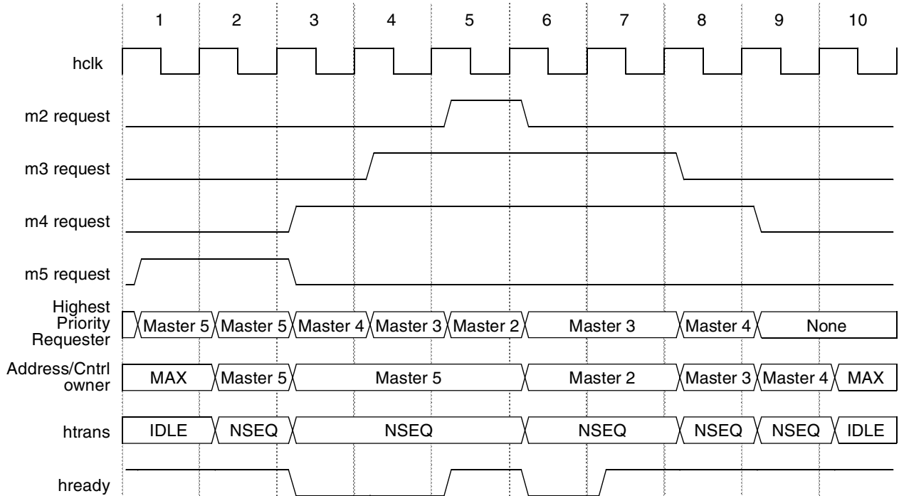
Figure 36-8. Low to High Priority Mastership Change
