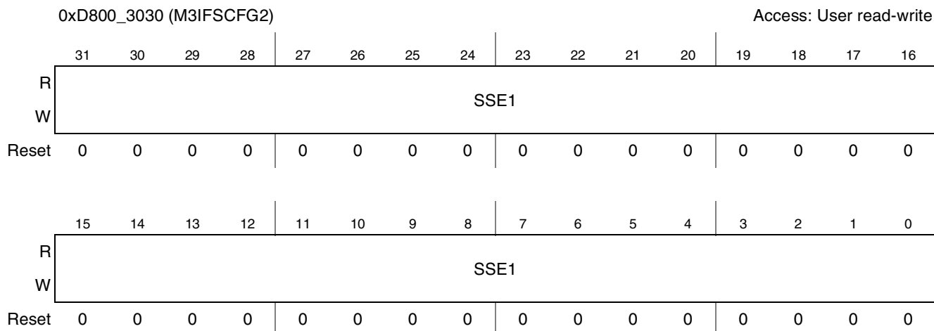
Figure 16-6. M3IF Snooping Configuration Register 2 (M3IFSCFG2)
