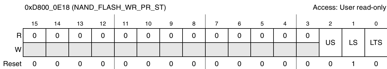
Figure 19-17. NAND_FLASH_WR_PR_ST Register
