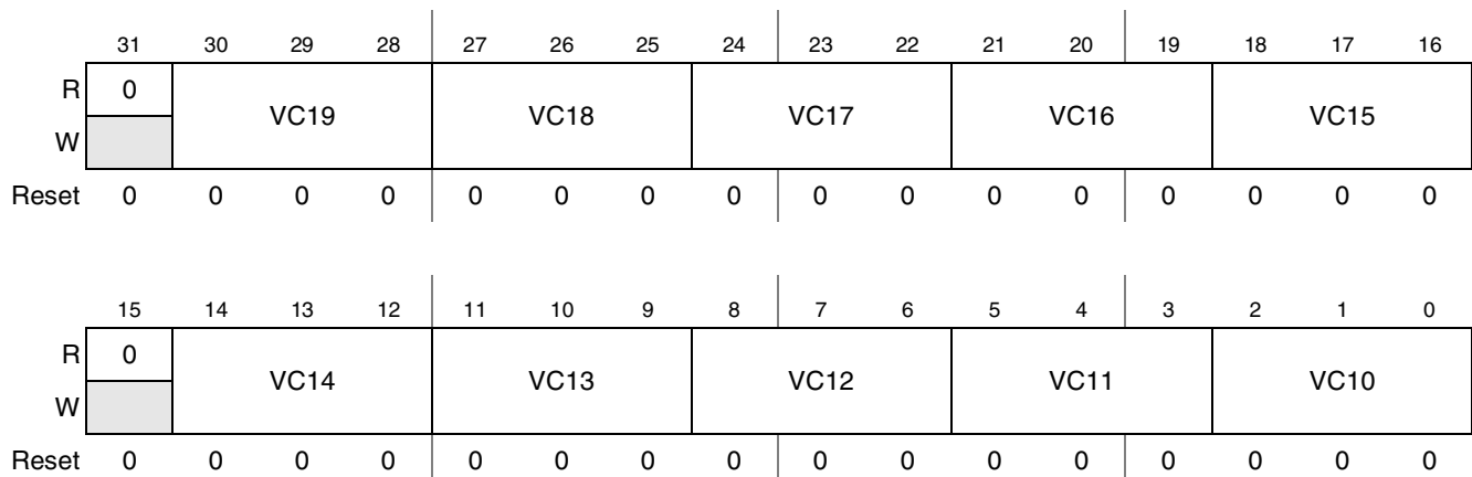
Figure 41-59. PrP Channel-2 Vertical Resize Coefficient 2
