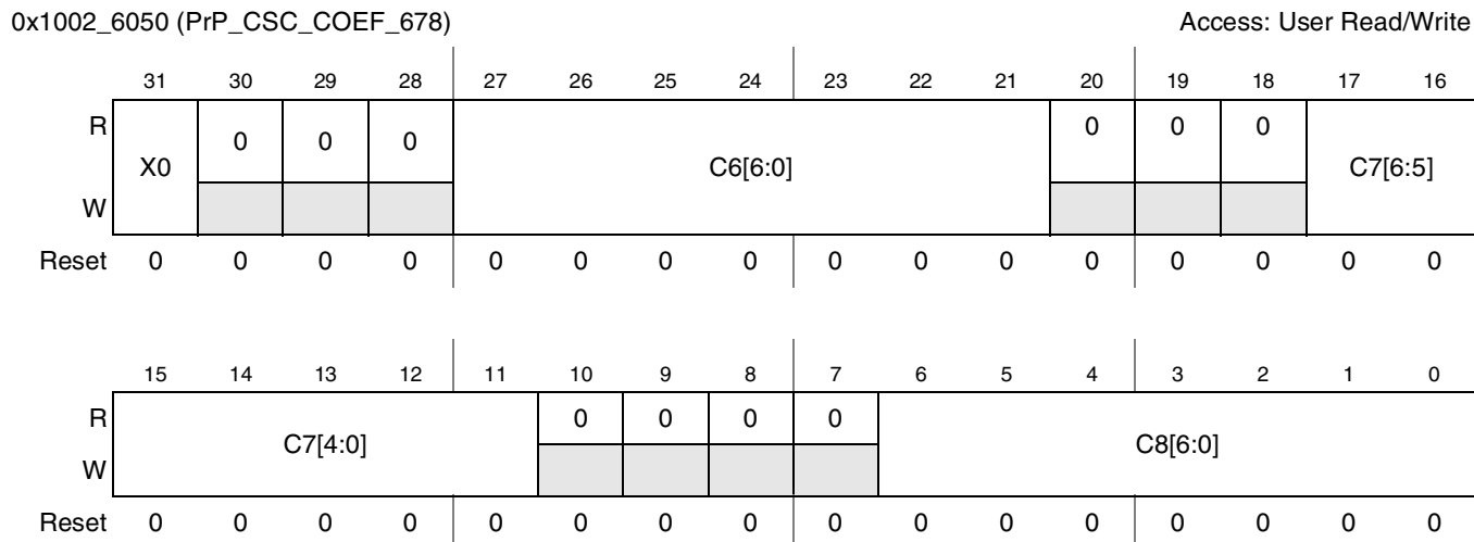
Figure 41-48. PrP CSC Coefficient 678
