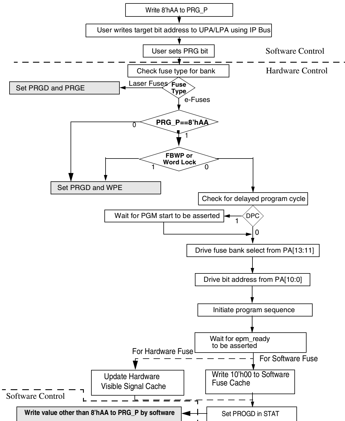
Figure 14-40. e-Fuse Program Sequence
