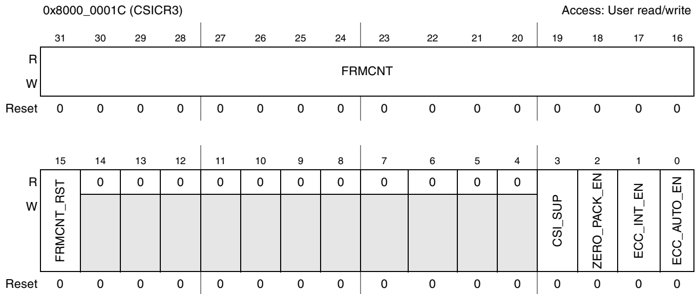
Figure 39-11. CSI Control Register 3 (CSICR3)
