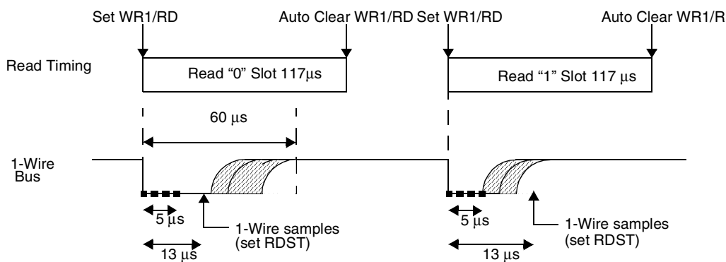
Figure 21-6. Read Timing
