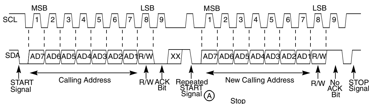
Figure 24-12. Repeated START
