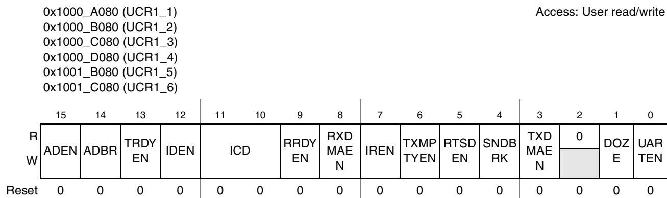
Figure 28-6. UART Control Register 1 (UCR1)
