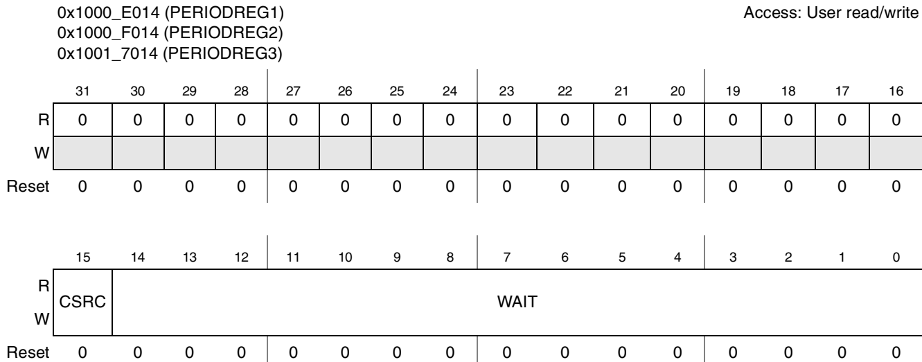
Figure 23-20. Sample Period Control Register Diagram
