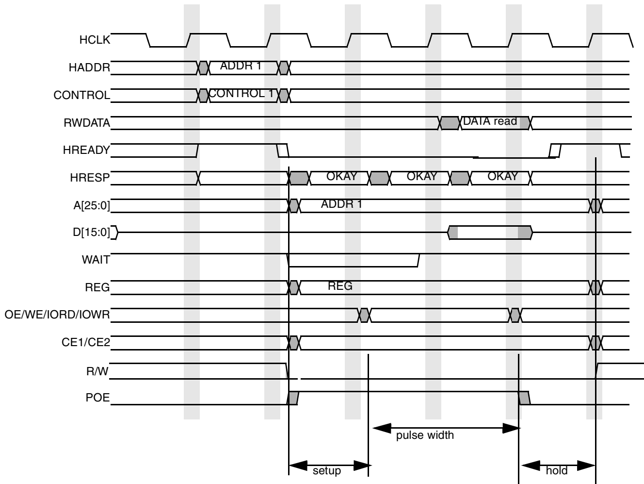
Figure 20-12. Read Cycle PSHT=1, PSST =1
