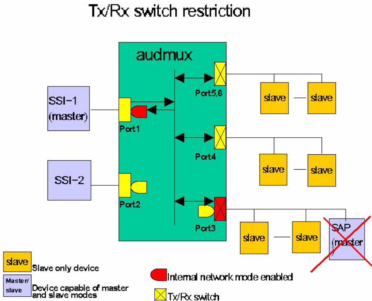
Figure 38-15. Tx-Rx Switch Restriction
