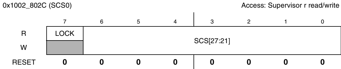
Figure 14-14. Software Controllable Signals Register 0
