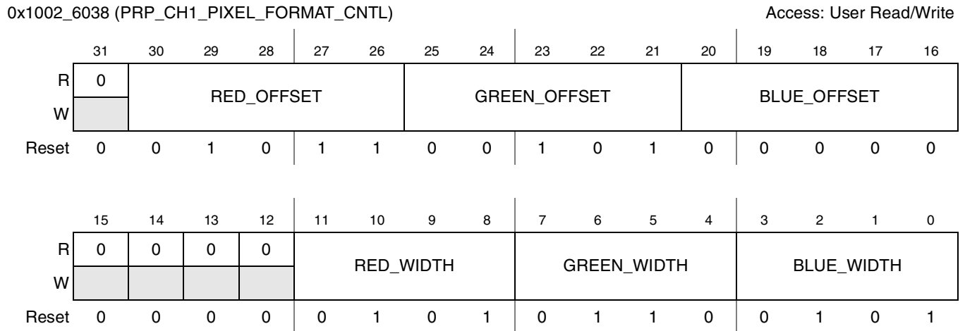
Figure 41-42. PrP CH1 Pixel Format Control Register
