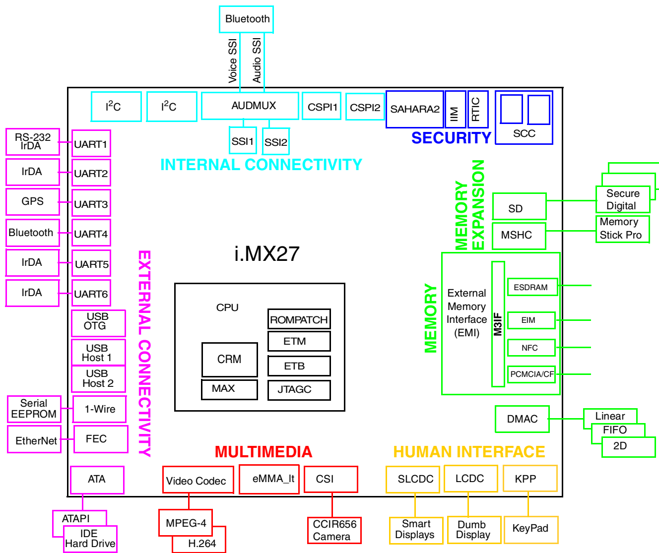
Figure 1-2. i.MX27 Connectivity Example
