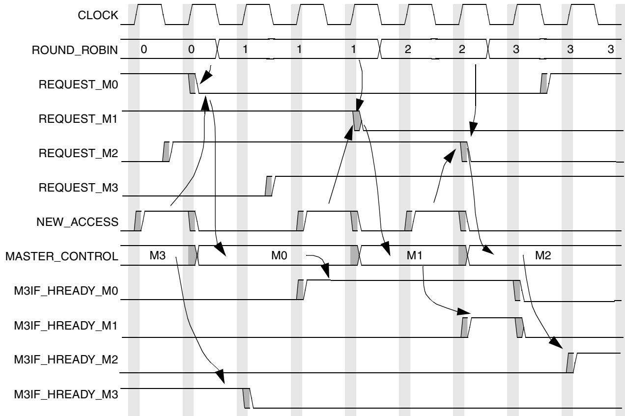
Figure 16-26. MAB Arbitration Process Timing Diagram
