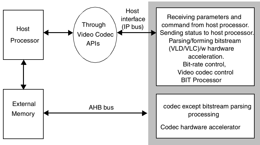
Figure 40-11. Video Codec Interface with Application Software Diagram
