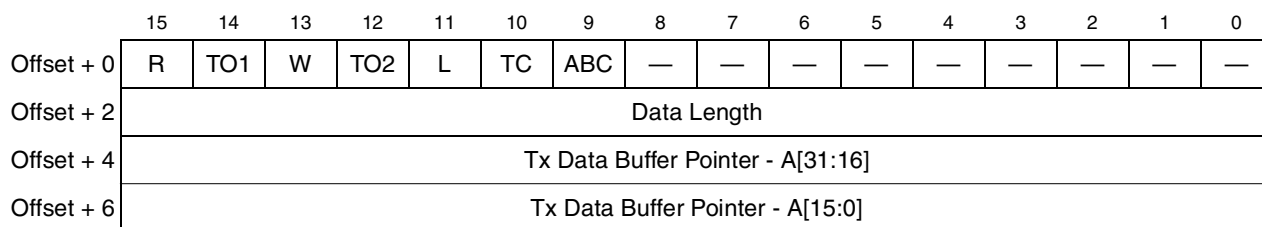
Figure 29-28. Transmit Buffer Descriptor (TxBD)
