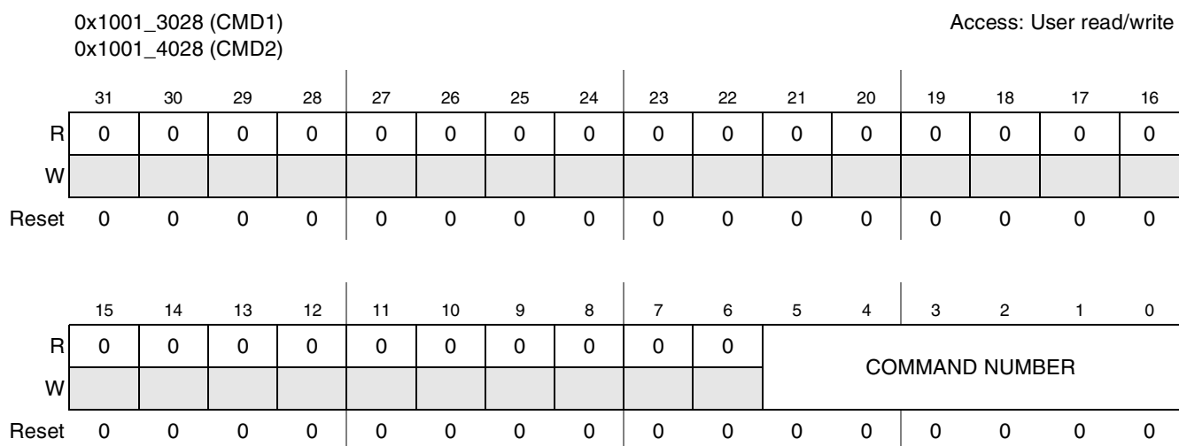
Figure 27-14. SDHC Command Number Register
