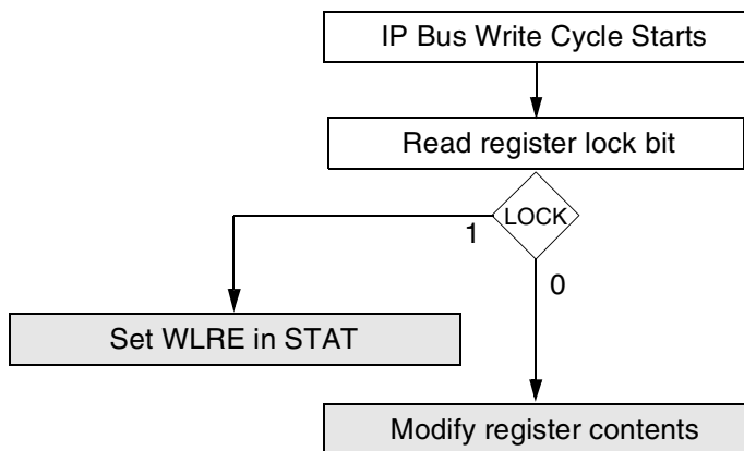
Figure 14-30. SCS Register Write Sequence
