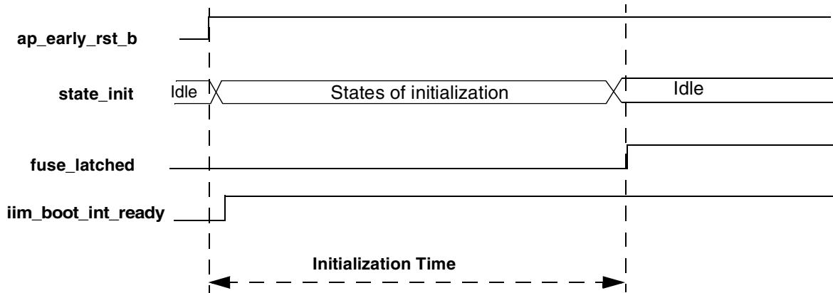
Figure 14-42. Timing Diagram of Initialization
