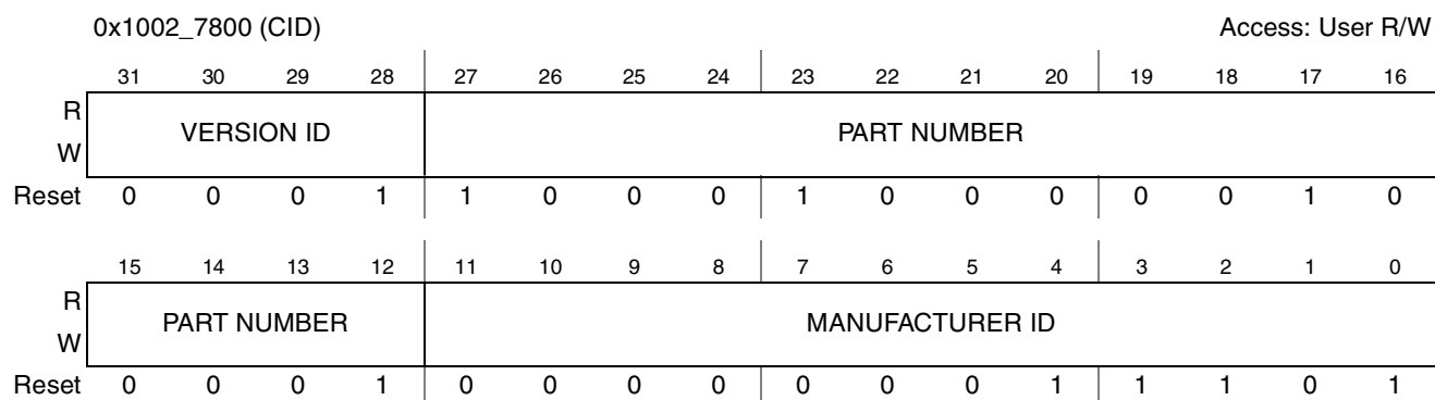
Figure 4-2. Chip ID Register (CID)
