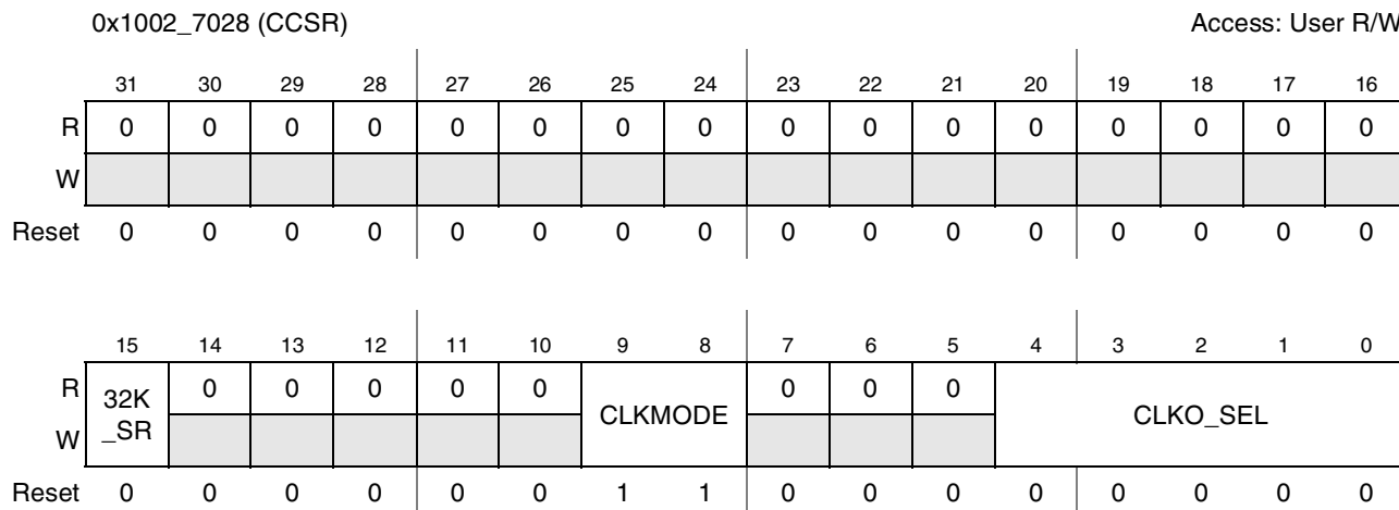
Figure 3-14. Clock Control Status Register (CCSR)
