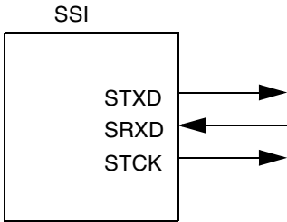
SSI Internal Gated Clock (RXDIR=1, TXDIR=1, SYN=1)
