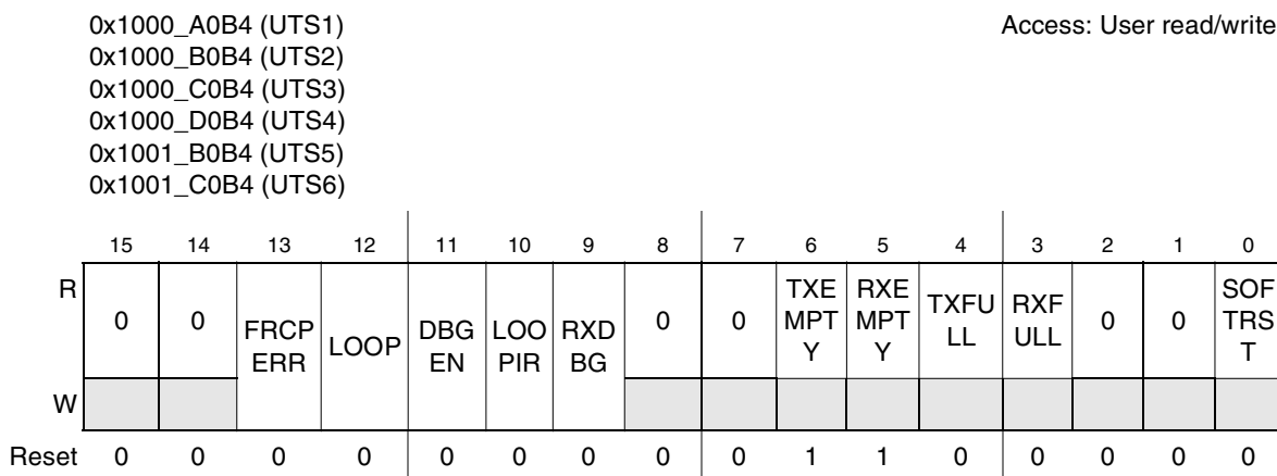
Figure 28-19. UART Test Register Summary (UTS)
