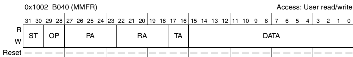
Figure 29-9. MMFR Register
