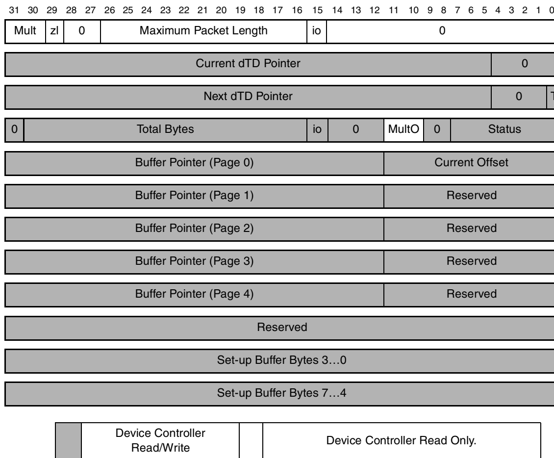
Figure 30-74. Endpoint Queue Head (dQH)
