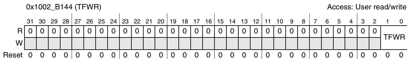
Figure 29-21. TFWR Register
