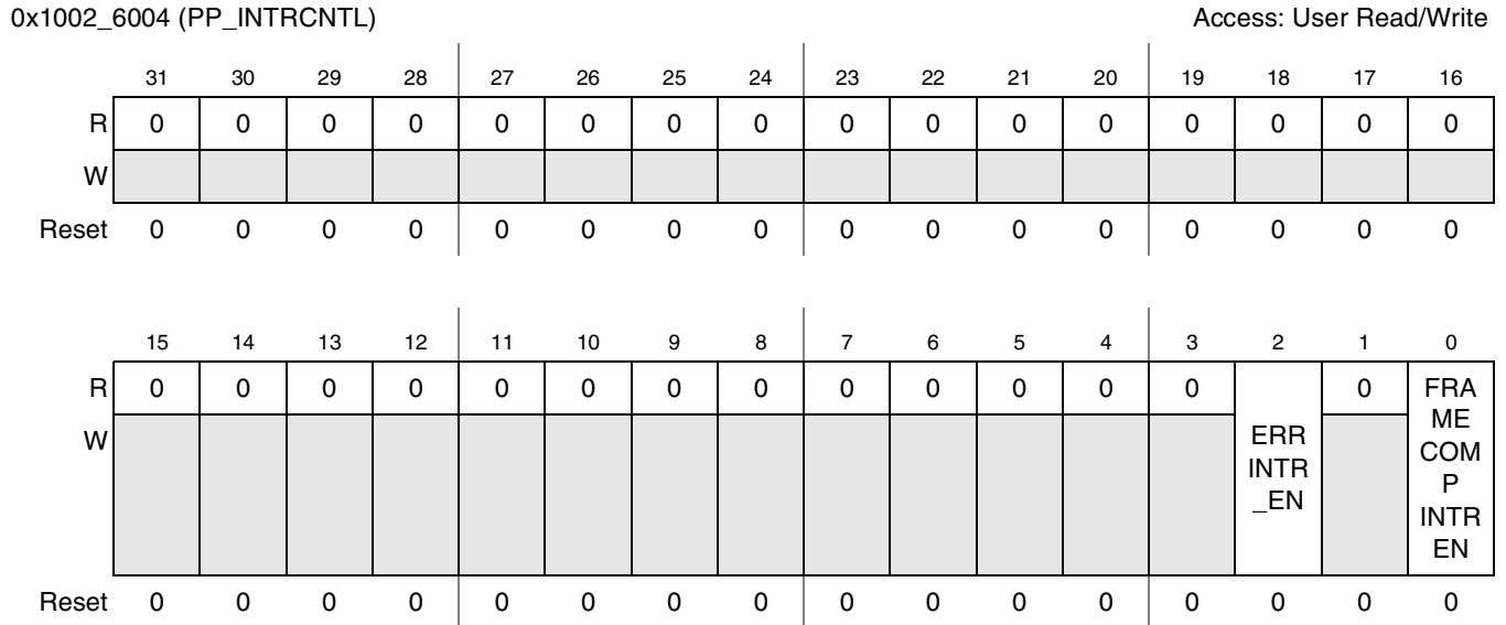
Figure 41-8. PP Interrupt Control Register
