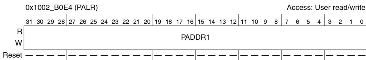
Figure 29-14. PALR Register
