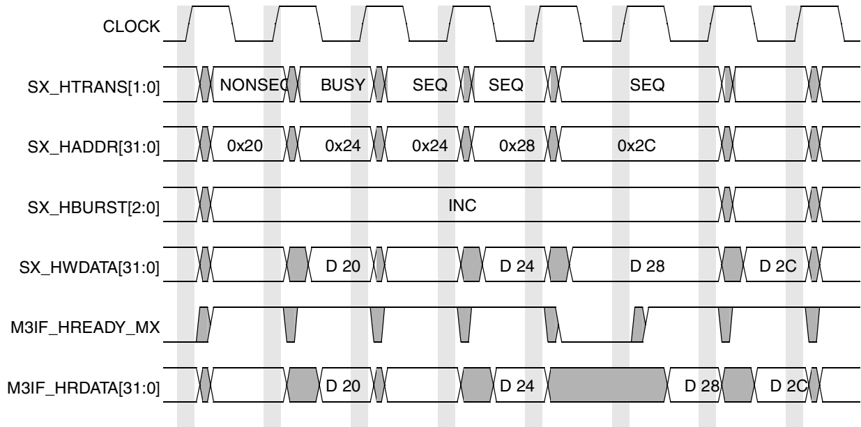
Figure 16-14. MPG—Transfer Type Examples
