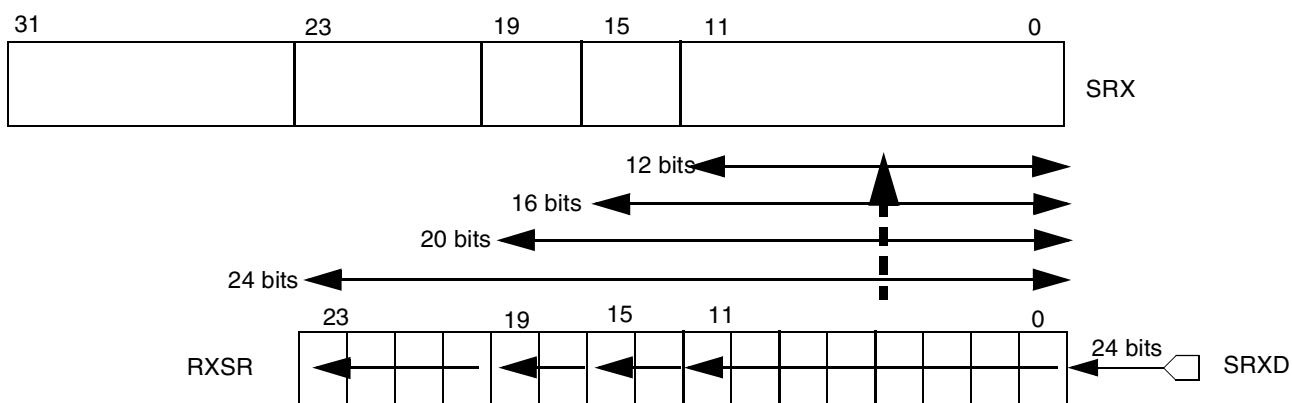
Figure 42-23. Receive Data Path (RXBIT0=1, RSHFD=0) (LSB Alignment)
