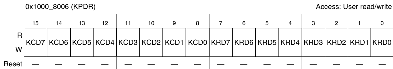
Figure 25-6. KPDR Register
