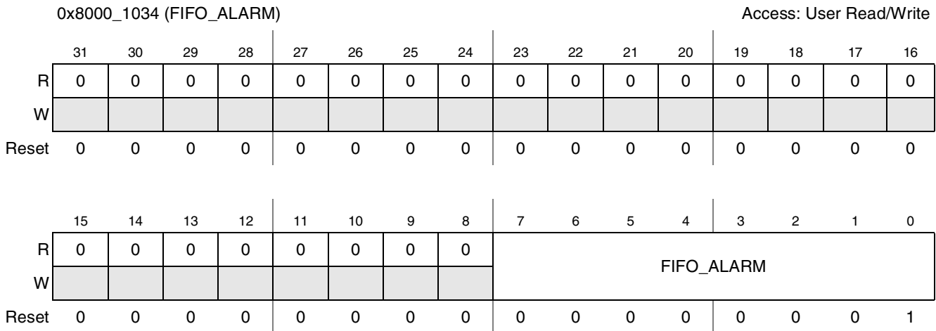
Figure 22-16. ATA FIFO_ALARM Register
