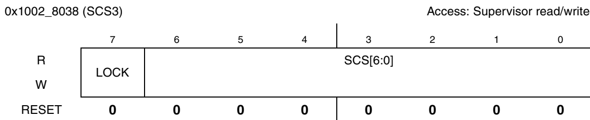
Figure 14-17. Software Controllable Signals Register 3
