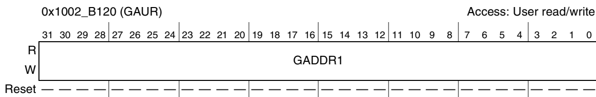
Figure 29-19. GAUR Register
