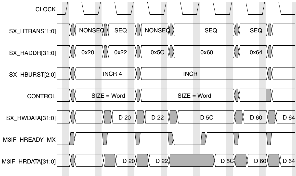
Figure 16-17. MPG Undefined Length Bursts
