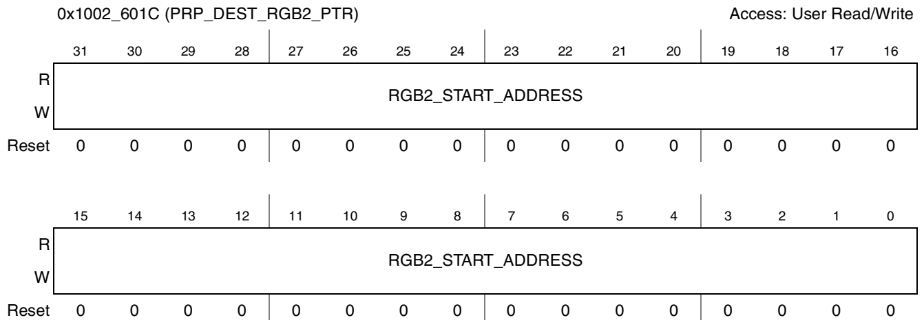
Figure 41-35. PrP Destination RGB2 Start Address Register
