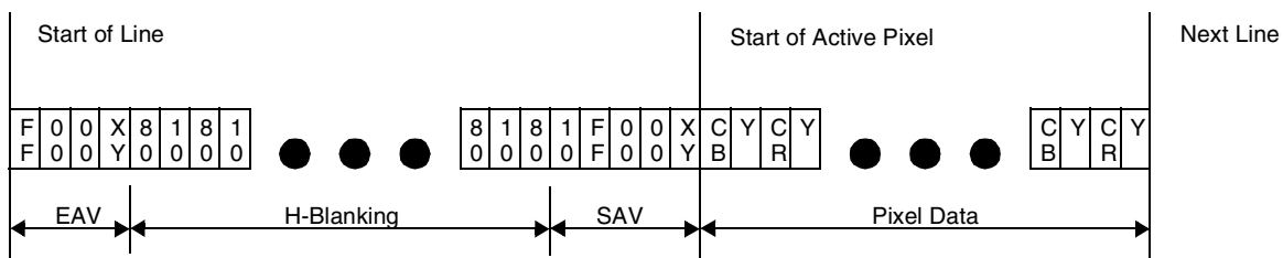
Figure 39-4. CCIR656 General Line Timing
