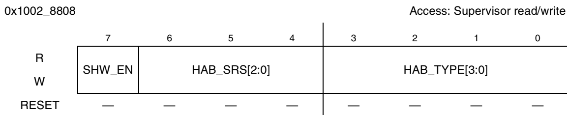
Figure 14-20. Word2 of Fusebank0
