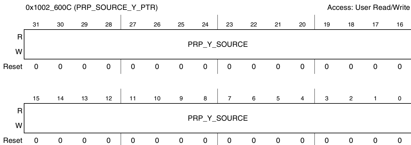
Figure 41-31. PrP Source Y Address Register
