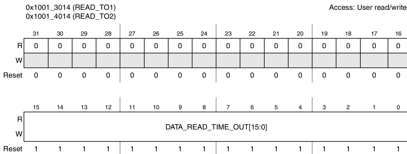
Figure 27-9. SDHC Read Time Out Register
