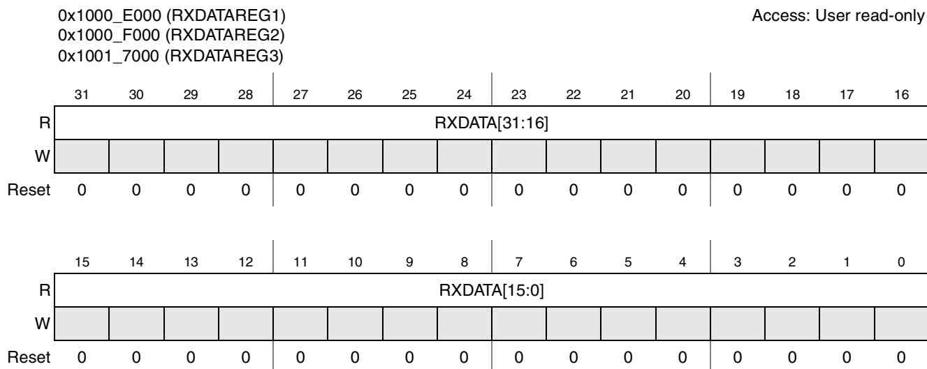
Figure 23-15. RXDATA Register Diagram
