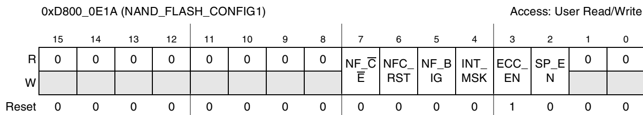
Figure 19-18. NAND_FLASH_CONFIG1 Register
