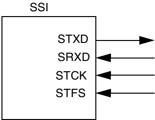
SSI External Continuous Clock (RXDIR=0, TXDIR=0, RFDIR=X, TFDIR=0, SYN=1) SSI I2S Slave Mode (I2S_Mode=10)
