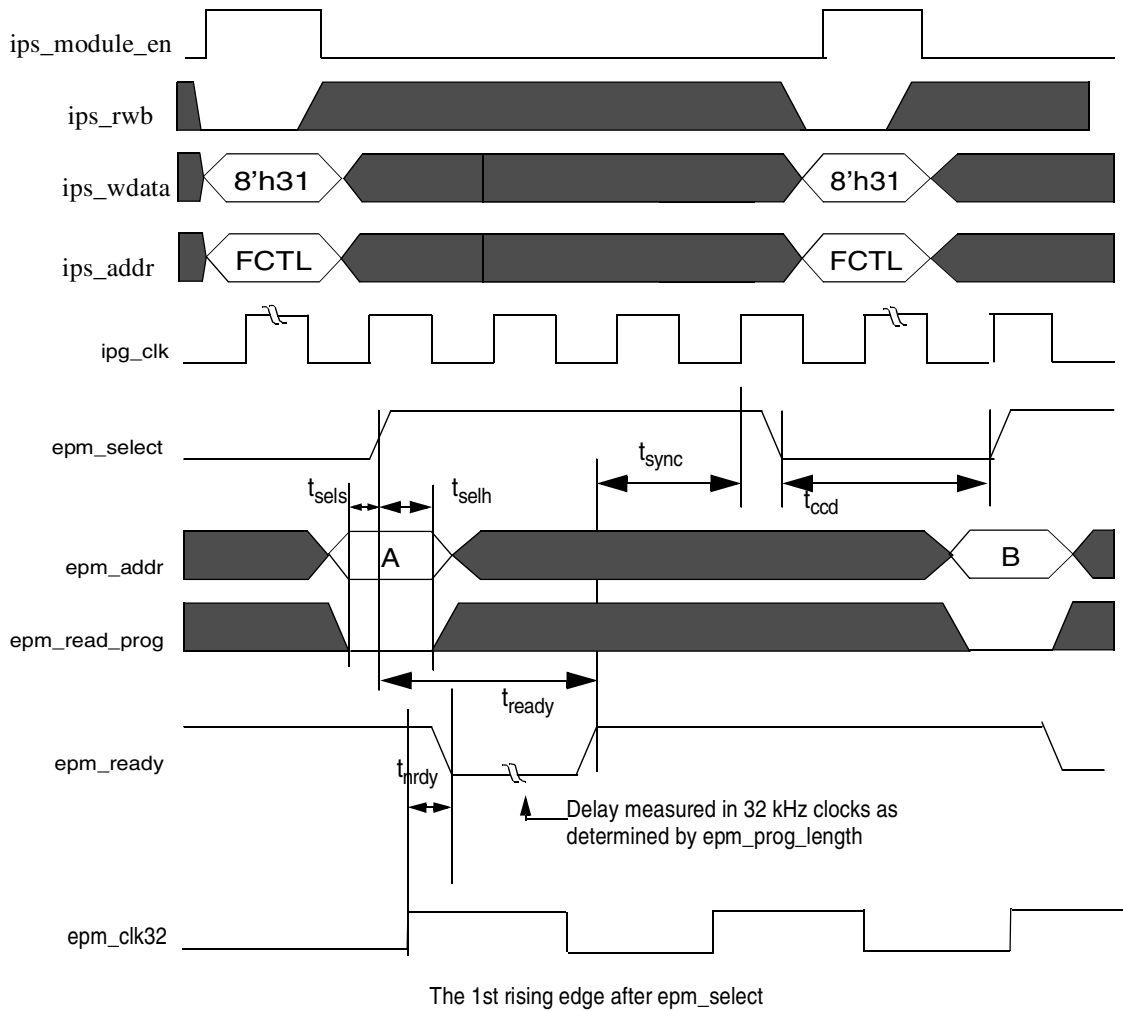
Figure 14-33. Fuse Program Cycle Timing
