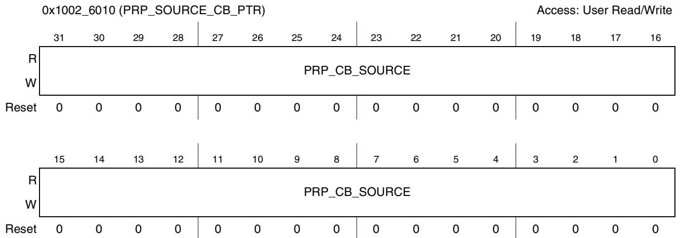
Figure 41-32. PrP Source Cb Address Register
