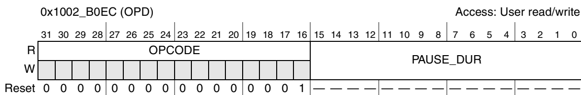
Figure 29-16. OPD Register
