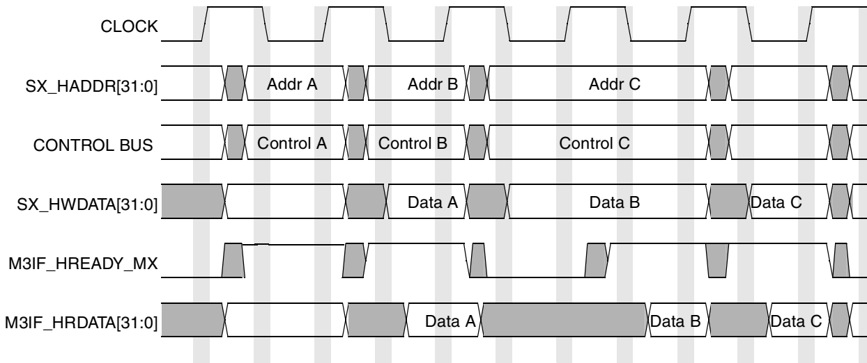
Figure 16-13. MPG Multiple Transfers
