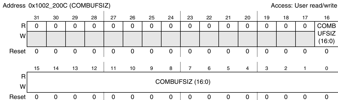
Figure 44-15. Command Buffer Size Register
