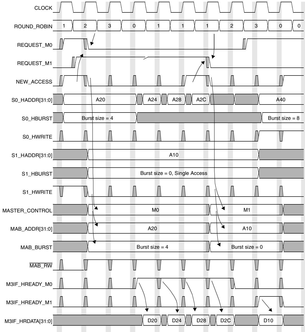
Figure 16-27. MAB Multi-Master Request Time Diagram
