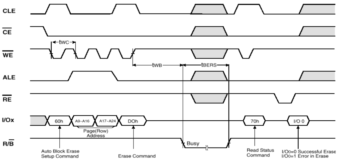
Figure 19-23. Erase Operation
