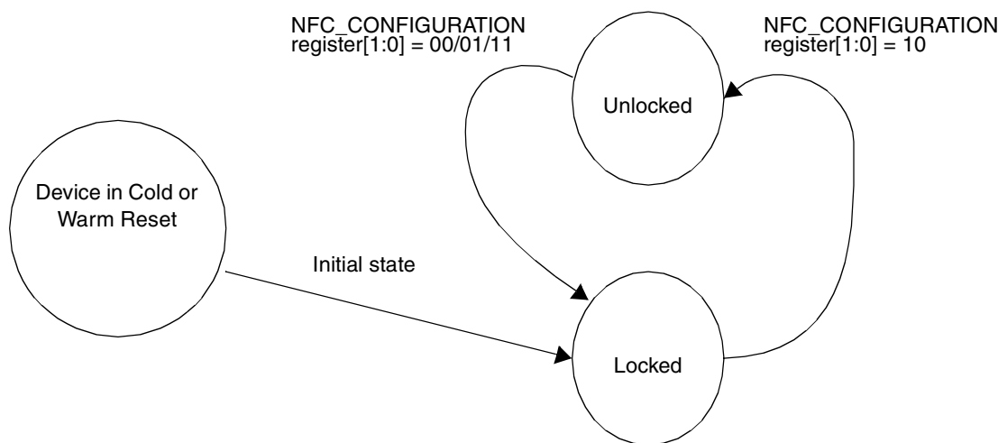
Figure 19-38. State Diagram of RAM Buffer Write Protection
