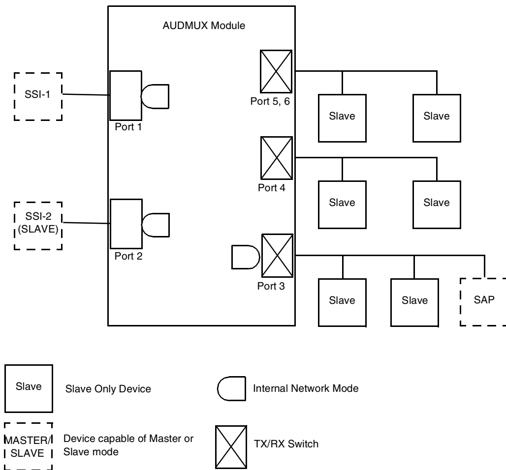
Figure 38-13. Configuration Overview
