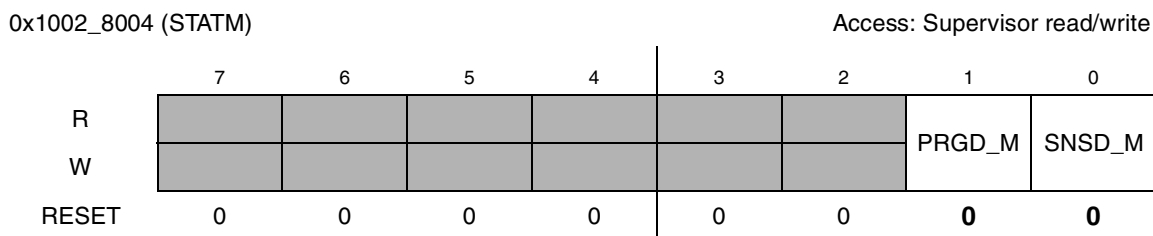
Figure 14-4. Status IRQ Mask Register
