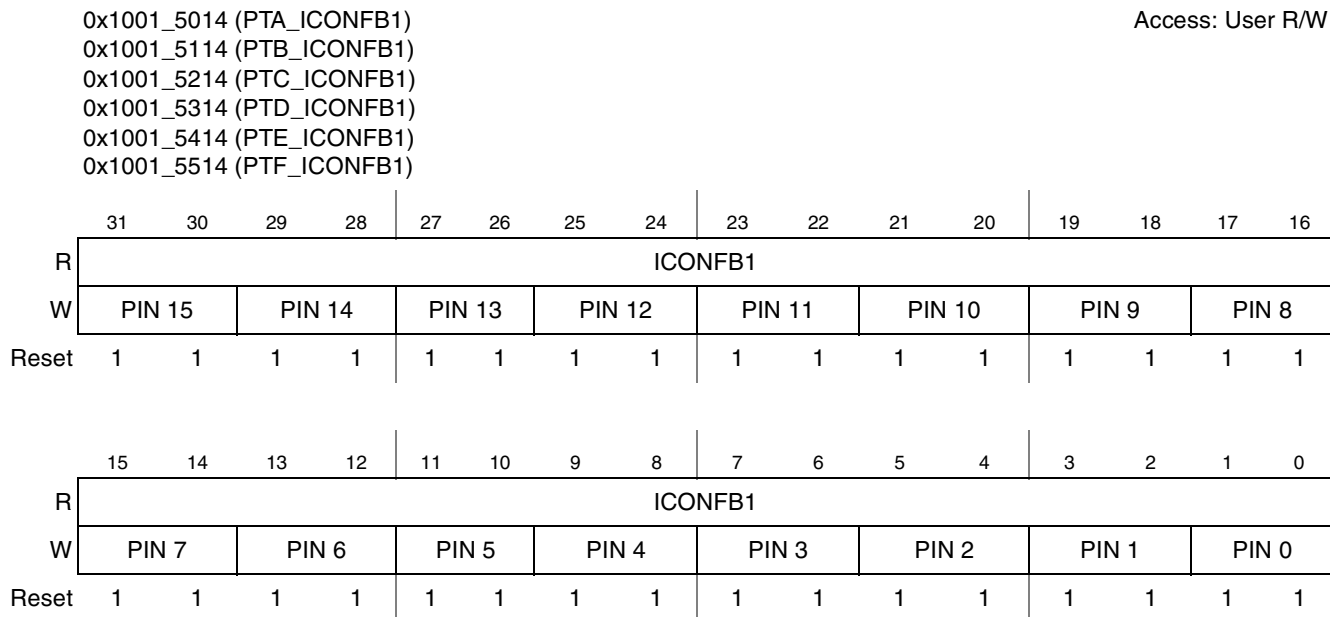
Figure 6-9. Input Configuration Register B1 (ICONFB1)
