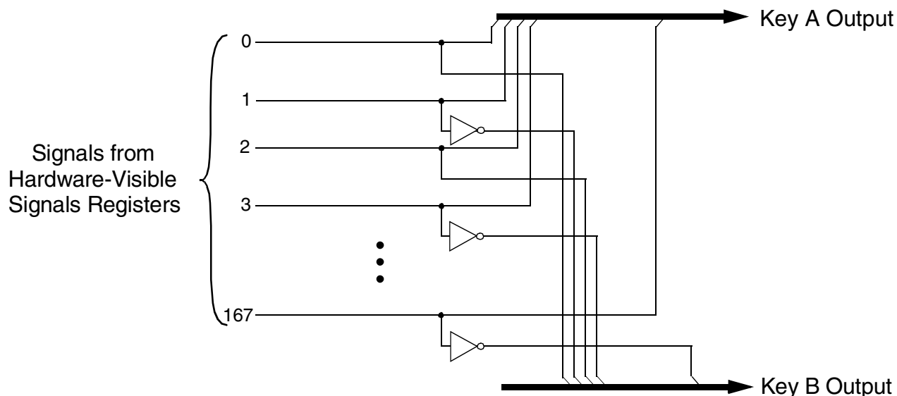
Figure 14-28. Second 3DES Key Derivation
