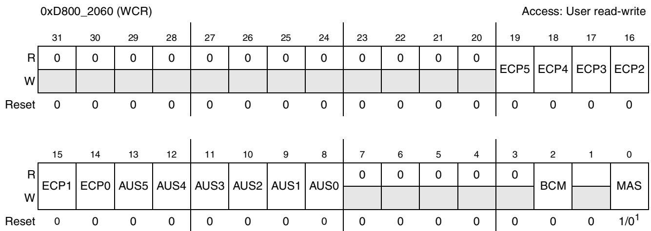
Figure 17-6. WCR Register
