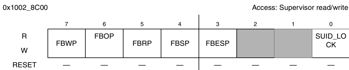
Figure 14-25. Fuse Bank 1 Access Protection Register
