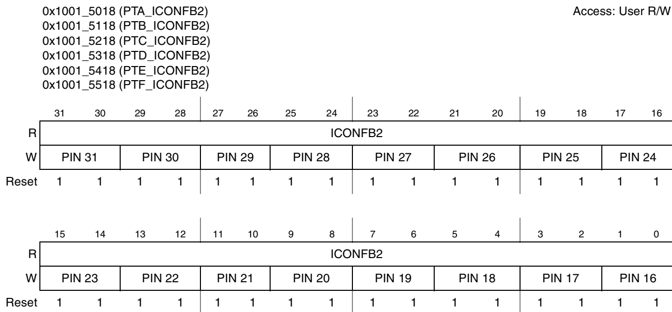
Figure 6-10. Input Configuration Register B1 (ICONFB2)
