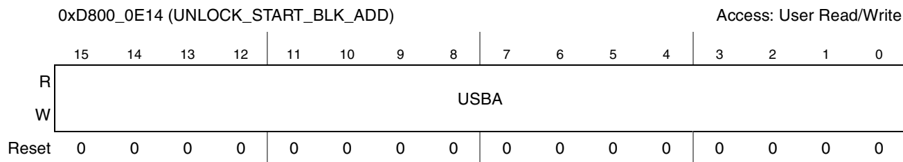
Figure 19-15. Unlock_Start_Blk_Add Register
