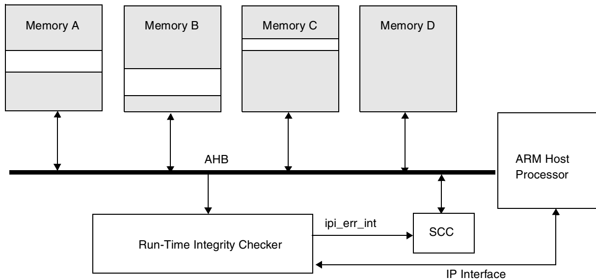
Figure 13-2. System Diagram
