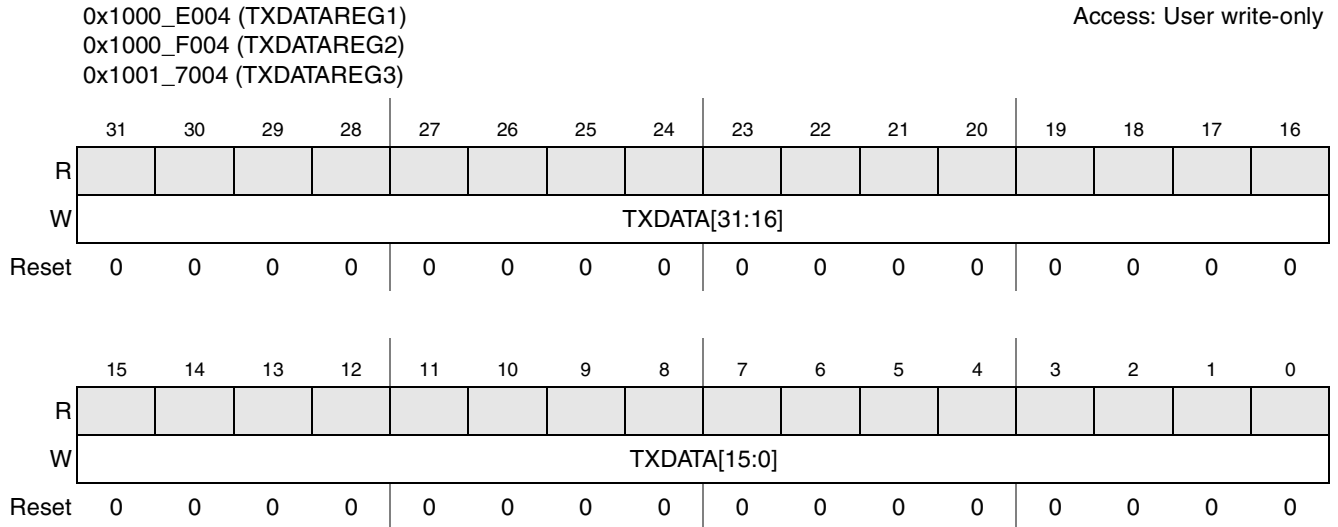
Figure 23-16. TXDATA Register Diagram
