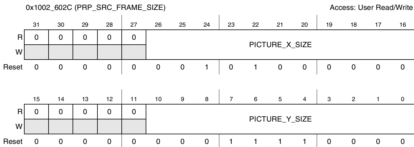
Figure 41-39. PrP Source Frame Size Register
