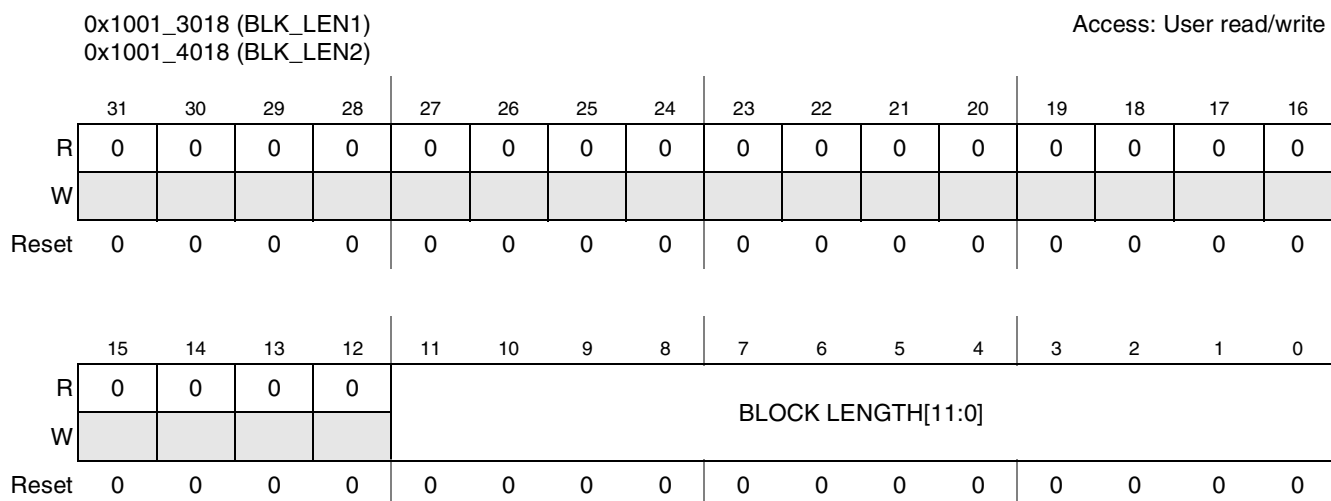
Figure 27-10. SDHC Block Length Register
