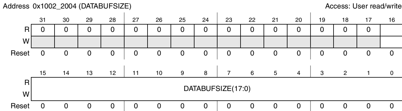
Figure 44-13. Data Buffer Size register
