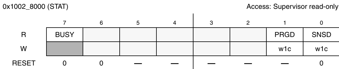
Figure 14-3. Status Register
