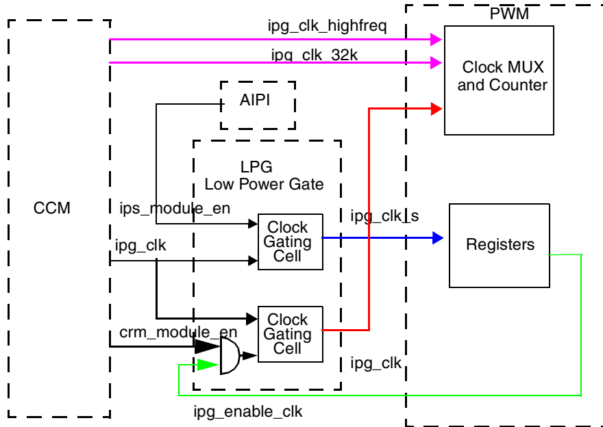
Figure 32-10. PWM Clocking
