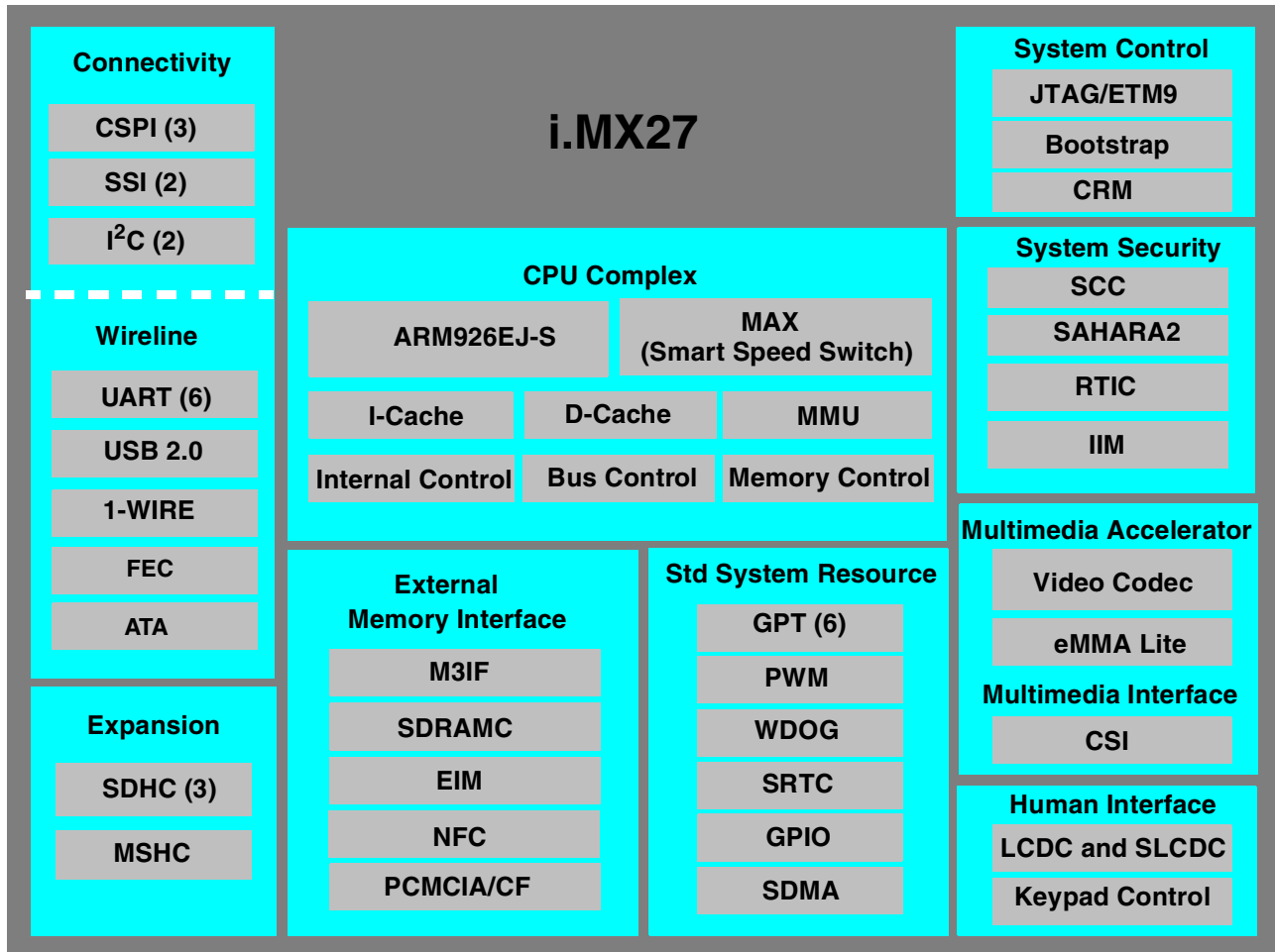
Figure 1-1. i.MX27 Processor Functional Block Diagram
