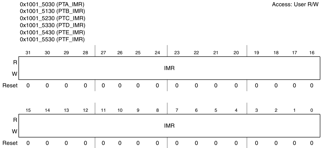
Figure 6-22. Interrupt Mask Register (IMR)
