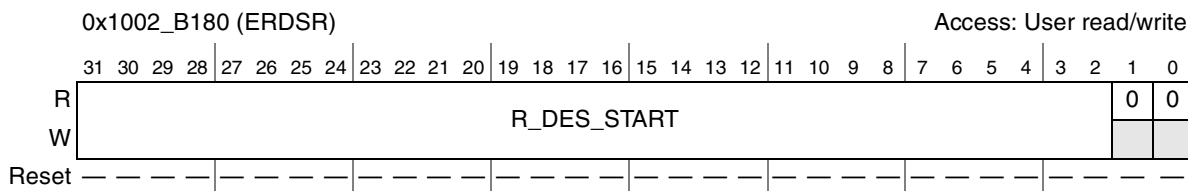
Figure 29-24. ERDSR Register
