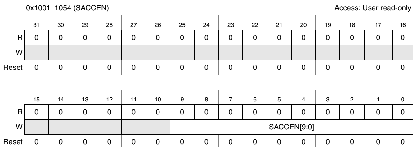
Figure 42-42. SSI AC97 Channel Enable Register
