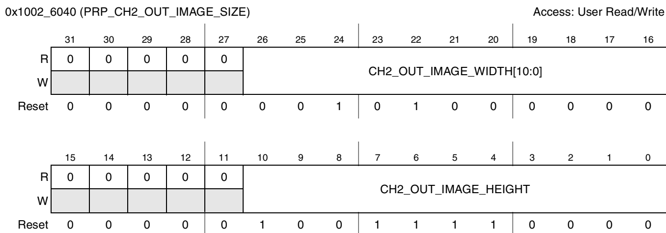
Figure 41-44. PrP Destination CH2 Output Image Size Register
