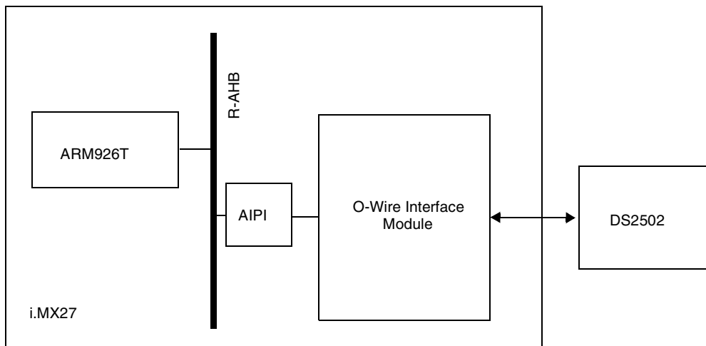
Figure 21-1. 1-Wire Connection
