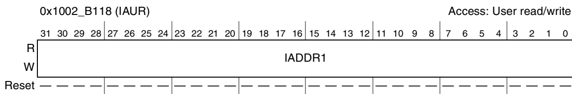
Figure 29-17. IAUR Register
