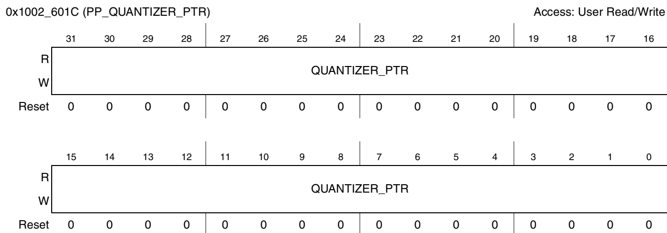
Figure 41-14. PP Quantizer Start Address Register
