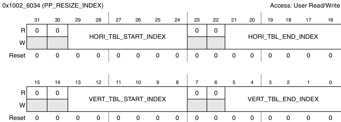
Figure 41-20. PP Resize Table Index Register
