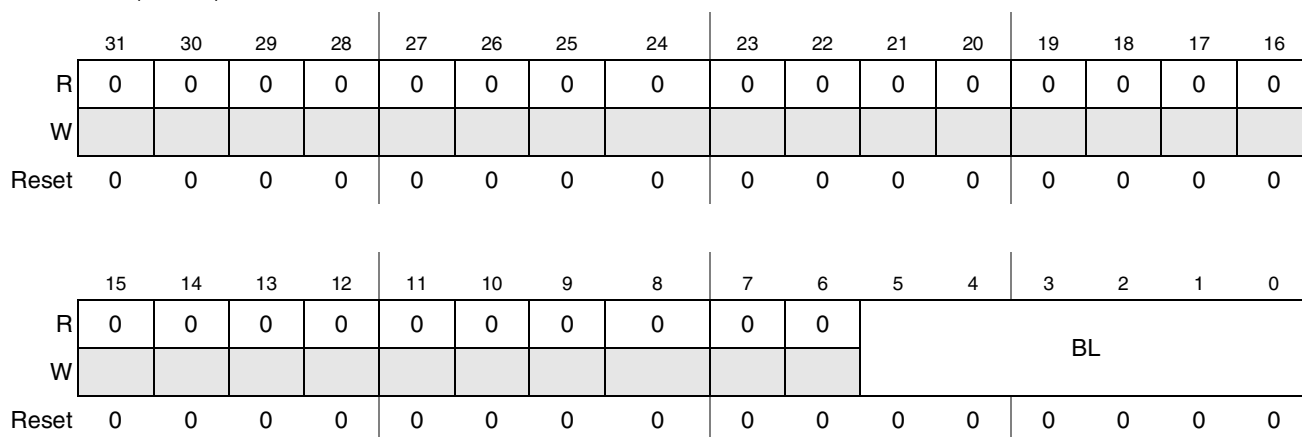
Figure 37-23. Channel Burst Length Registers (BLR0–BLR15)
