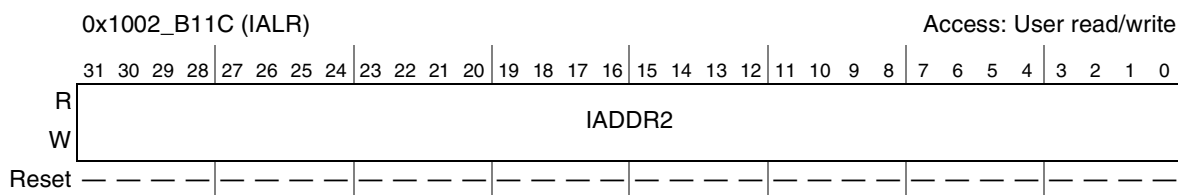
Figure 29-18. IALR Register
