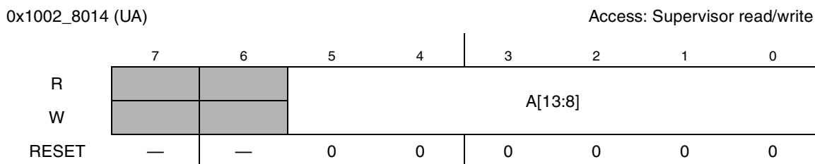
Figure 14-8. Upper Address Register
