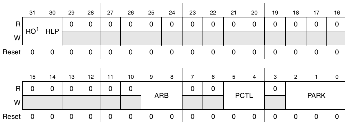
Figure 36-3. Slave General Purpose Control Register (SGPCR0-2)
