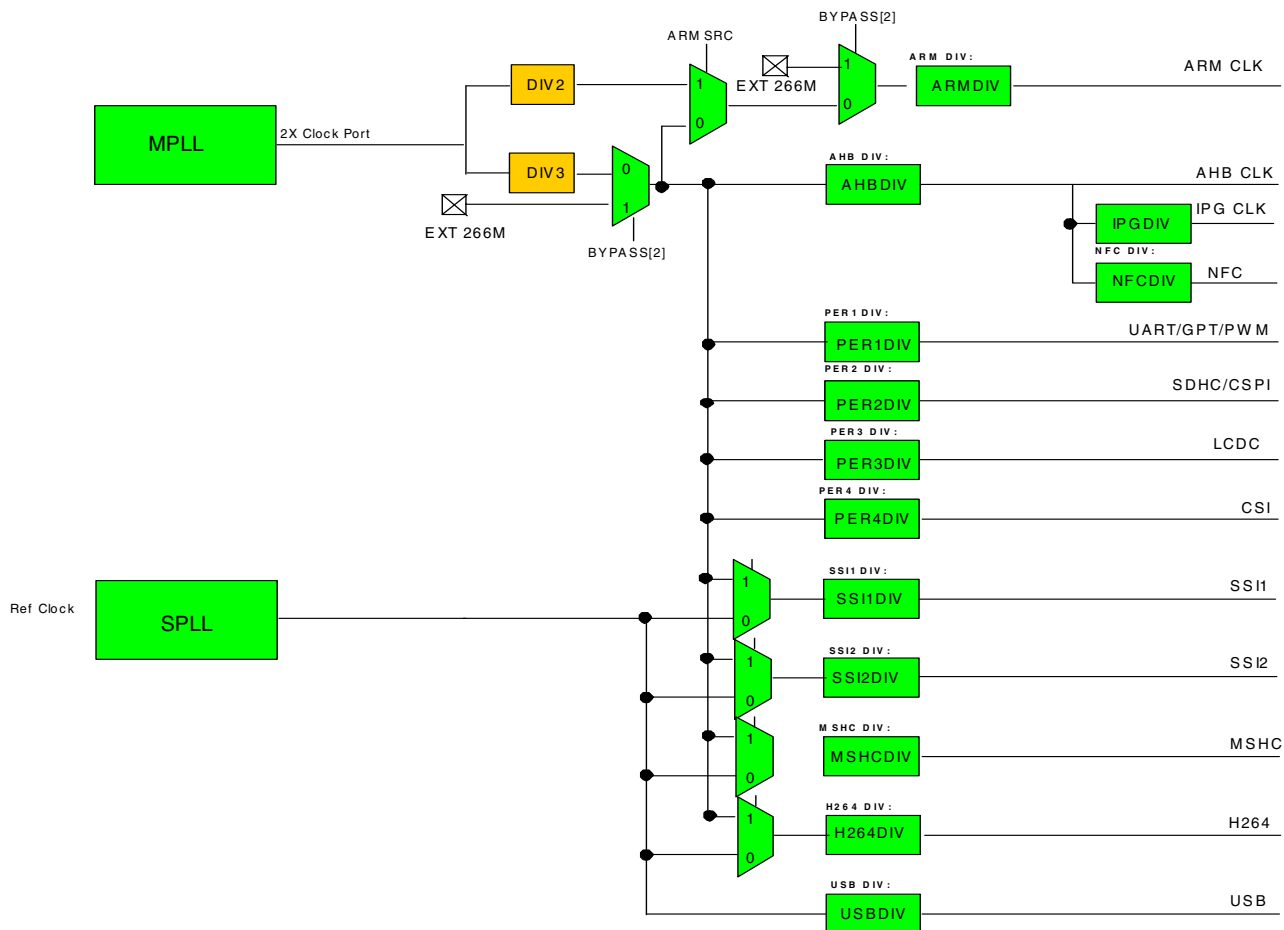
Figure 3-2. i.MX27 Clock Distribution Block Diagram (2 of 2)
