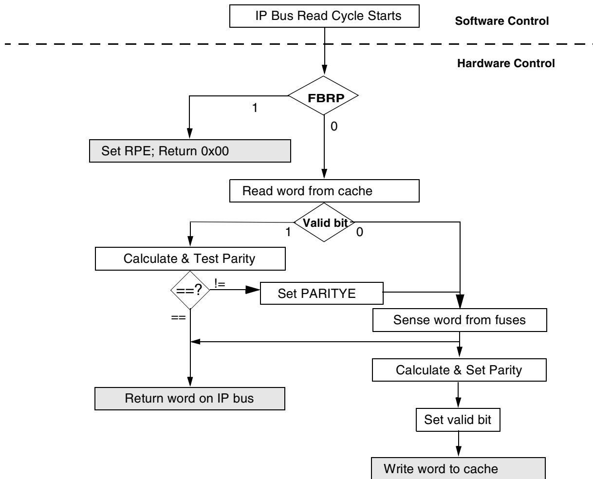
Figure 14-38. Software Fuse Read
