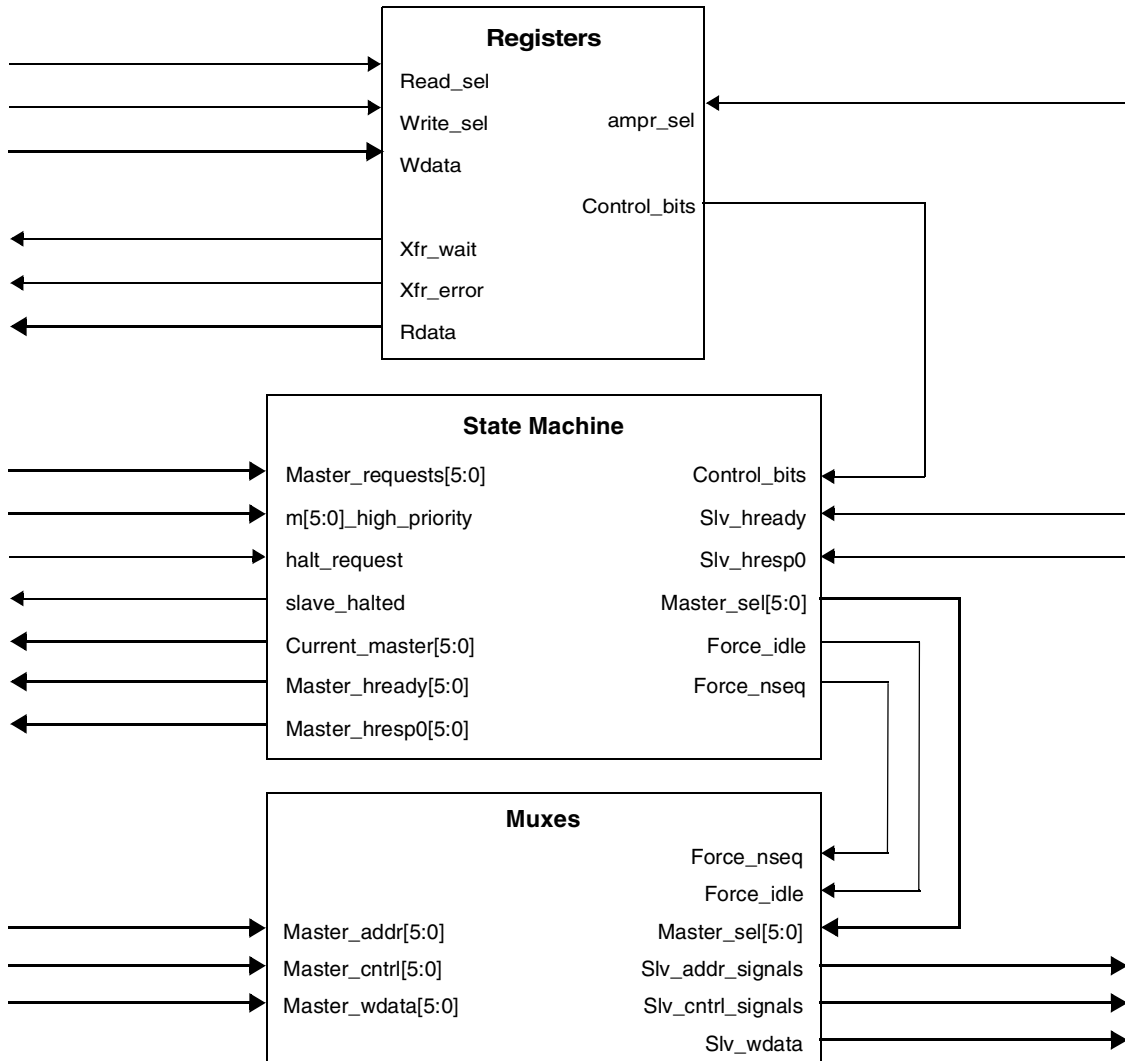
Figure 36-7. MAX Slave Port Block Diagram
