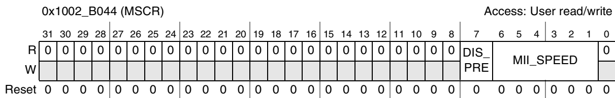
Figure 29-10. MSCR Register
