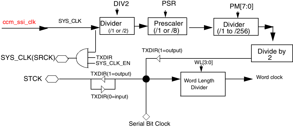
Figure 42-45. SSI Transmit Clock Generator Block Diagram
