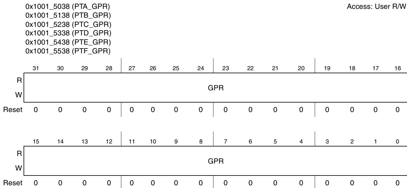
Figure 6-24. General Purpose Register
