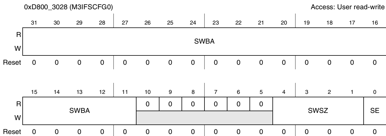
Figure 16-4. M3IF Snooping Configuration Register 0 (M3IFSCFG0)
