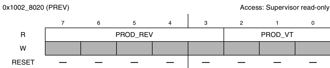
Figure 14-11. Product Revision Register
