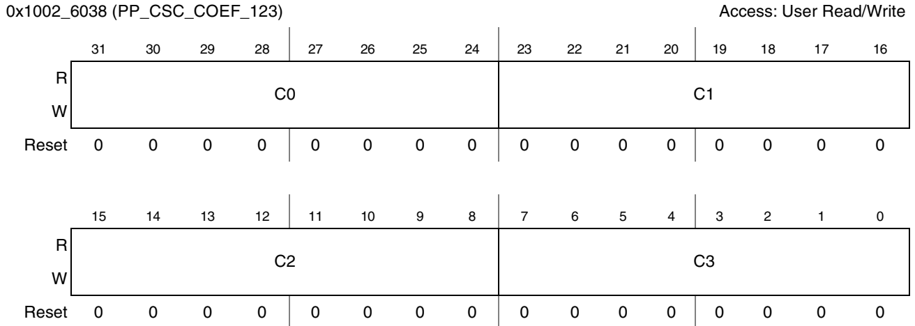
Figure 41-21. PP CSC Coefficient_123 Register
