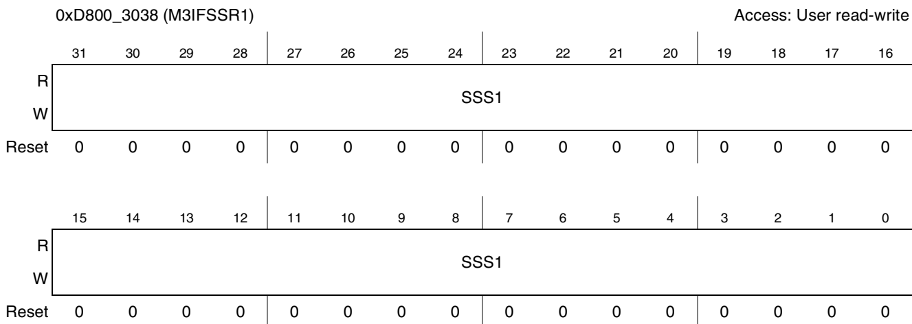
Figure 16-8. M3IF Snooping Status Register 1 (M3IFSSR1)
