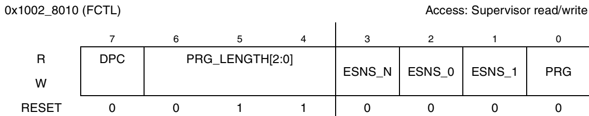
Figure 14-7. Fuse Control Register
