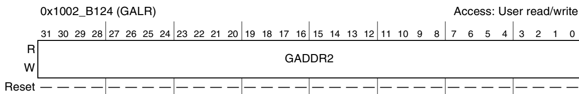
Figure 29-20. GALR Register
