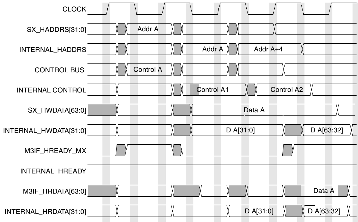
Figure 16-19. MPG64 Simple Double Word Transfer
