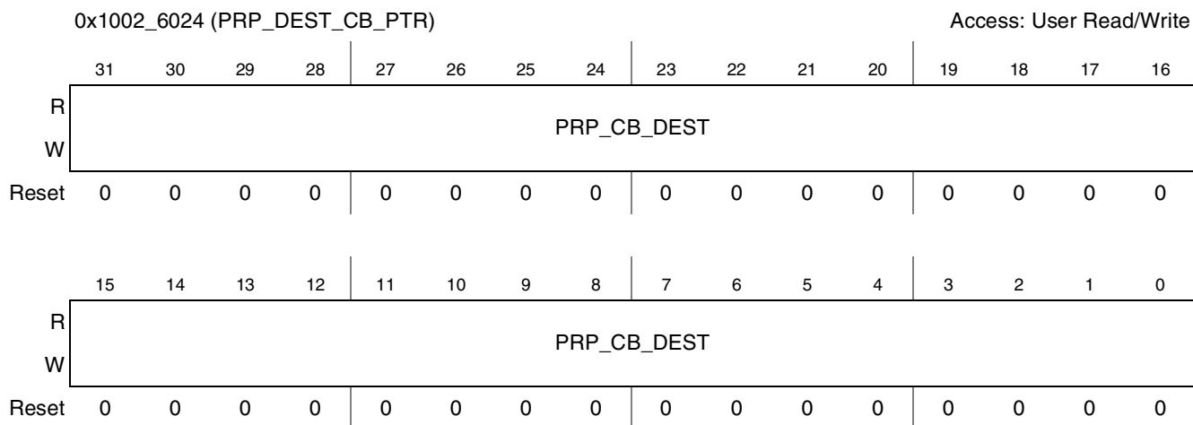
Figure 41-37. PrP Destination Cb Address Register
