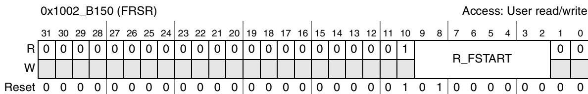
Figure 29-23. FRSR Register
