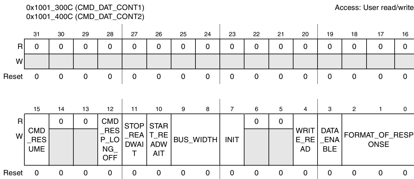
Figure 27-7. SDHC Command and Data Control Register
