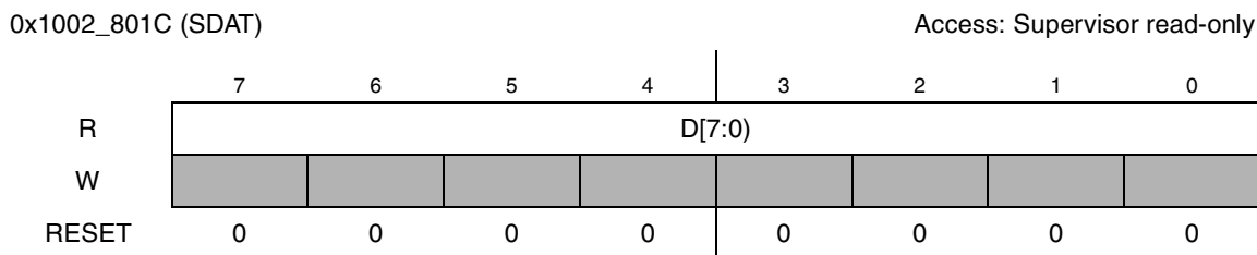
Figure 14-10. Explicit Sense Data Register
