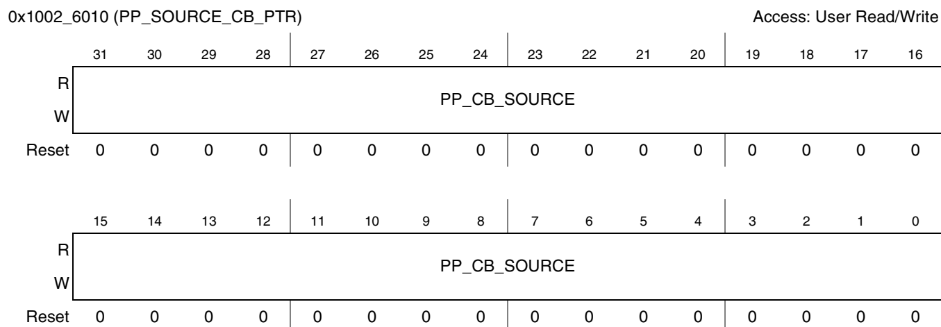
Figure 41-11. PP Source Cb Address Register
