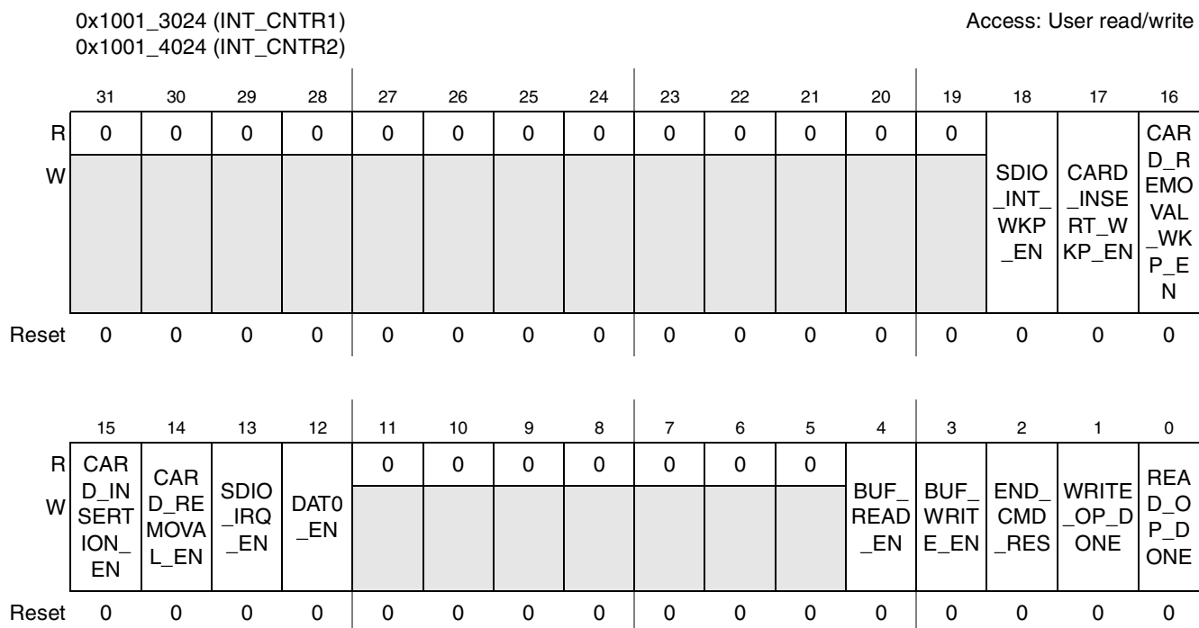
Figure 27-13. SDHC Interrupt Control Register
