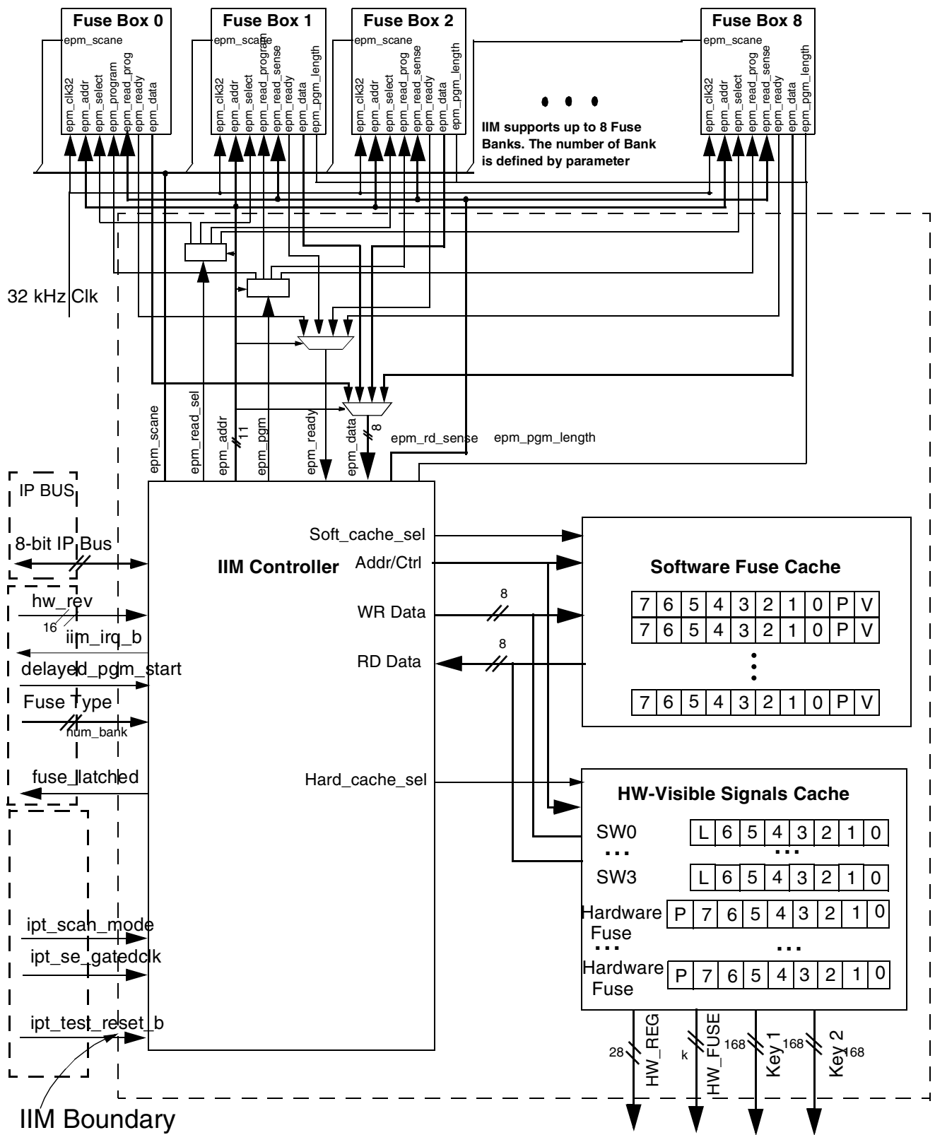
Figure 14-2. IIM Microarchitecture
