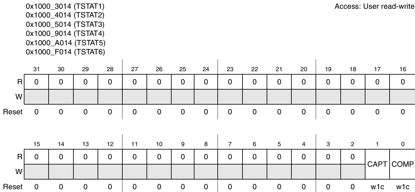
Figure 31-7. GPT Status Register
