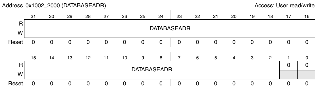
Figure 44-12. Data Buffer Base Address register
