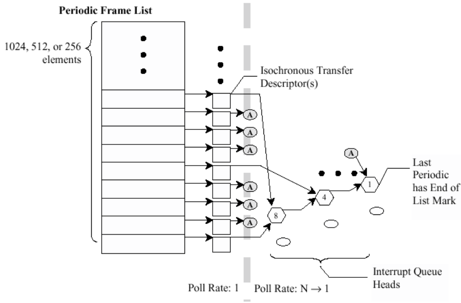
Figure 30-57. Example Periodic Schedule
