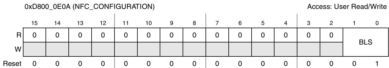
Figure 19-8. NFC_Configuration Register
