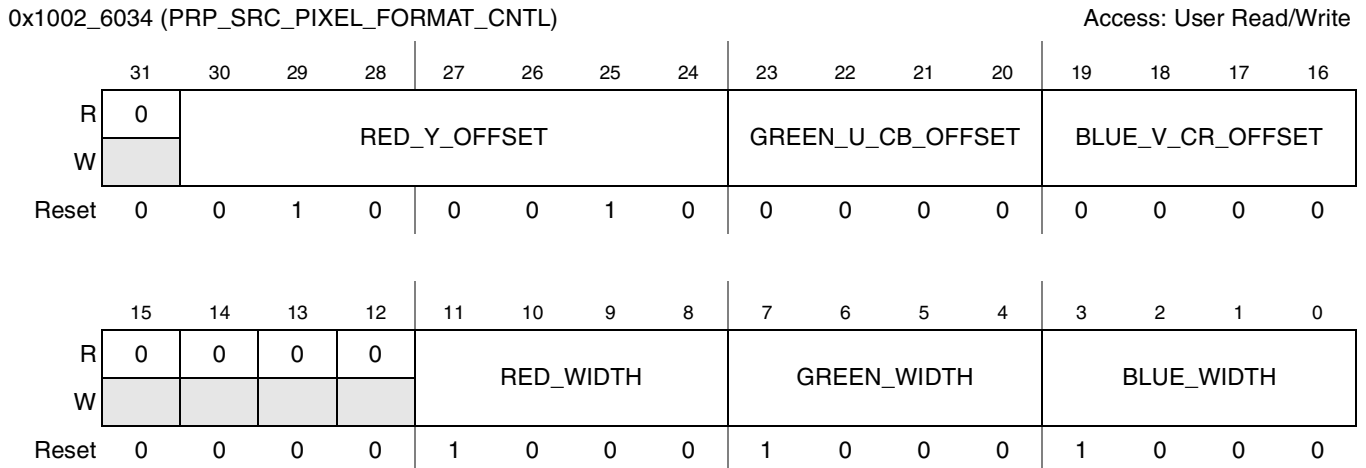
Figure 41-41. PrP Source Pixel Format Control Register
