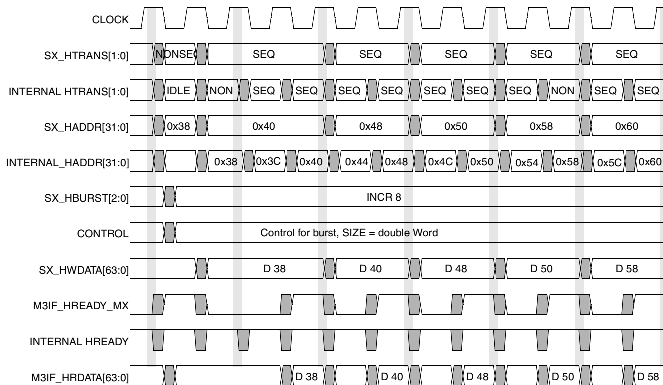
Figure 16-20. MPG64—8 Beat Incremental Burst of Double Words to 32-bit SDRAM
