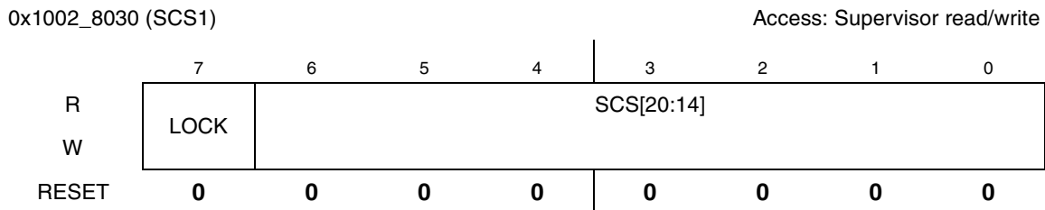
Figure 14-15. Software Controllable Signals Register 1
