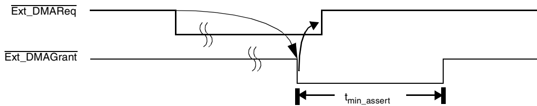
Figure 37-2. Assertion of DMA External Grant Signal
