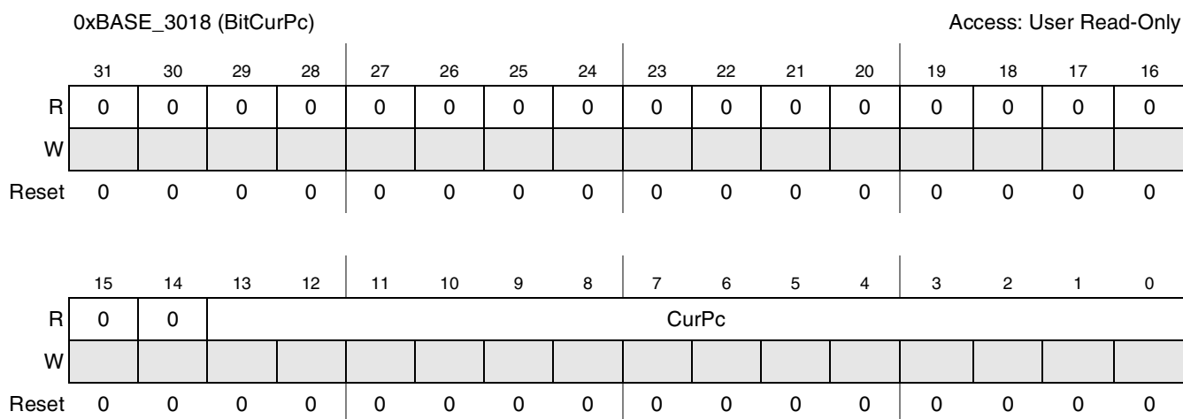
Figure 40-9. Video Codec BIT Current PC Register
