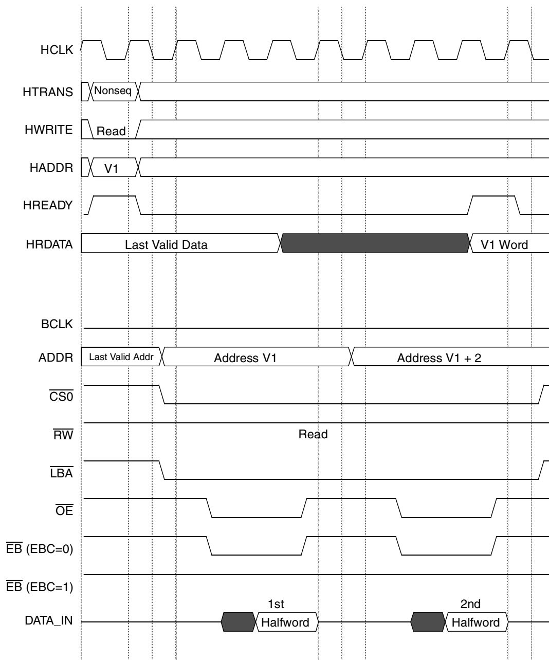
Figure 17-21. Read Access, WSC=3, OEA=2, OEN=2, EBRA=2, EBRN=2
