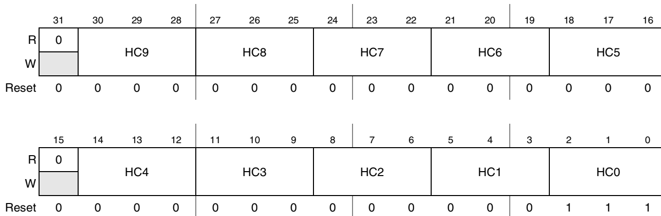
Figure 41-49. PrP Channel-1 Horizontal Resize Coefficient 1
