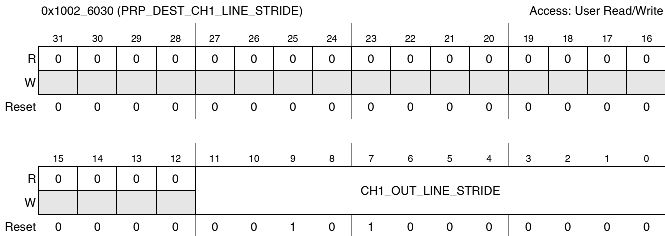
Figure 41-40. PrP Destination Channel-1 Line Stride Register
