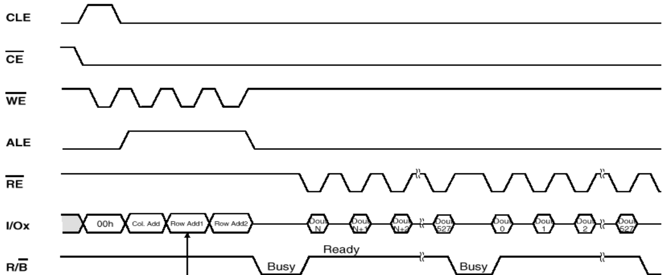
Figure 19-21. Read Operation
