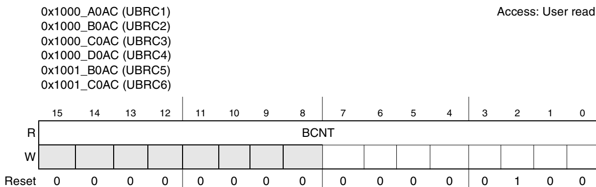
Figure 28-17. UART Baud Rate Count Register Summary (UBRC)
