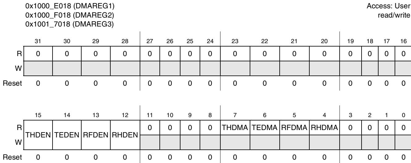
Figure 23-21. DMA Control Register Diagram
