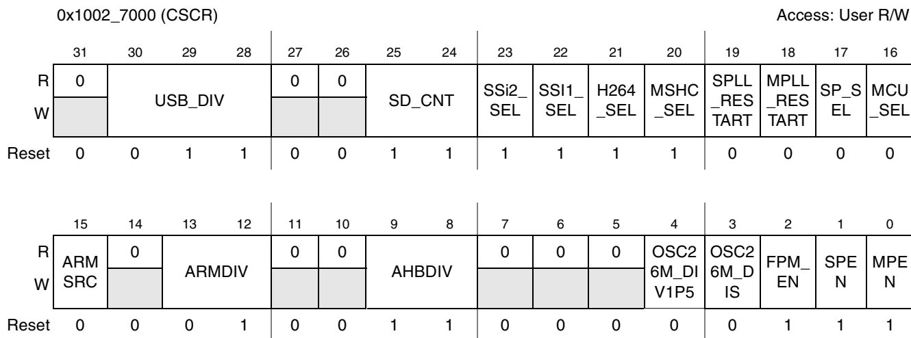
Figure 3-4. Clock Source Control Register (CSCR)
