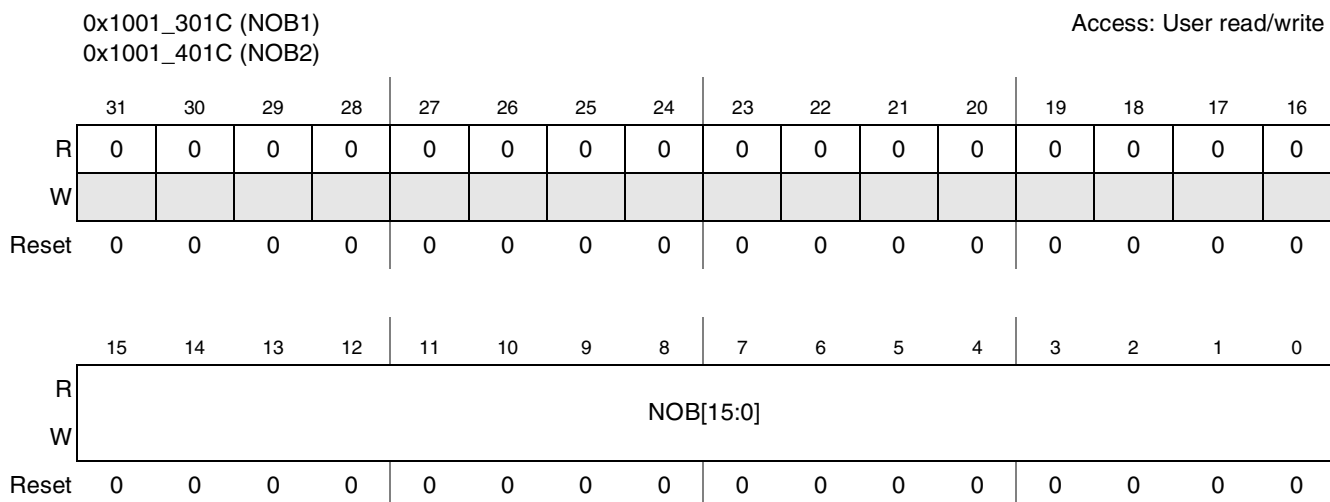
Figure 27-11. SDHC Number of Blocks Register
