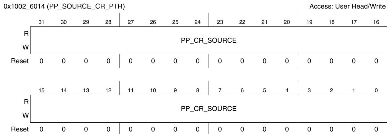
Figure 41-12. PP Source Cr Address Register
