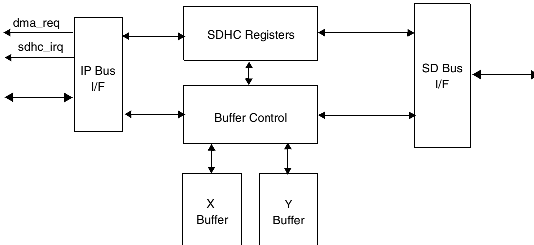
Figure 27-18. SDHC Buffer Scheme
