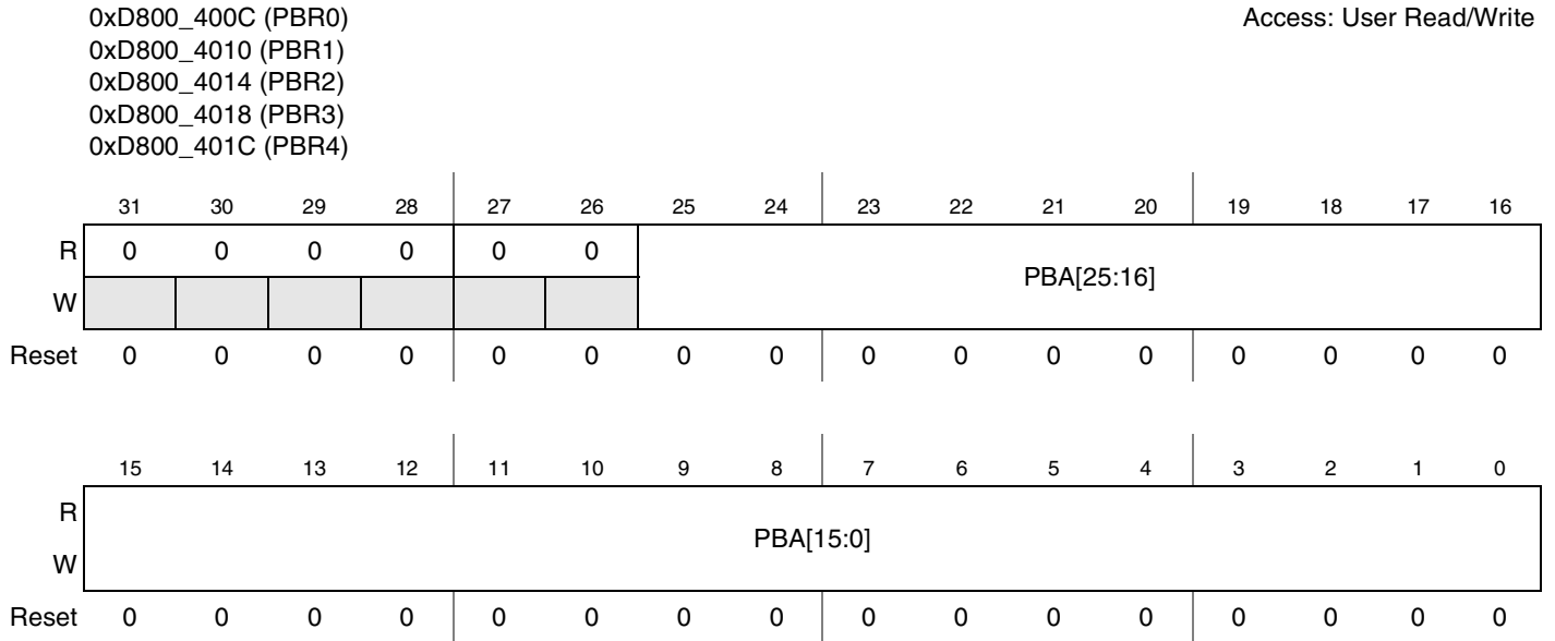
Figure 20-6. PCMCIA Base Registers 0–4 (PBR0–PBR4)
