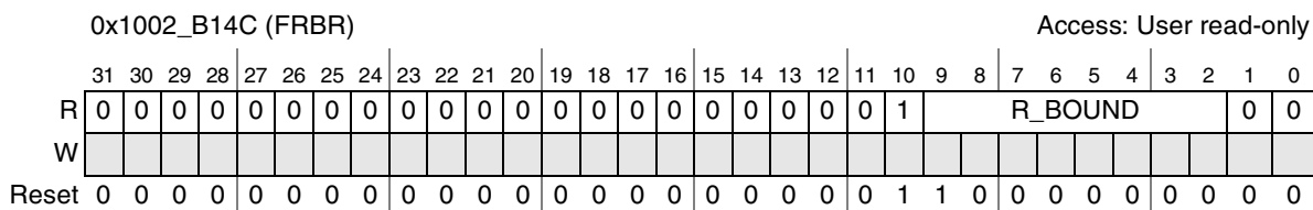
Figure 29-22. FRBR Register
