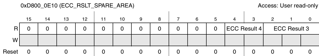
Figure 19-12. ECC_Rslt_Spare_Area Register
