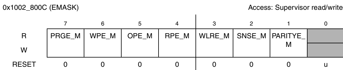
Figure 14-6. Error IRQ Mask Register
