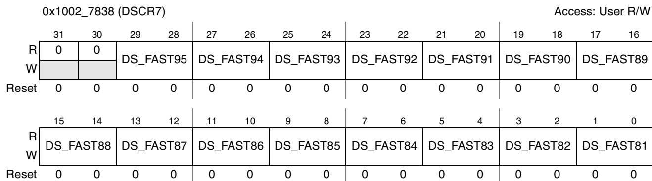
Figure 4-12. Drive Strength Control Register 7 (DSCR7)
