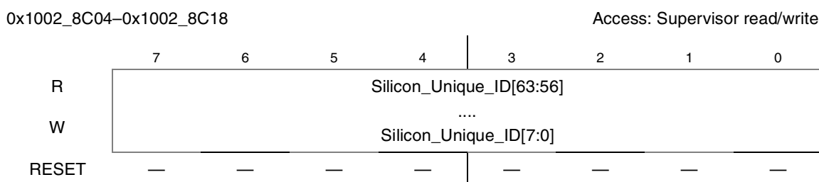
Figure 14-26. Silicon_Unique_ID Register
