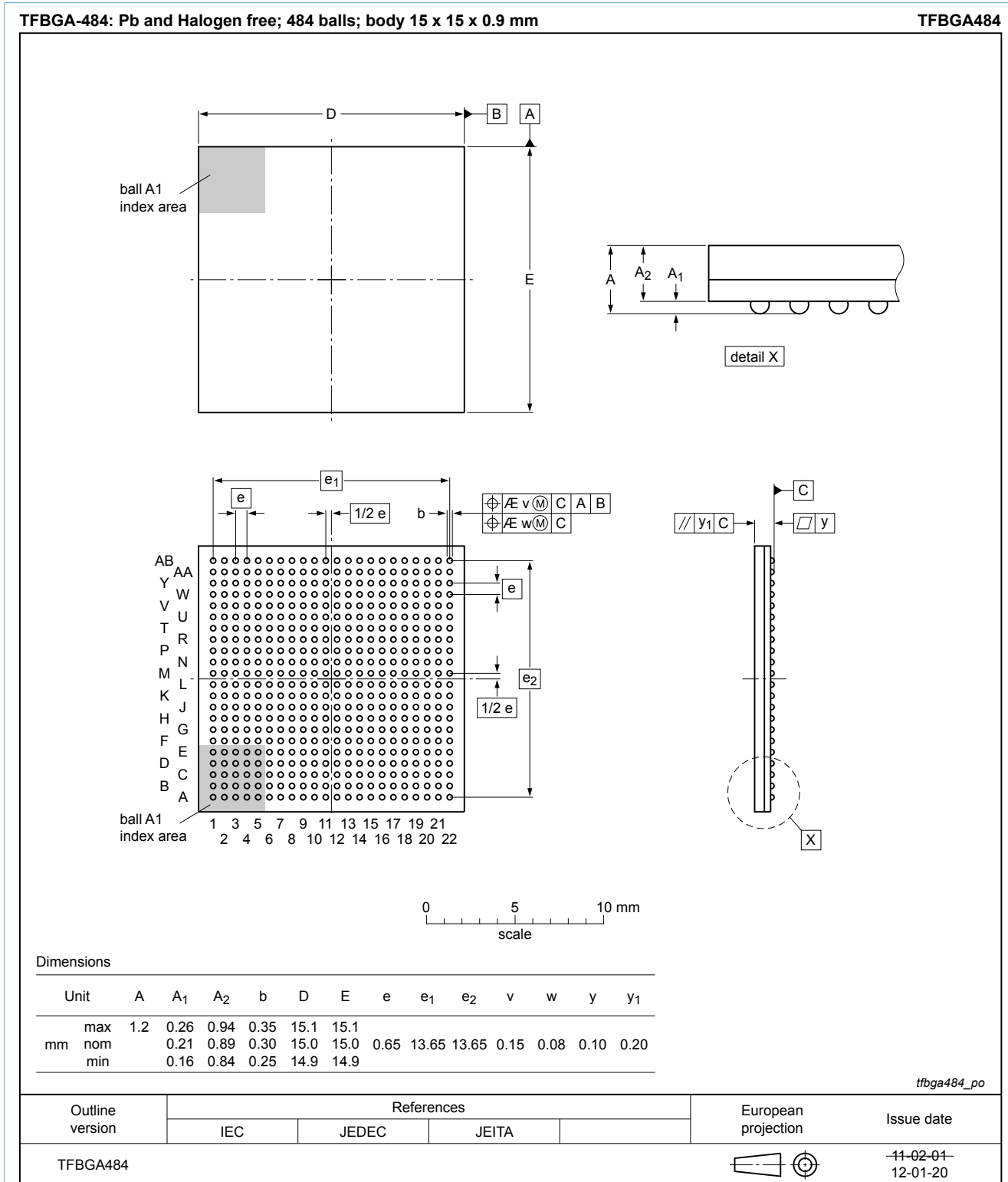
Fig. 1. Package outline TFBGA484 (TFBGA_ASC88x)
