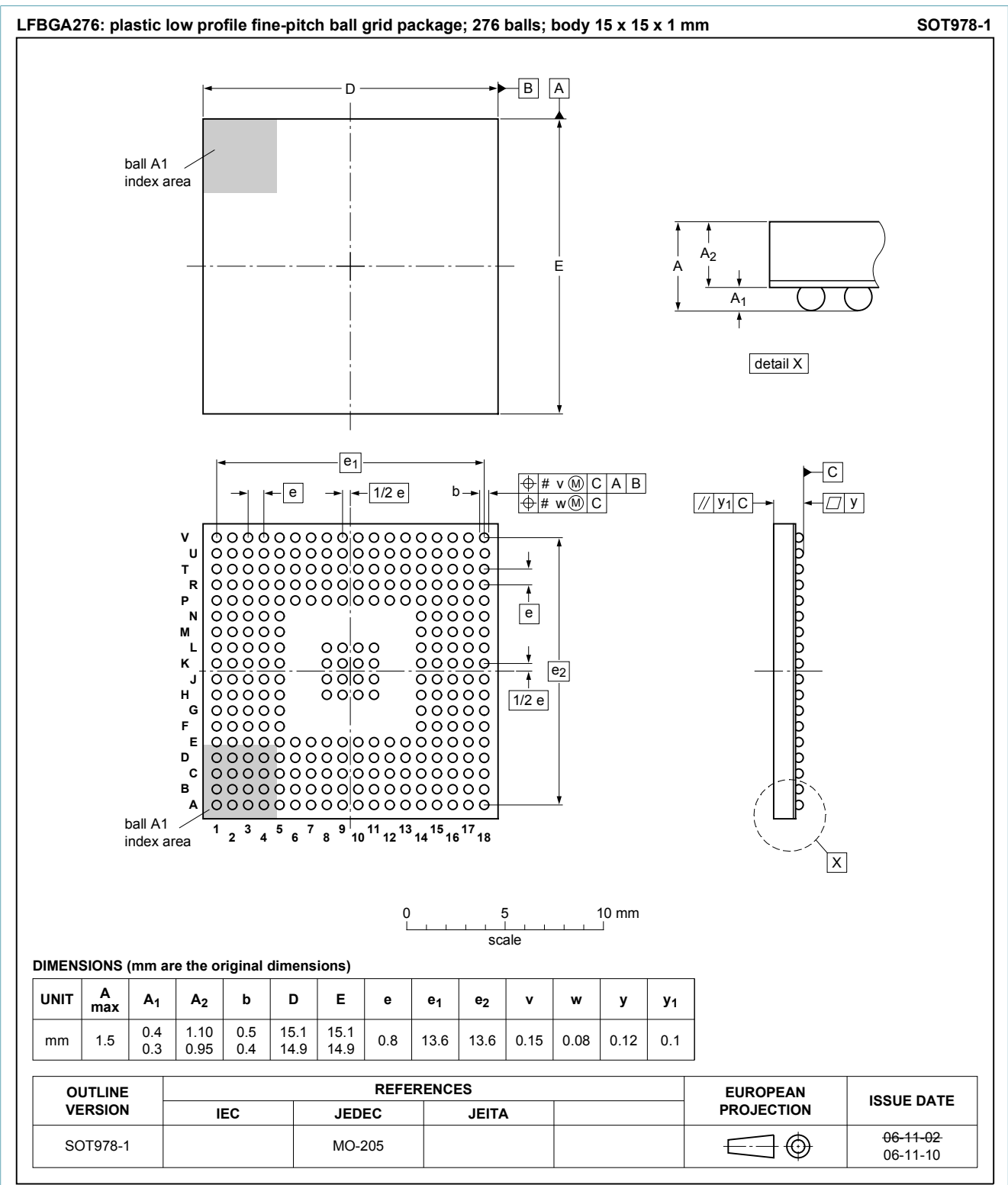
Fig. 1. Package outline LFBGA276 (SOT978-1)
