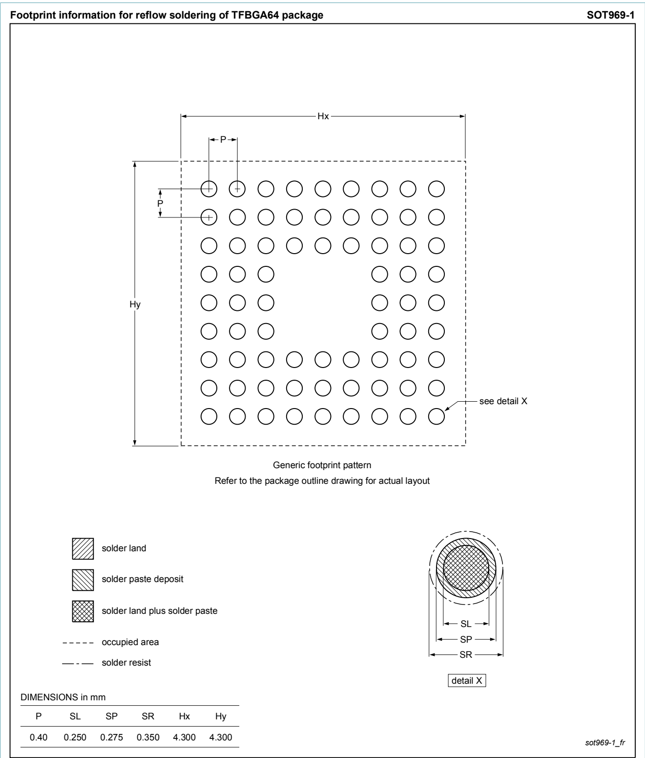
Fig. 2. Reflow soldering footprint for TFBGA64 (SOT969-1)
