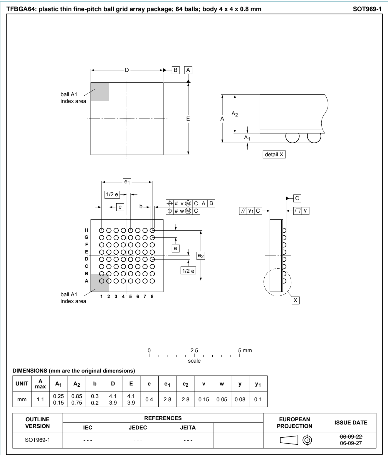
Fig. 1. Package outline TFBGA64 (SOT969-1)
