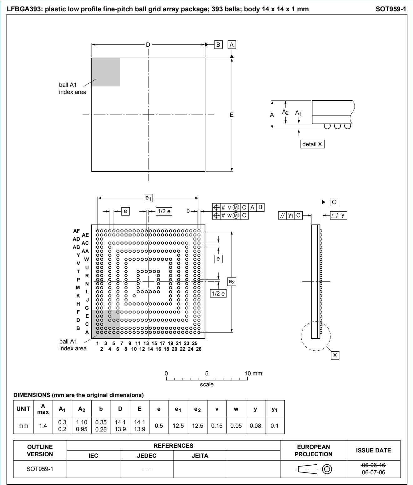
Fig. 1. Package outline LFBGA393 (SOT959-1)
