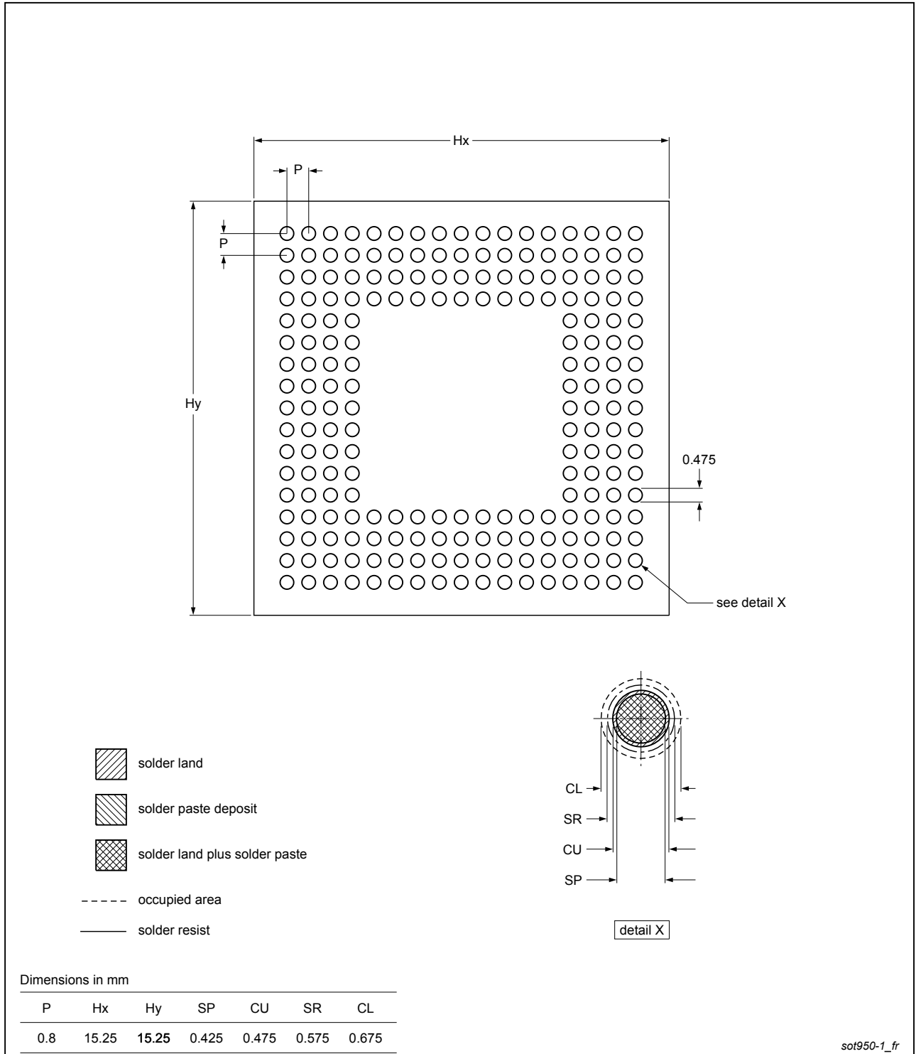
Fig. 2. Reflow soldering footprint for TFBGA208 (SOT950-1)
