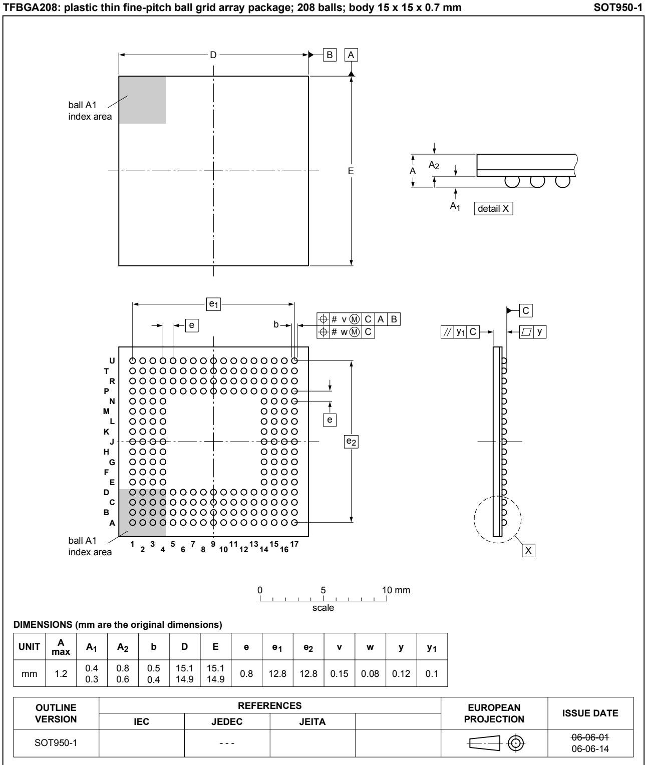
Fig. 1. Package outline TFBGA208 (SOT950-1)
