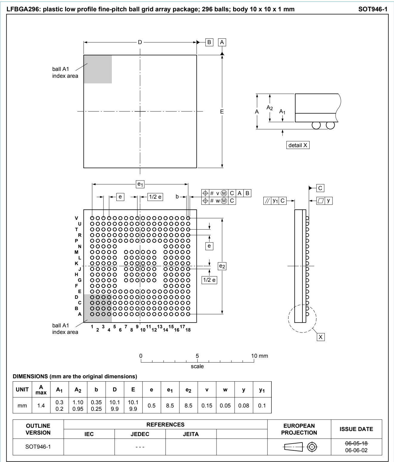
Fig. 1. Package outline LFBGA296 (SOT946-1)
