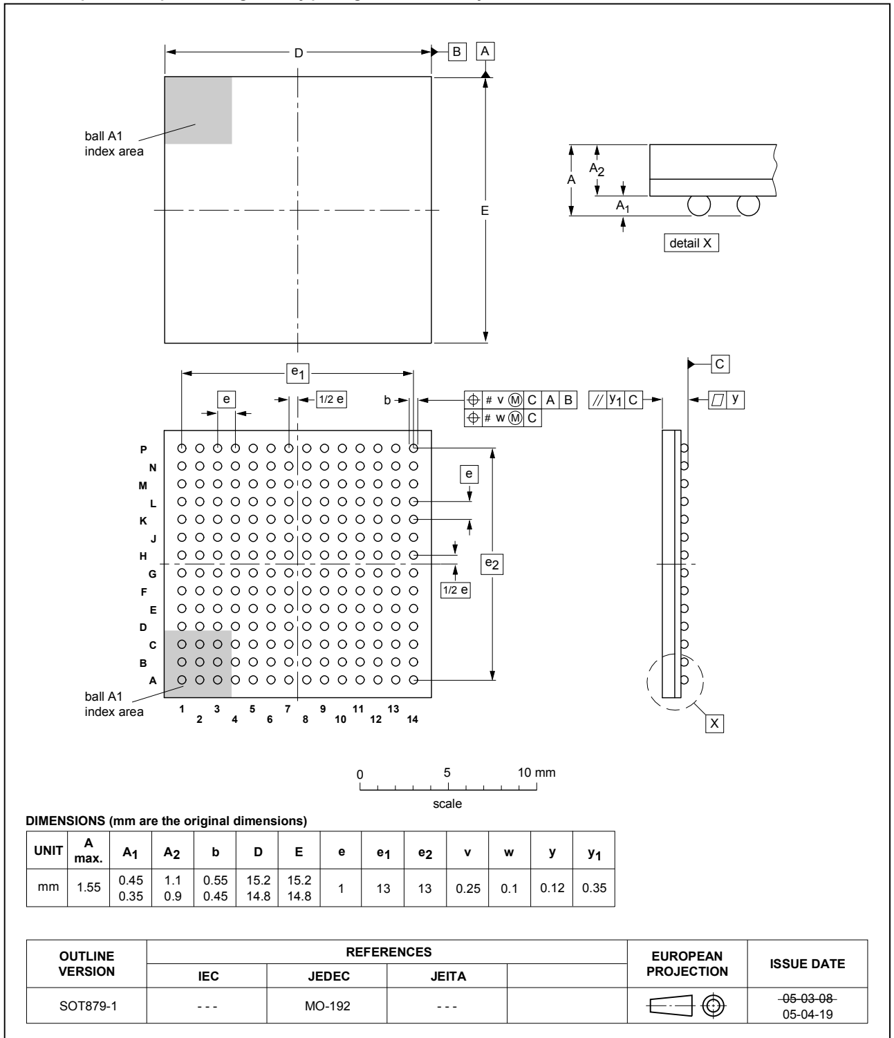
Fig. 1. Package outline LPGA196 (SOT879-1)
