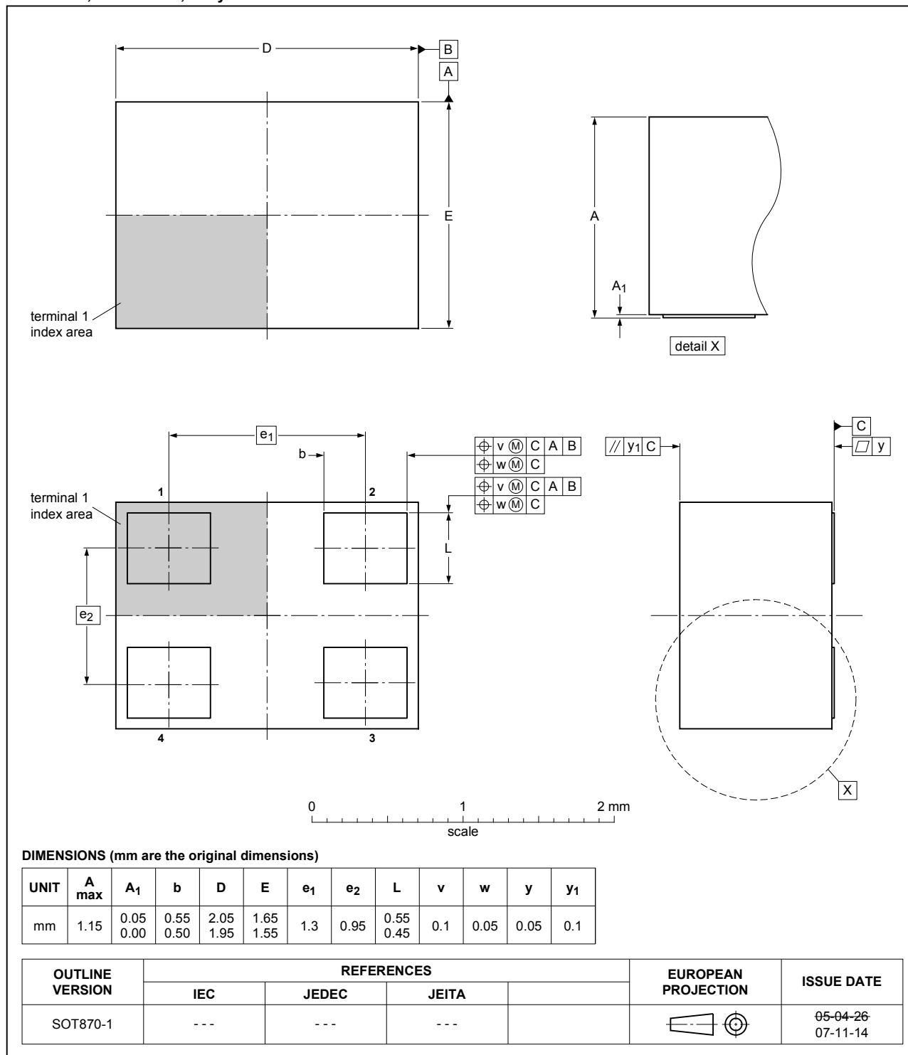
Fig. 1. Package outline TSON4R (SOT870-1)
