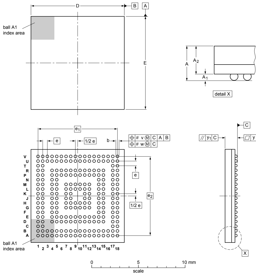
LFBGA240: plastic low profile fine-pitch ball grid array package; 240 balls; body 10 x 10 x 1.05 mm
