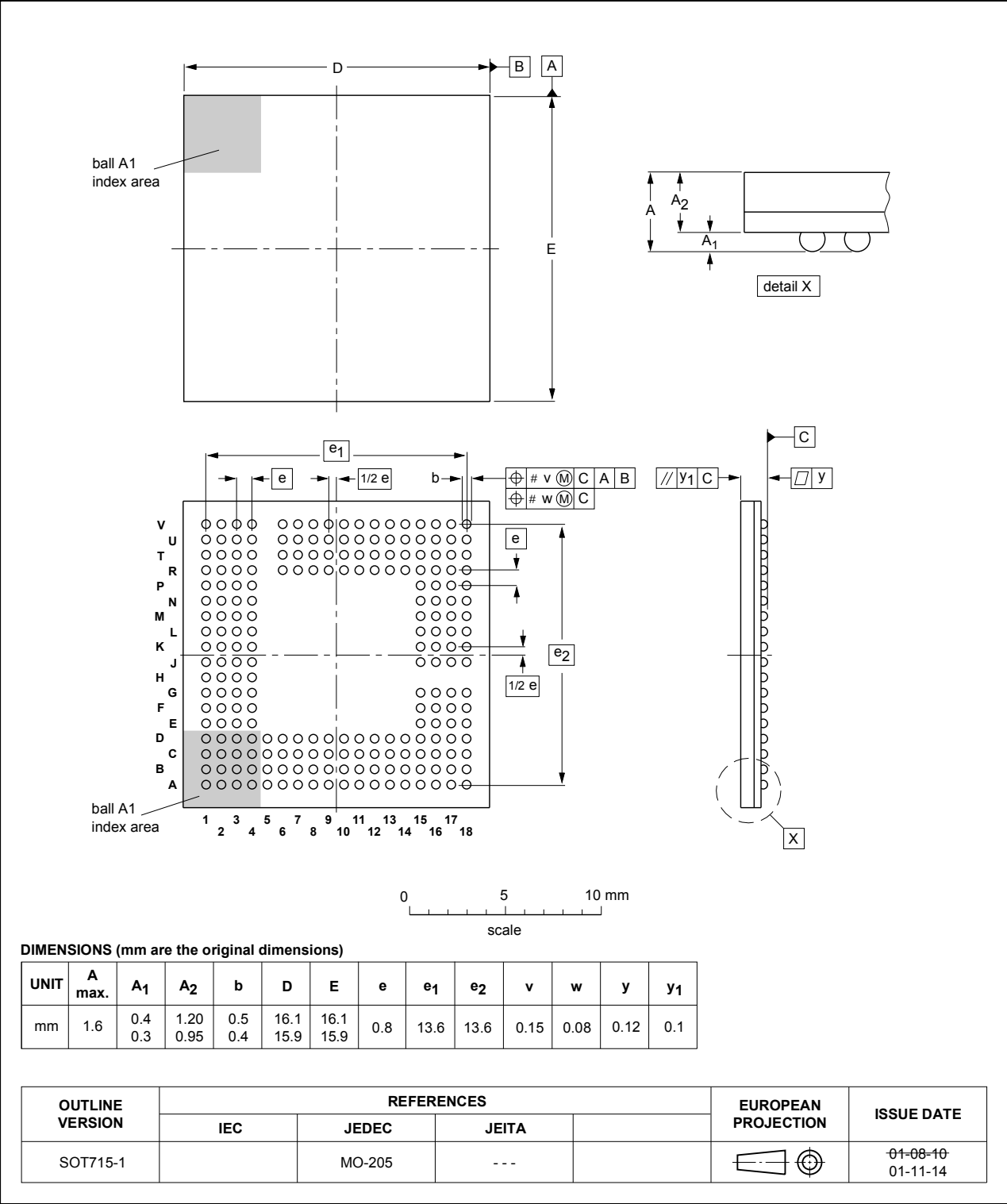
Fig. 1. Package outline LFBGA216 (SOT715-1)
