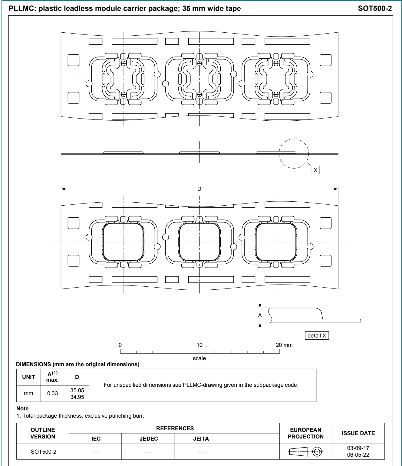
Figure 1. Package outline PLLMC (SOT500-2)
