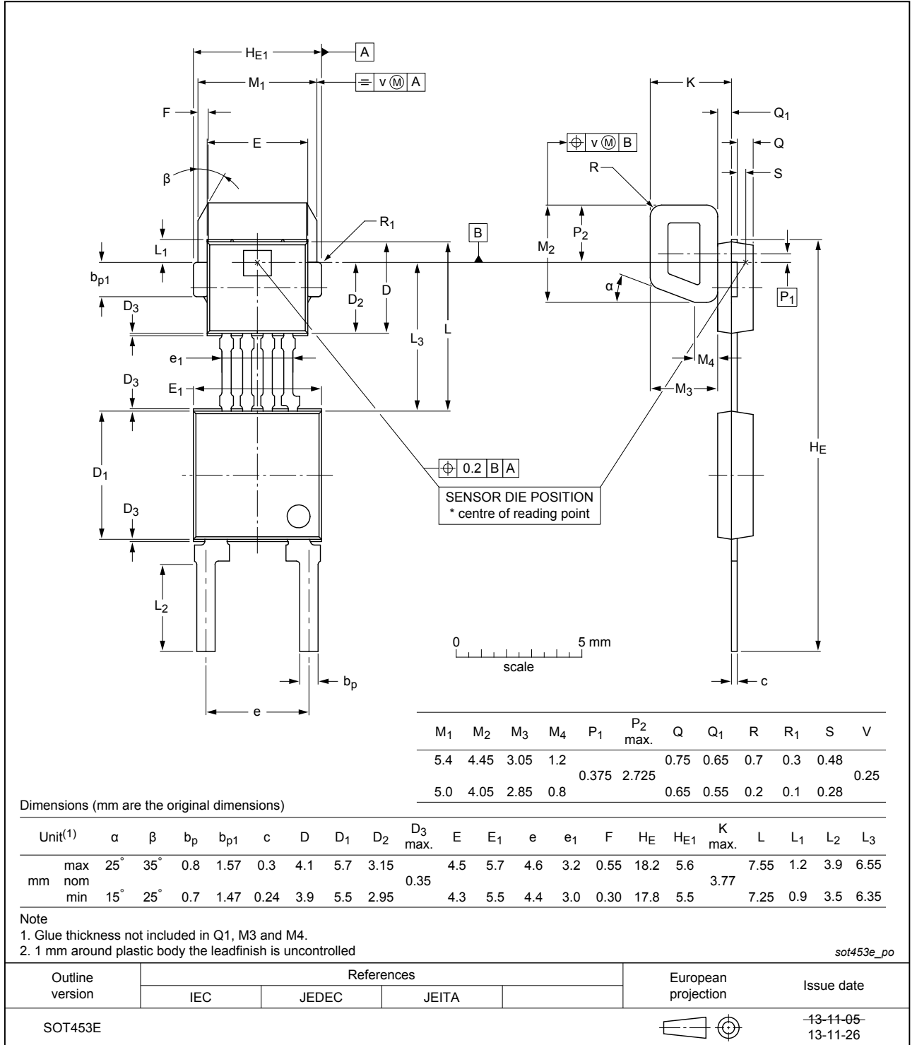
Fig. 1. Package outline SIP2 (SOT453E)
