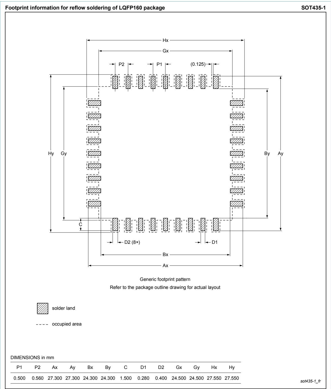
Fig. 2. Reflow soldering footprint for LQFP160 (SOT435-1)
