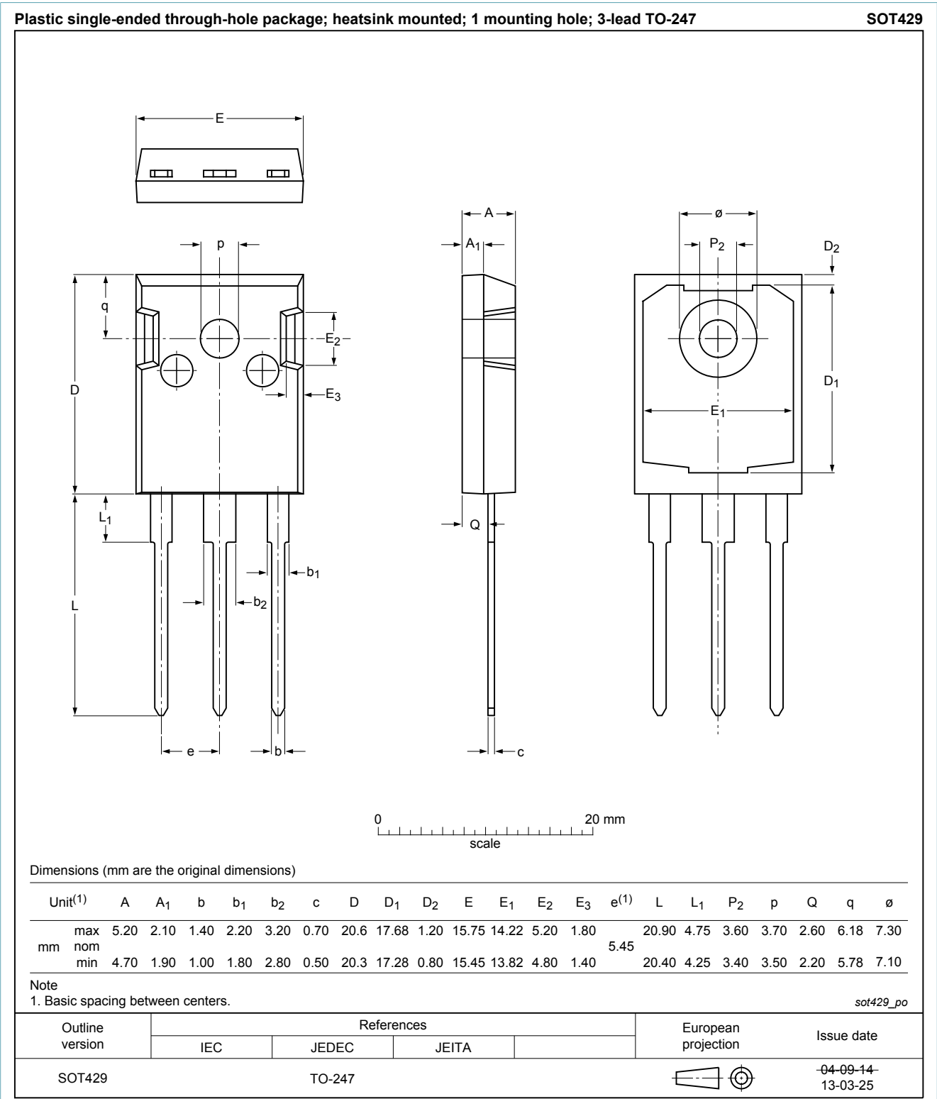
Fig. 1. Package outline TO-247 (SOT429)
