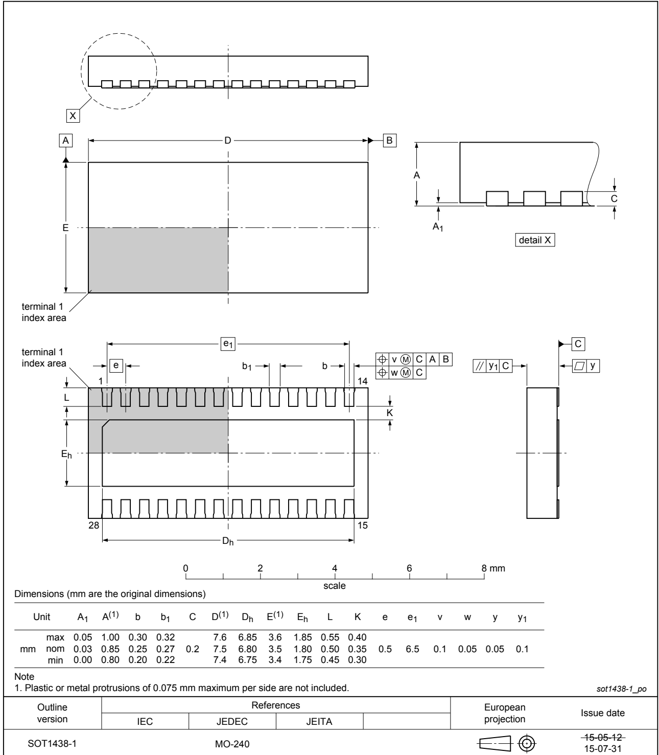
Fig. 1. Package outline HVSON28 (SOT1438-1)
