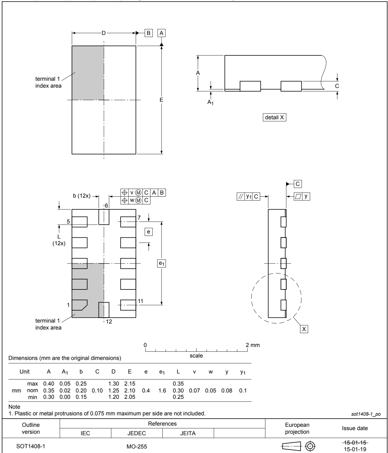
Fig. 1. Package outline X2QFN12 (SOT1408-1)
