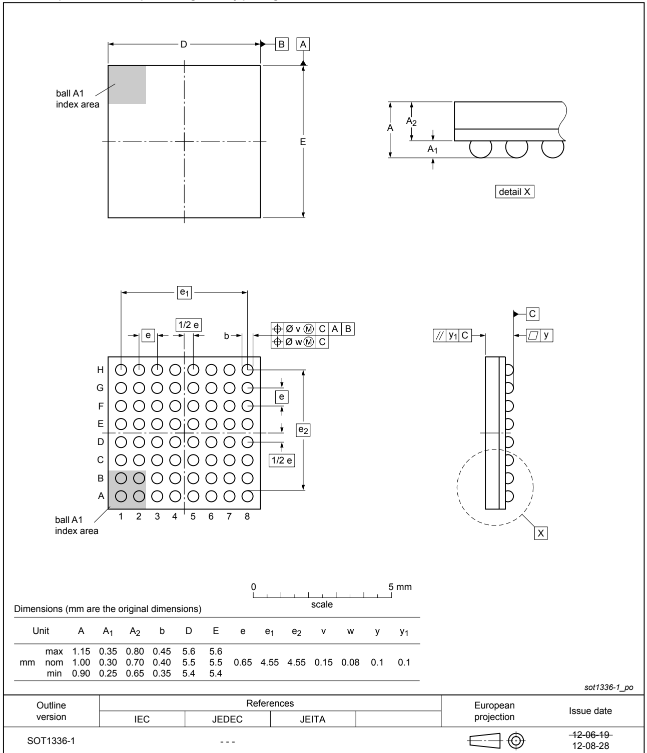
Fig. 1. Package outline TFBGA64 (SOT1336-1)
