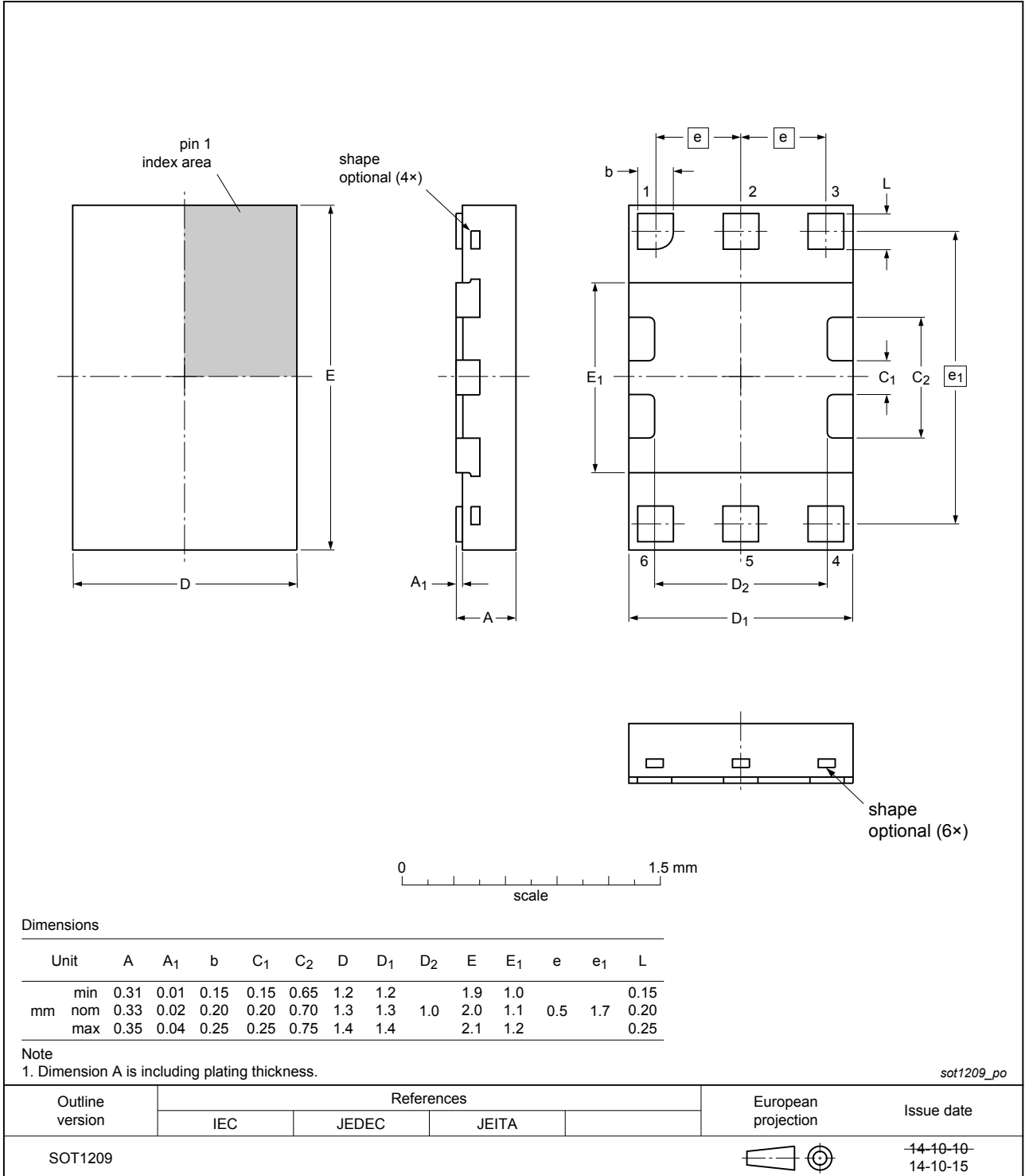
Fig. 1. Package outline HXSON6 (SOT1209)
