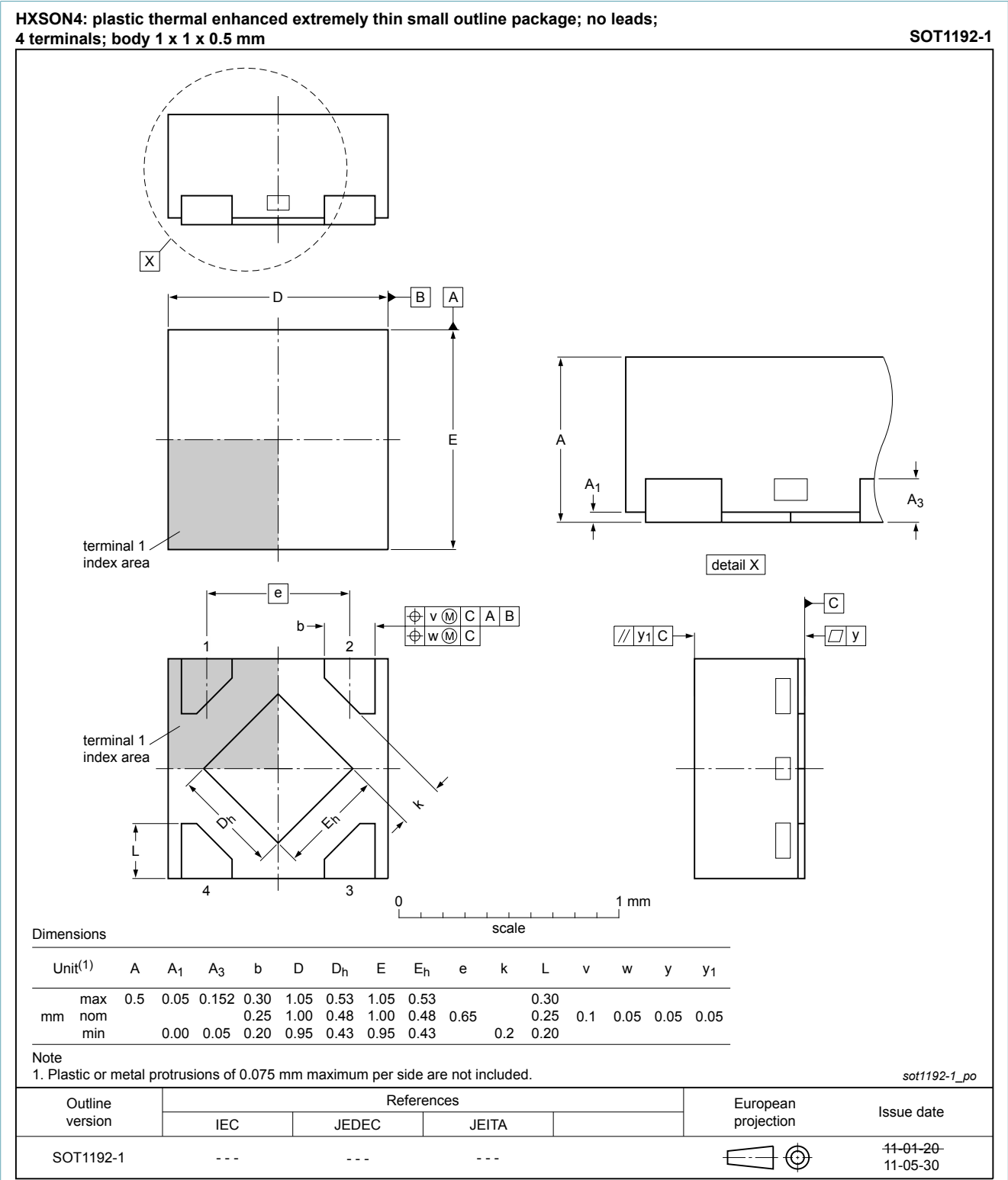
Fig. 1. Package outline HXSON4 (SOT1192-1)
