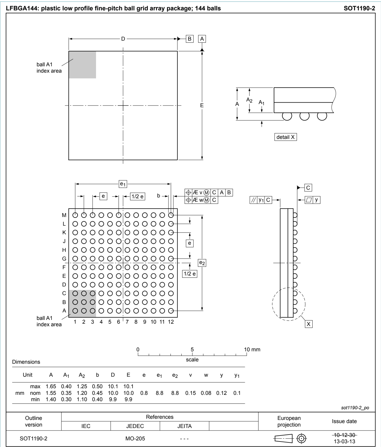
Fig. 1. Package outline LFBGA144 (SOT1190-2)
