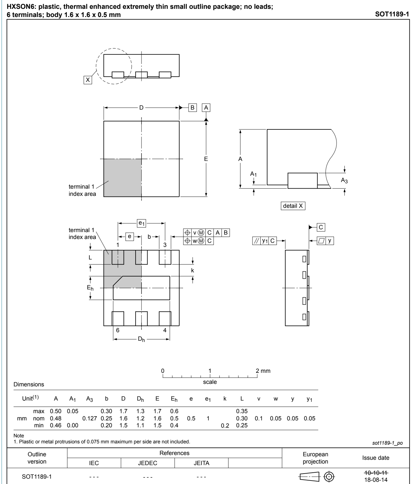
Figure 1. Package outline DFN1616-6 (SOT1189-1)
