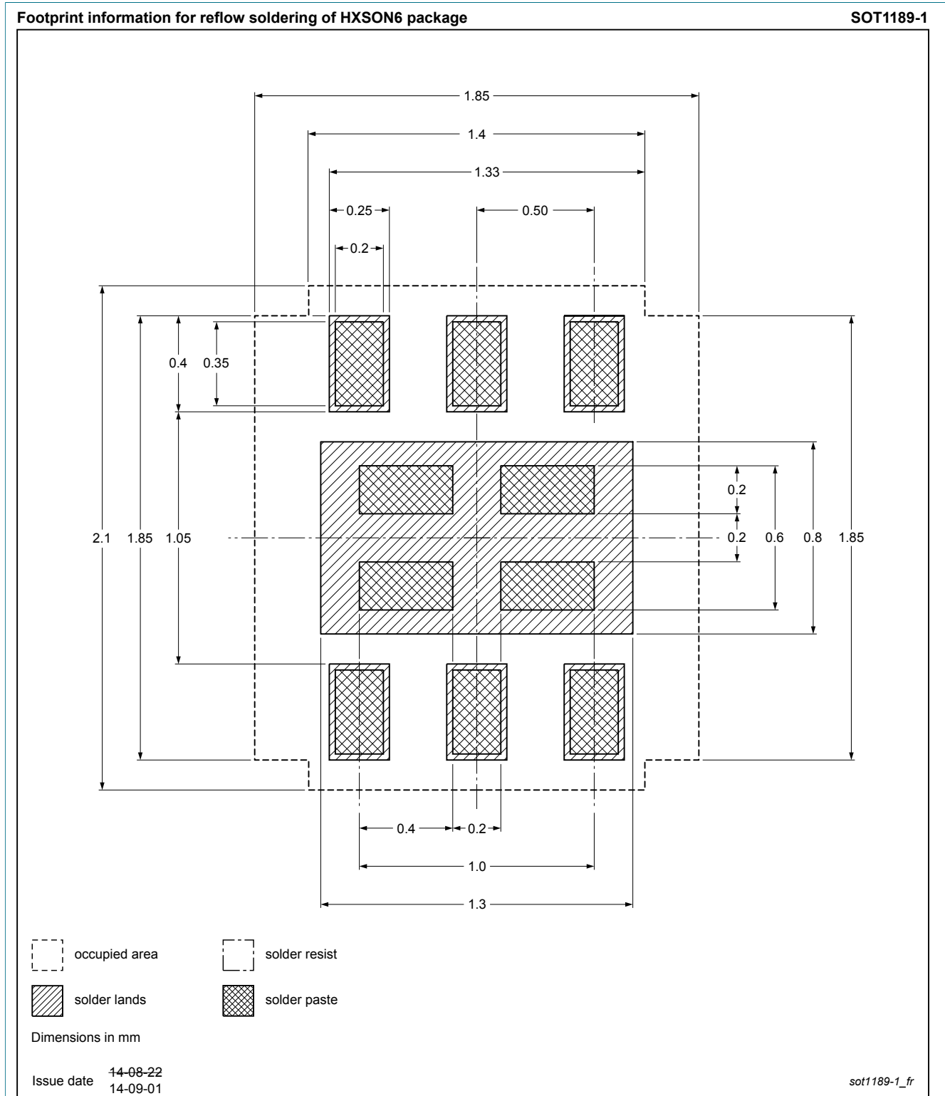
Figure 2. Reflow soldering footprint for DFN1616-6 (SOT1189-1)
