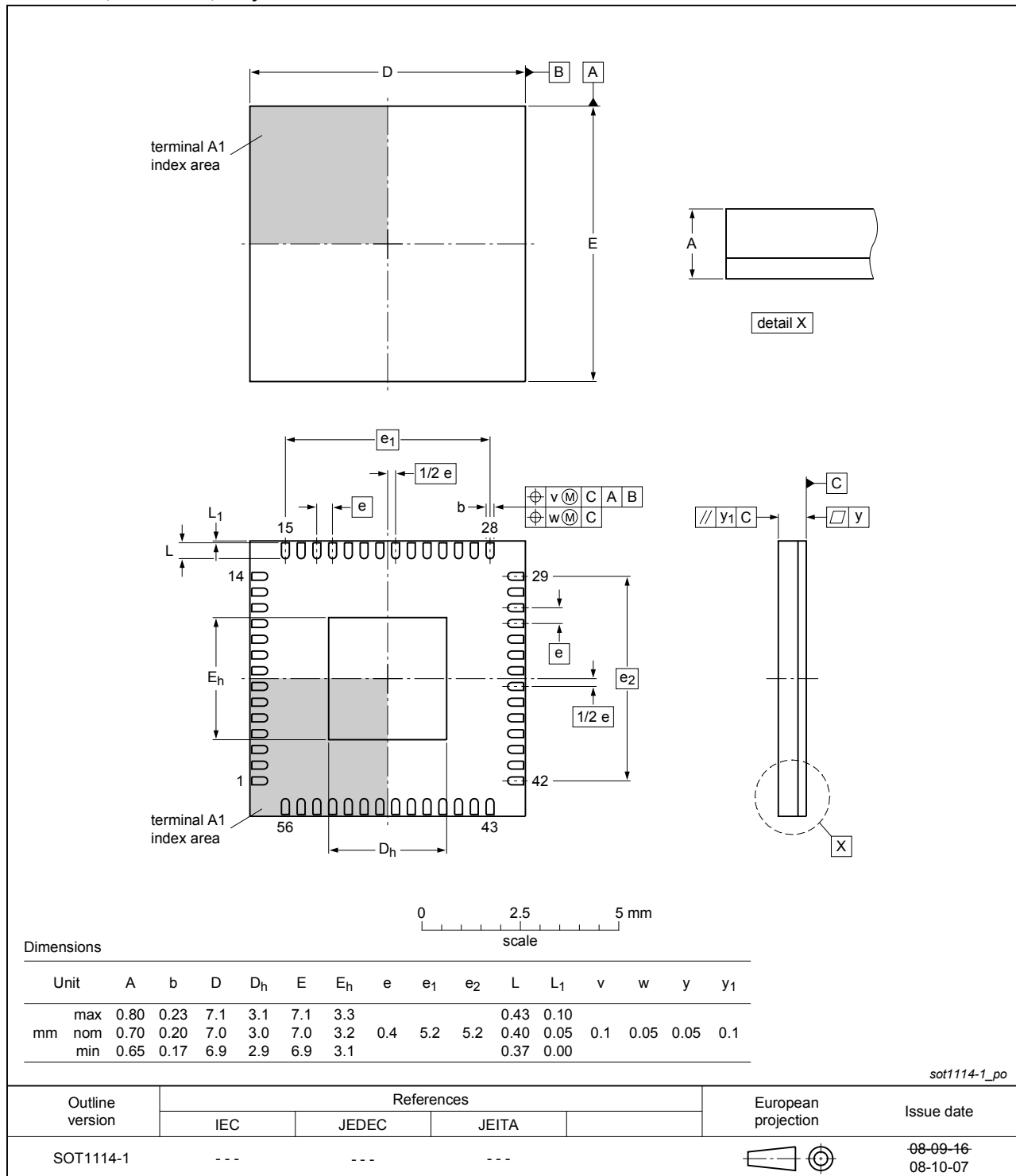
Fig. 1. Package outline HWQFN56R (SOT1114-1)
