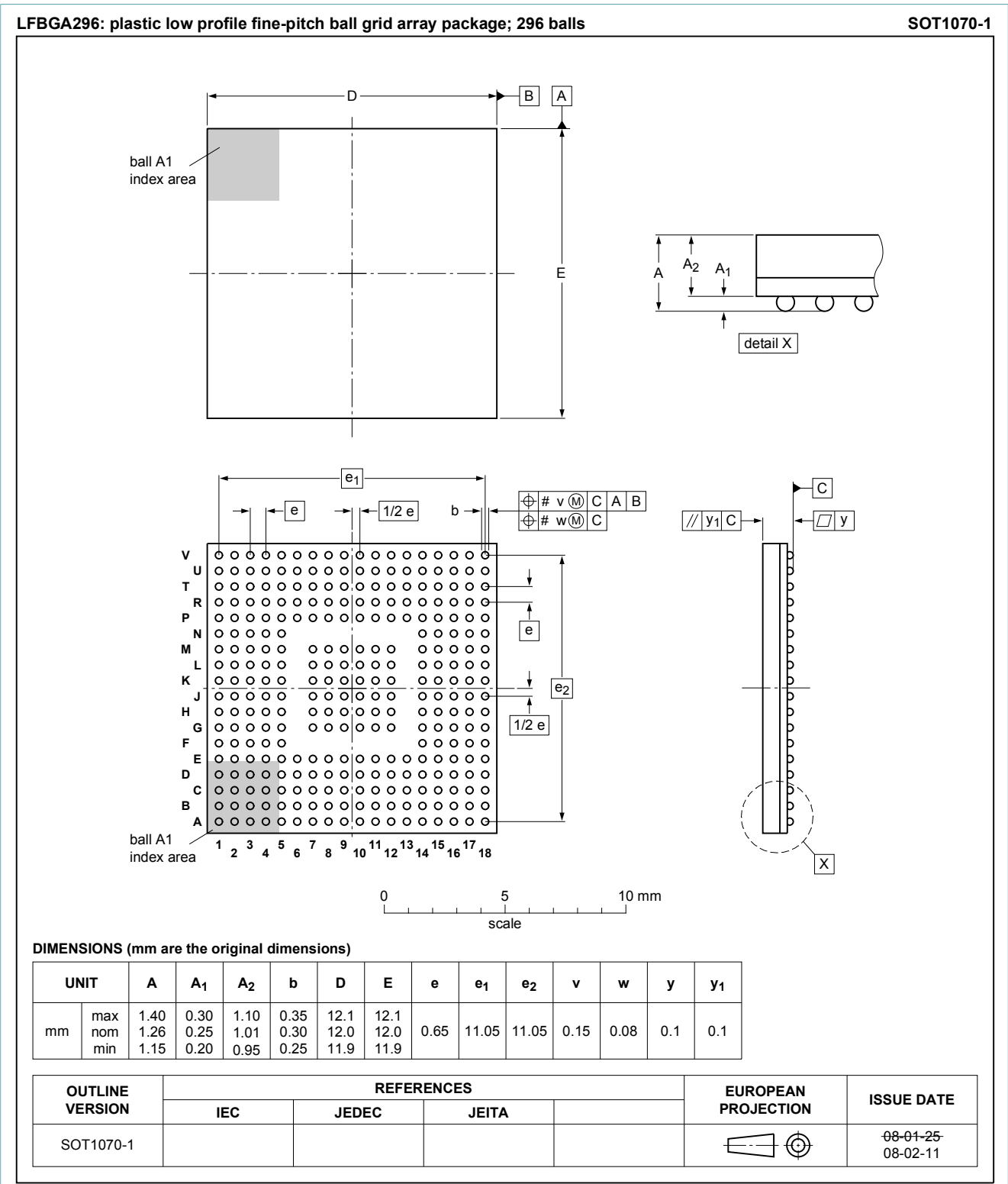
Fig. 1. Package outline LFBGA296 (SOT1070-1)
