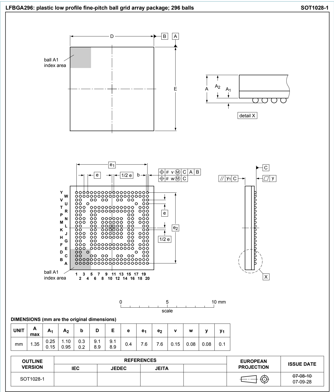
Fig. 1. Package outline LFBGA296 (SOT1028-1)
