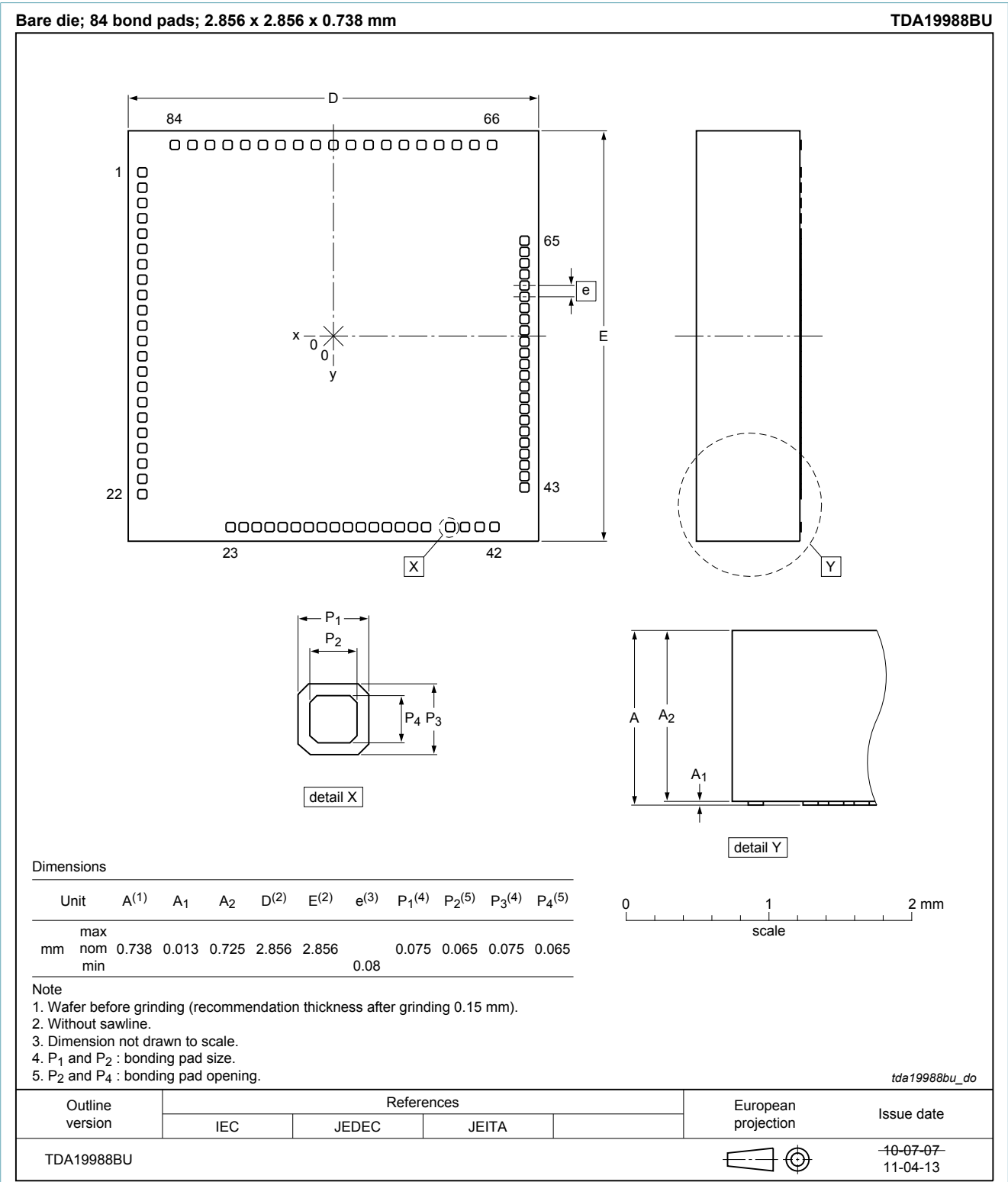
Fig. 1. Package outline UC (OL-TDA19988BU)
