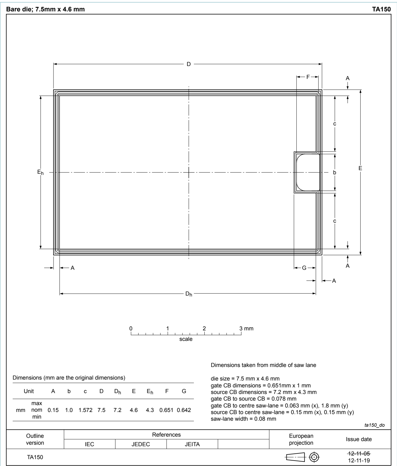
Fig. 1. Package outline UC (OL-TA150KGD)
