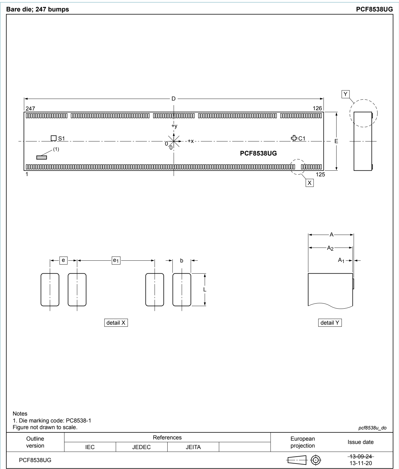
Fig. 1. Package outline UC (OL-PCF8538U)
