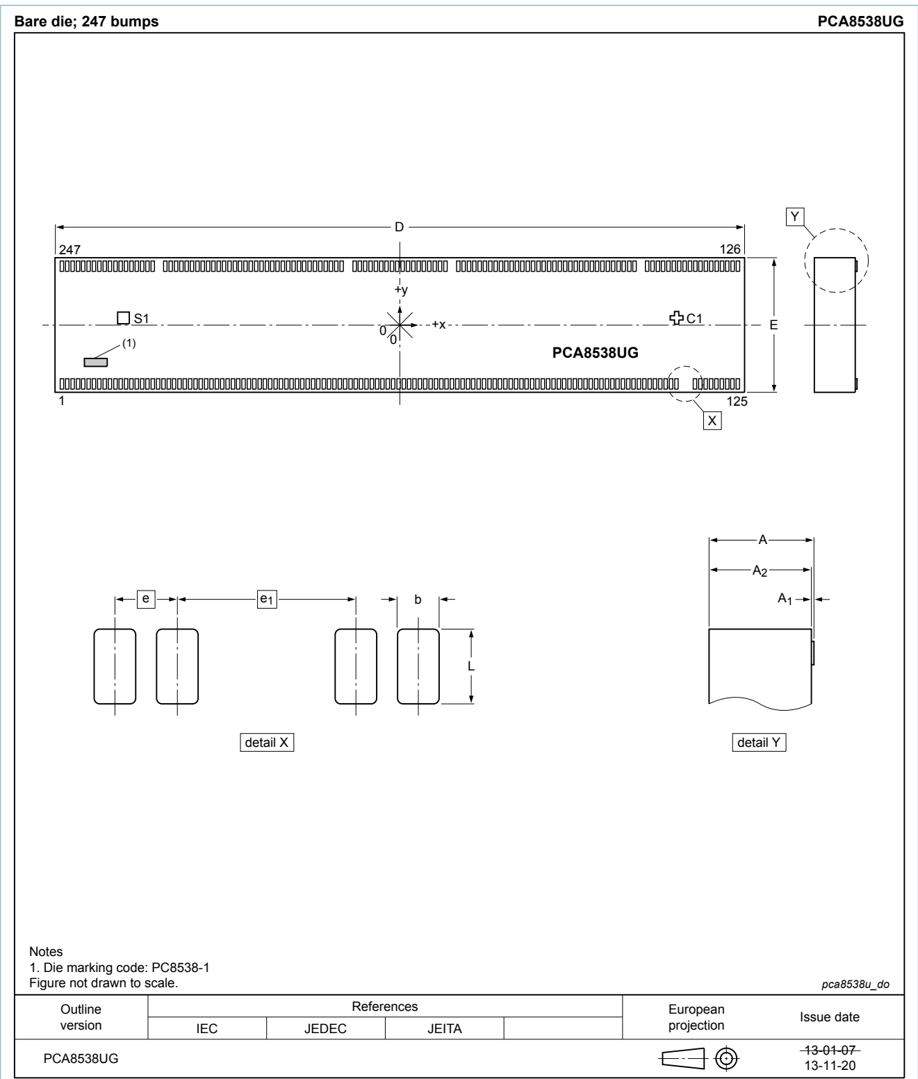
Fig. 1. Package outline UC (OL-PCA8538U)
