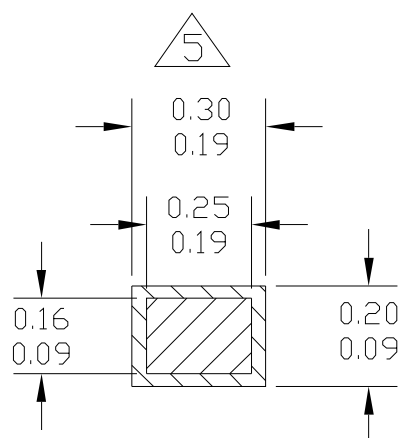
SECTION N-N
