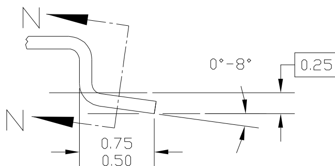
DETAIL E
