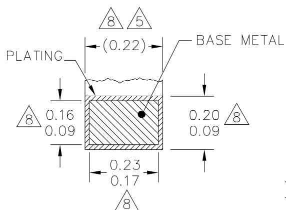
SECTION A-A 176 PLACES ROTATED 90°CLOCKWISE
