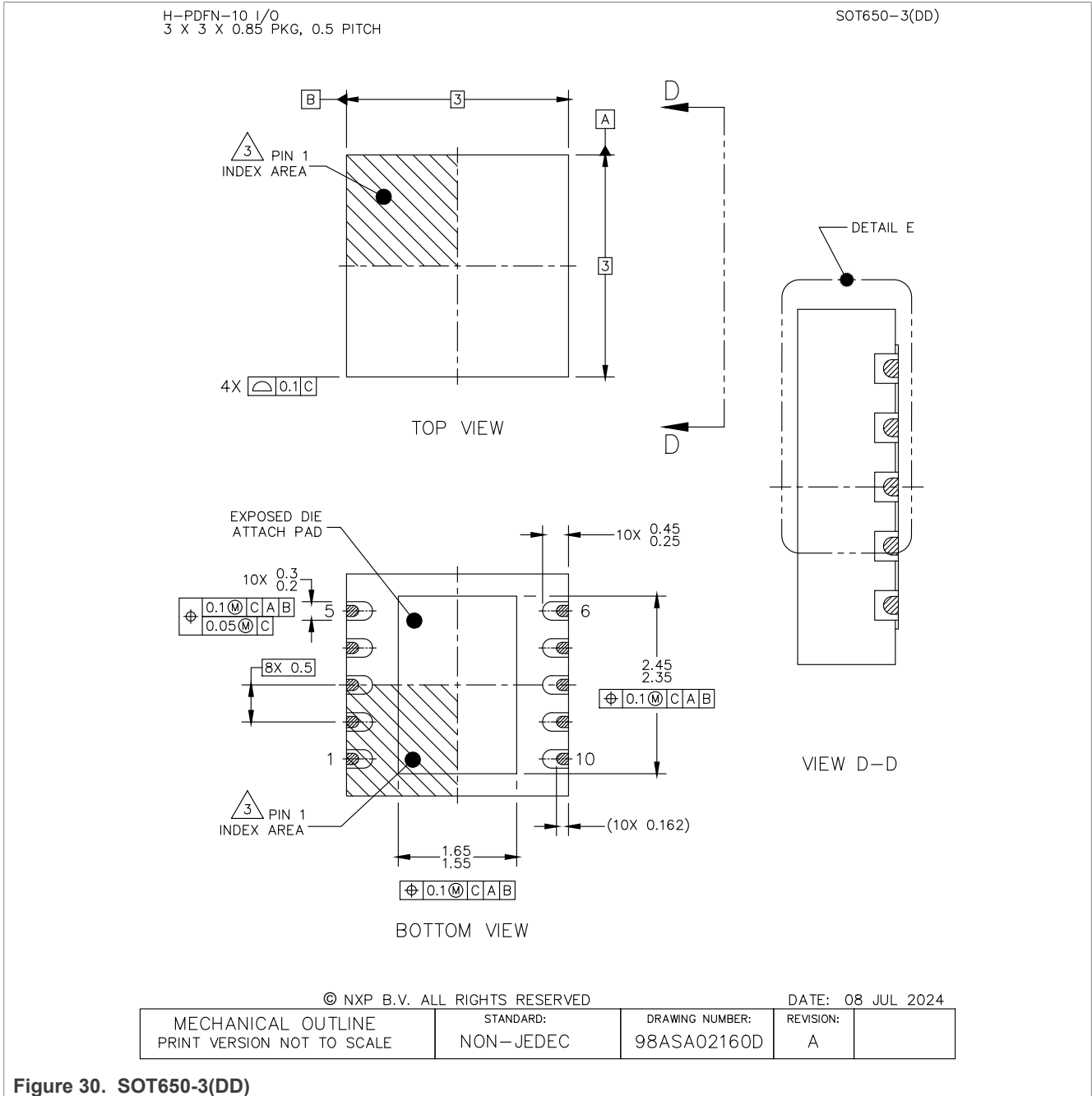
Figure 30. SOT650-3(DD)
