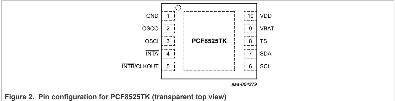
Figure 2. Pin configuration for PCF8525TK (transparent top view)
