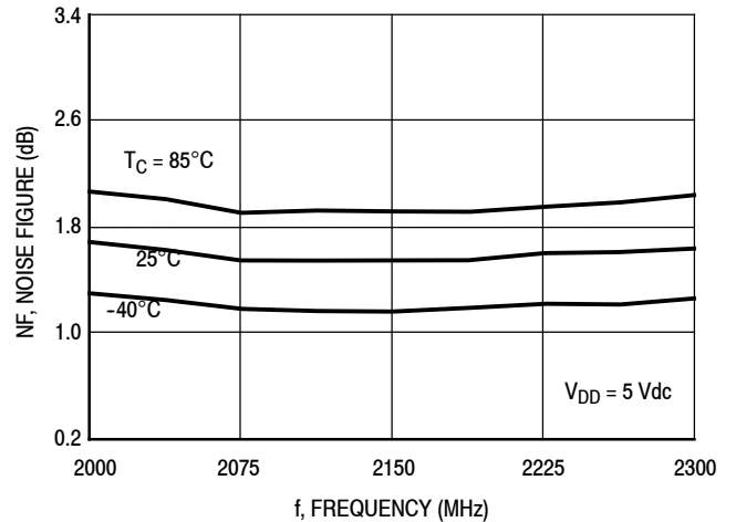
Figure 9. Noise Figure versus Frequency versus Temperature
