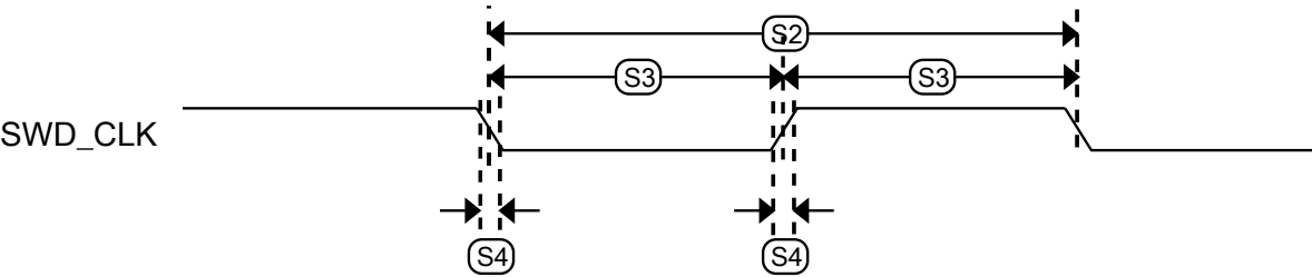
Figure 4. Serial wire clock input timing
