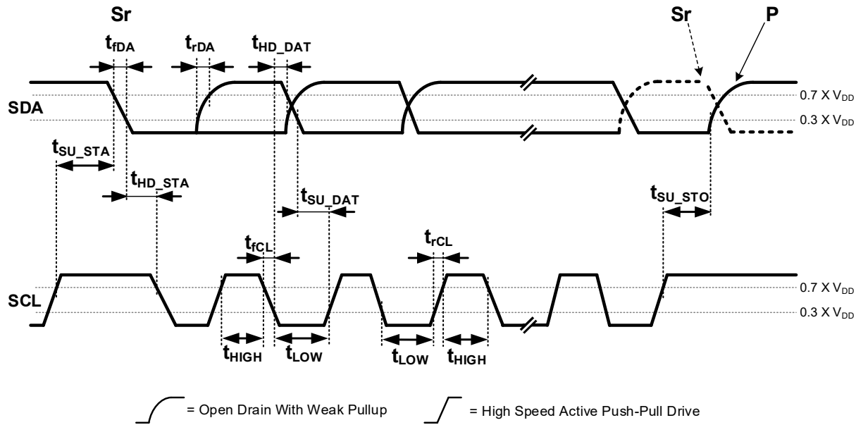
Figure 16. I3C legacy mode timing
