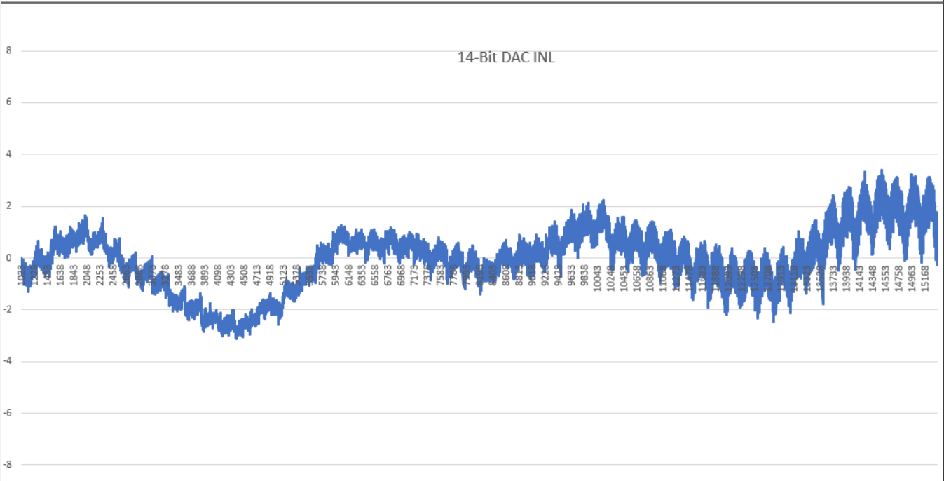
Figure 27. 14-bit DAC INL
