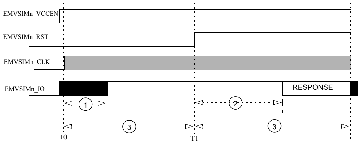
Figure 45. Active-Low-Reset Smart Card Reset Sequence
