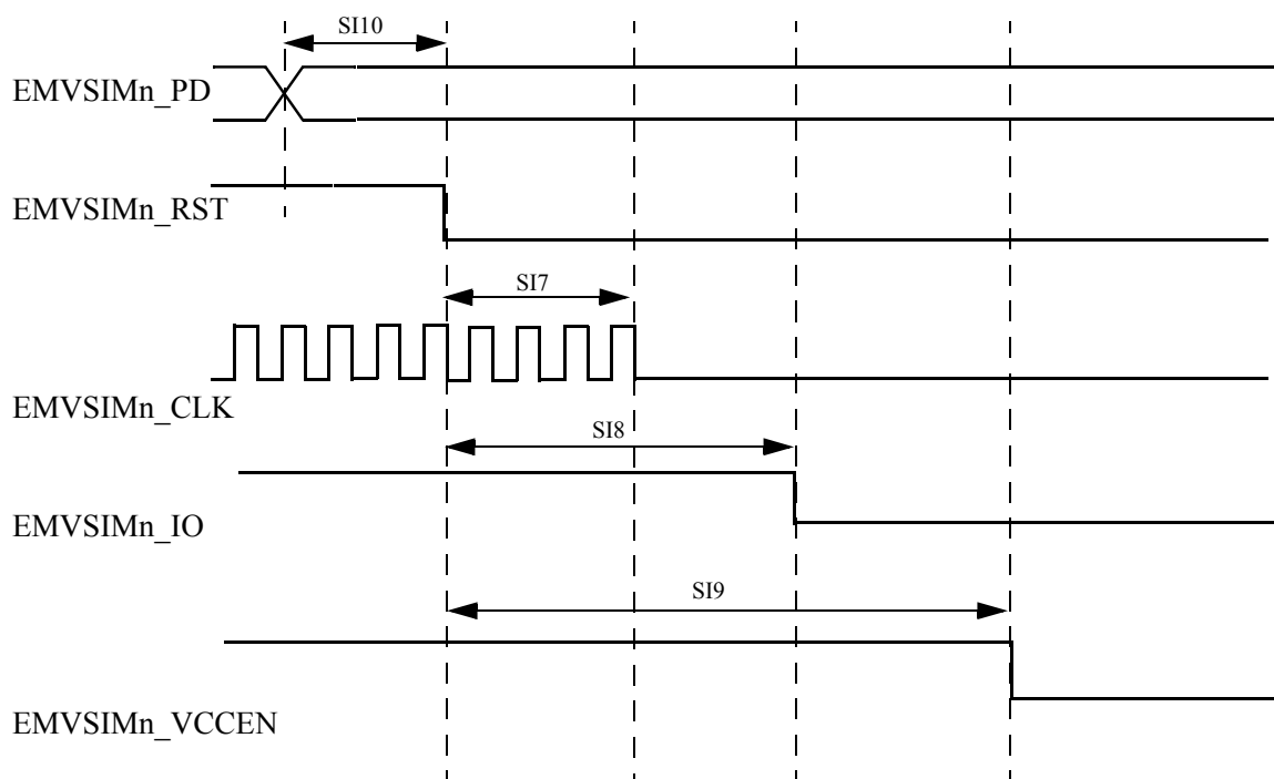
Figure 43. EMV SIM Clock Timing Diagram
