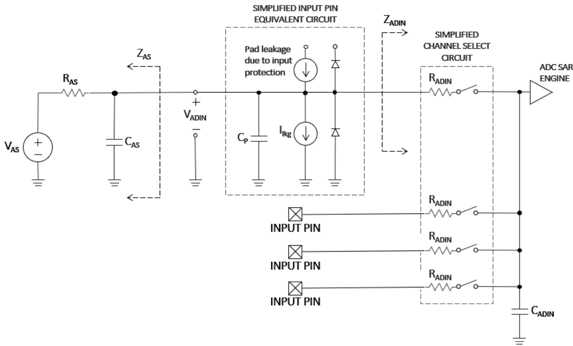
Figure 22. ADC input impedance equivalency diagram
