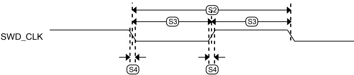
Figure 11. Serial wire clock input timing
