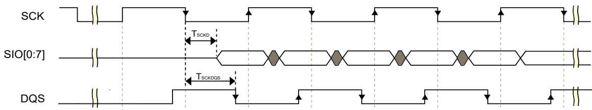
Figure 18. FlexSPI input timing in DDR mode where FlexSPI n _MCR0[RXCLKSRC] = 0x3 (case B1)
