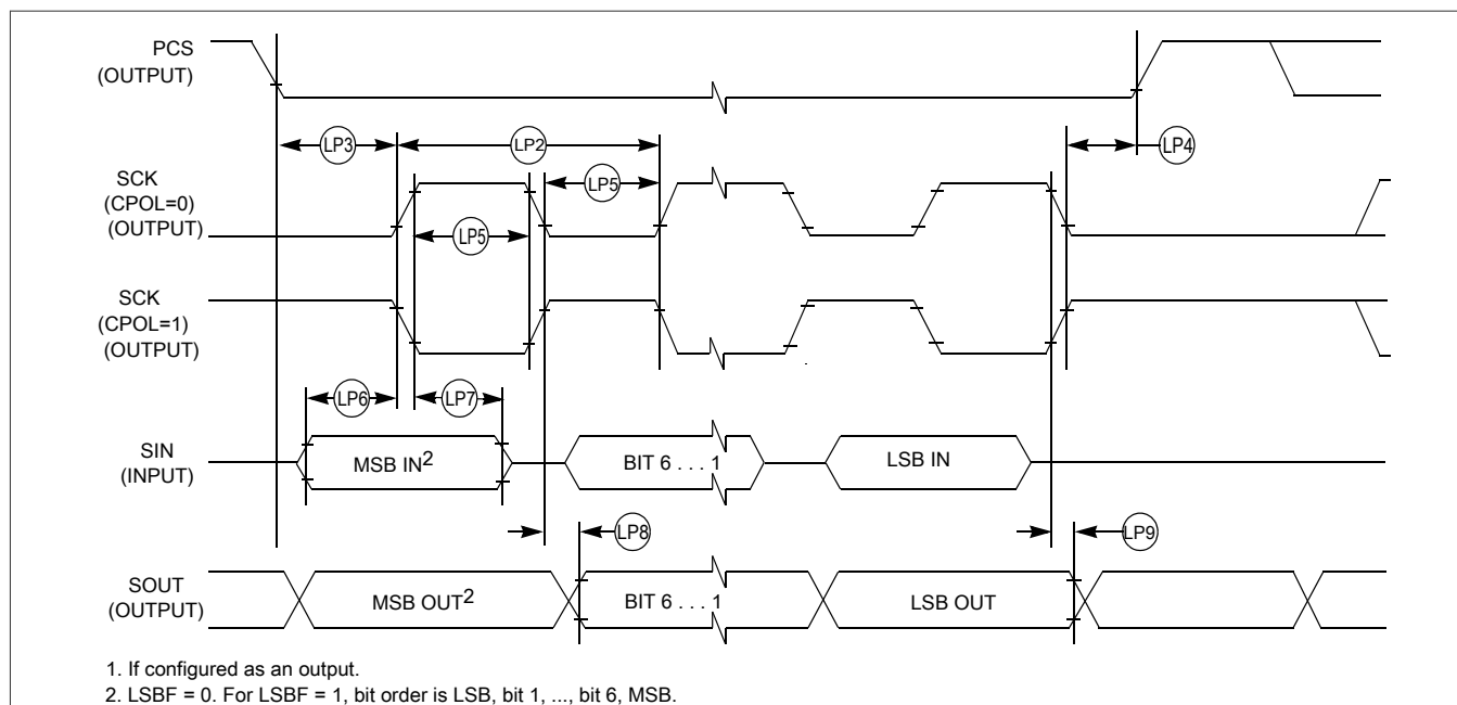
Figure 31. LPSPI master mode timing (CPHA = 0)
