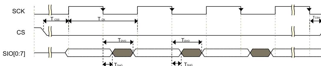
Figure 20. FlexSPI output timing in SDR mode
