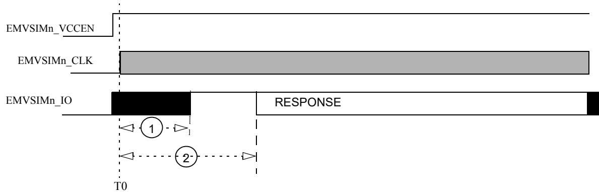
Figure 44. Internal Reset Card Reset Sequence
