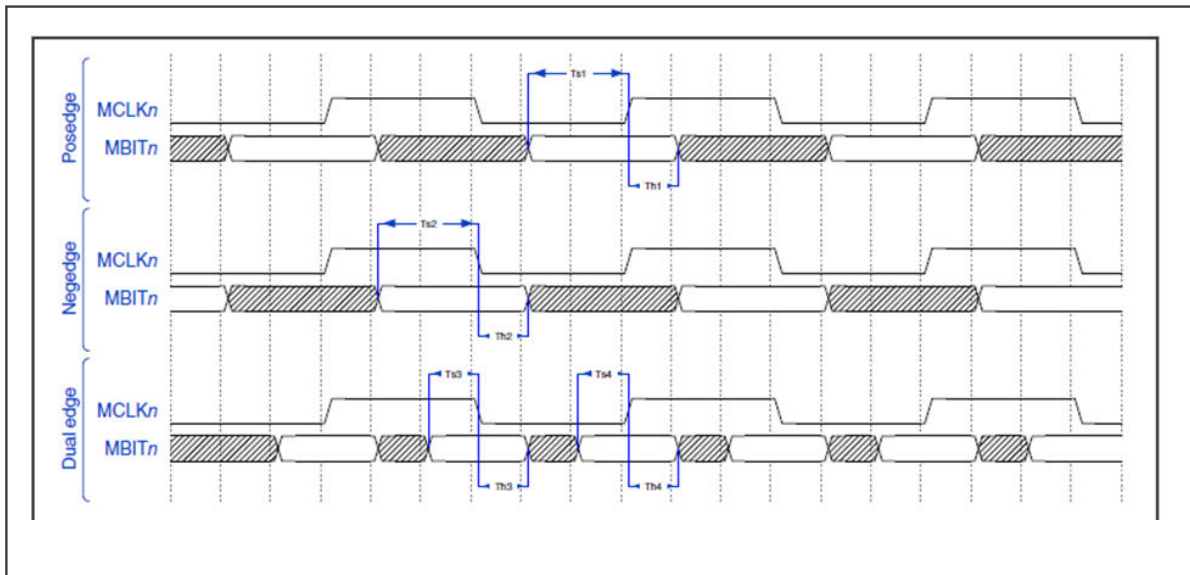
Figure 40. SINC timing
