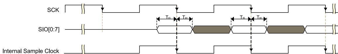
Figure 14. FlexSPI input timing in SDR mode where FlexSPI \eta _MCR0[RXCLKSRC] = 0x0 or 0x1 or 0x2
