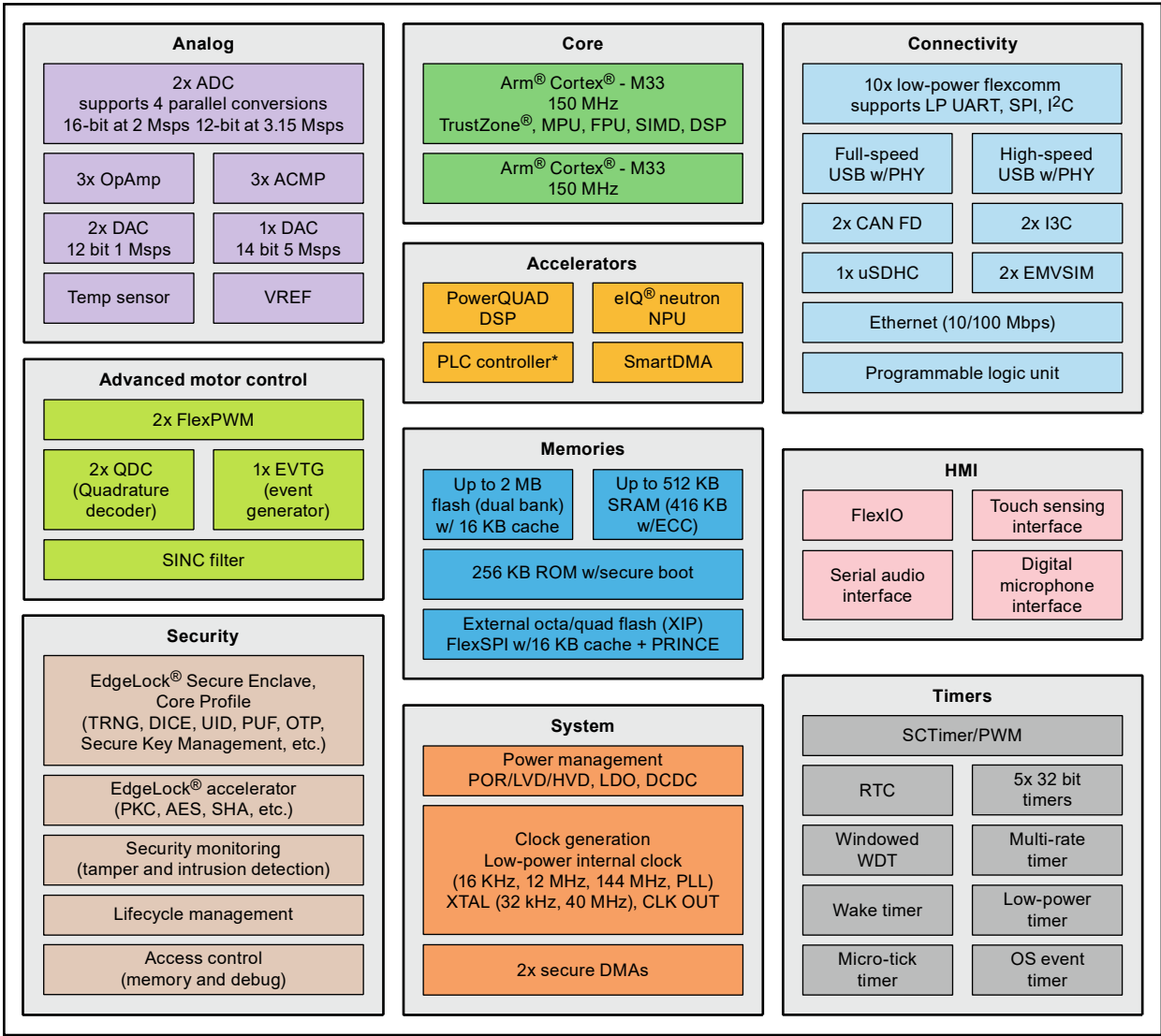
Figure 1. Block diagram
