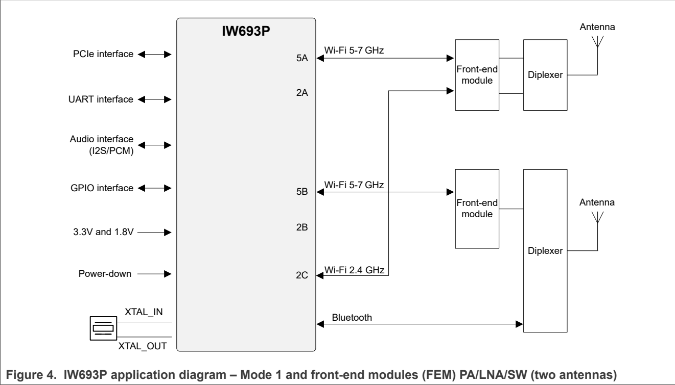
Figure 4 shows IW693P application diagram for mode 1, front-end modules (FEM), and two antennas.
