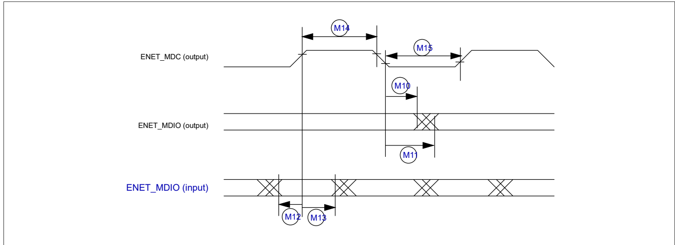
Figure 61. MII serial management channel timing diagram
