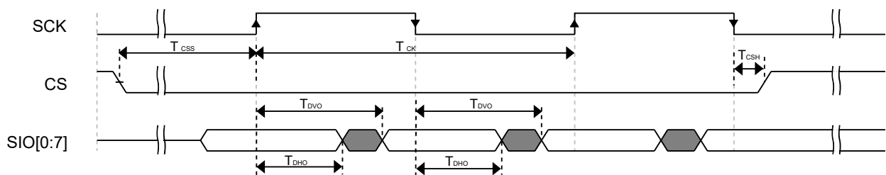
Figure 27. FlexSPI output timing in DDR mode
