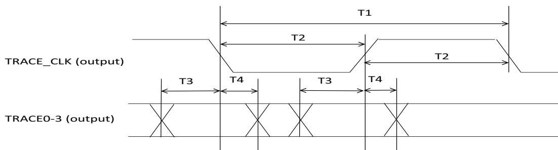
Figure 16. Trace timing
