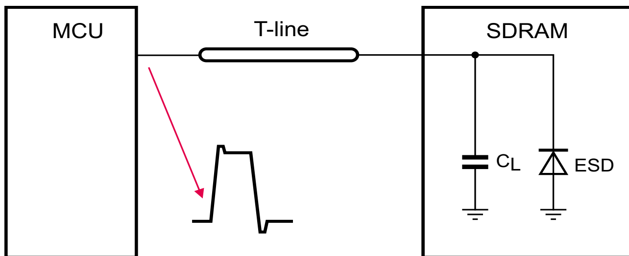
Figure 9. MCU-SDRAM circuit with overshoot/undershoot
